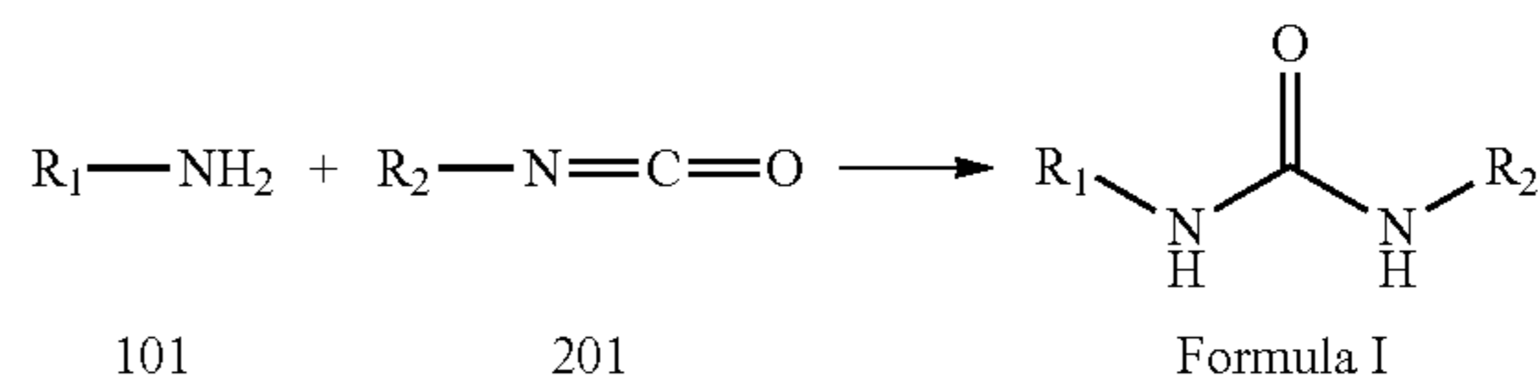
REACTION SCHEME 2
