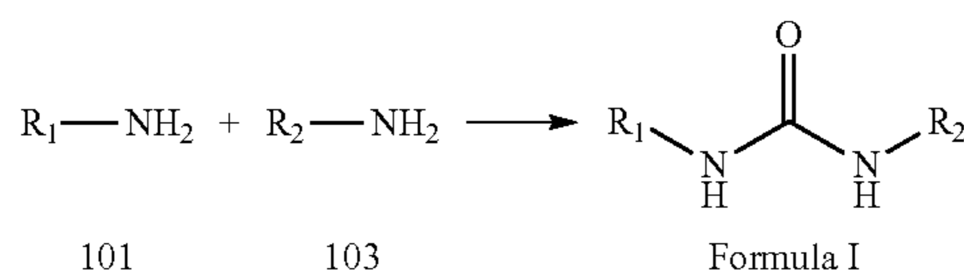
REACTION SCHEME 1
