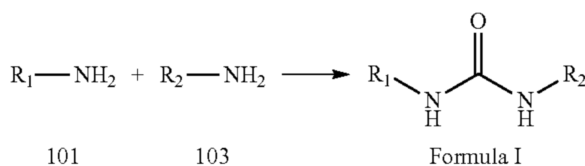
REACTION SCHEME 1
