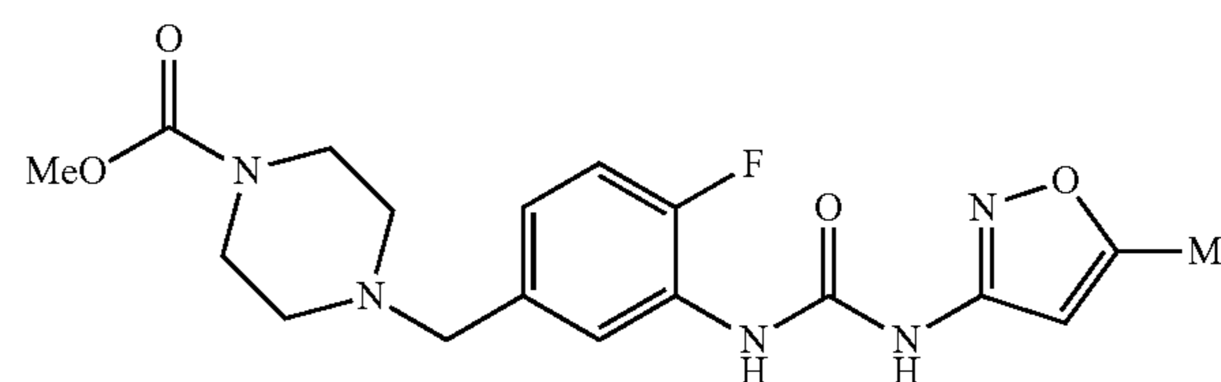
methyl 4-(4-fluoro-3-(3-(5-methylisoxazol-3-yl)ureido)benzyl)piperazine-1-carboxylate
