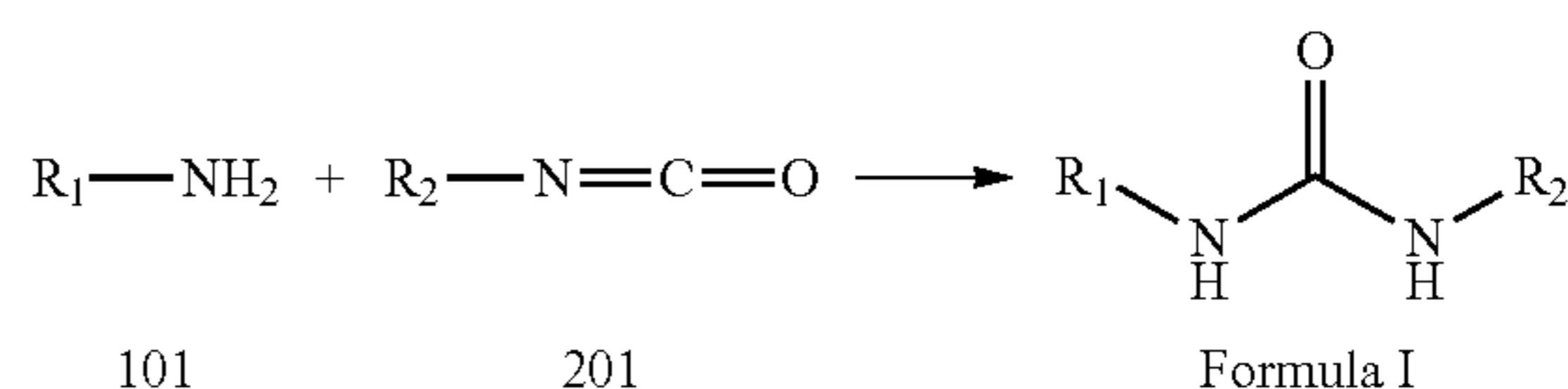
REACTION SCHEME 2
