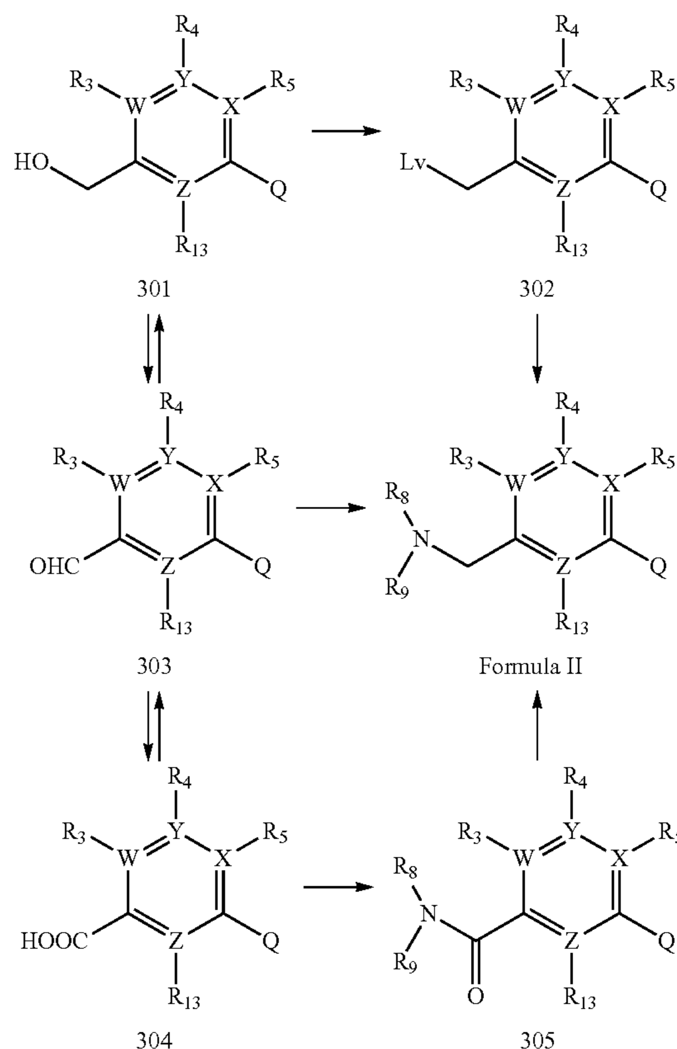
REACTION SCHEME 3
