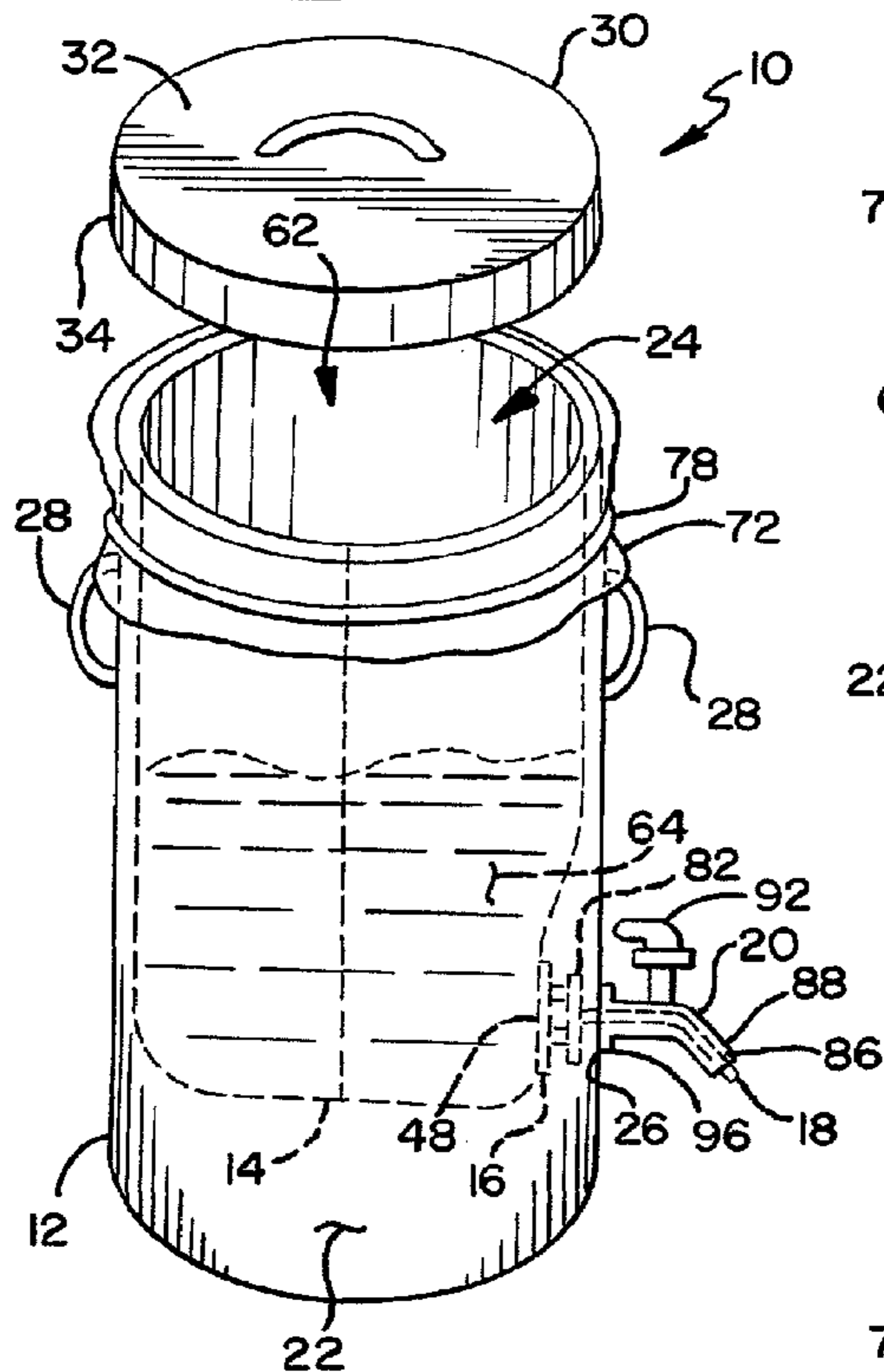
FIG. 1 PRIOR ART
