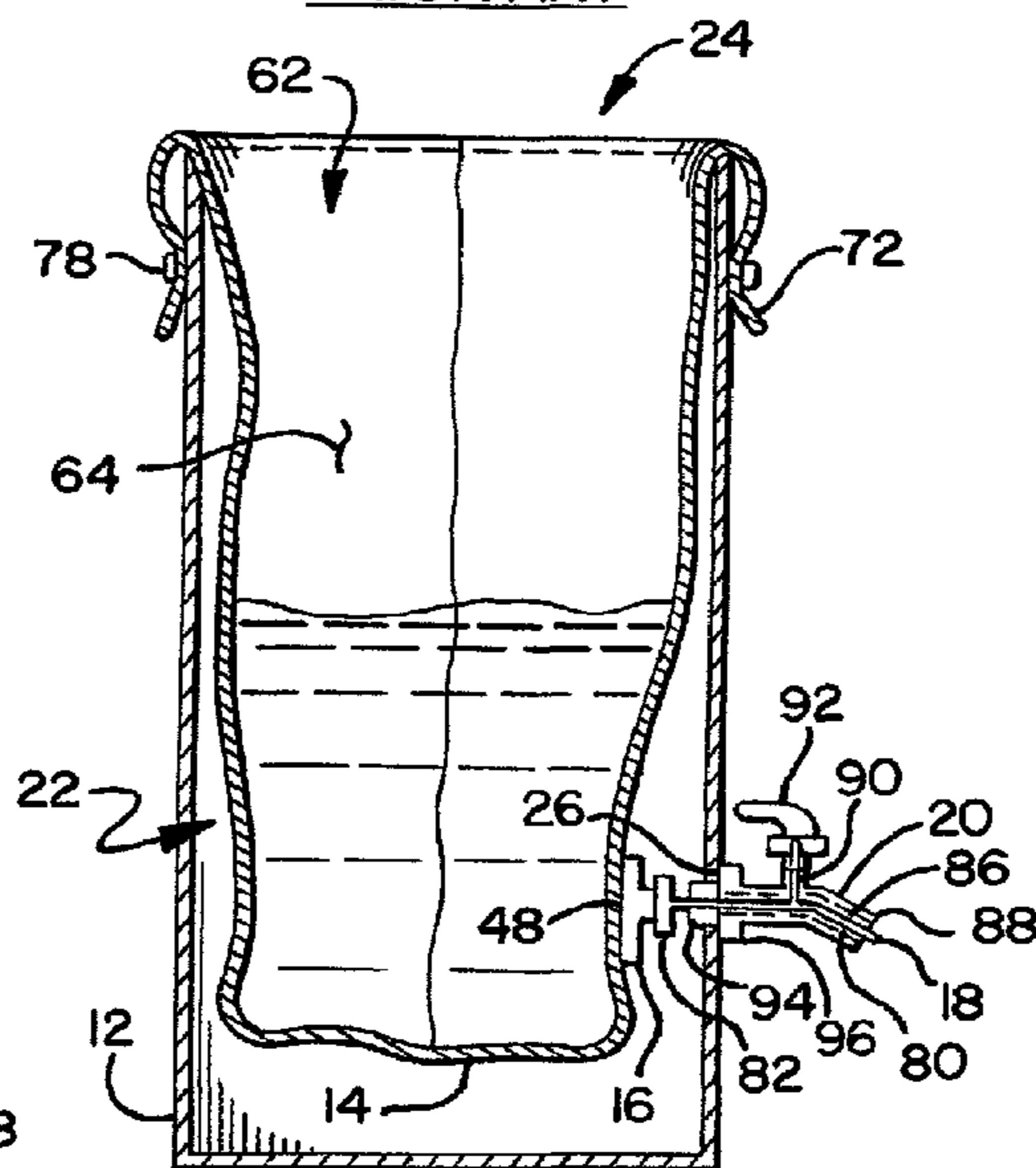
FIG. 2 PRIOR ART
