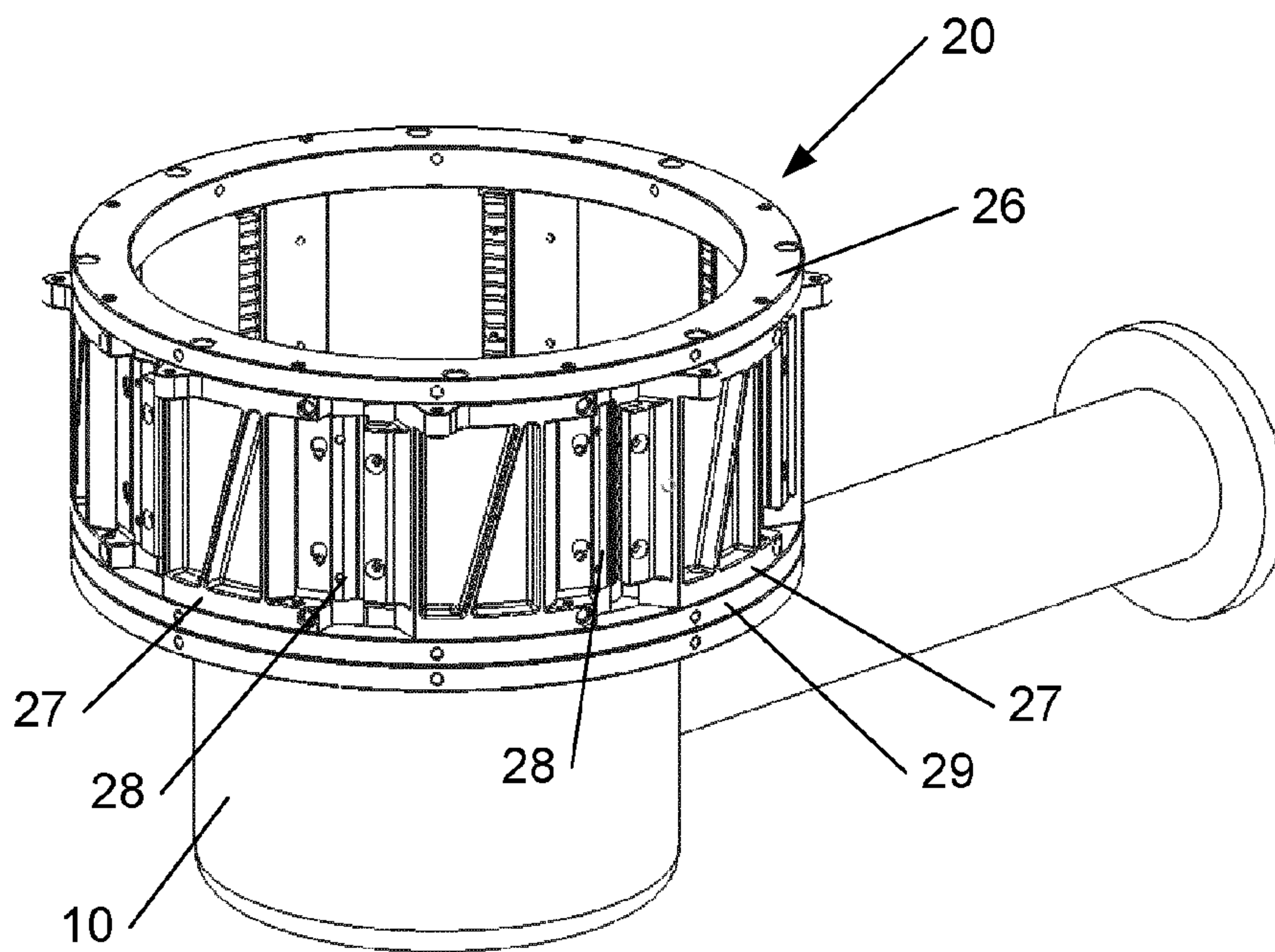
Fig. 2 (prior art)
