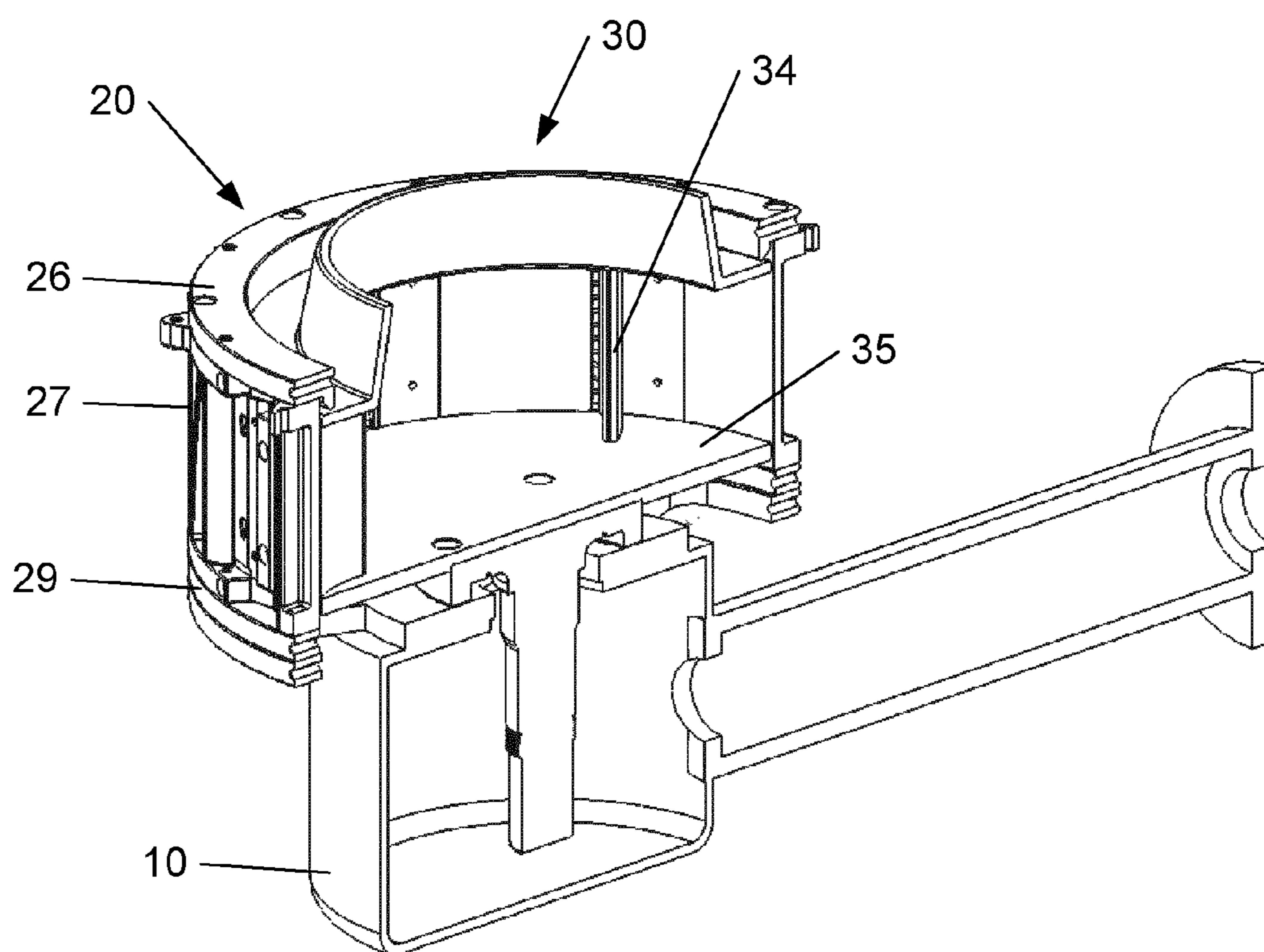
Fig. 3 (prior art)
