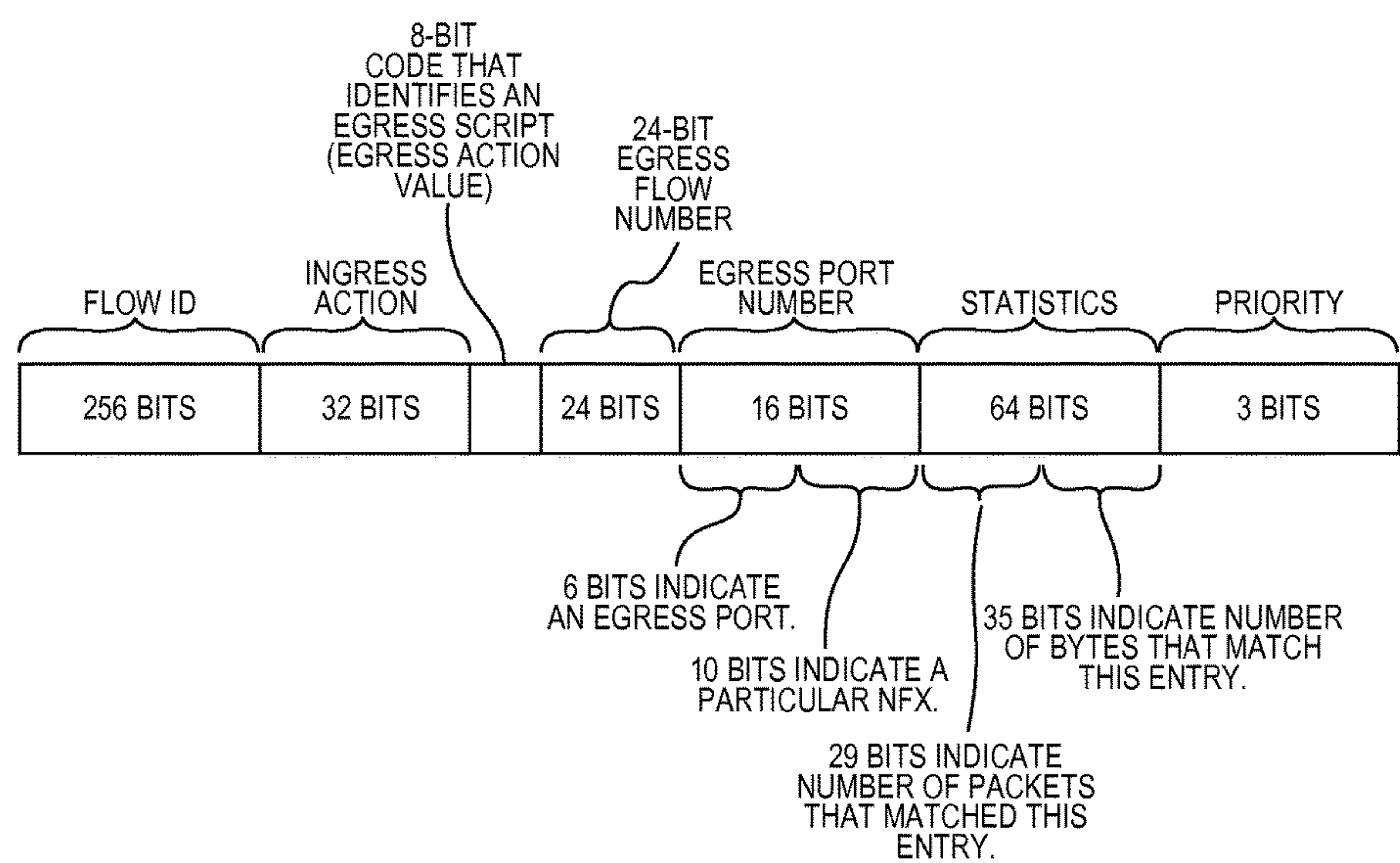
FLOW ID (FOR PACKET TYPE C TO PACKET TYPE B CONVERSION EXAMPLE) FIG. 30
