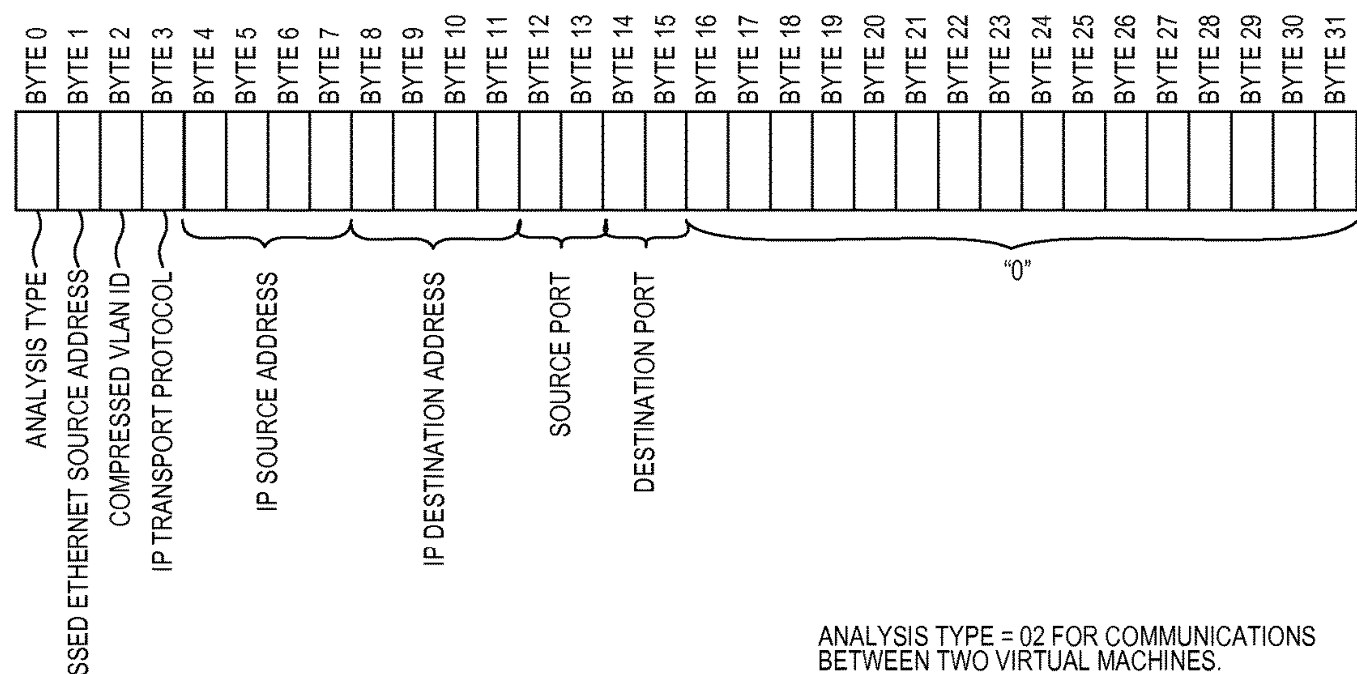
FLOW ID (FOR PACKET TYPE C TO PACKET TYPE B CONVERSION EXAMPLE) FIG. 30
