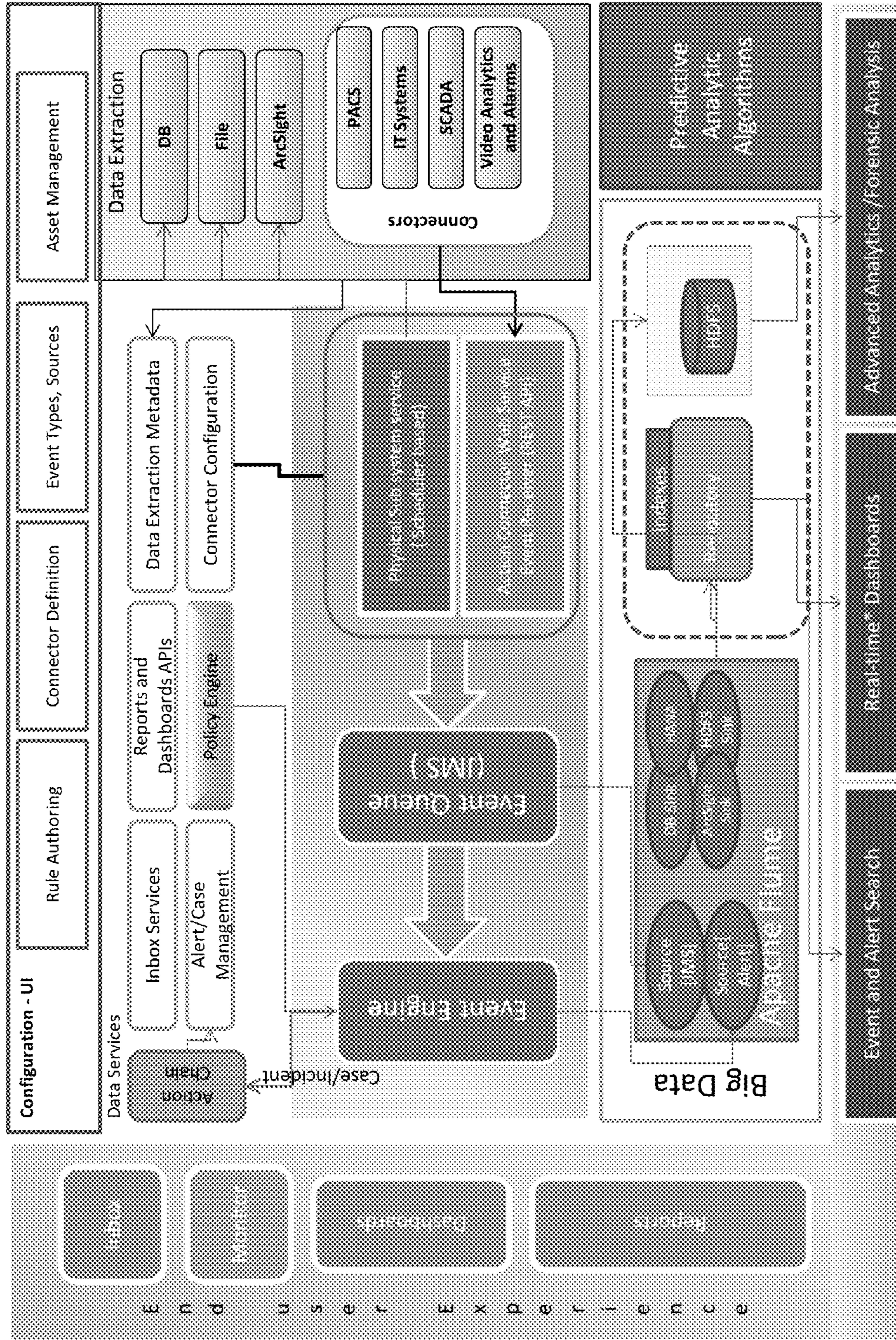
FIG. 30 (Technical Architecture)
