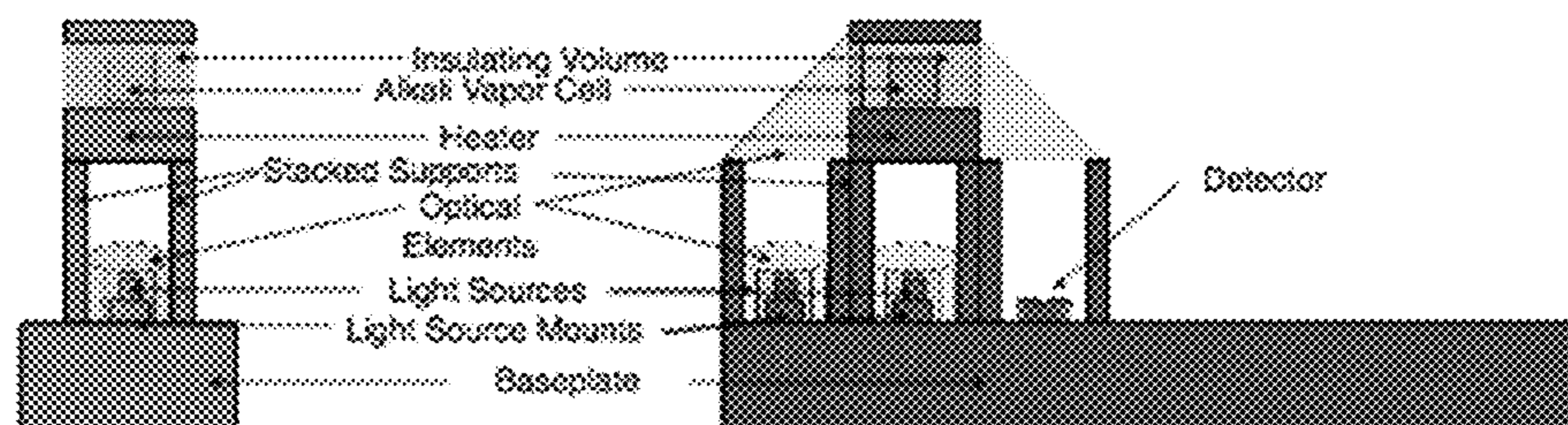
End View
