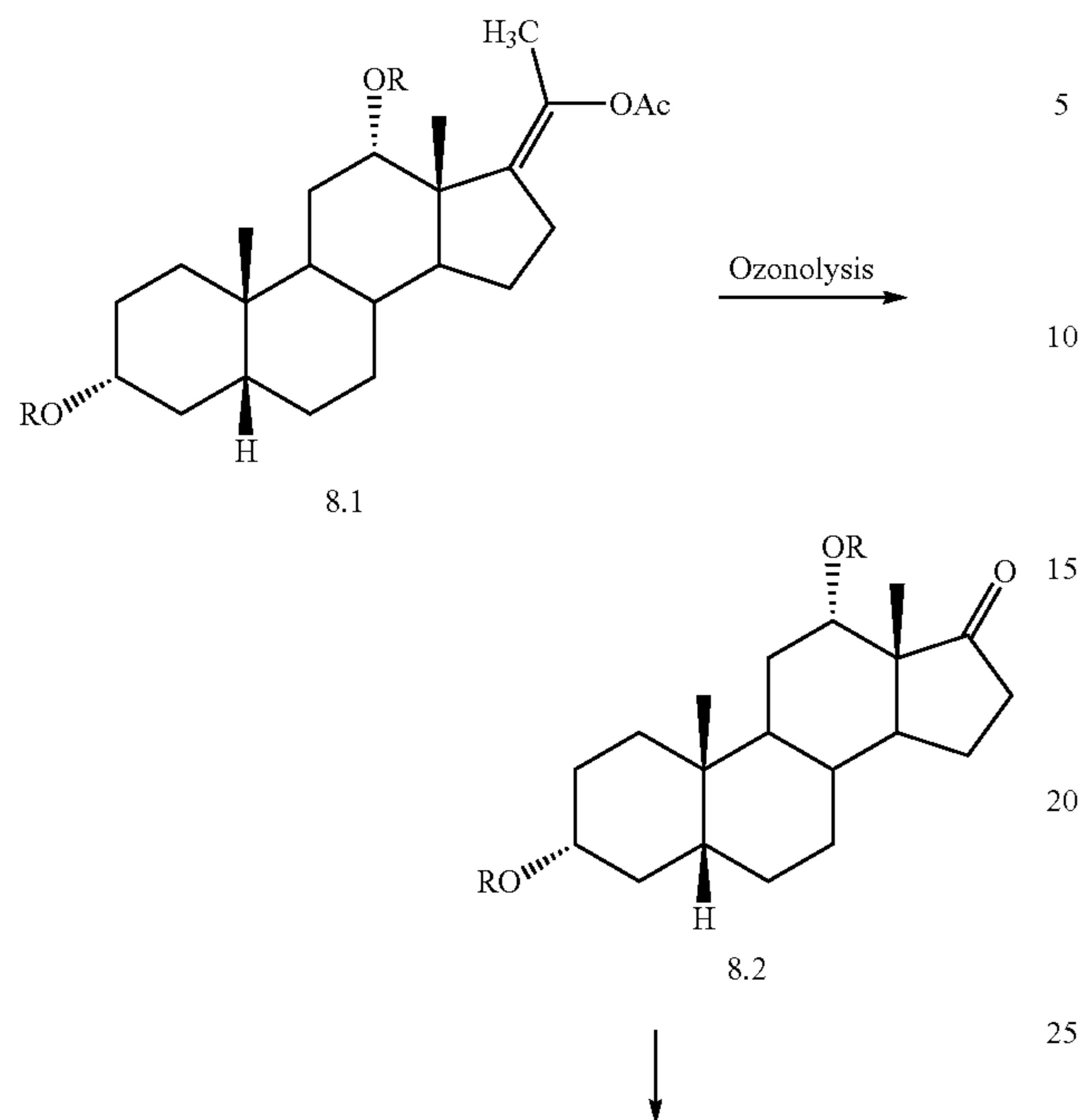
Scheme 8. Side-chain introduction
