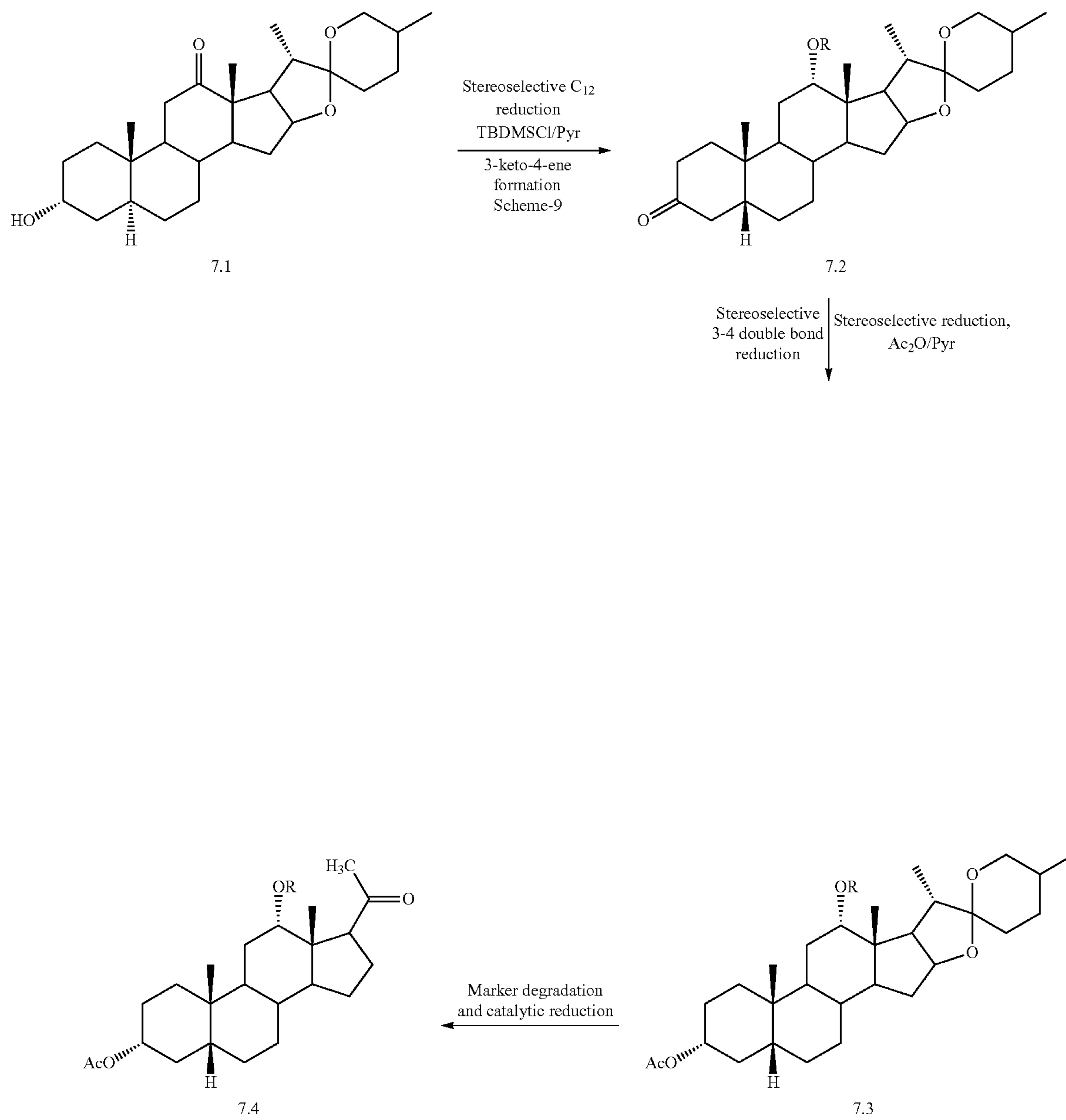
Scheme 7. C 12 -hydroxyl group introduction, AB ring modification and side chain cleavage
