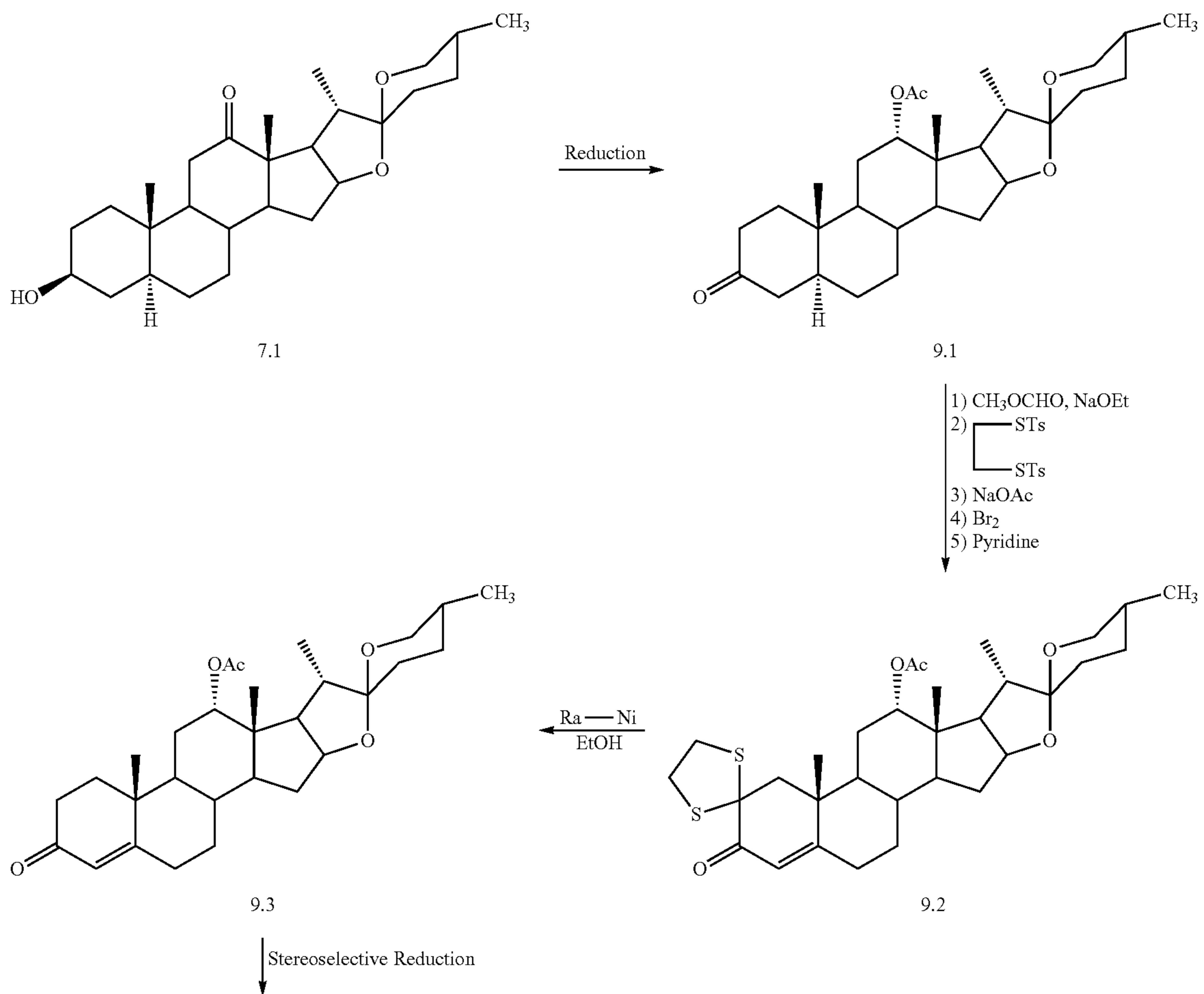
Scheme 9. Dithioethane route to 3-keto-4-ene
