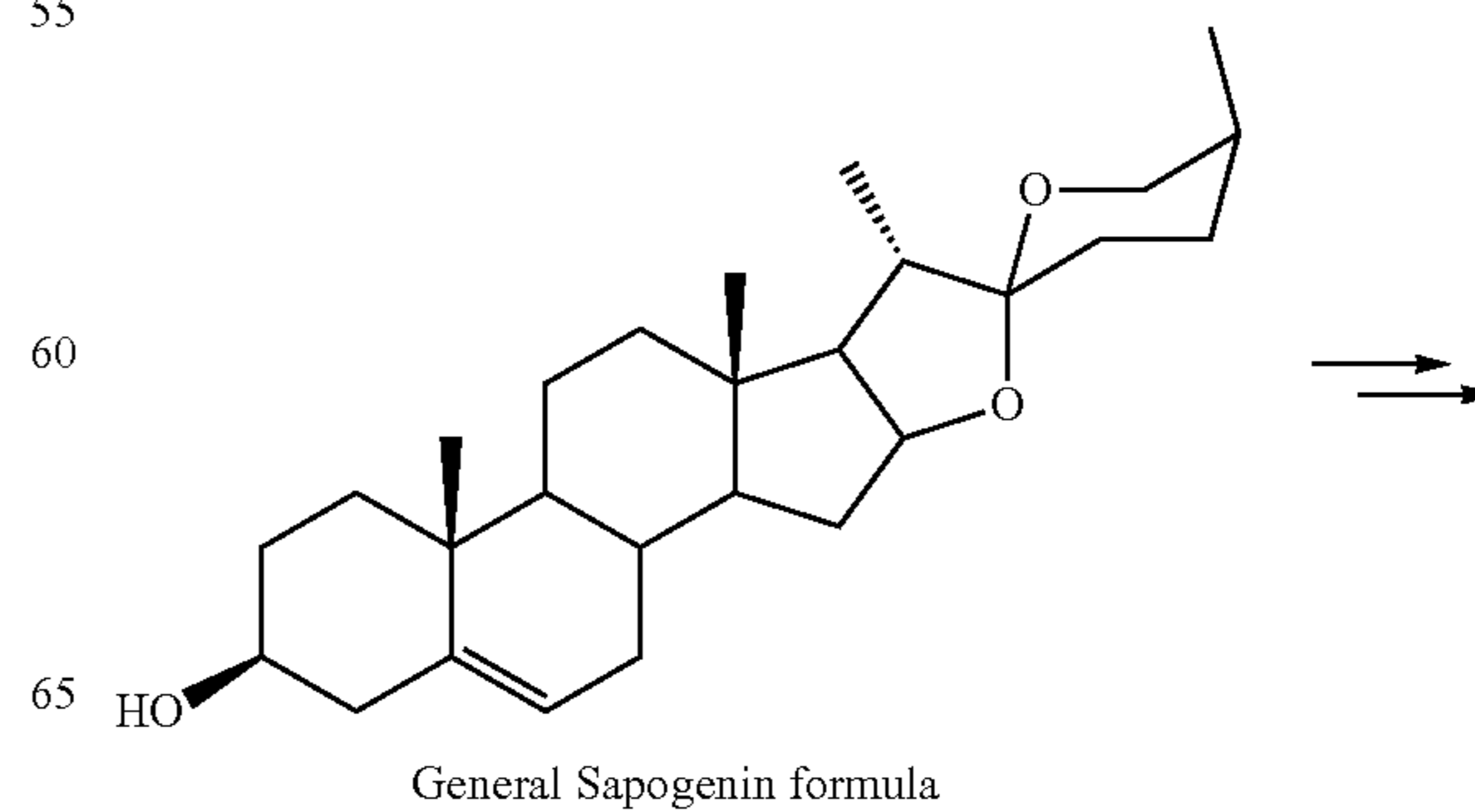
Scheme 10B. Synthetic route from saponin.
