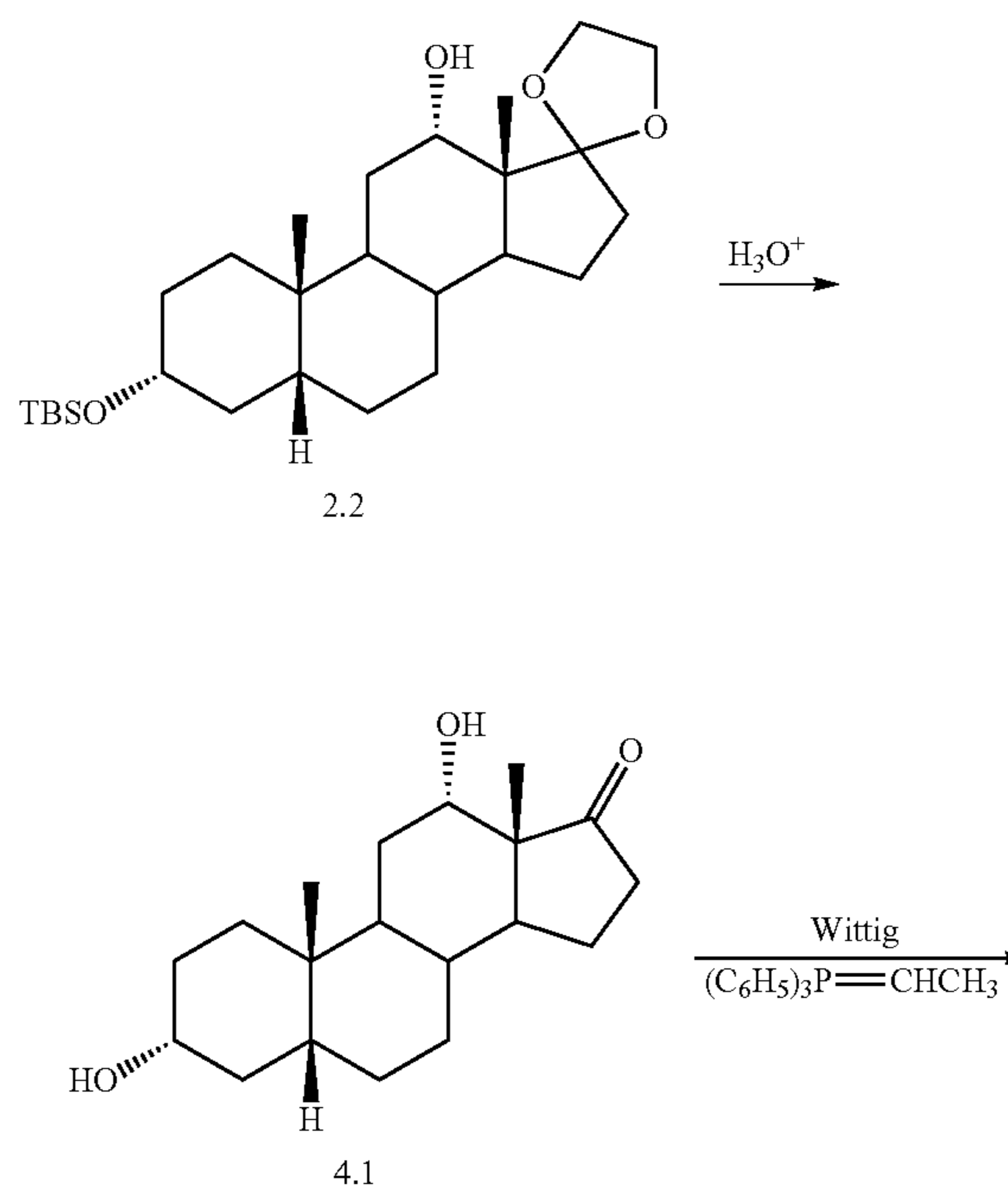
Scheme 4. Deprotection and Wittig Reaction
