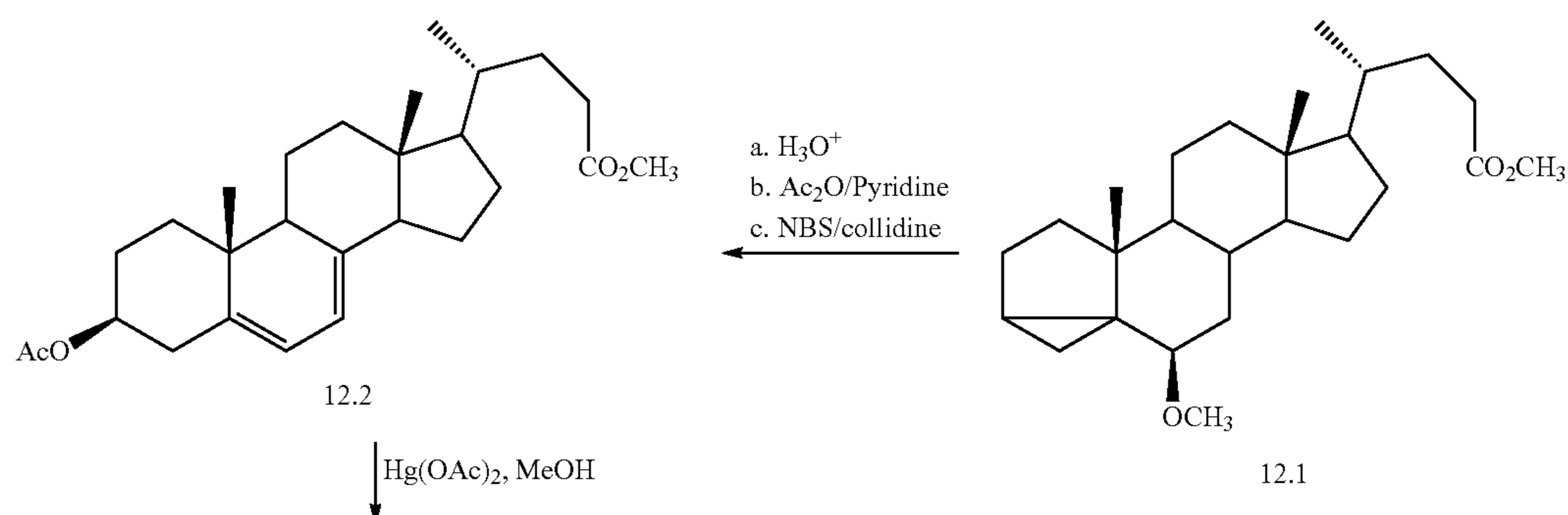
Scheme 12. Triene formation and allylic oxidation
