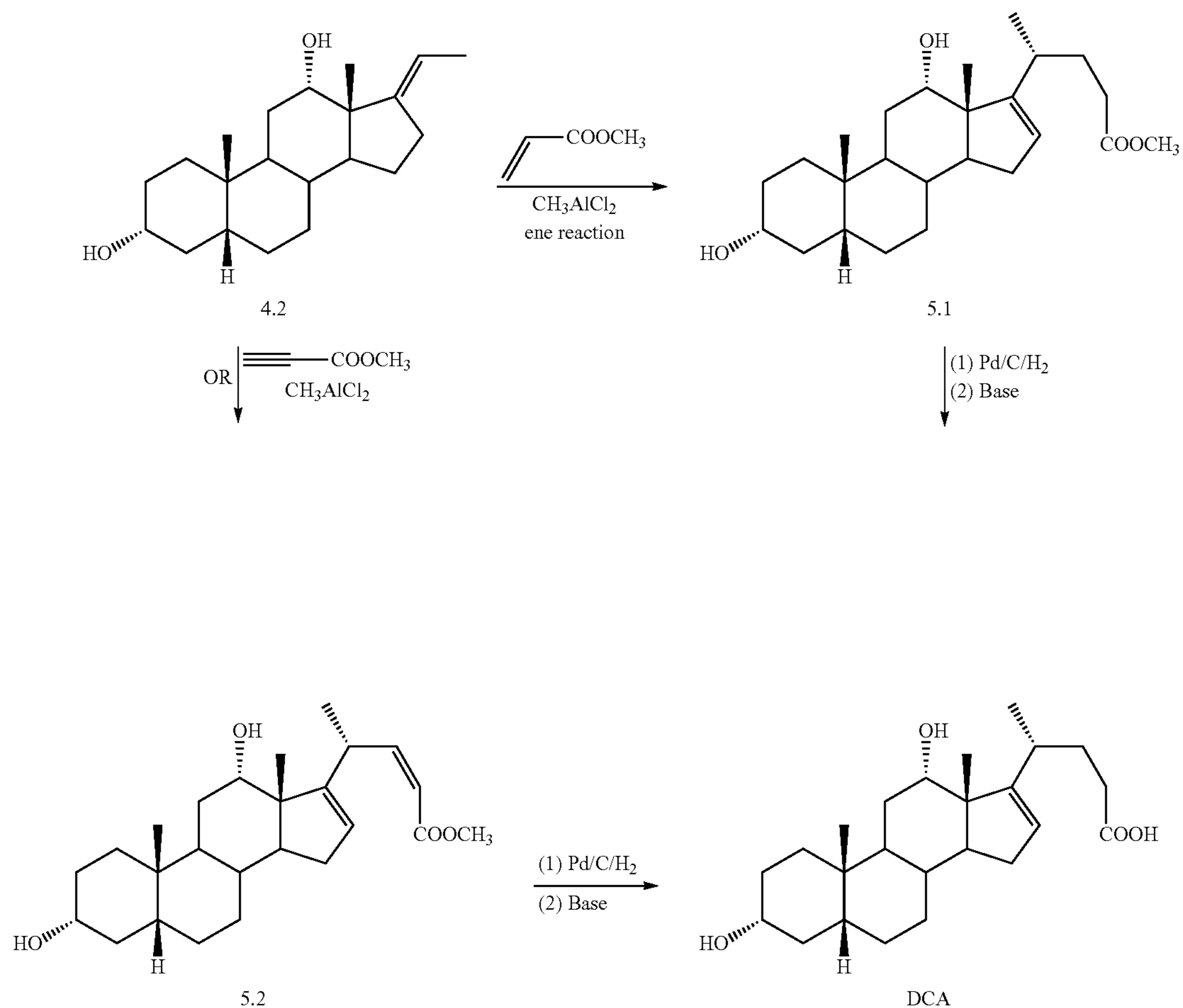
Scheme 5. Ene reaction and catalytic reduction for installation of DCA side chain
