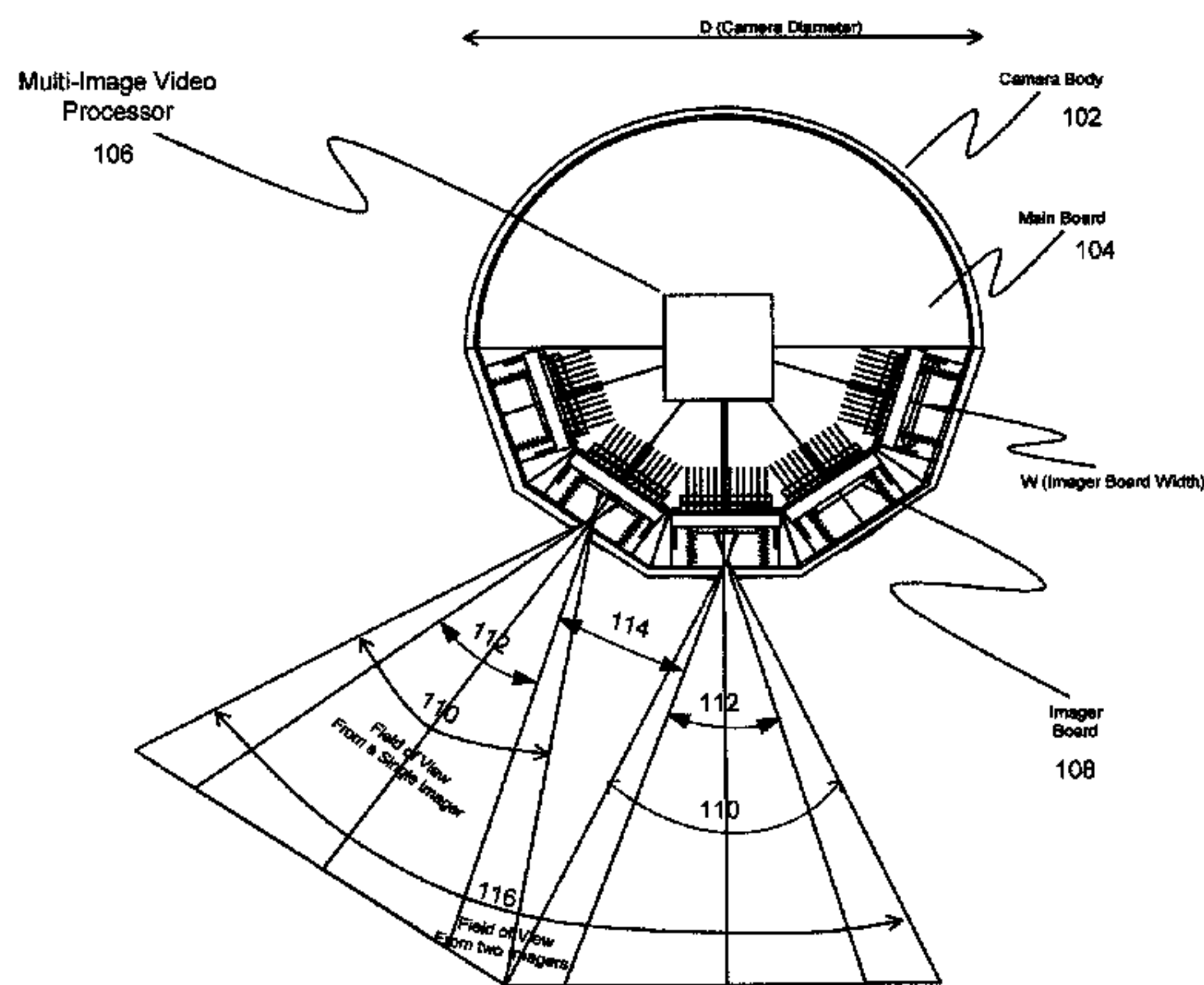
(top schematic view)
