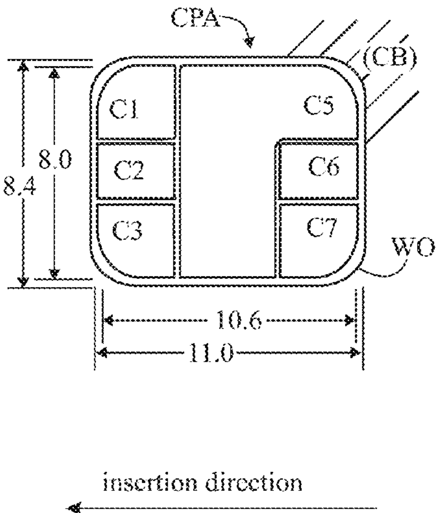
FIG. 1C 6-pad contact pattern
