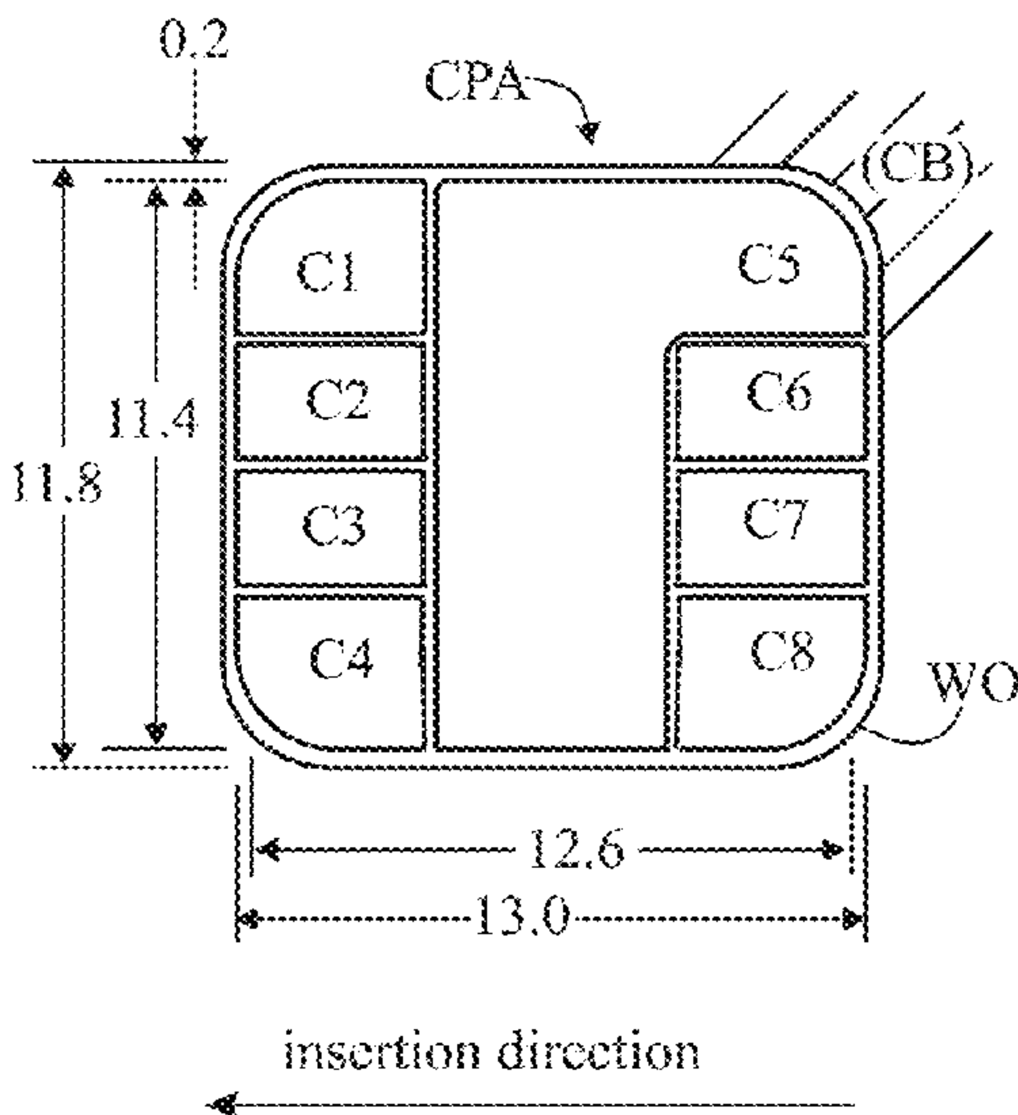
FIG. 1B 8-pad contact pattern
