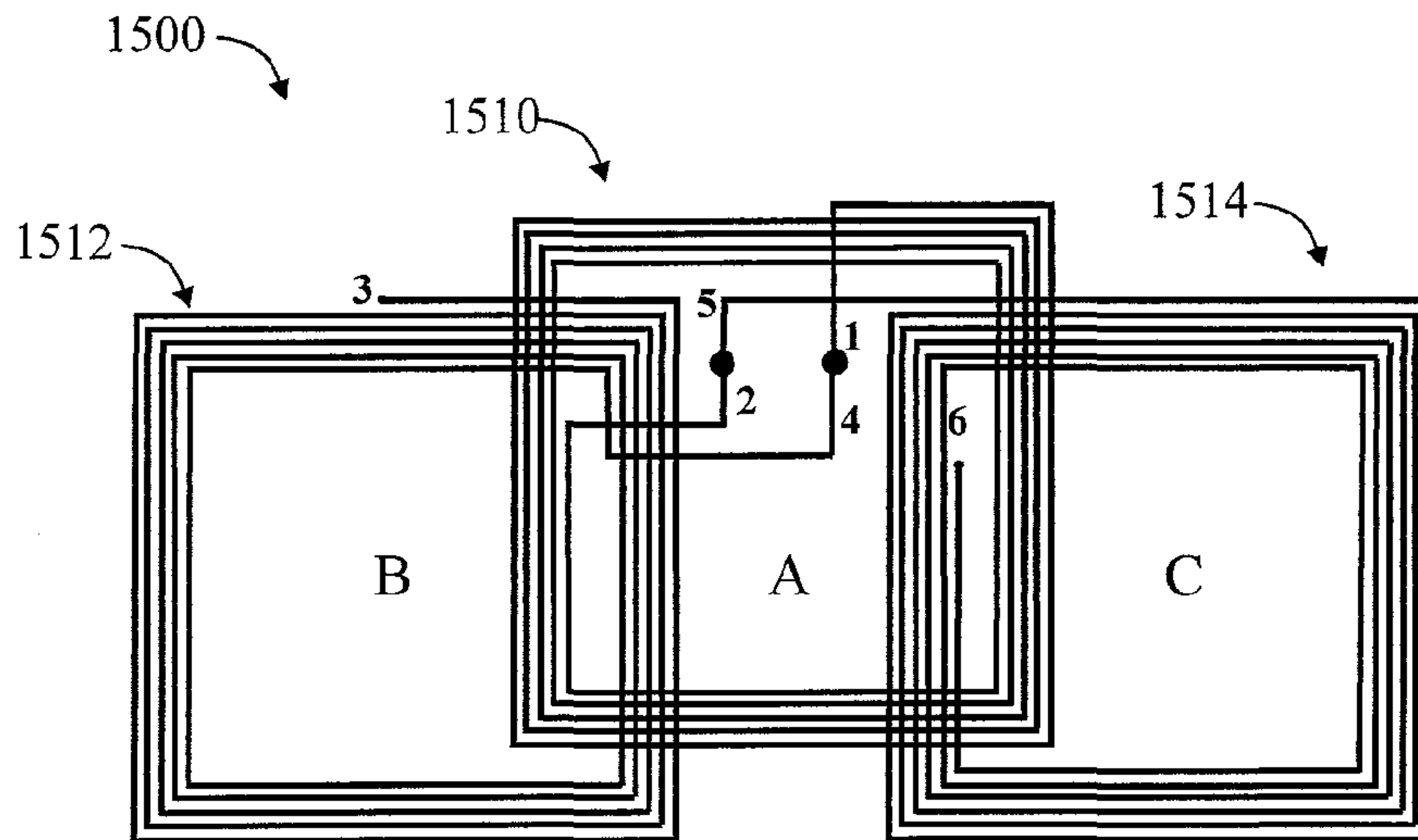
Booster Antenna with Capacitive Extensions
