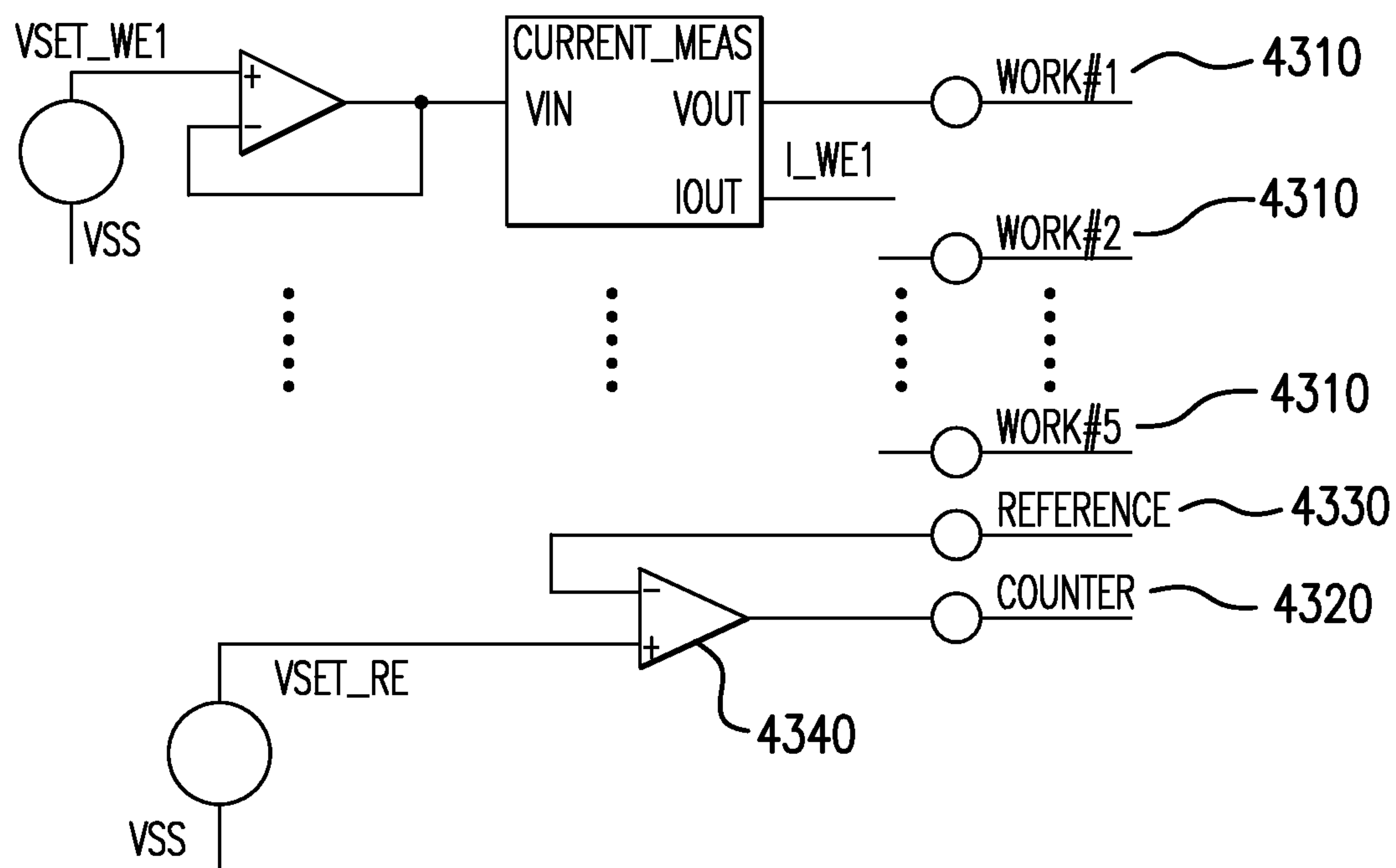
POTENTIOSTAT CONFIGURATION
