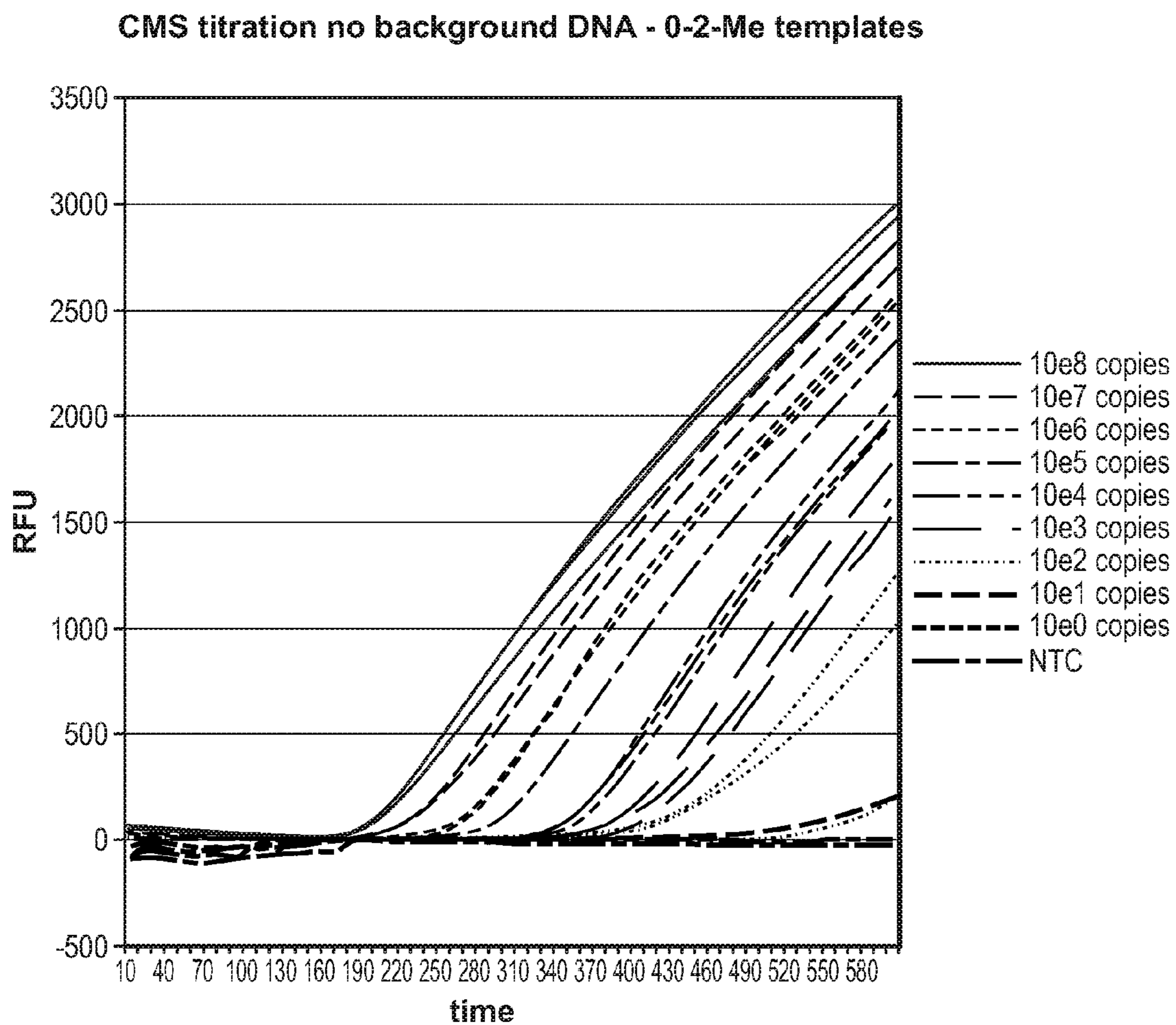
Cms Synthetic long-mer dynamic range evaluation - Exemplary titration of Cms synthetic "long-mer" target and detection via a fluorobeacon. The signal in the No Target Controls (NTC's) is suppressed in the 2'-o-Methyl modified template-containing reactions (left panel). The Standard Curve displays a wide dynamic range using the 2'-o-Methyl template reactions (right panel).
