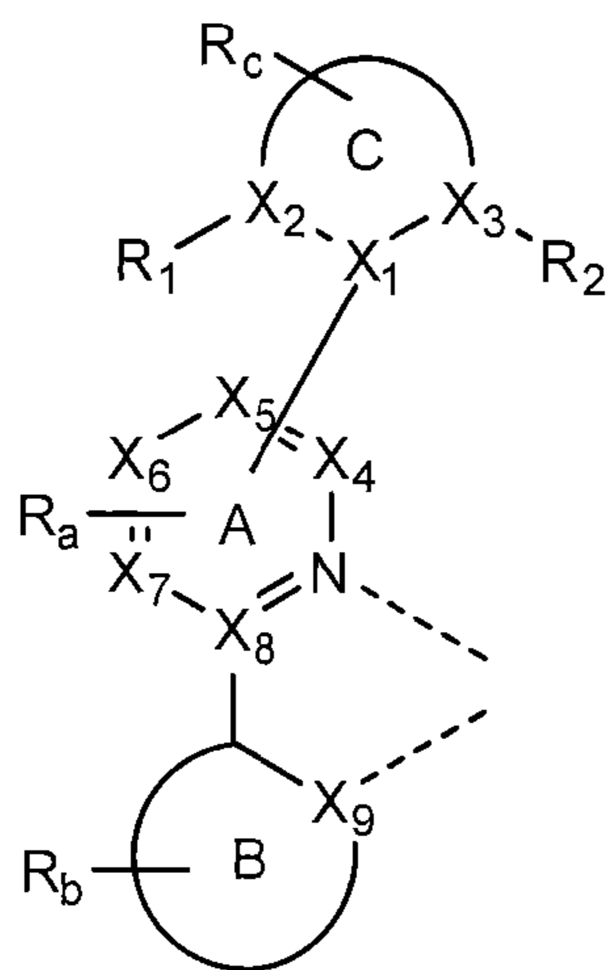
Formula I
