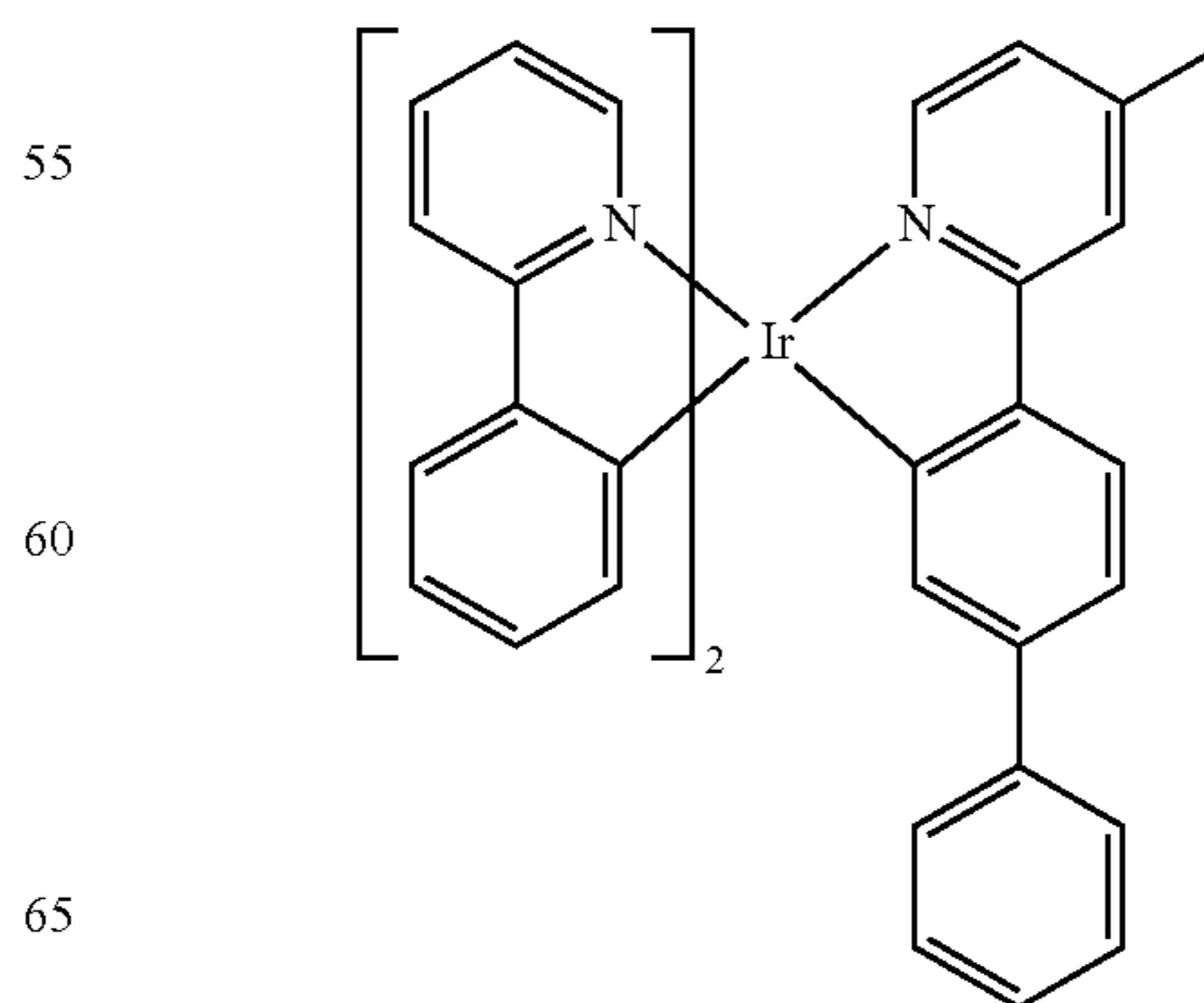
Compound 5
