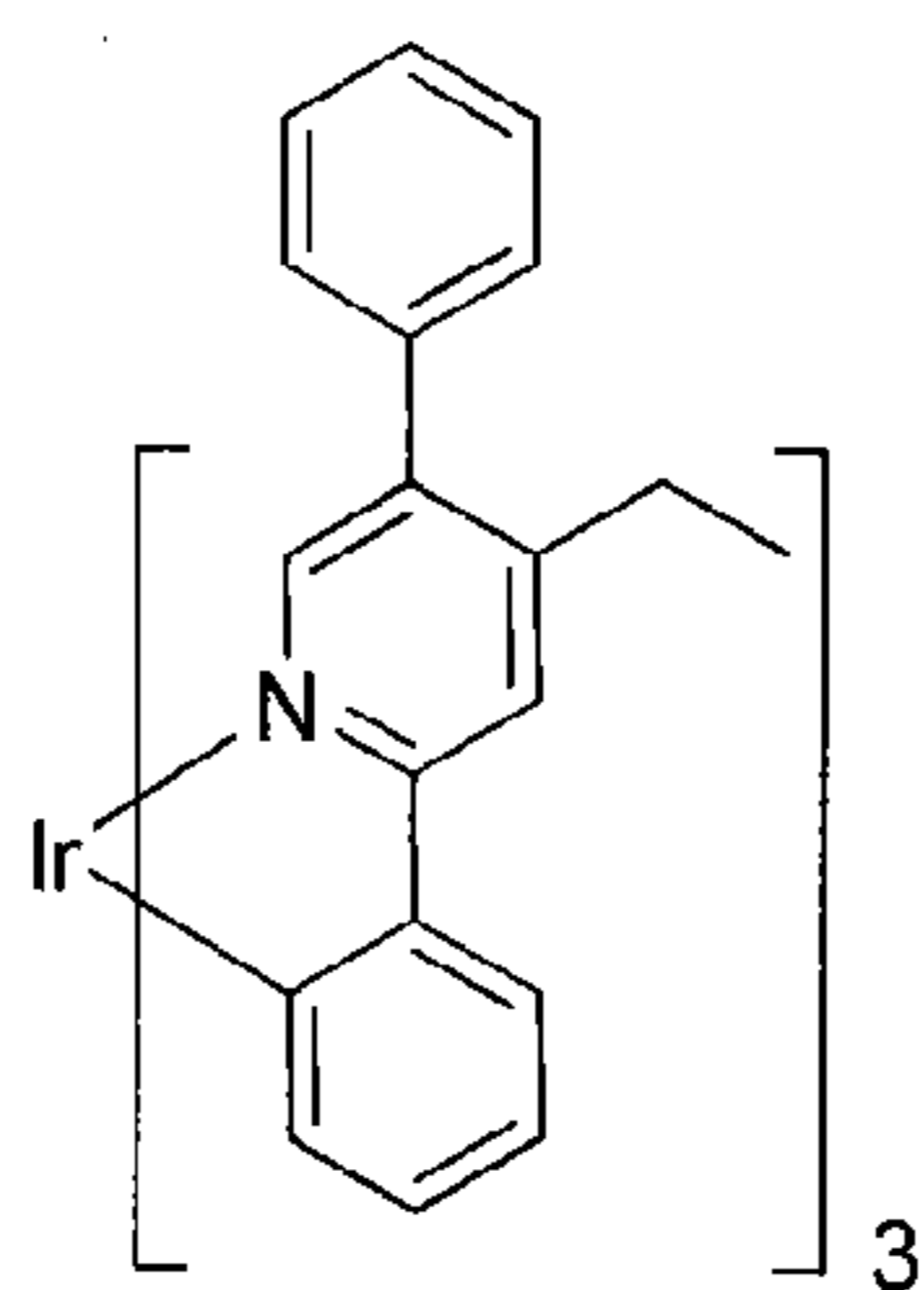
Compound 22
