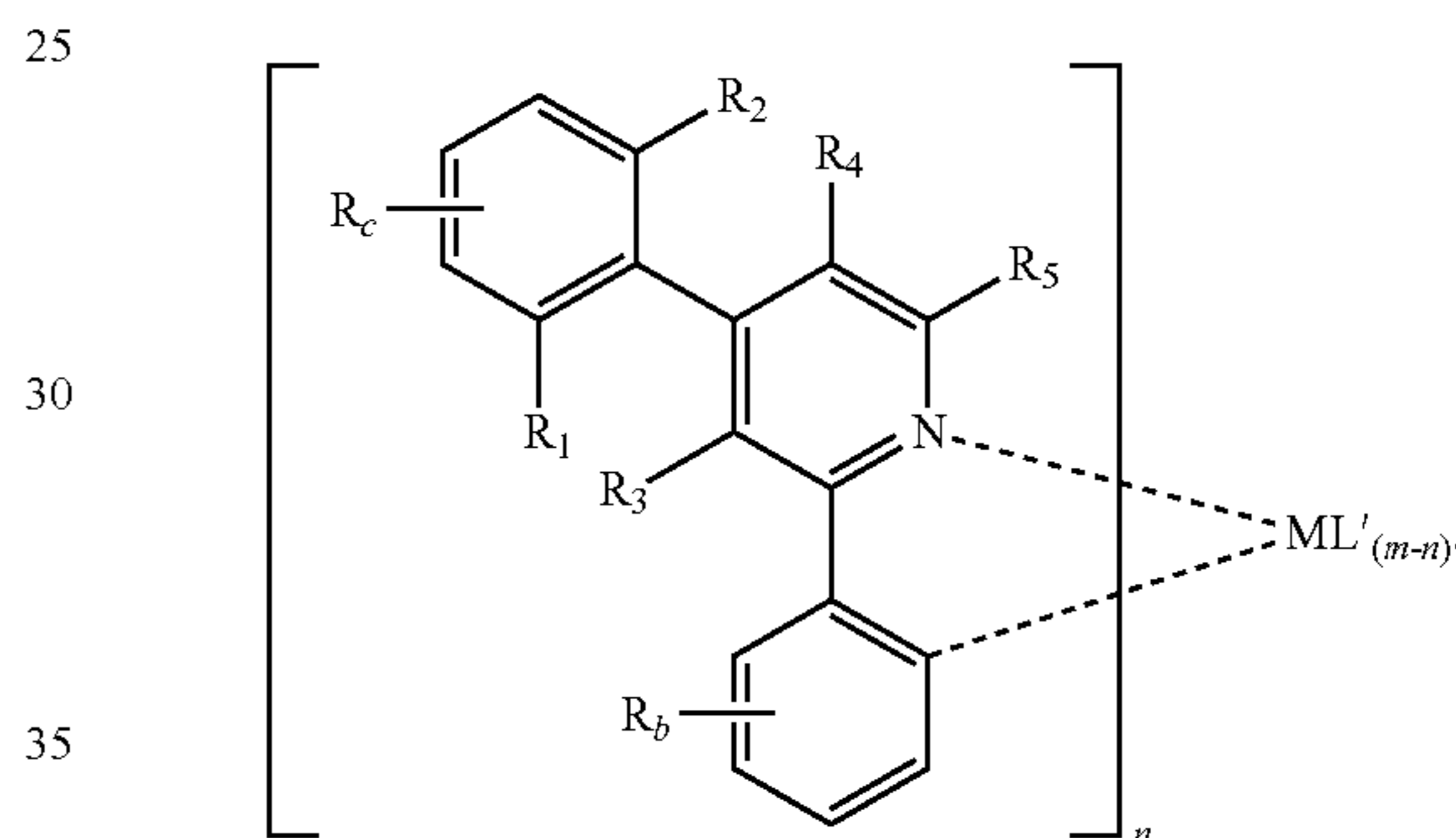
Formula VI
