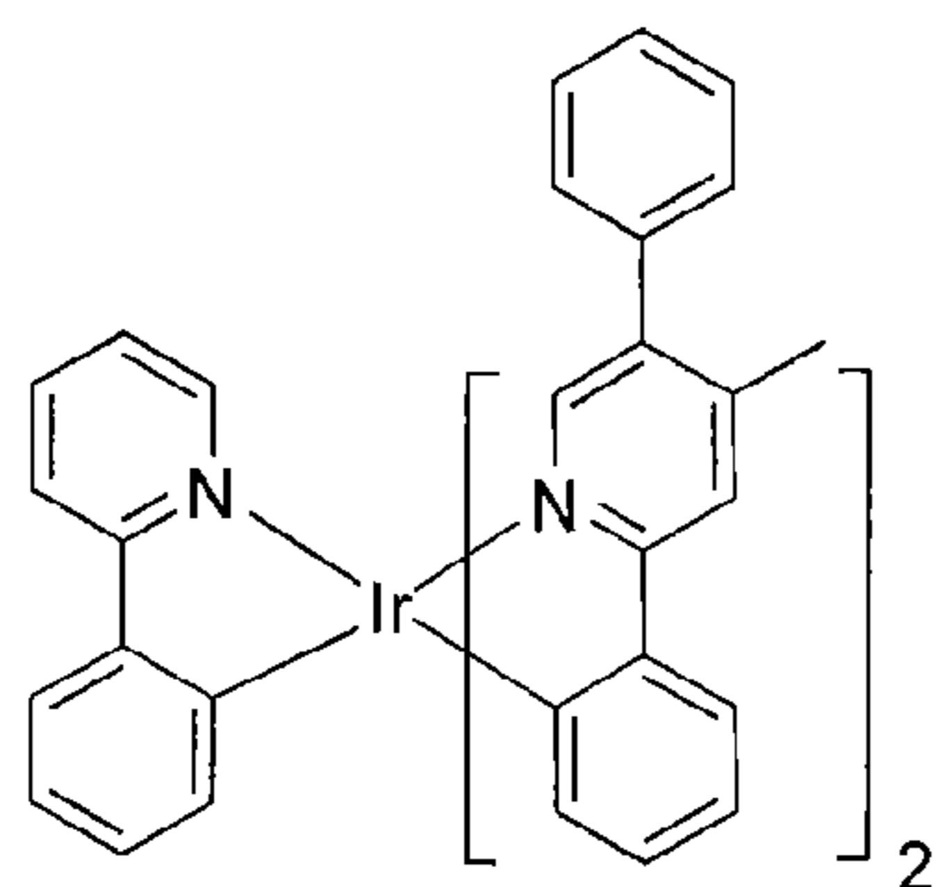
Compound 29
