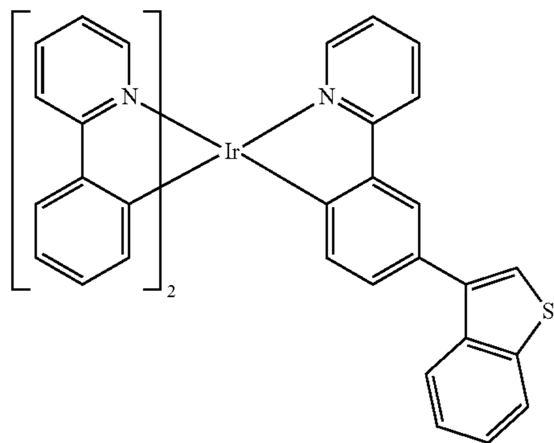
Compound 6
