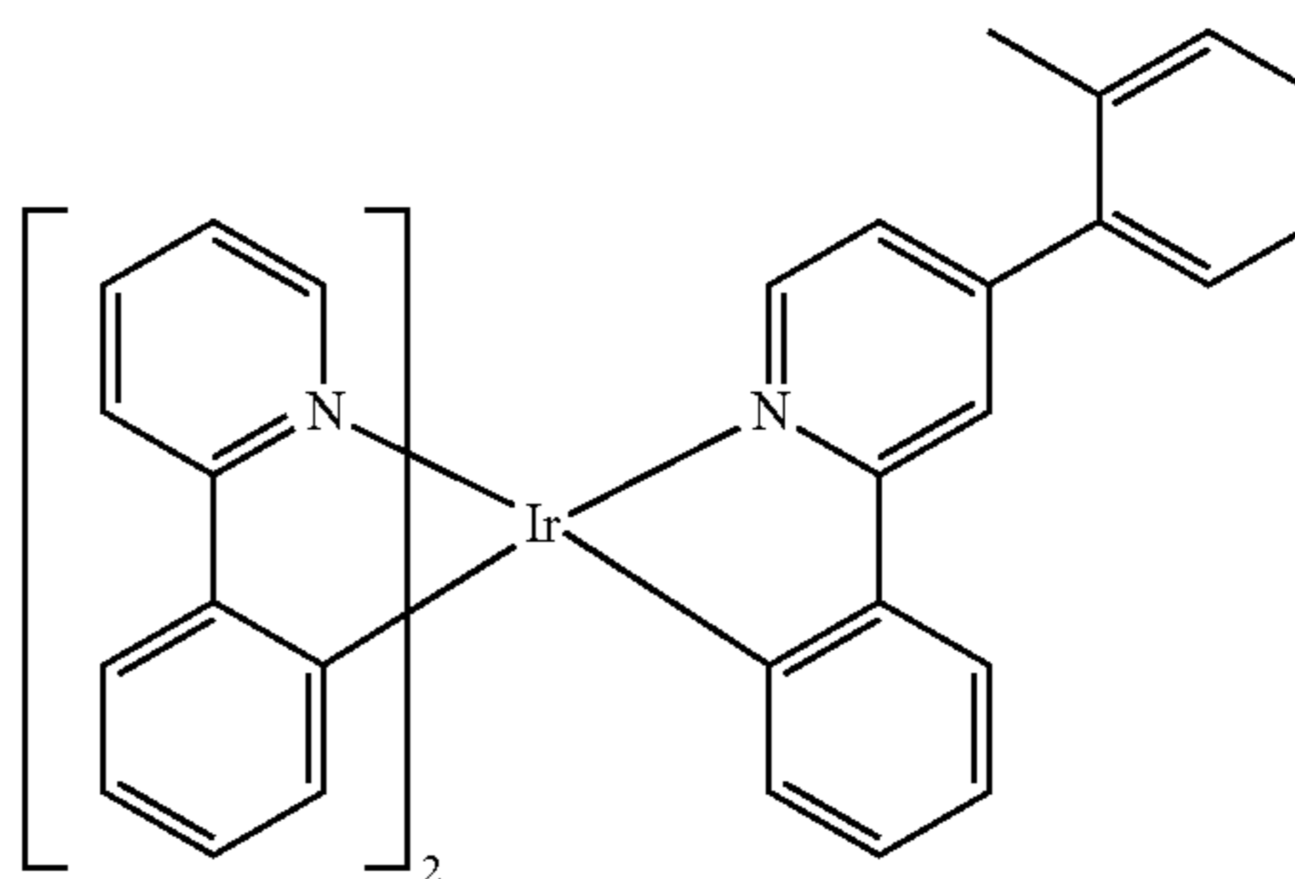
Compound 27
