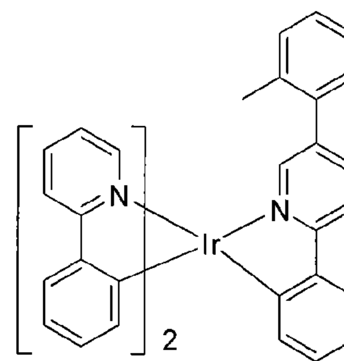
Compound 25
