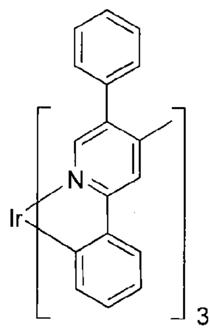
Compound 21
