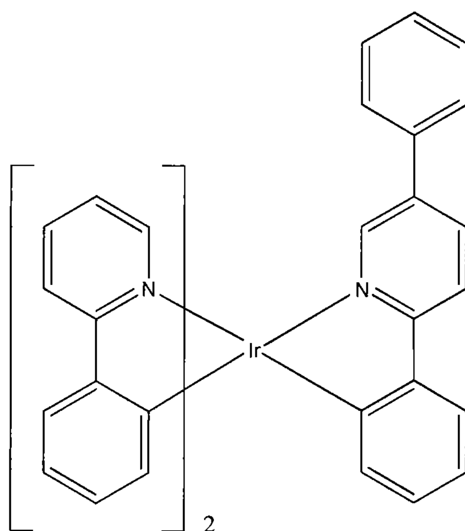
Compound 2
