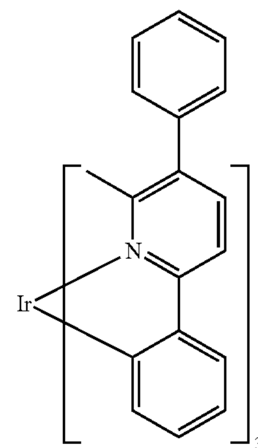
Compound 23
