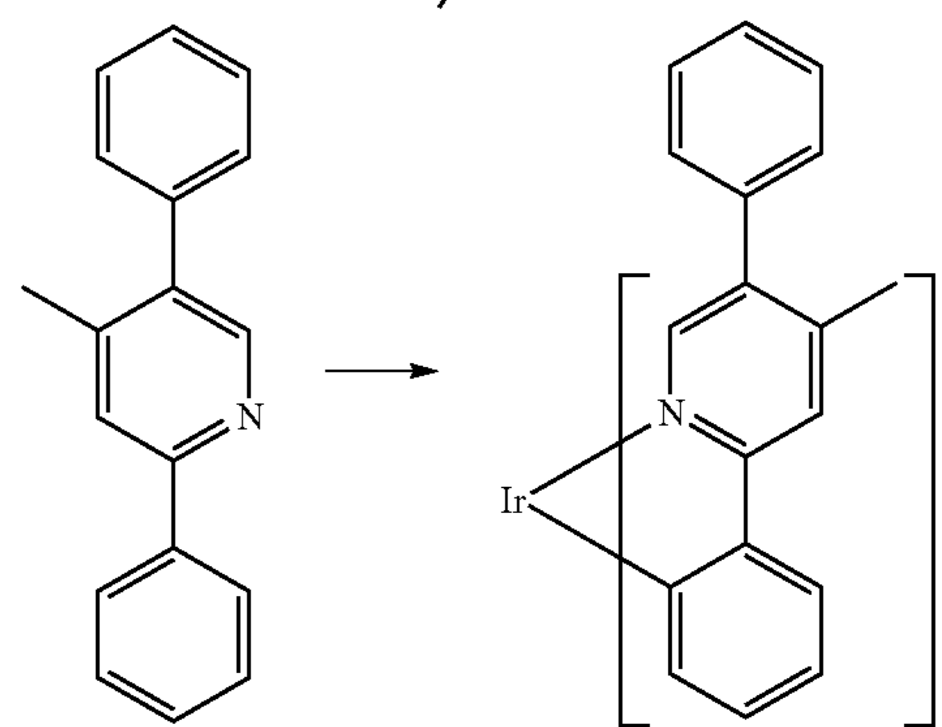
Compound 21
