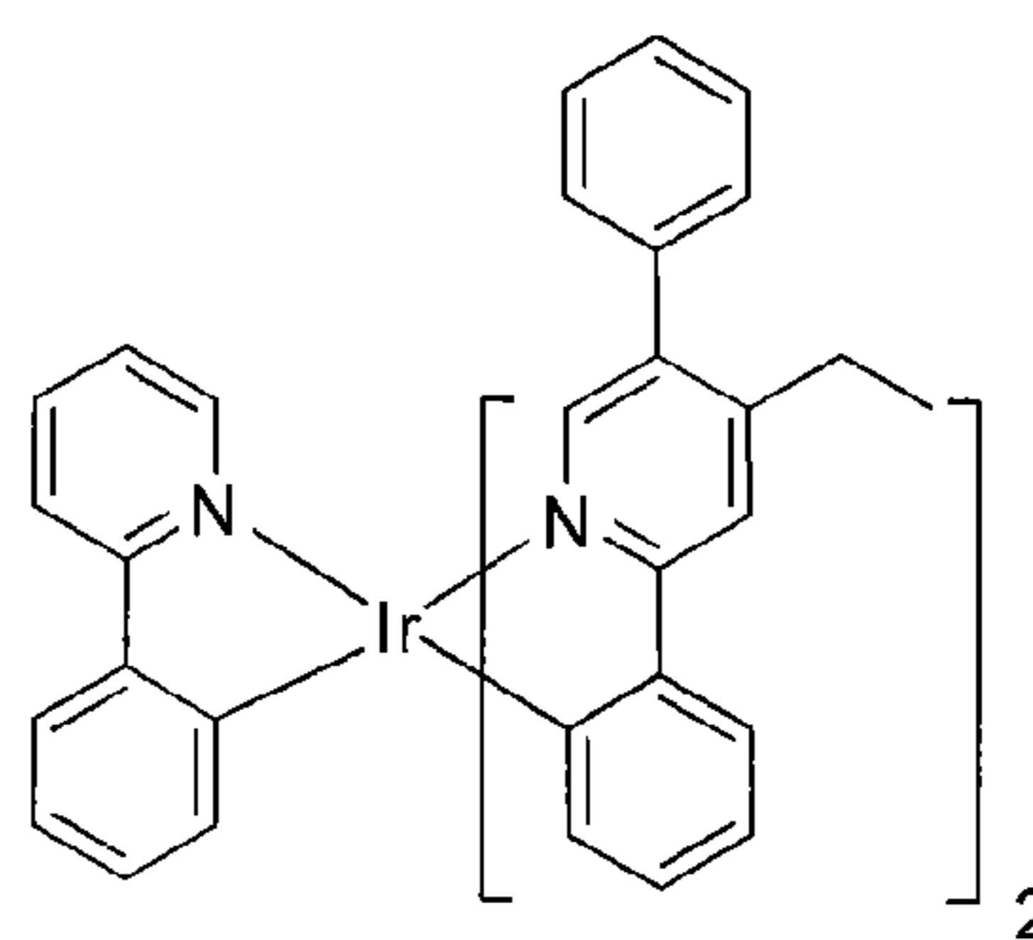
Compound 30
