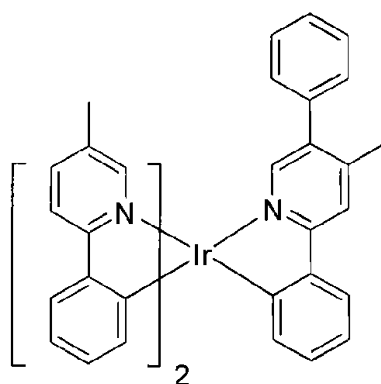
Compound 31
