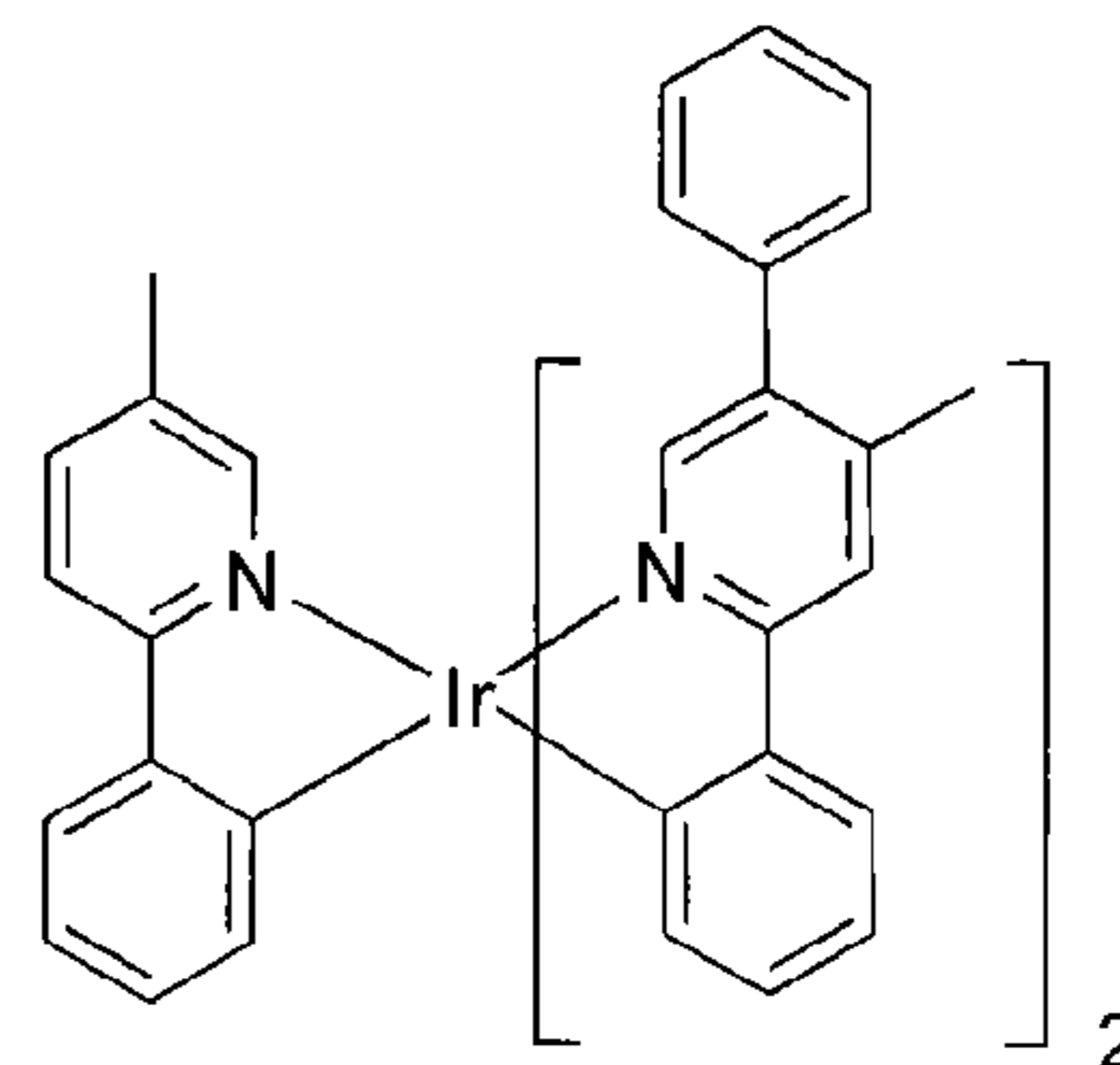
Compound 34
