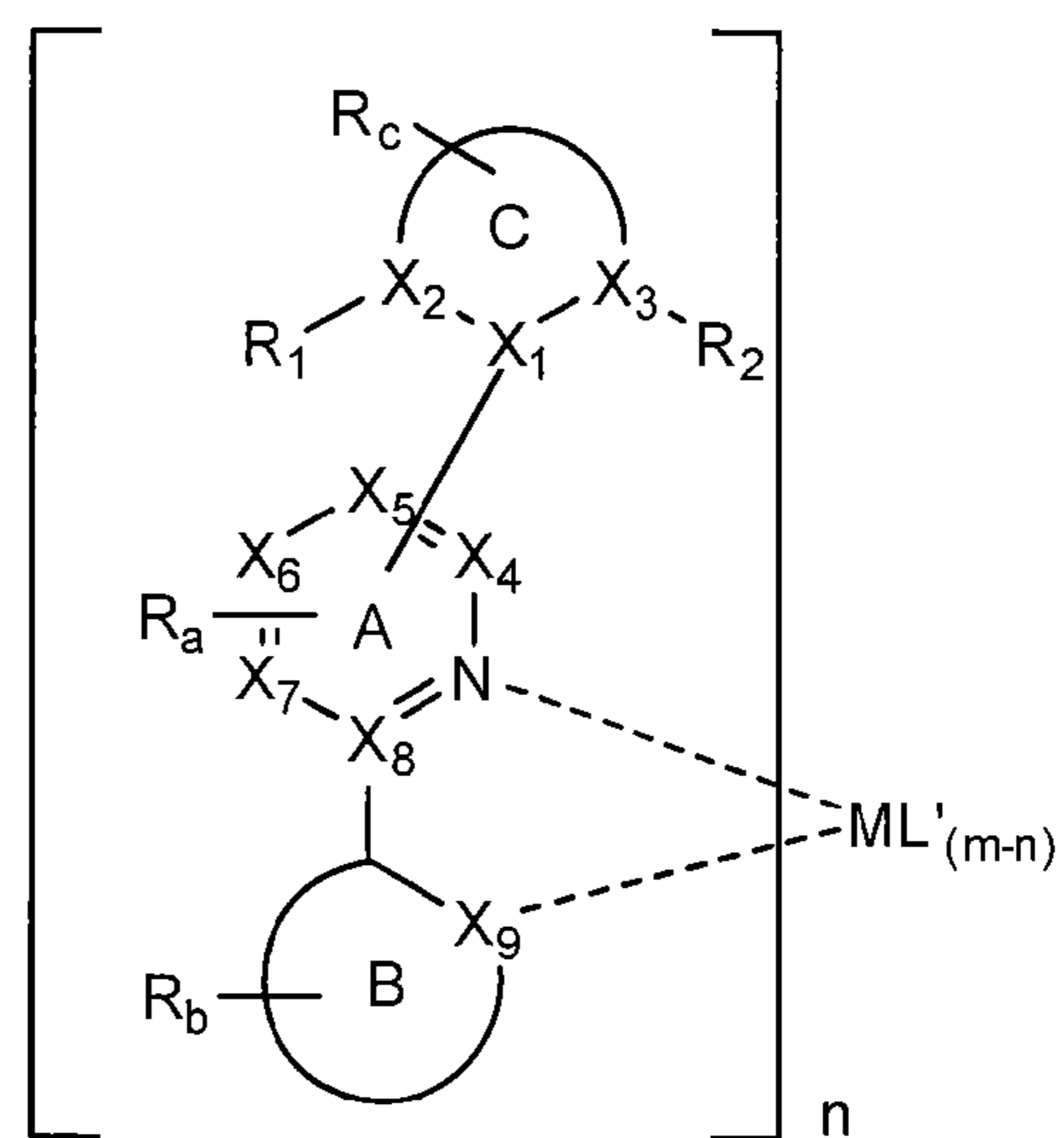
Formula II
