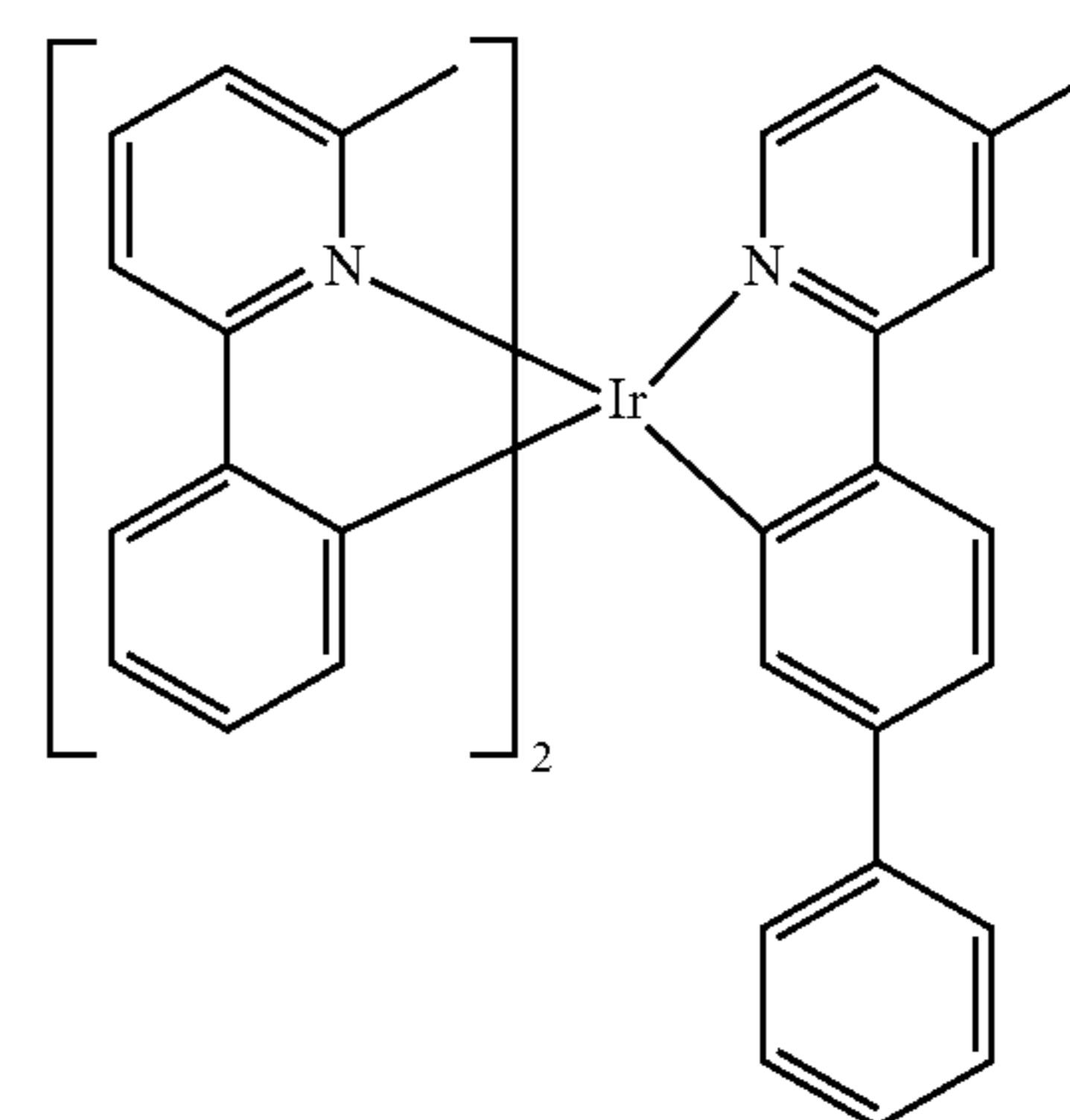
Compound 10
