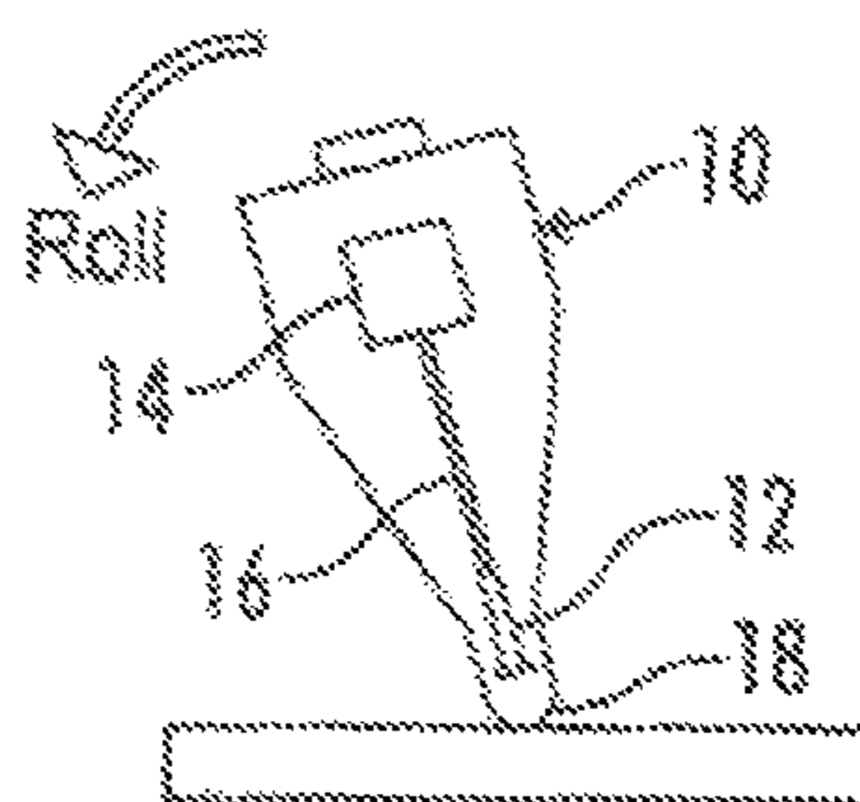
FIG. 4 (PRIOR ART)
