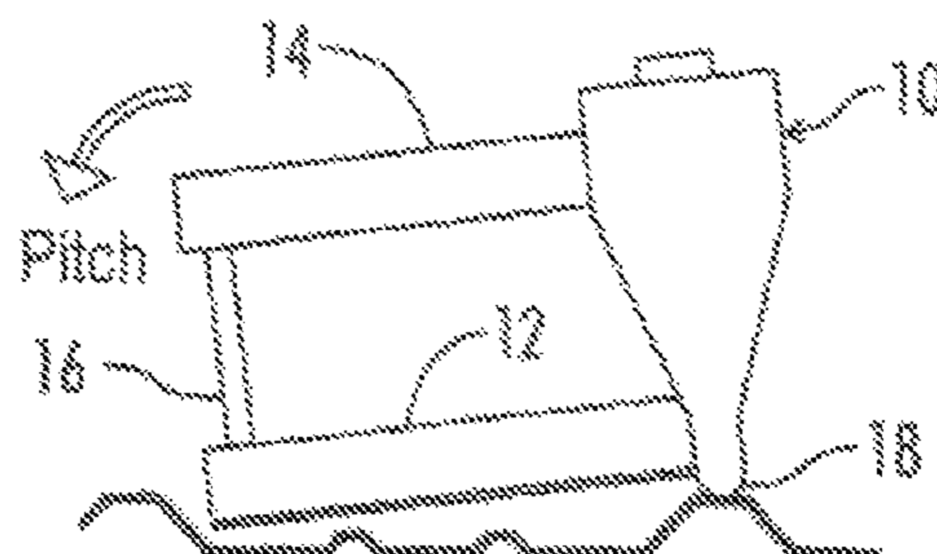
FIG. 2 (PRIOR ART)
