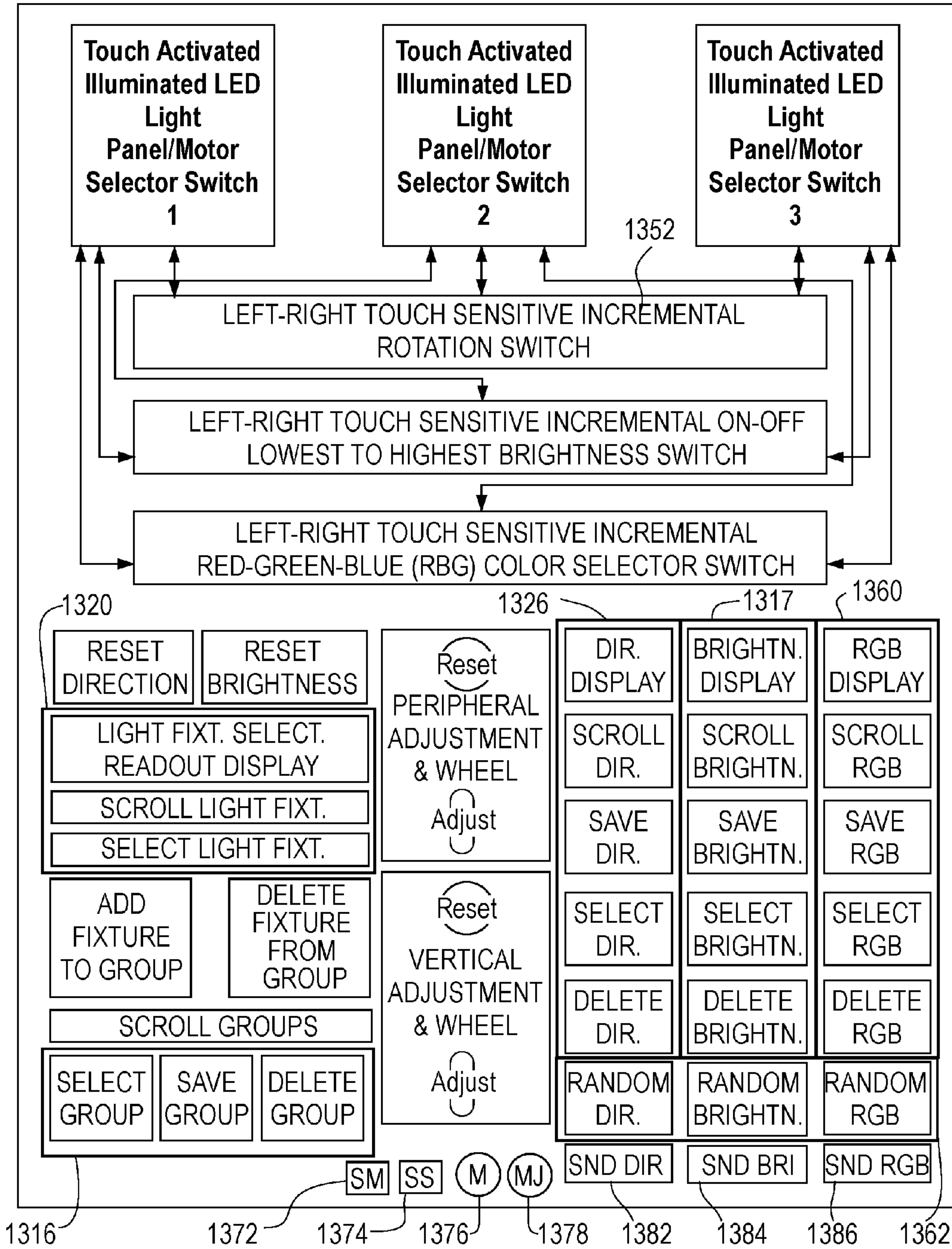
RGB-SOUND CONTROLLER INTERFACE BLOCK DIAGRAM
