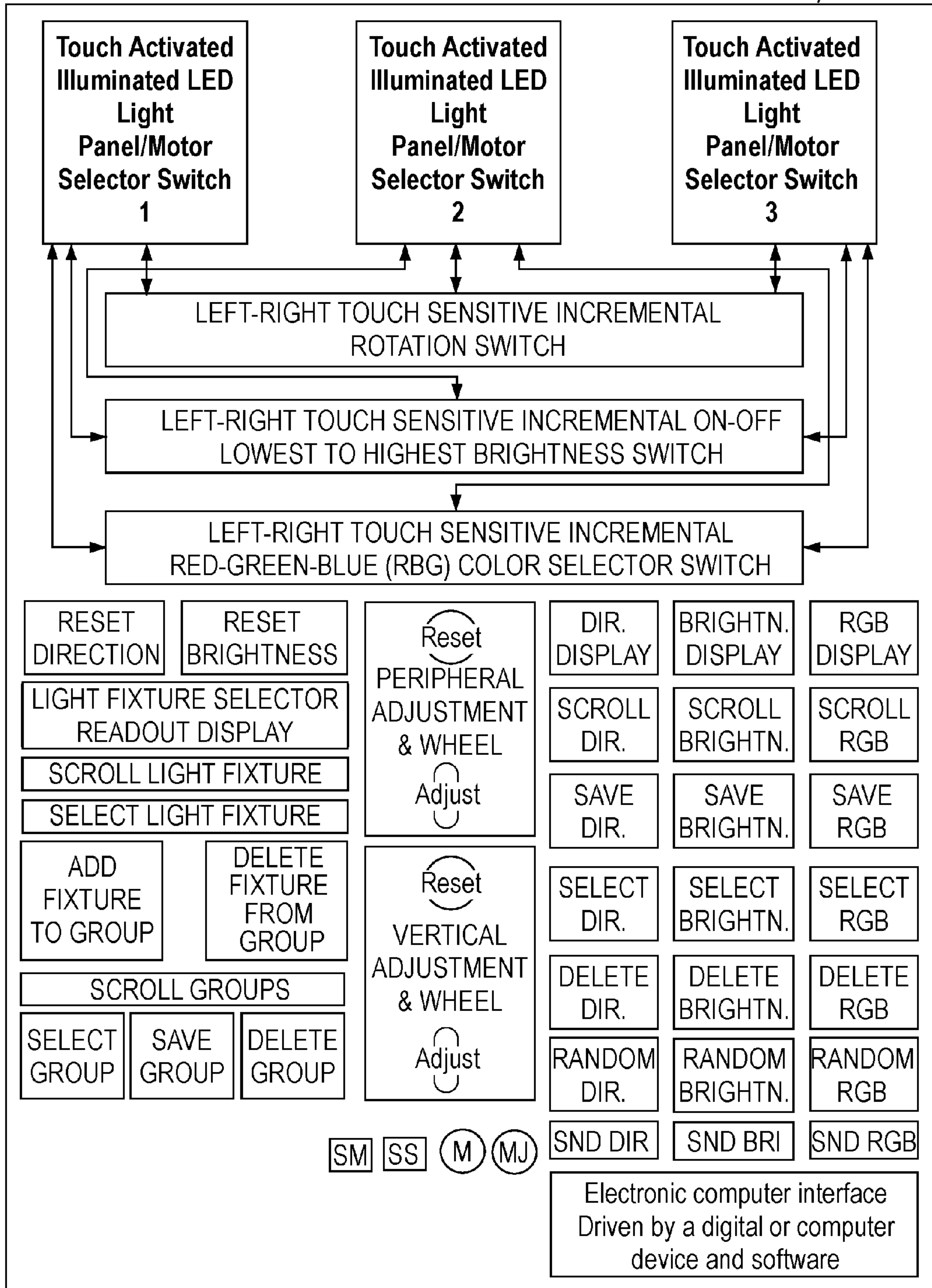
Fig. 18 RGB-SOUND CONTROLLER BLOCK DIAGRAM 1800 w/ COMPUTER INTERFACE
