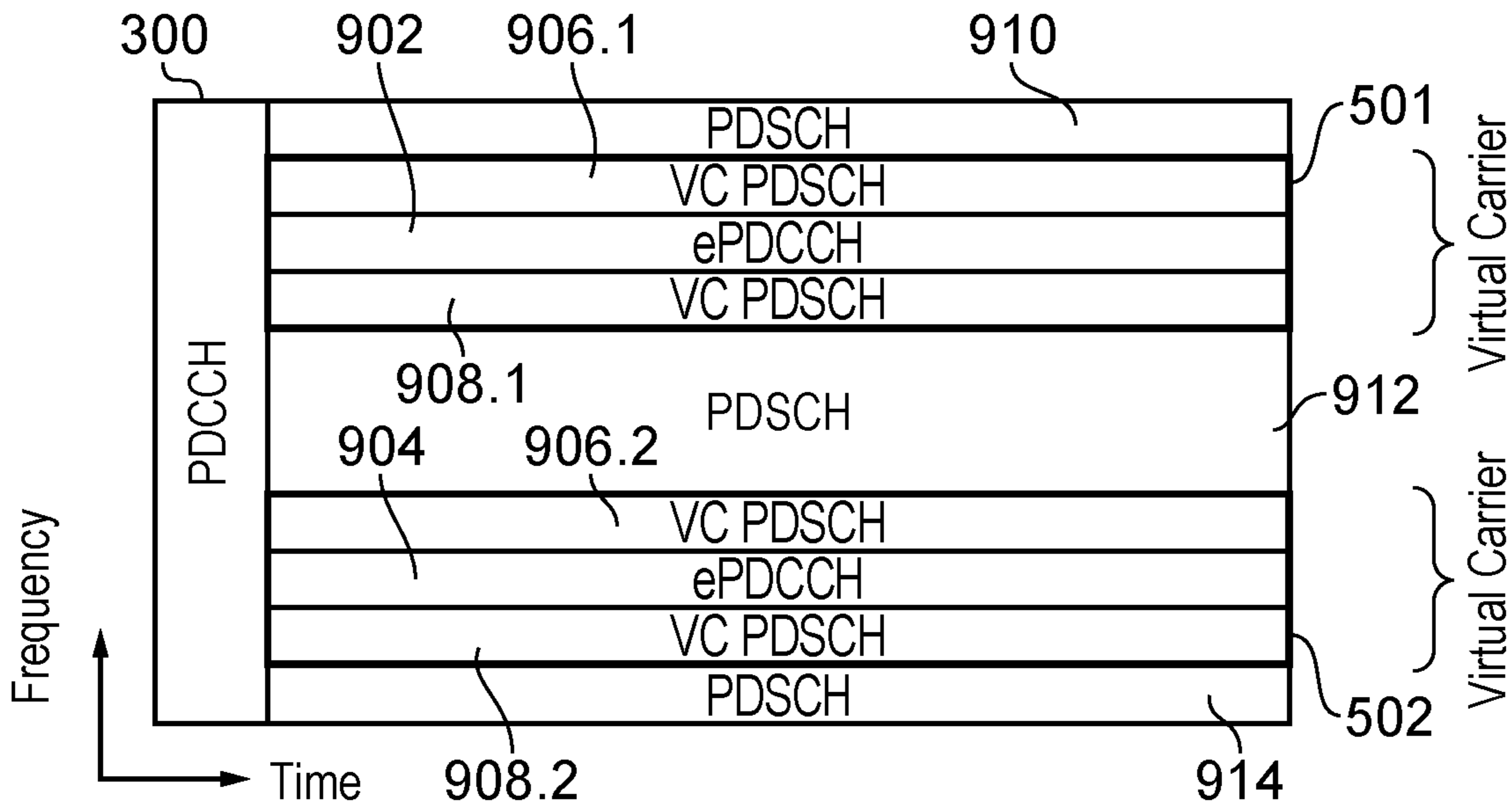
FIG. 11 ePDCCH Sharing 3 (Distributed)
