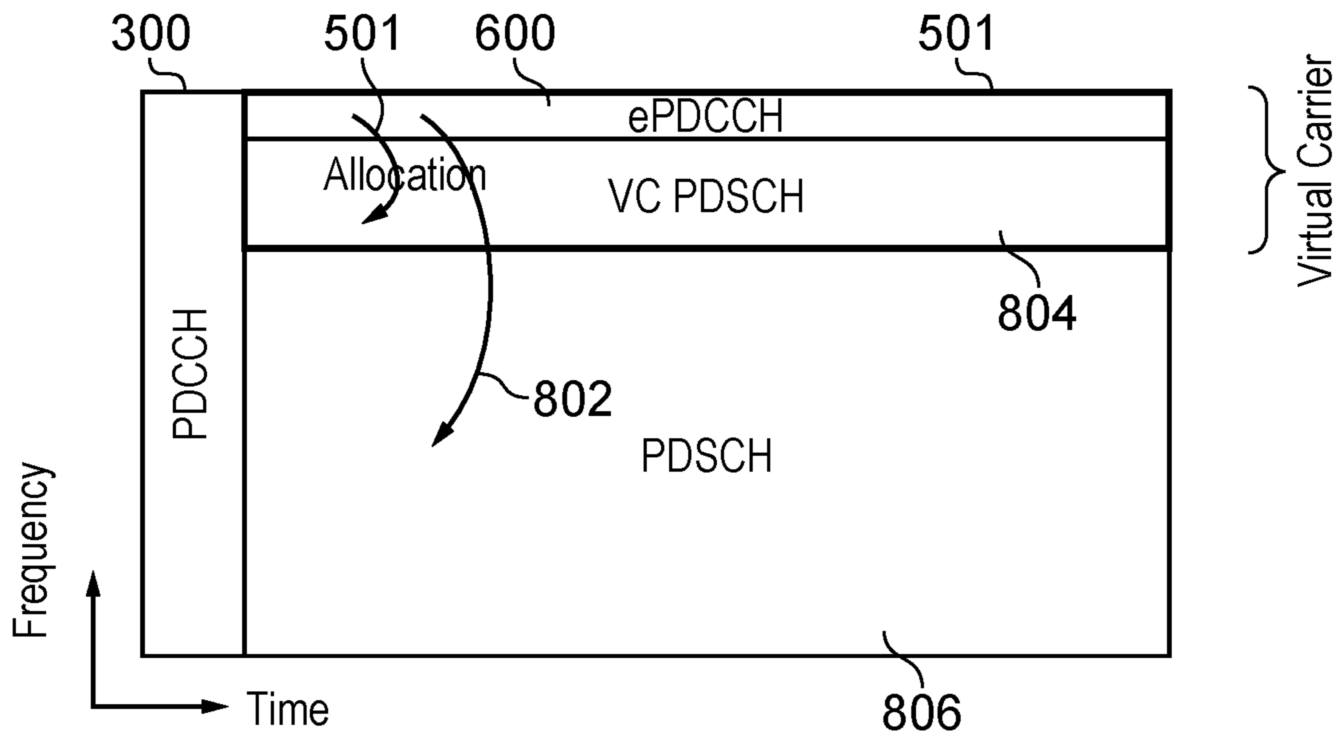
FIG. 8 Resource Allocation for VC PDSCH using ePDCCH
