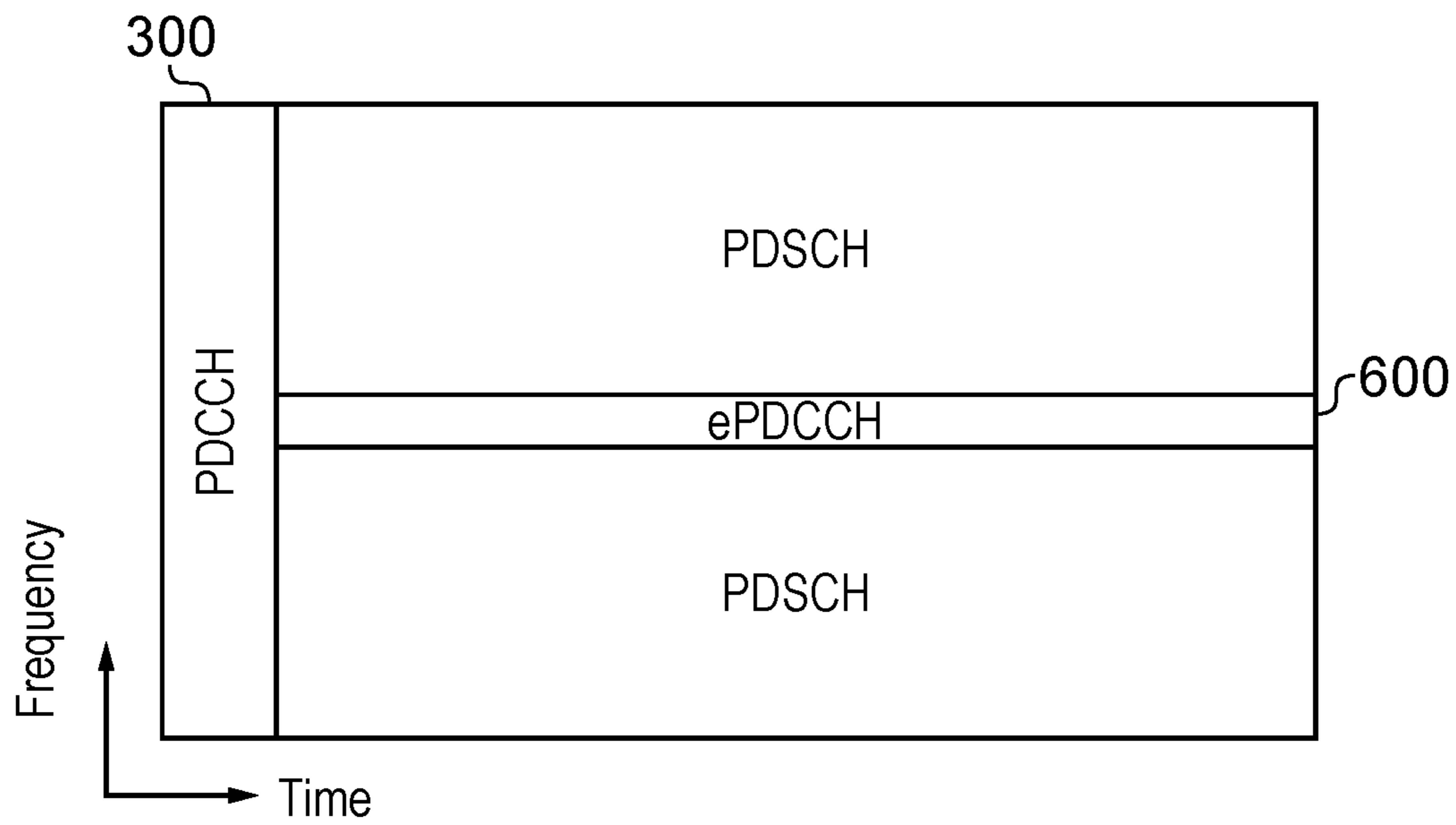
FIG. 5 Rel-11 ePDCCH (Localized)
