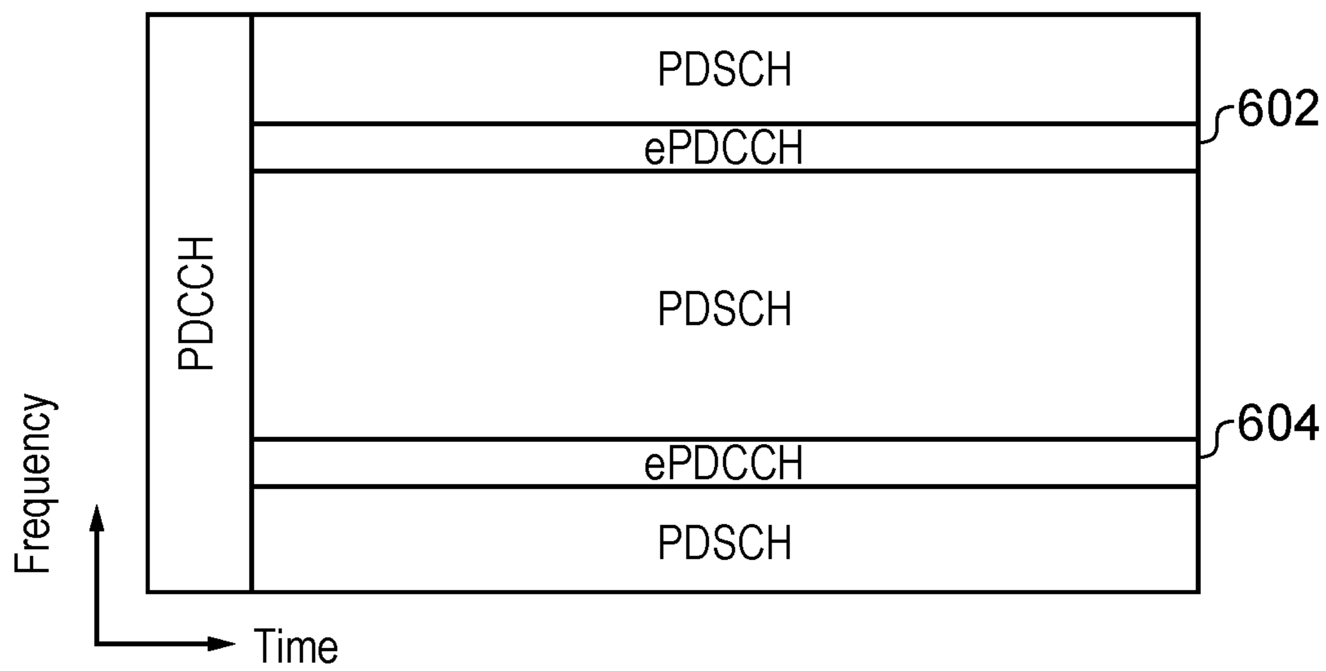
FIG. 6 Rel-11 ePDCCH (Distributed)
