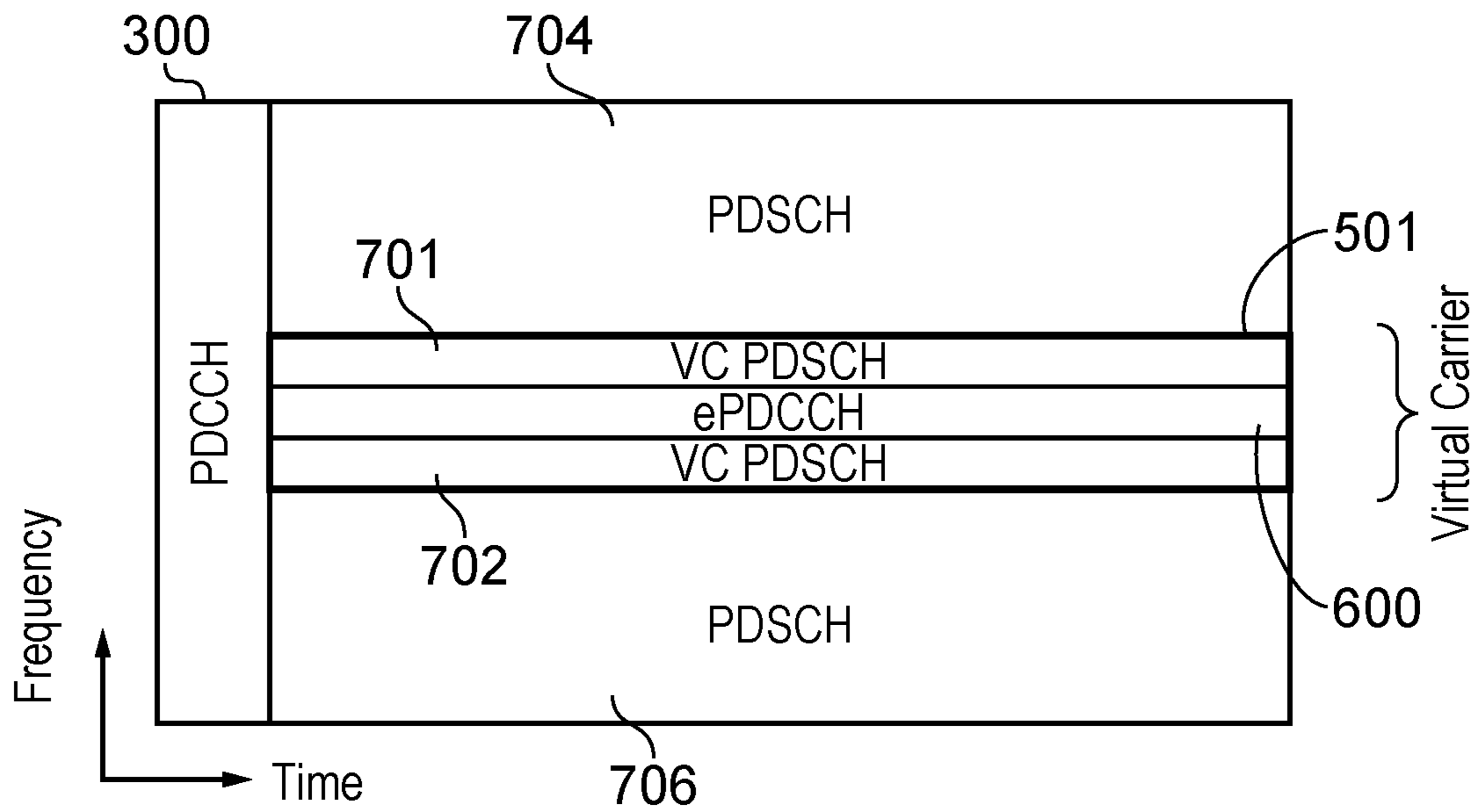
FIG. 7 ePDCCH Sharing (Localized)
