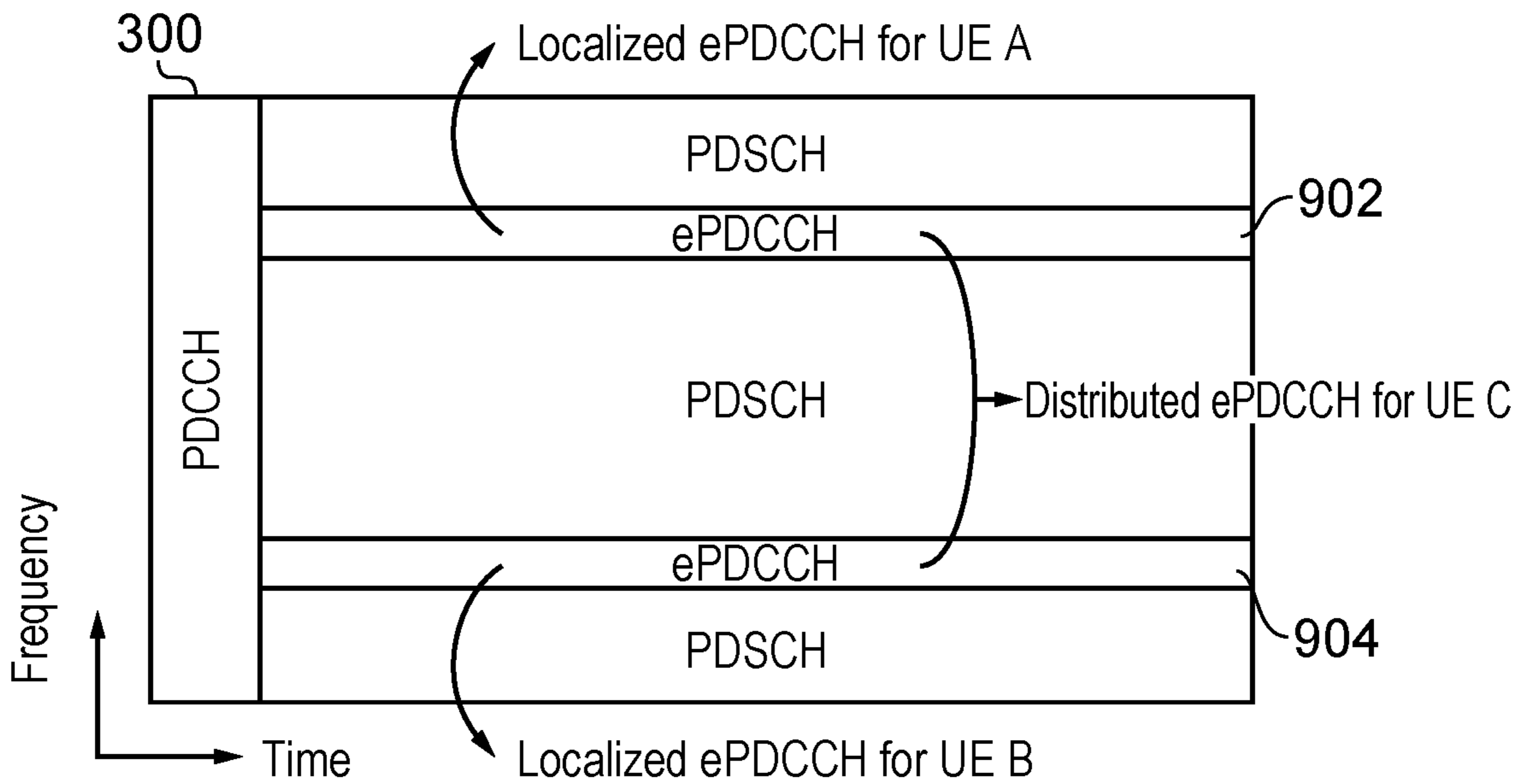
FIG. 12 ePDCCH Sharing (Localized & Distributed)
