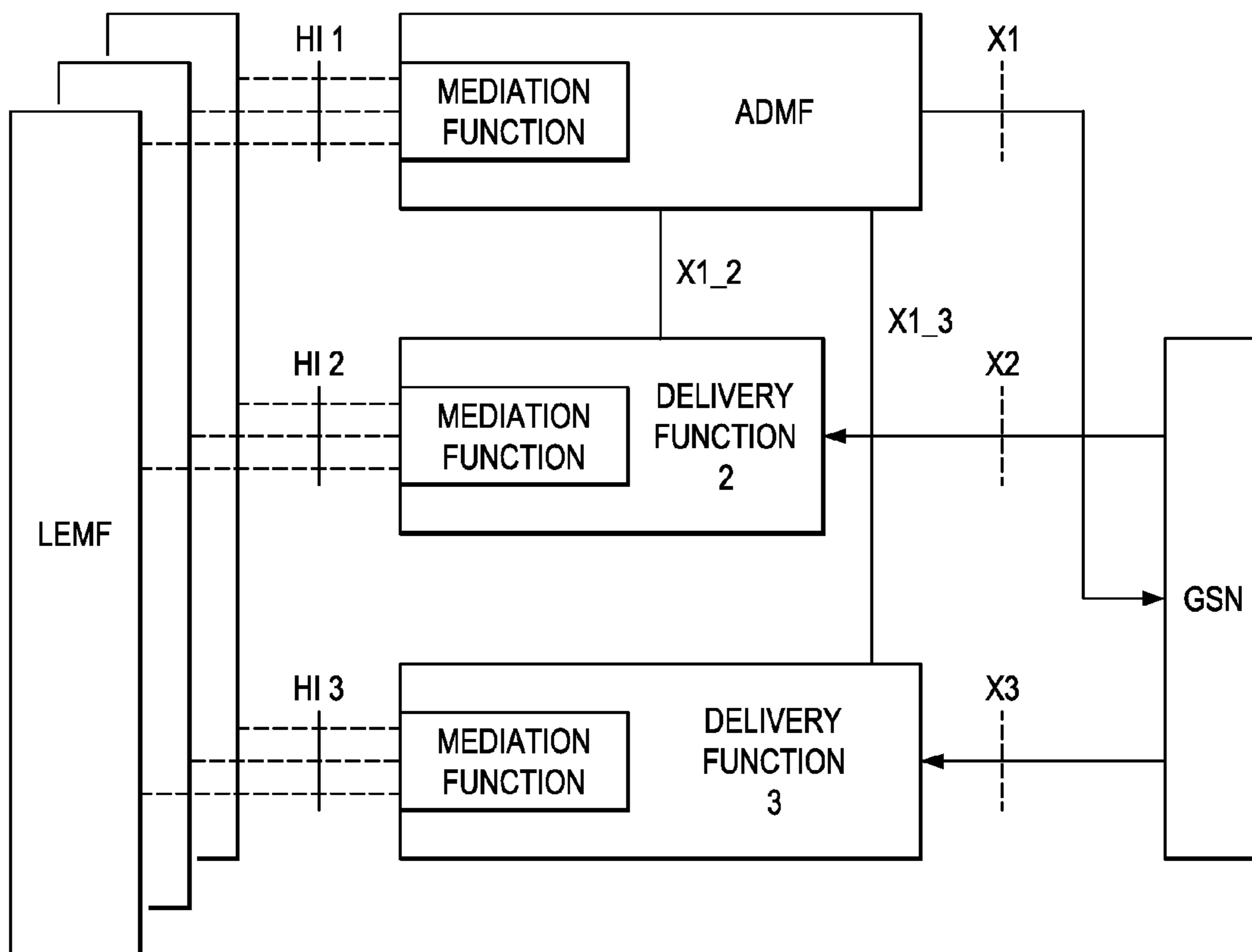
FIG. 16 (PRIOR ART)
