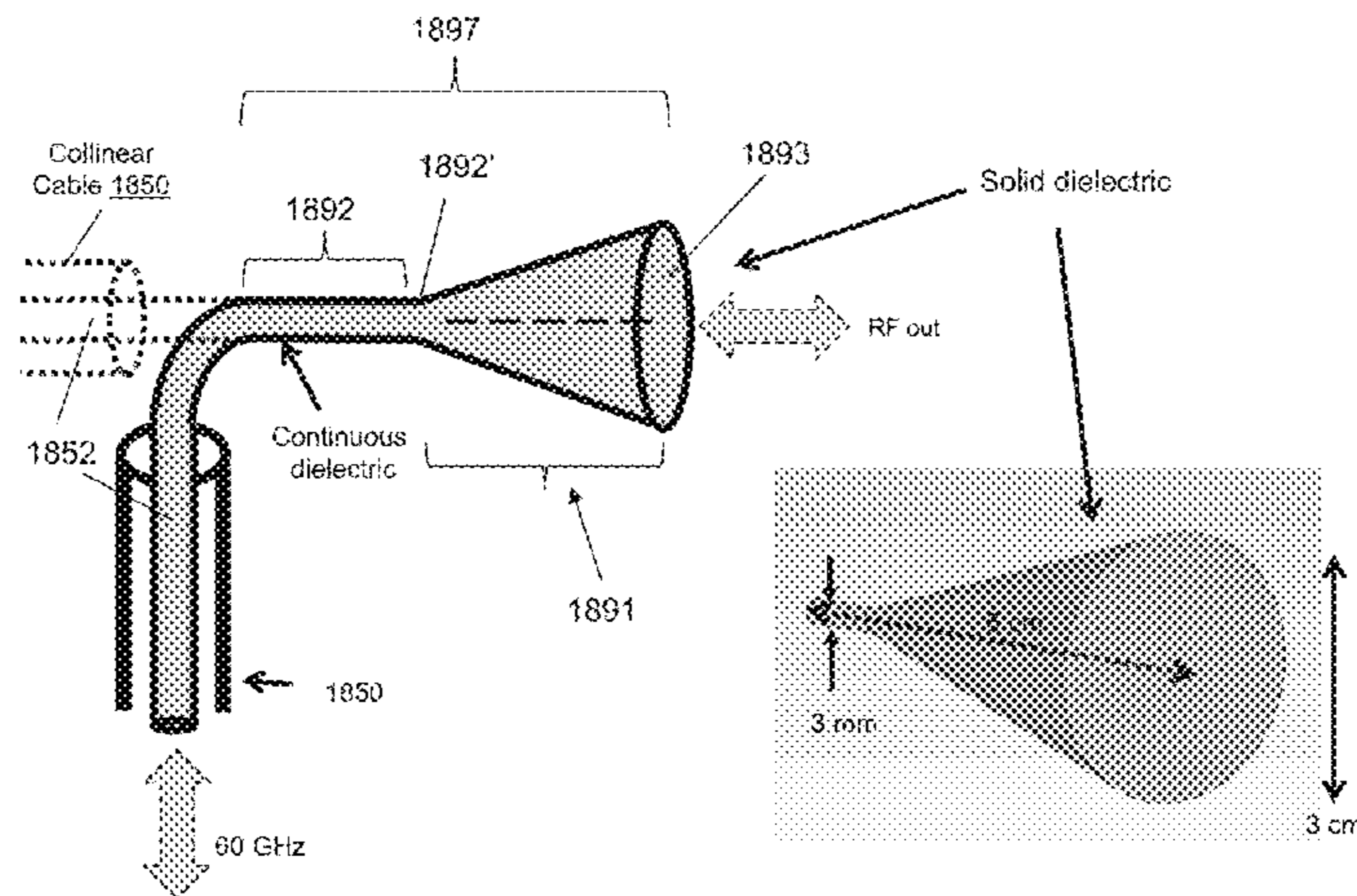
Dielectric Horn Antenna
