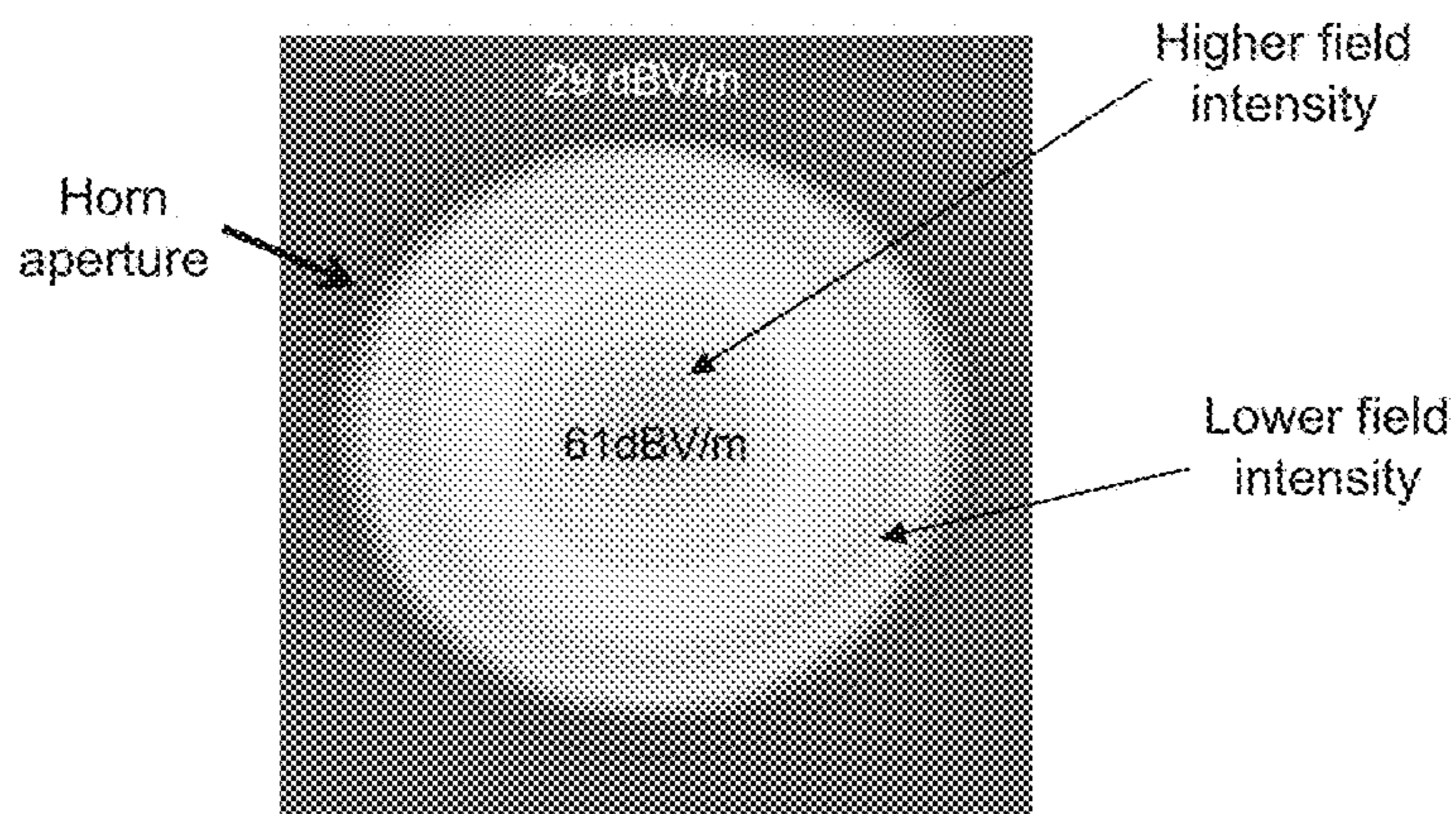
E-field Intensity Pattern
