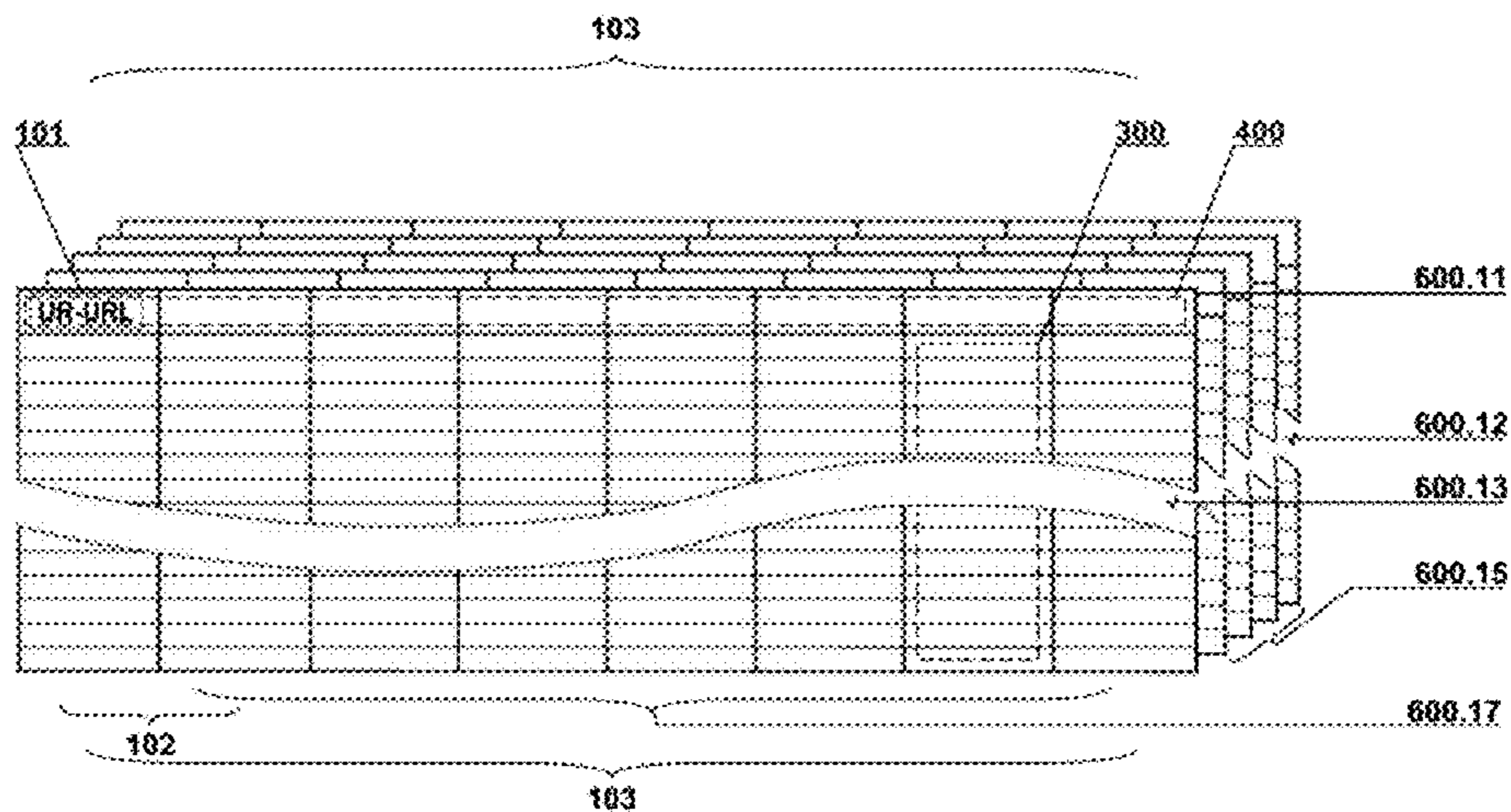
FIG. 40 Database With Unitary Reference Architecture
