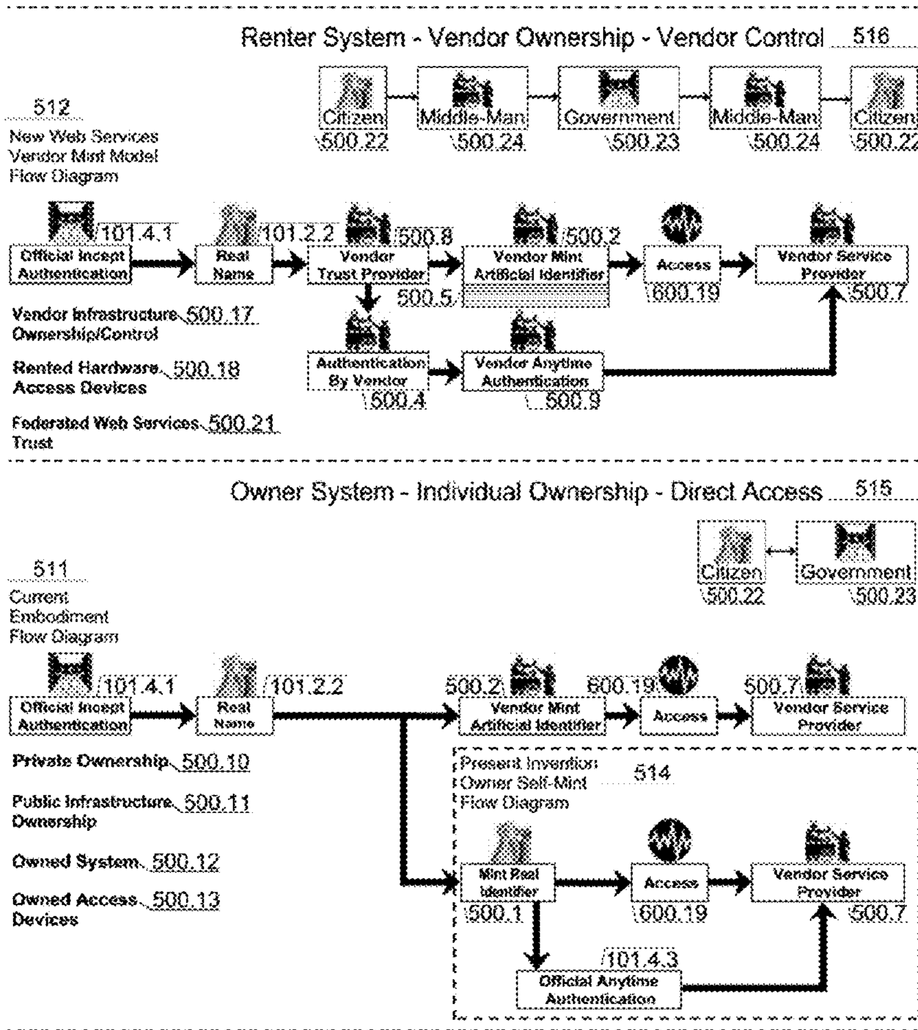
FIG. 61 Ownership Process Components Comparison
