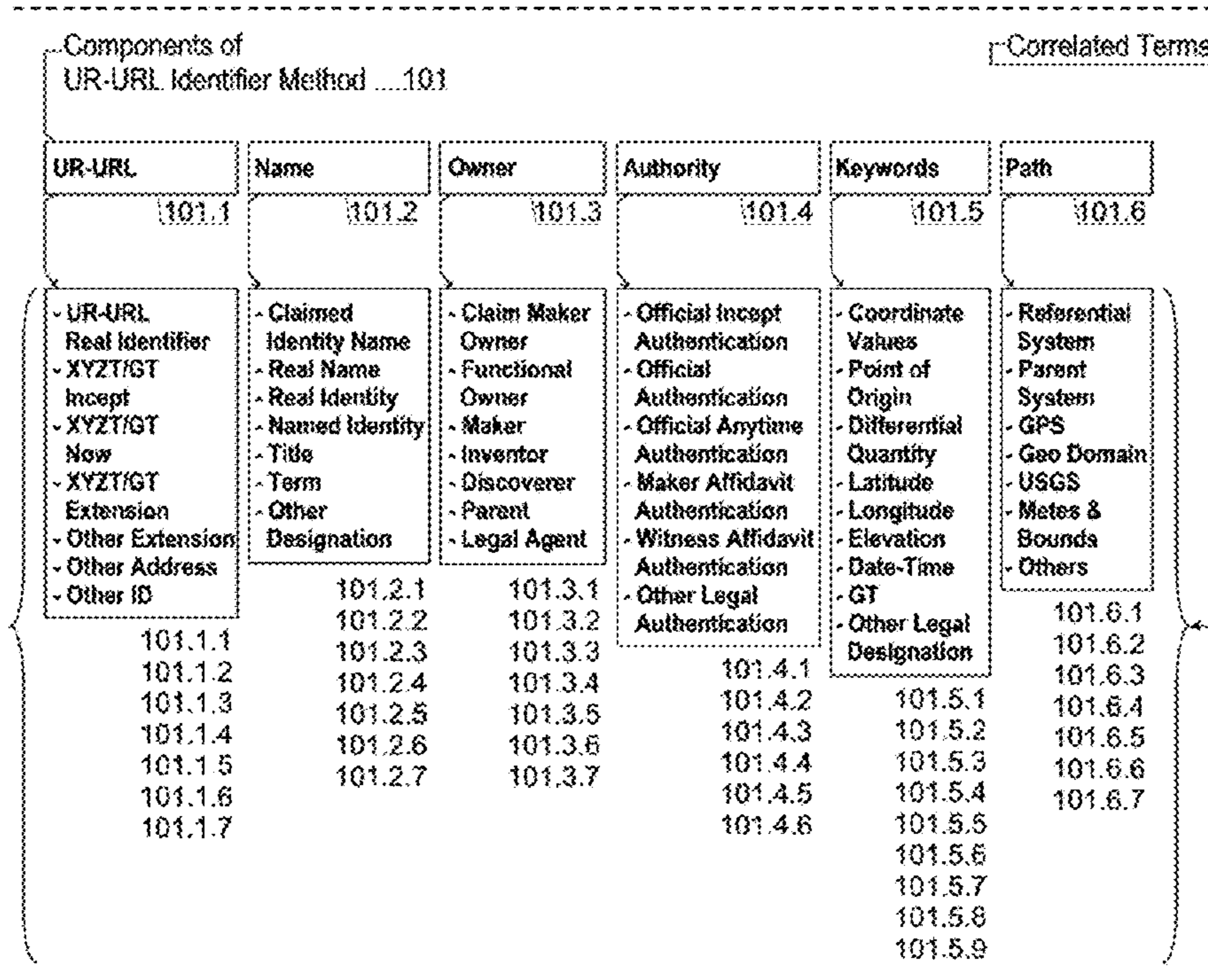
FIG. 12 UR-URL Identity Architecture Components
