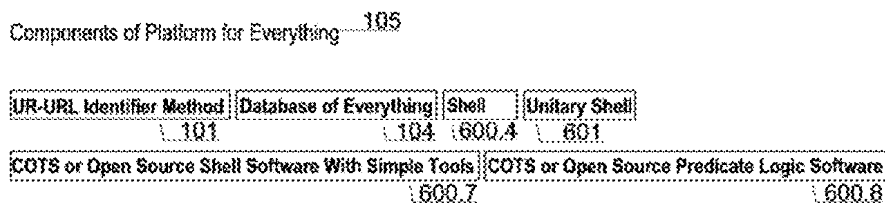
FIG. 43 Platform View
