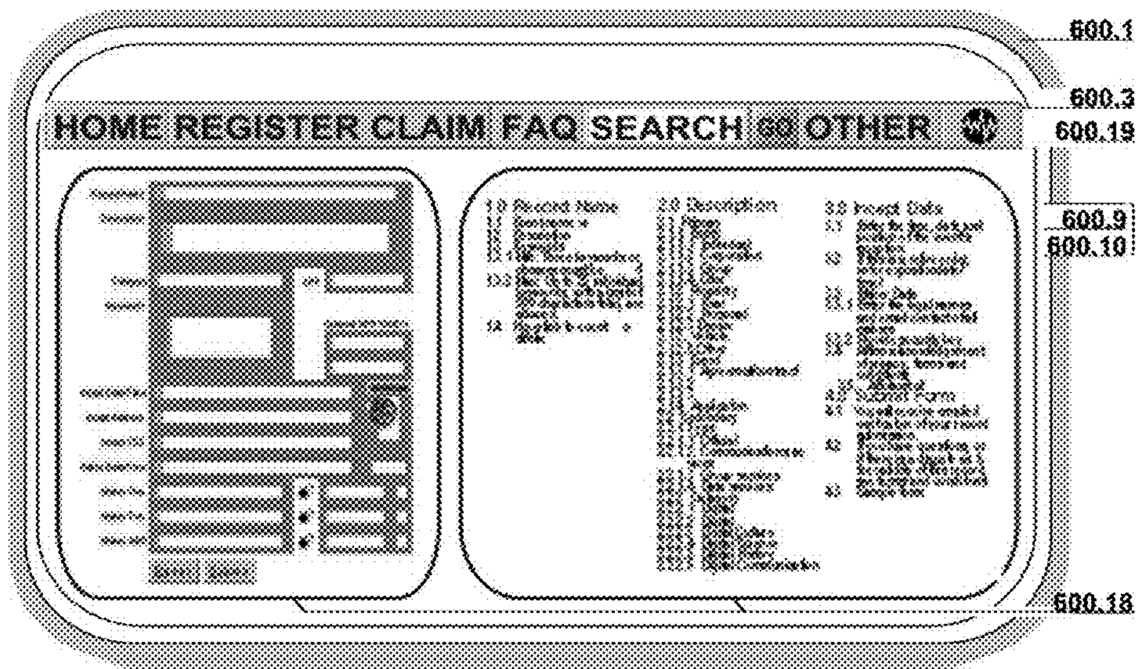
FIG. 88 Homepage 8
