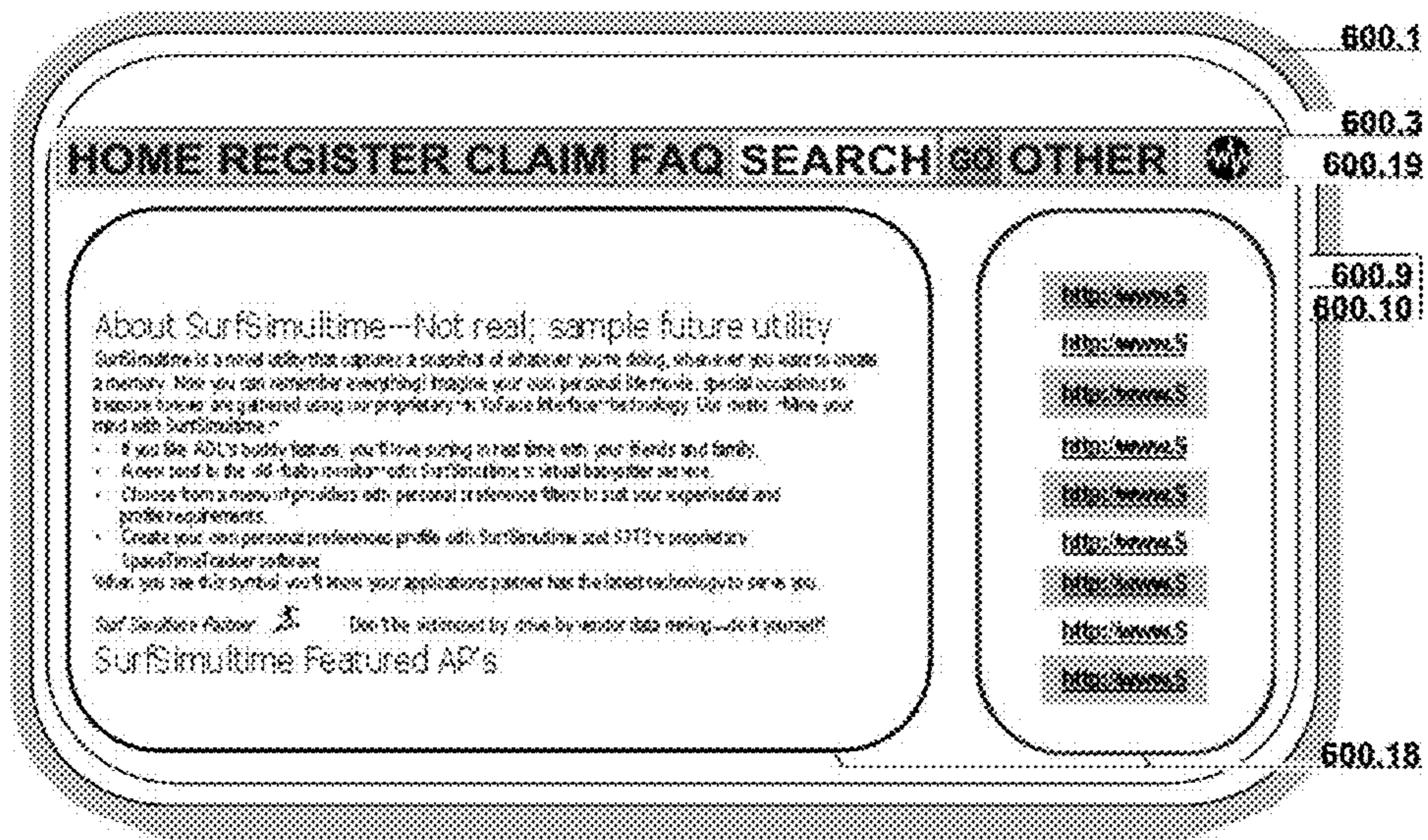
FIG. 87 Homepage 7
