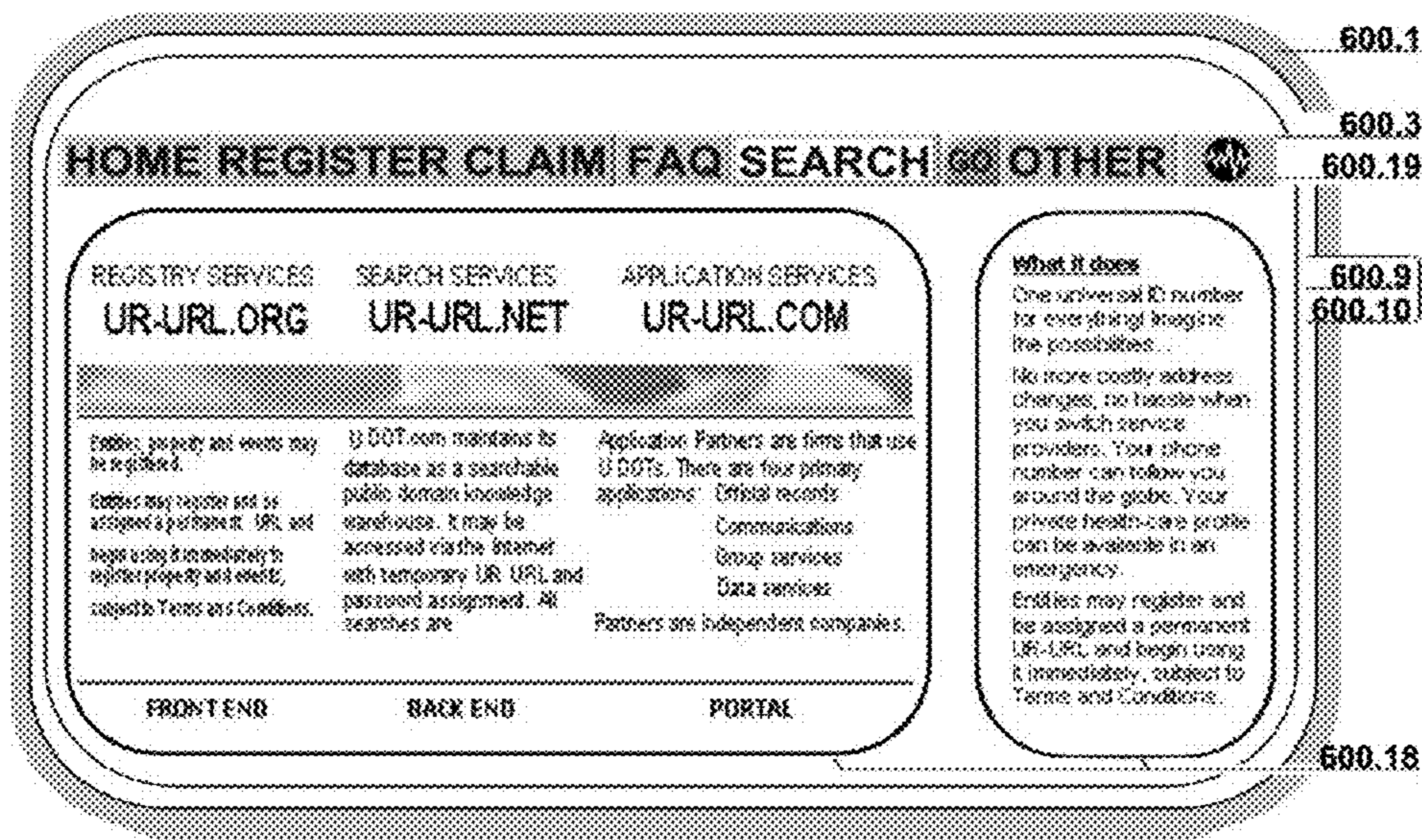
FIG. 82 Homepage 2
