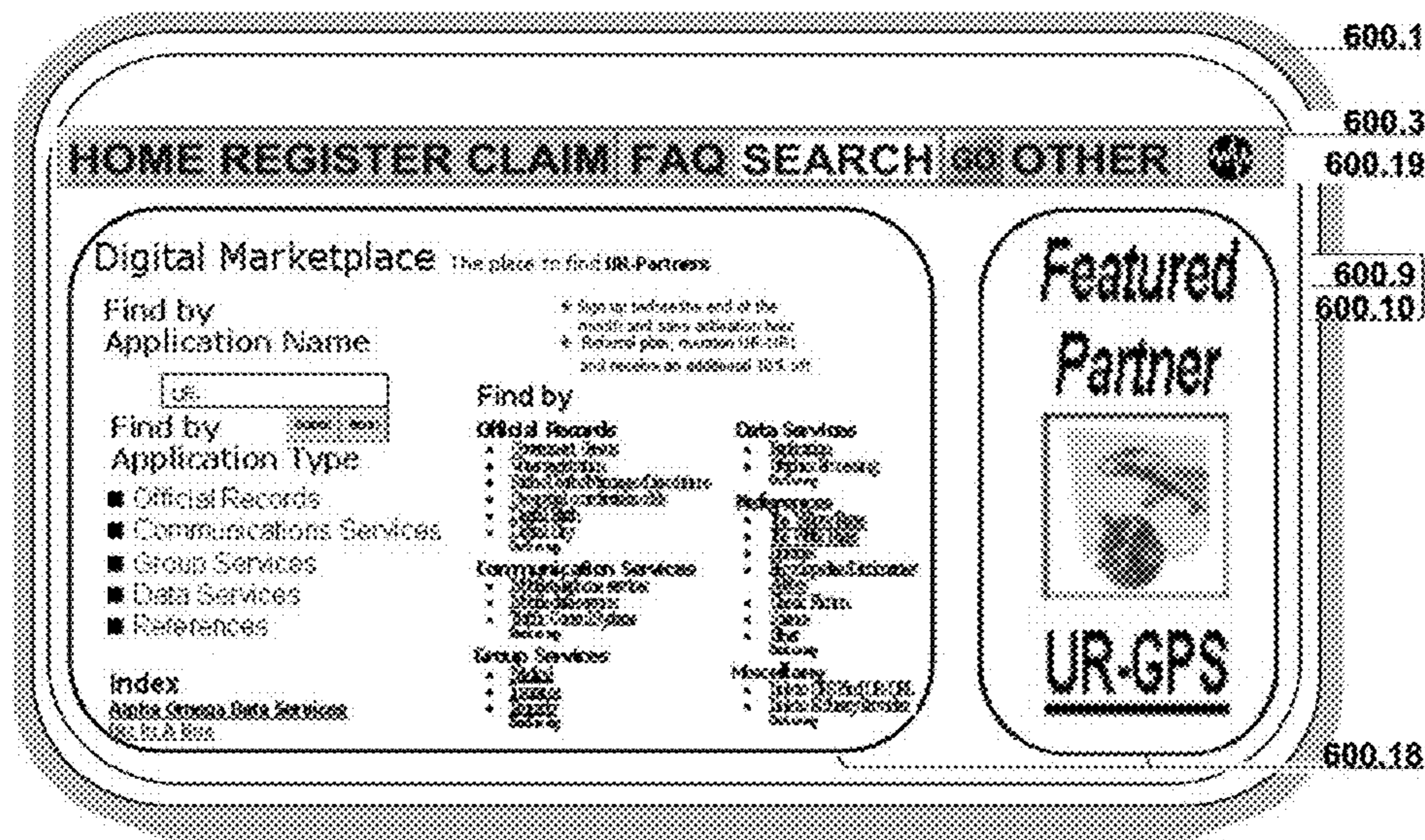
FIG. 91 Homepage 11
