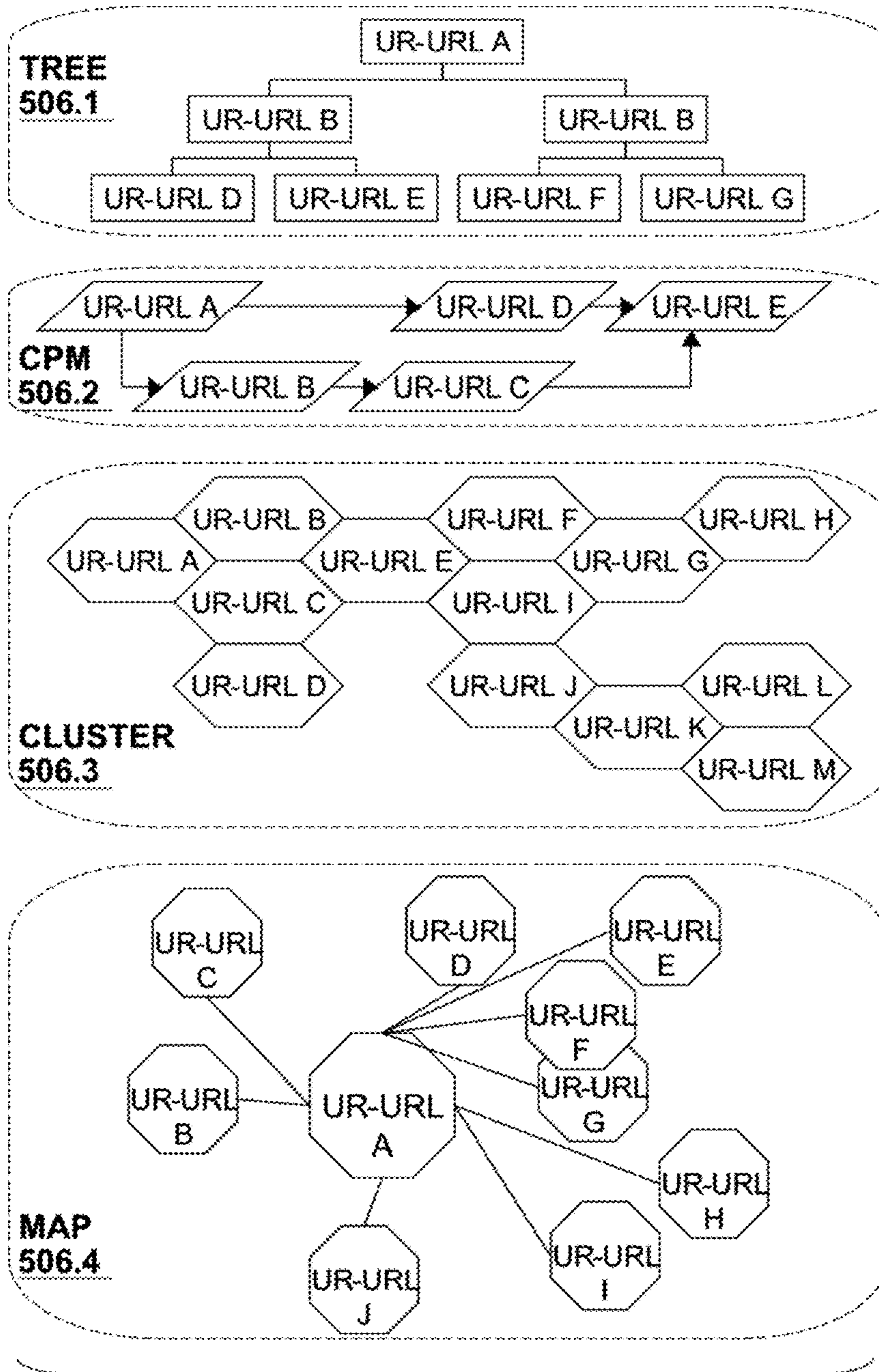
506 Diagrammatic Forms
