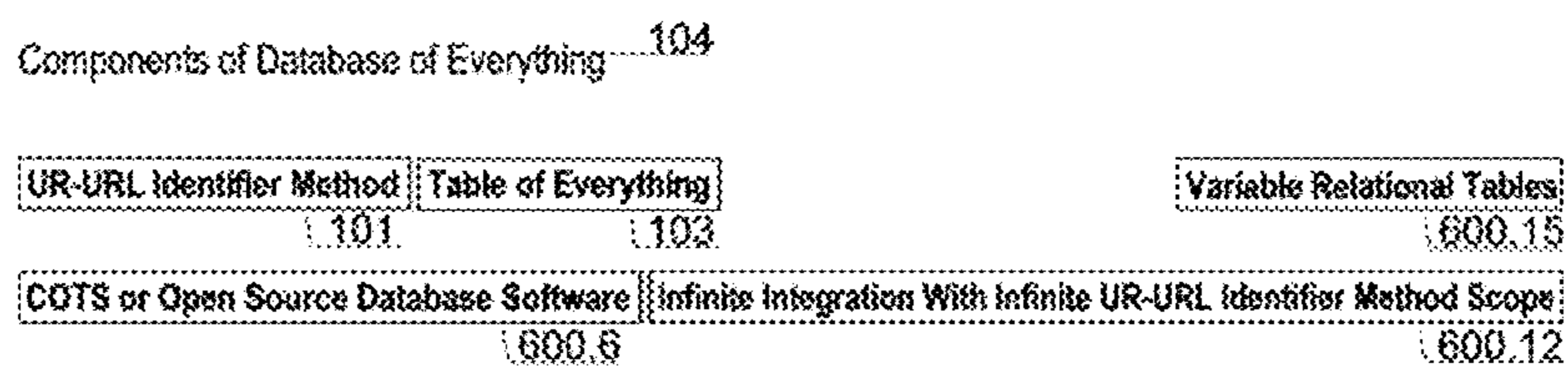
FIG. 38 Database View
