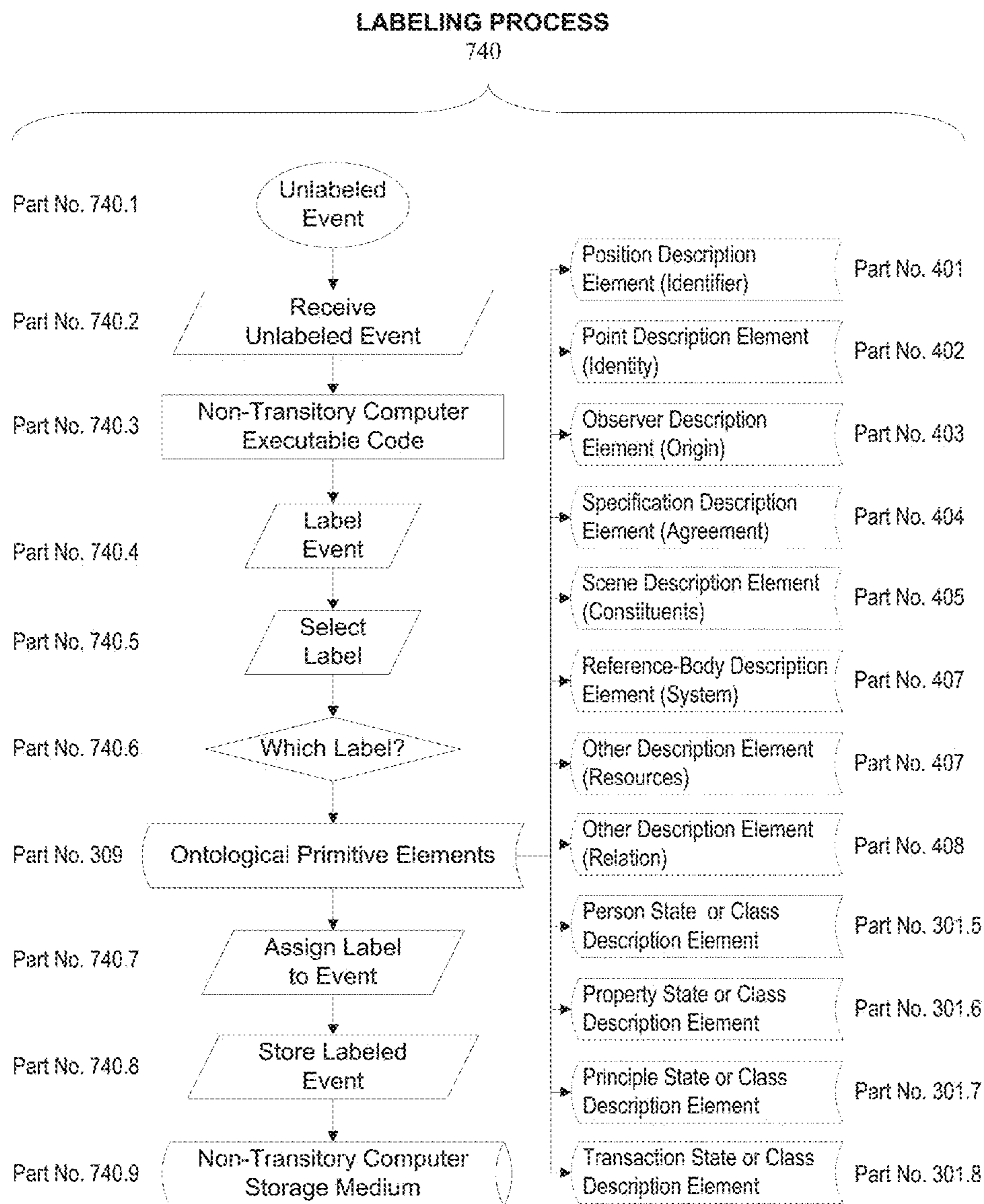
FIG. 112 Block Diagram of Event Claim Labeling Process
