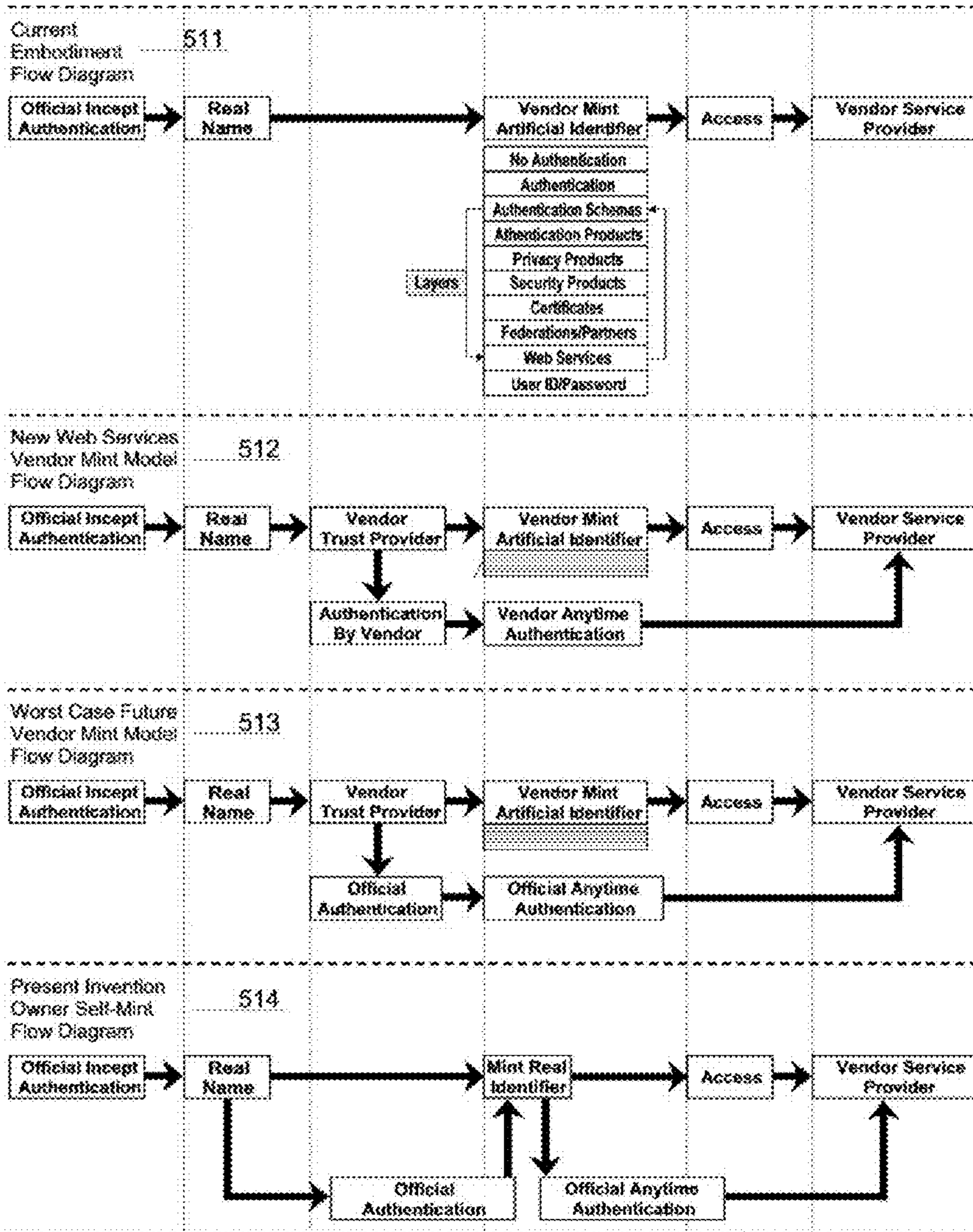
FIG. 58 Access Process Comparison
