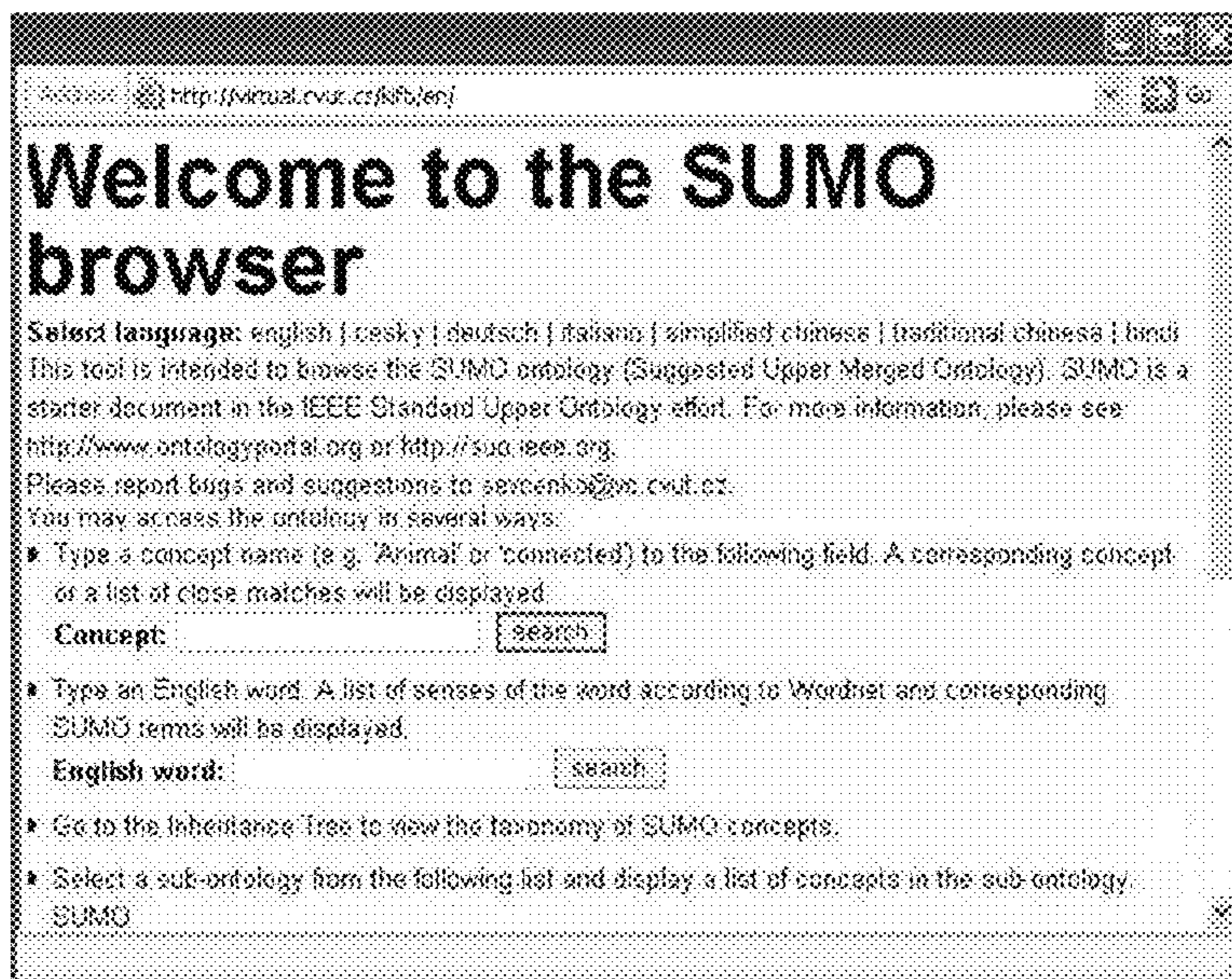
FIG. 25 Object Ontology
