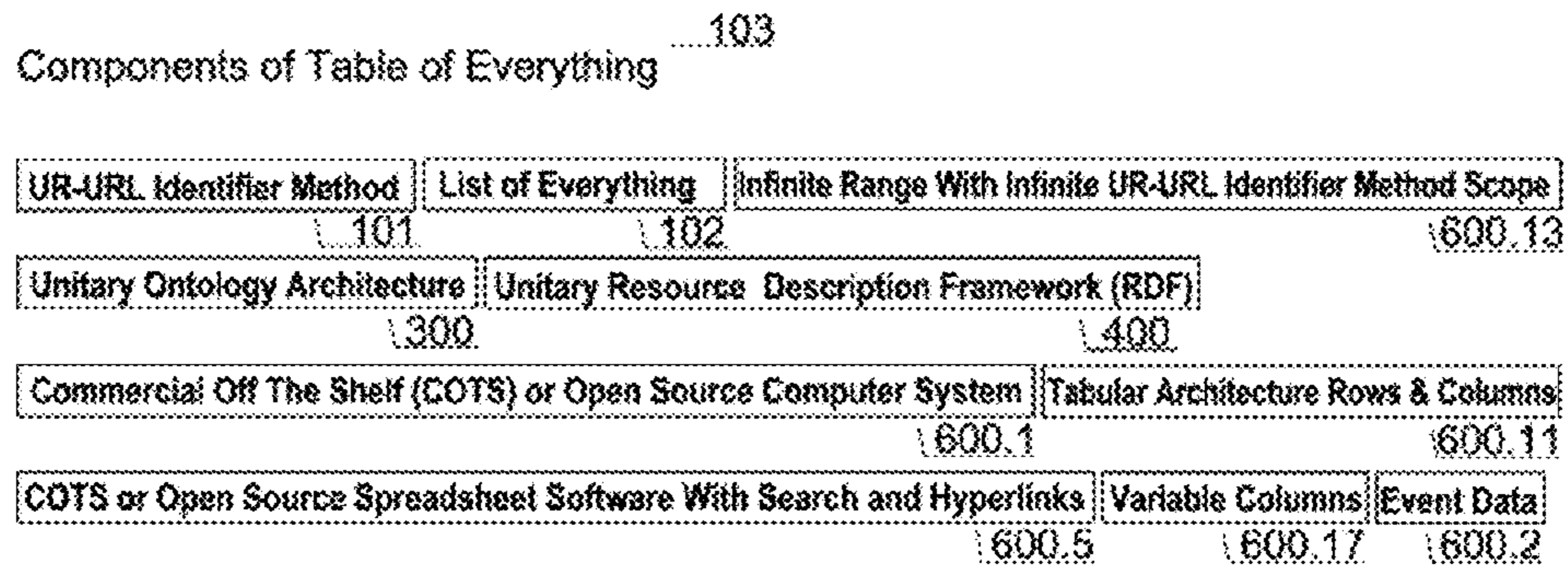
FIG. 18 Table View
