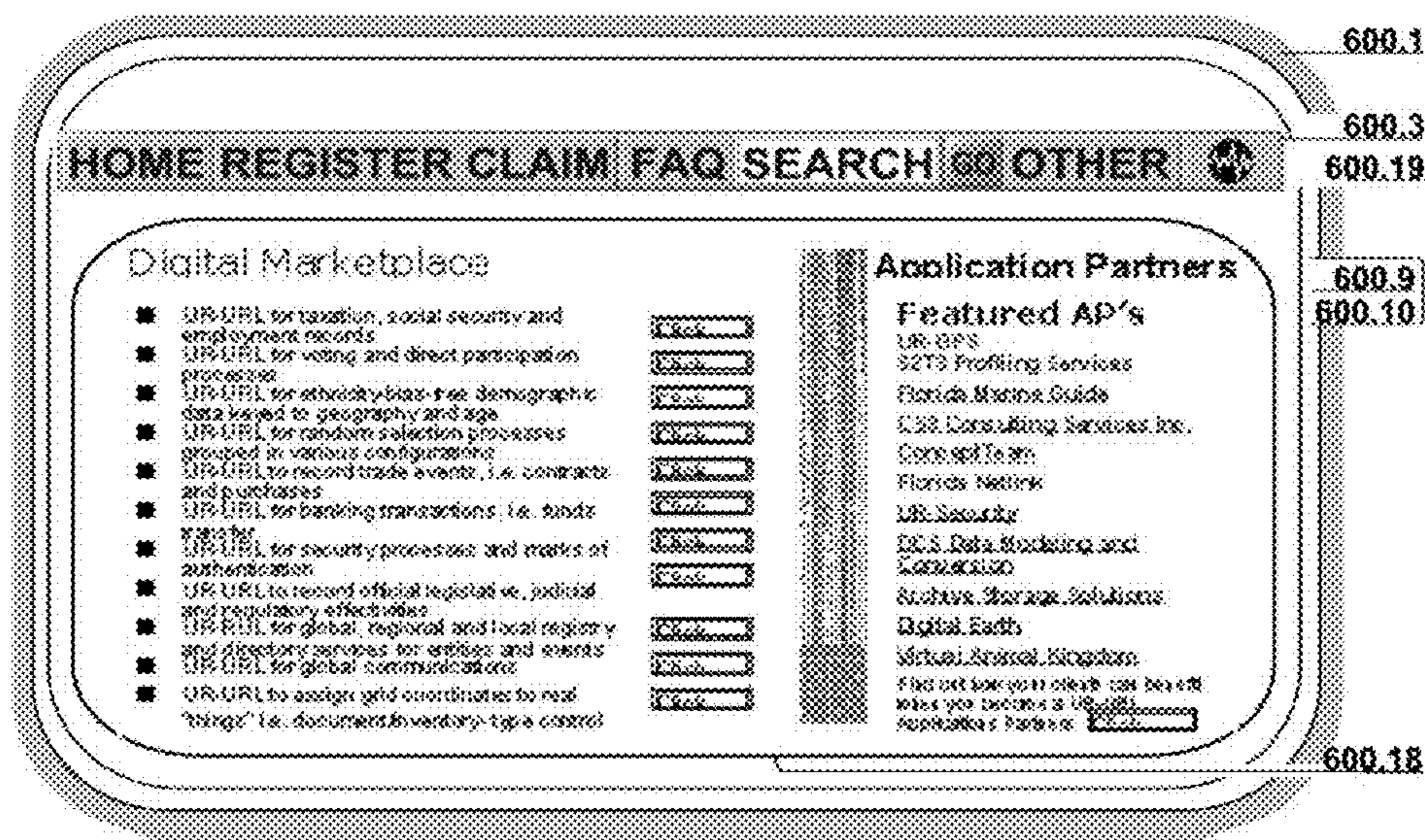
FIG. 92 Homepage 12
