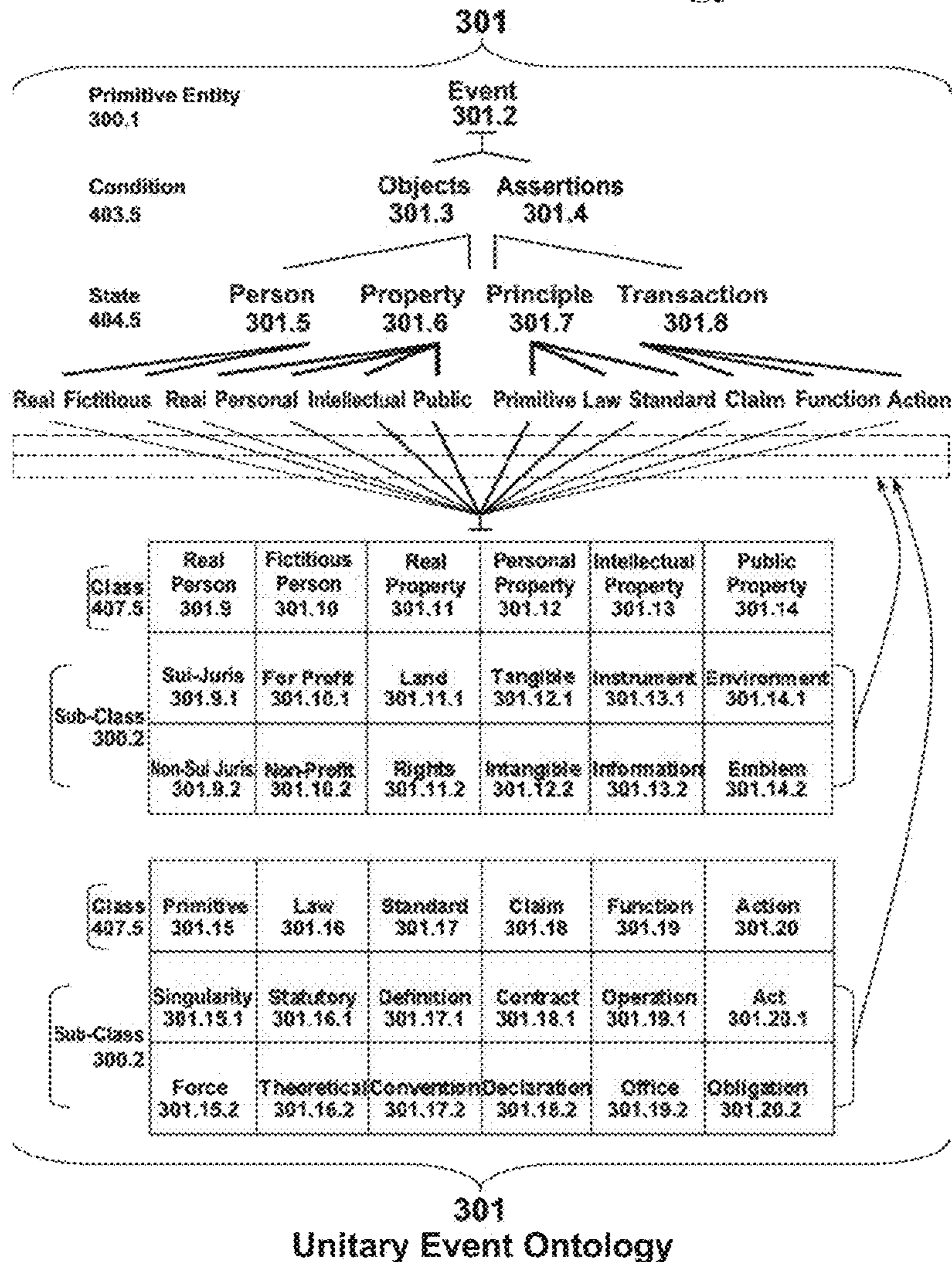
FIG. 22 Event Ontology
