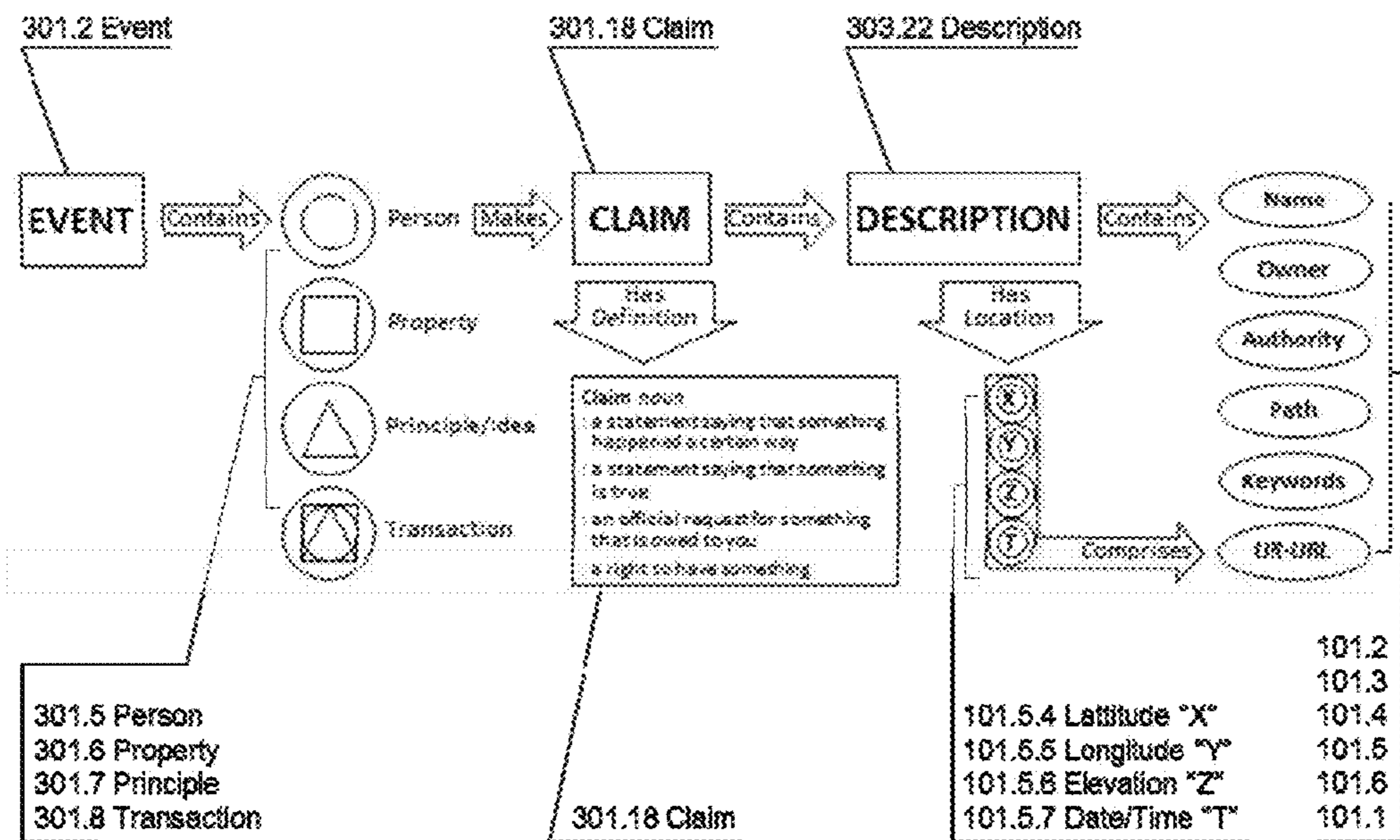
FIG. 115 Concept Map
