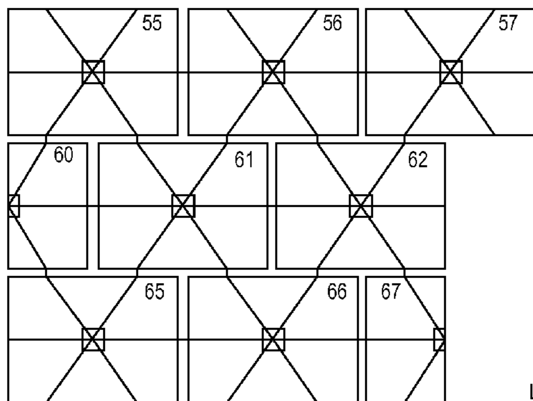
CONFIGURABLE MESH DATA BUS
