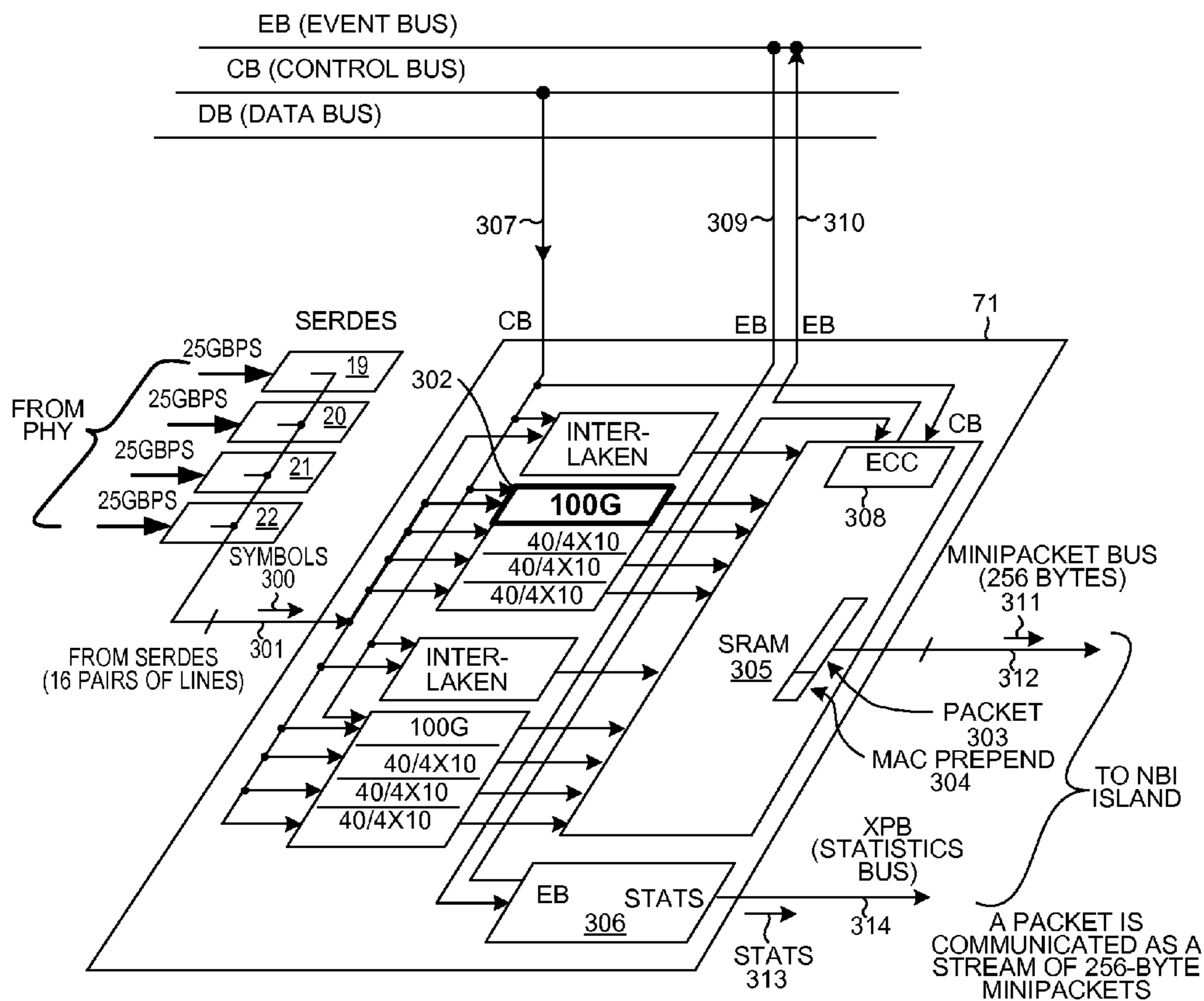
MAC ISLAND (INGRESS)
