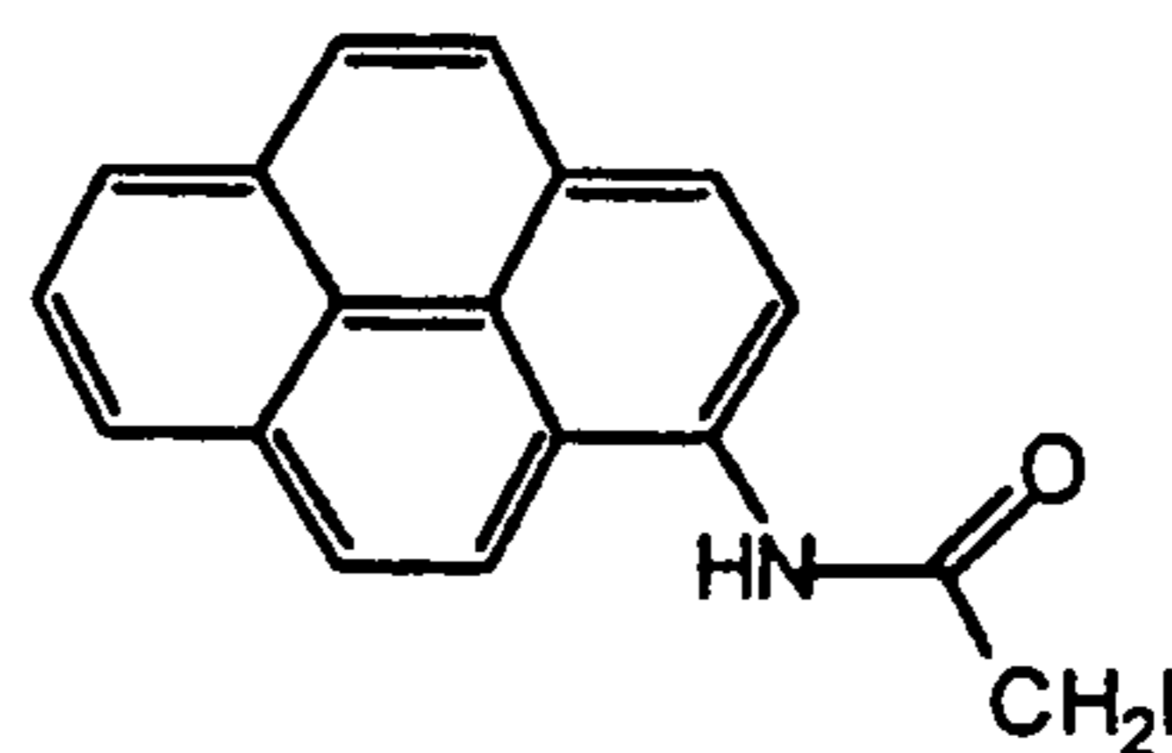
Pyrene
