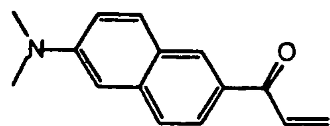
Acrylodan
