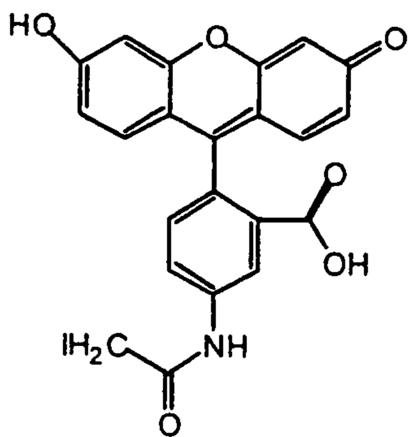
Fluorescein
