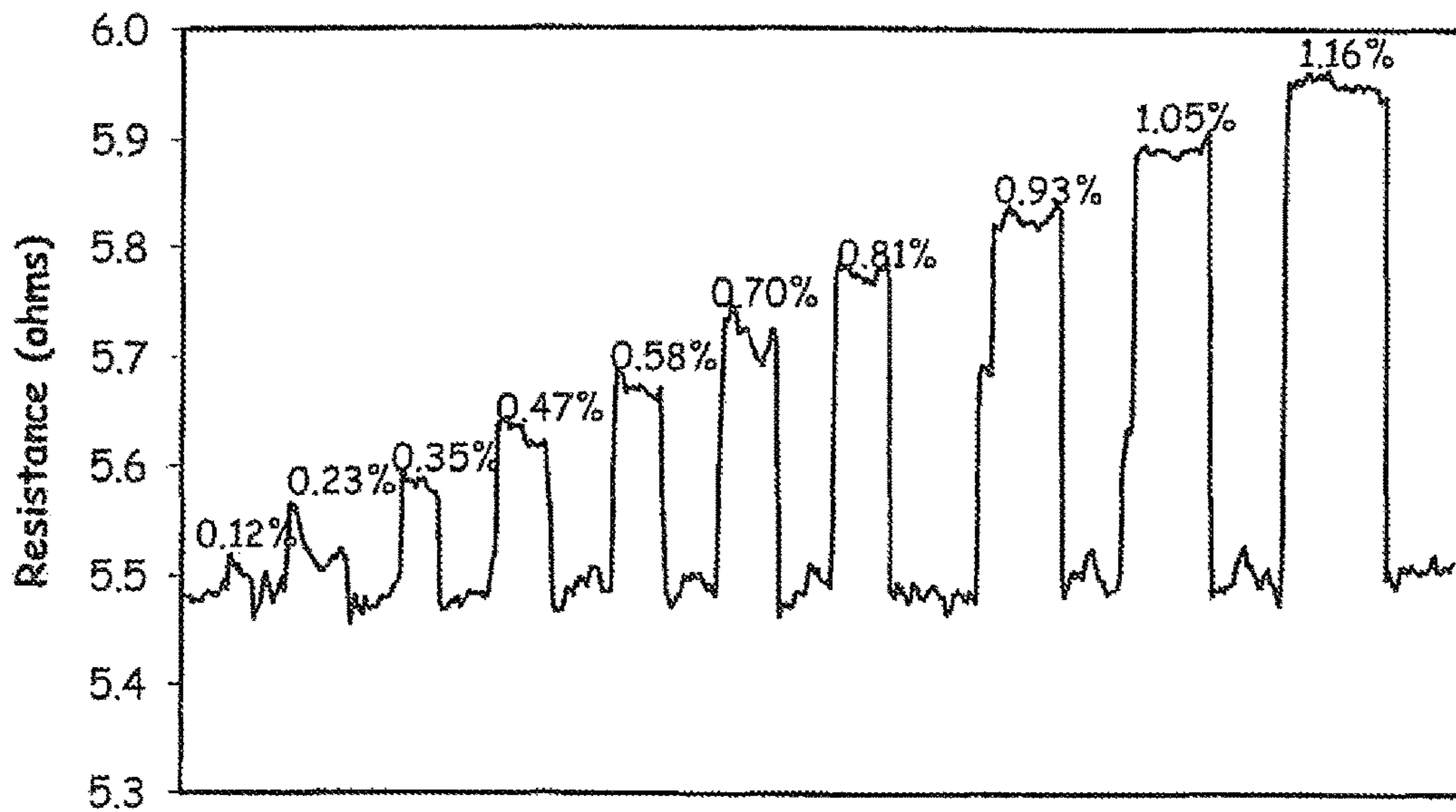
Resistance under Increasing Strain (0 - 1.2%)
