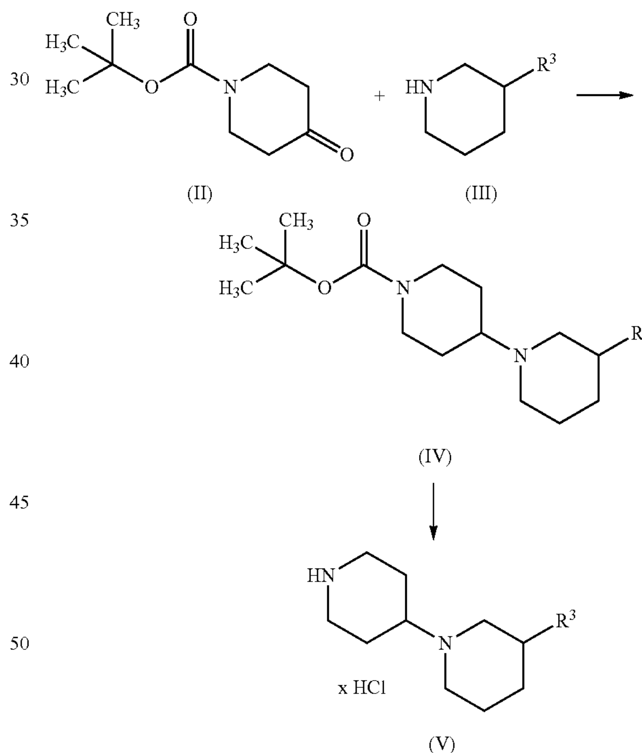
Synthesis Scheme 1:
