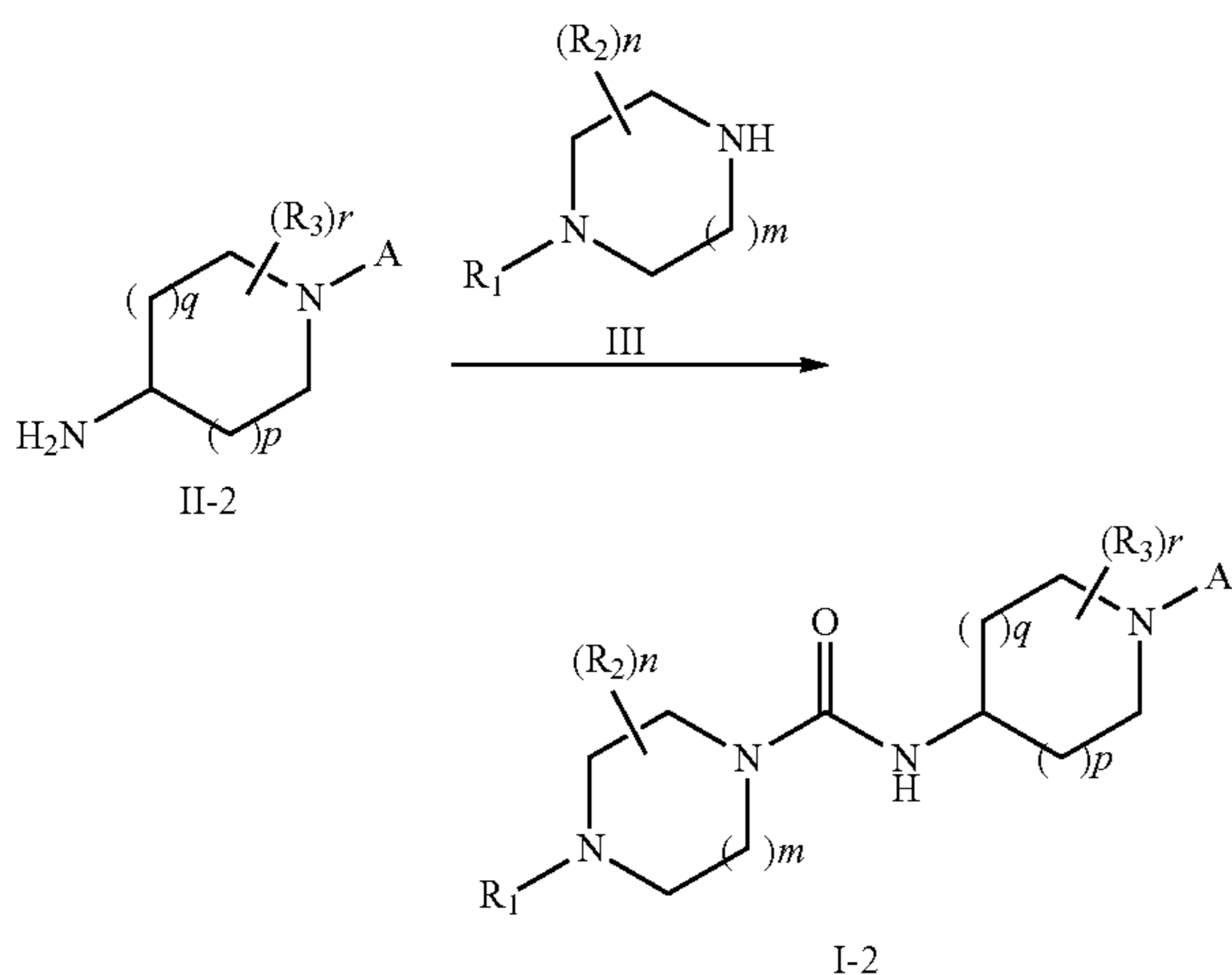
Scheme 2:
