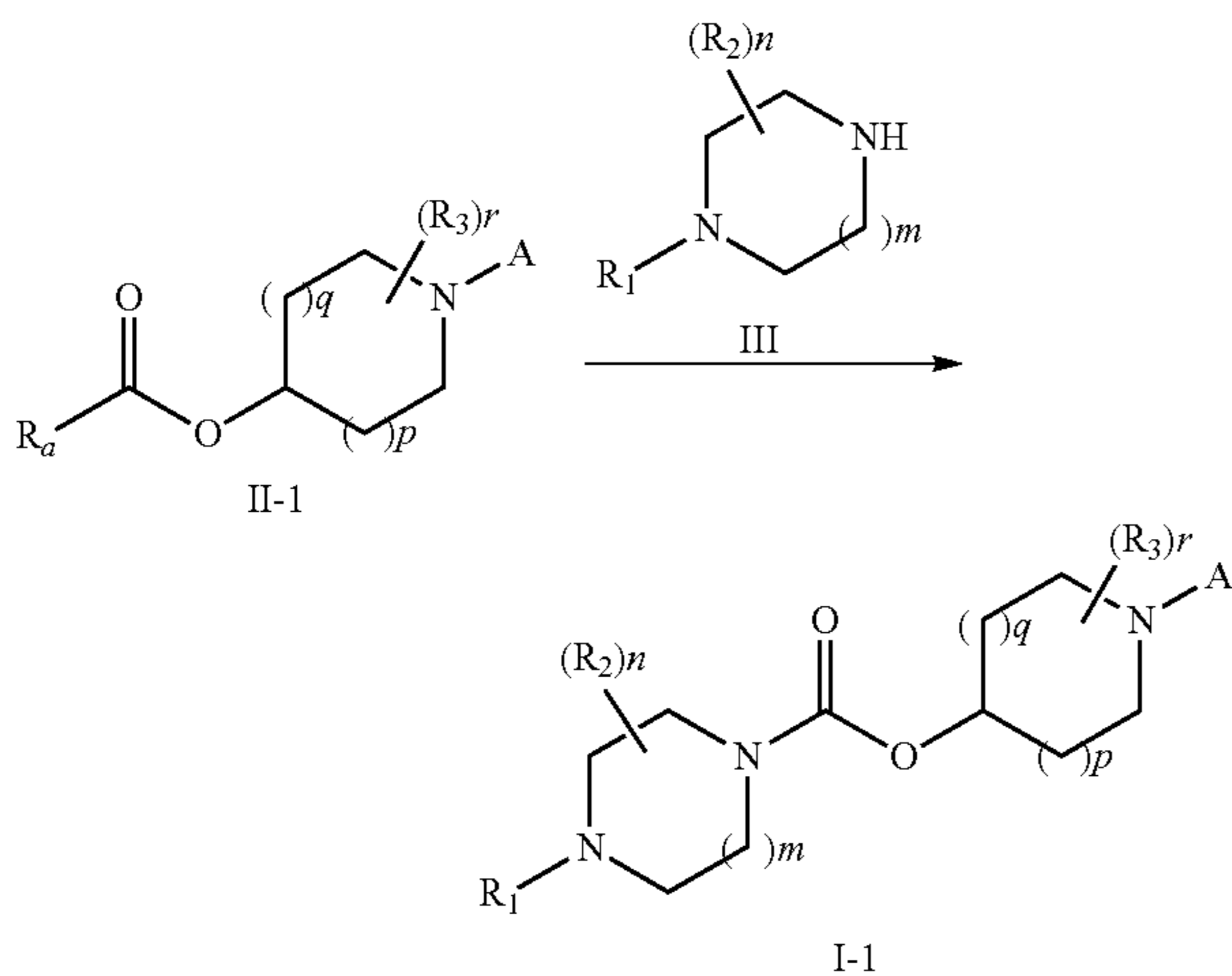
Scheme 1:
