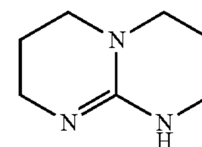
1,5,7-Triazabicyclo[4.4.0]dec-5-ene (TBD)
