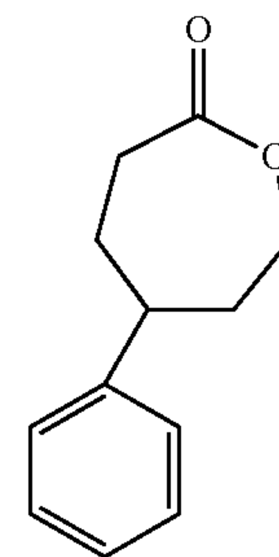
5-Phenyloxepan-2-one (PXO)
