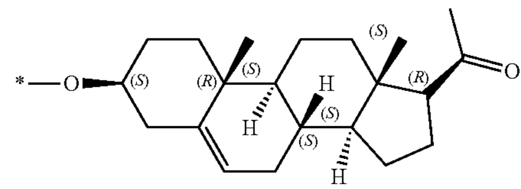
from pregnenolone
