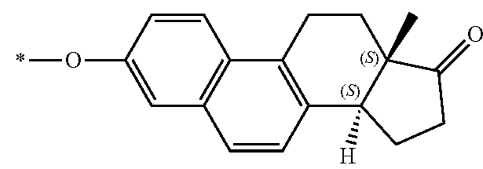
from equilenin
