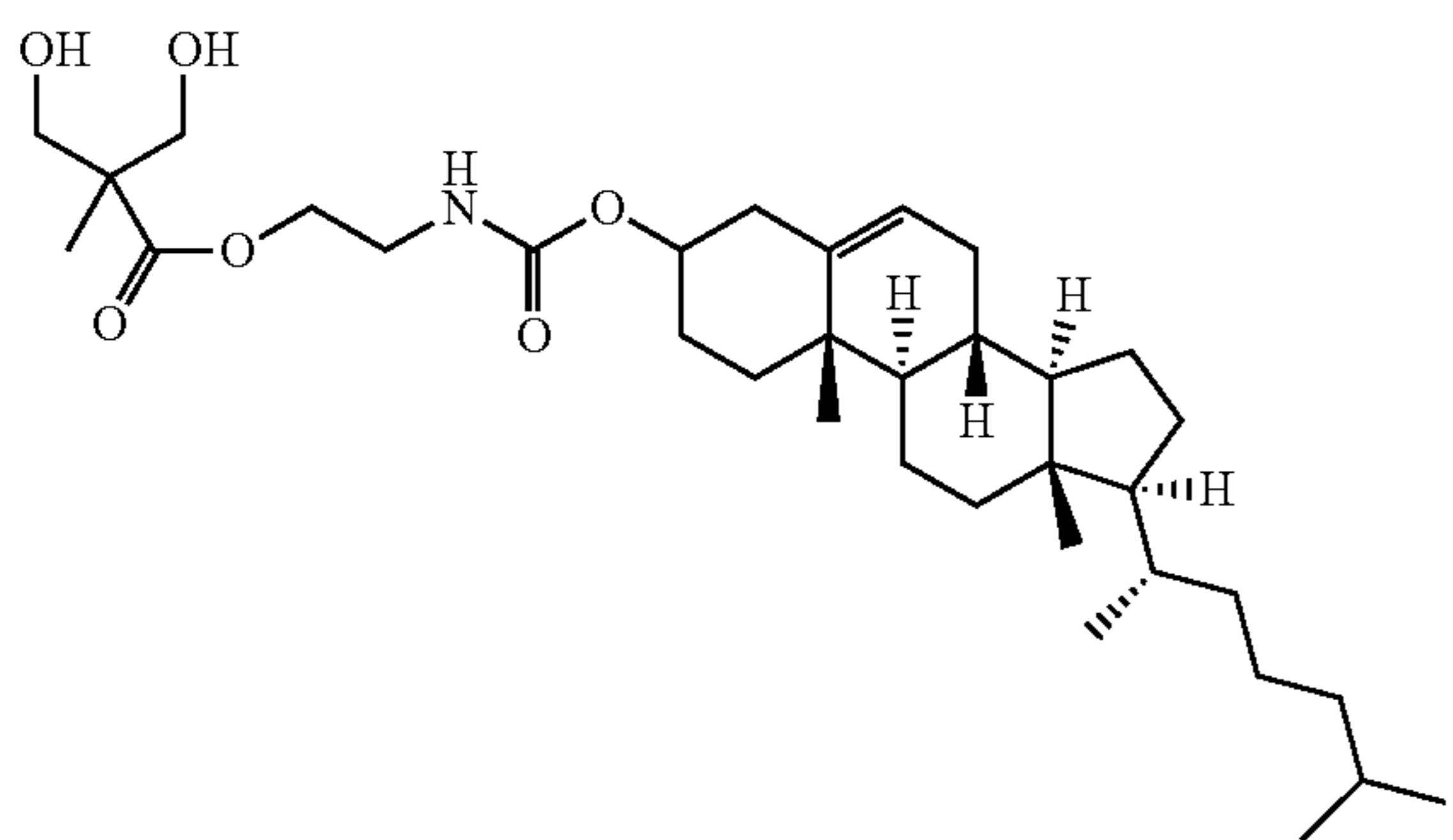
(Chol-MPA)
