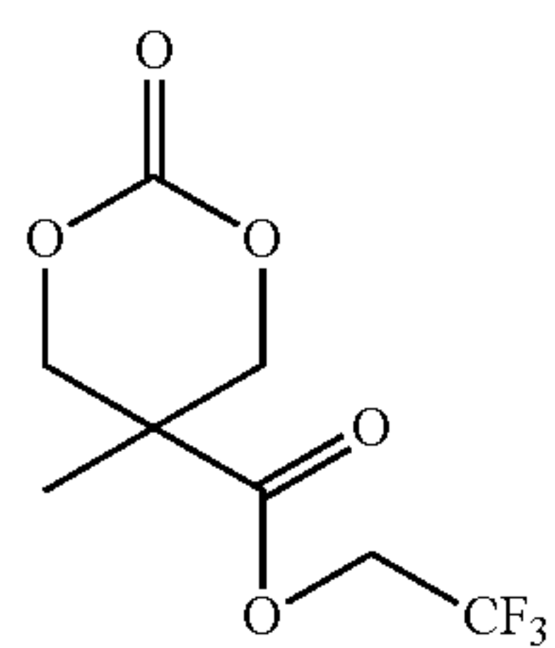
(MTCTFE)
