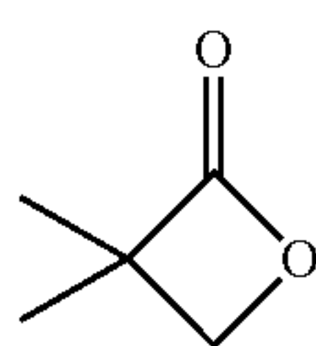
Pivalolactone (PVL)
