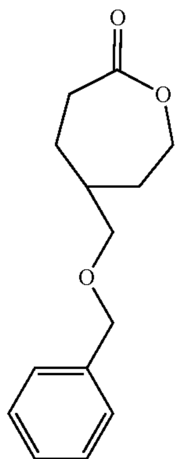
5-(Benzyloxymethyl)oxepan-2-one (BOMXO)
