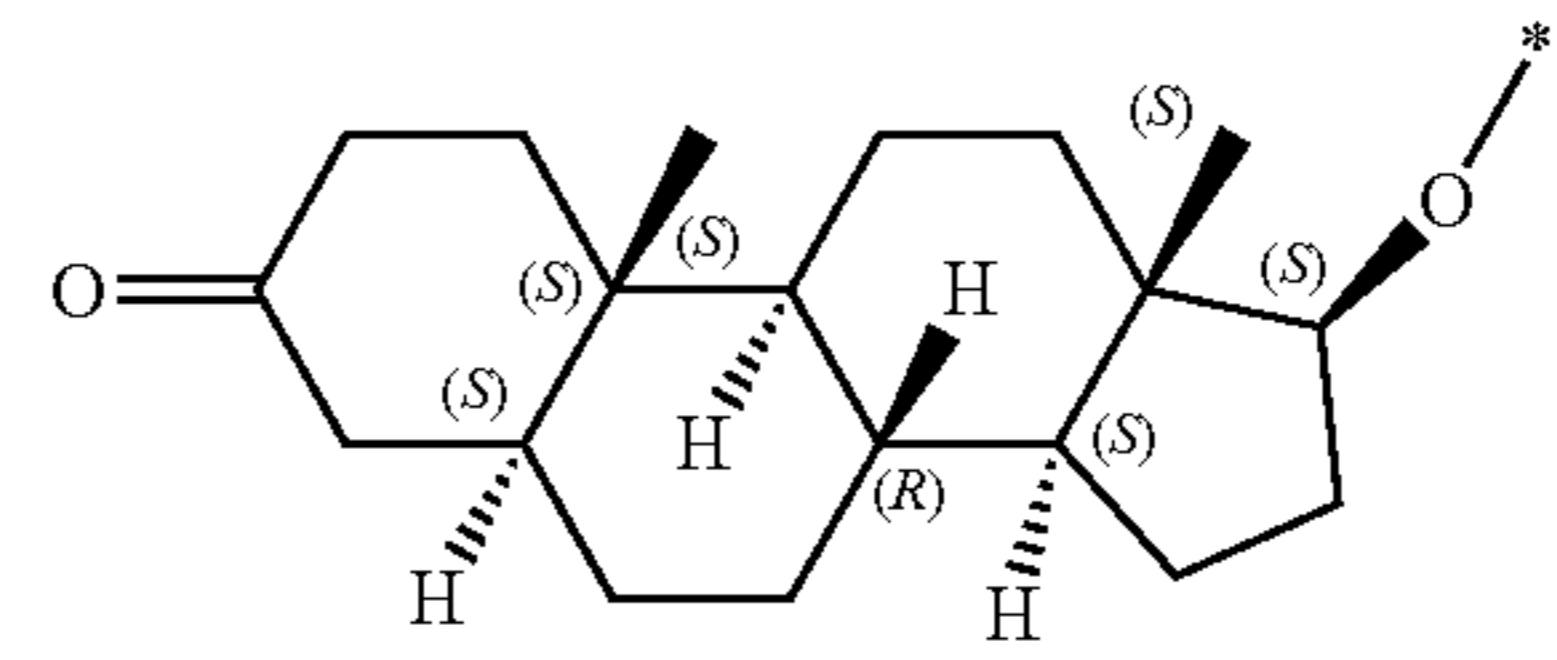
from dihydrotestosterone
