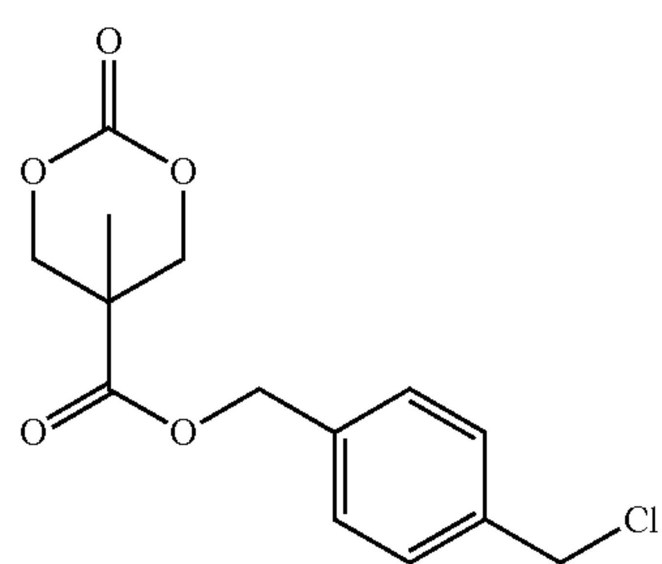
(MTC-BnCl)
