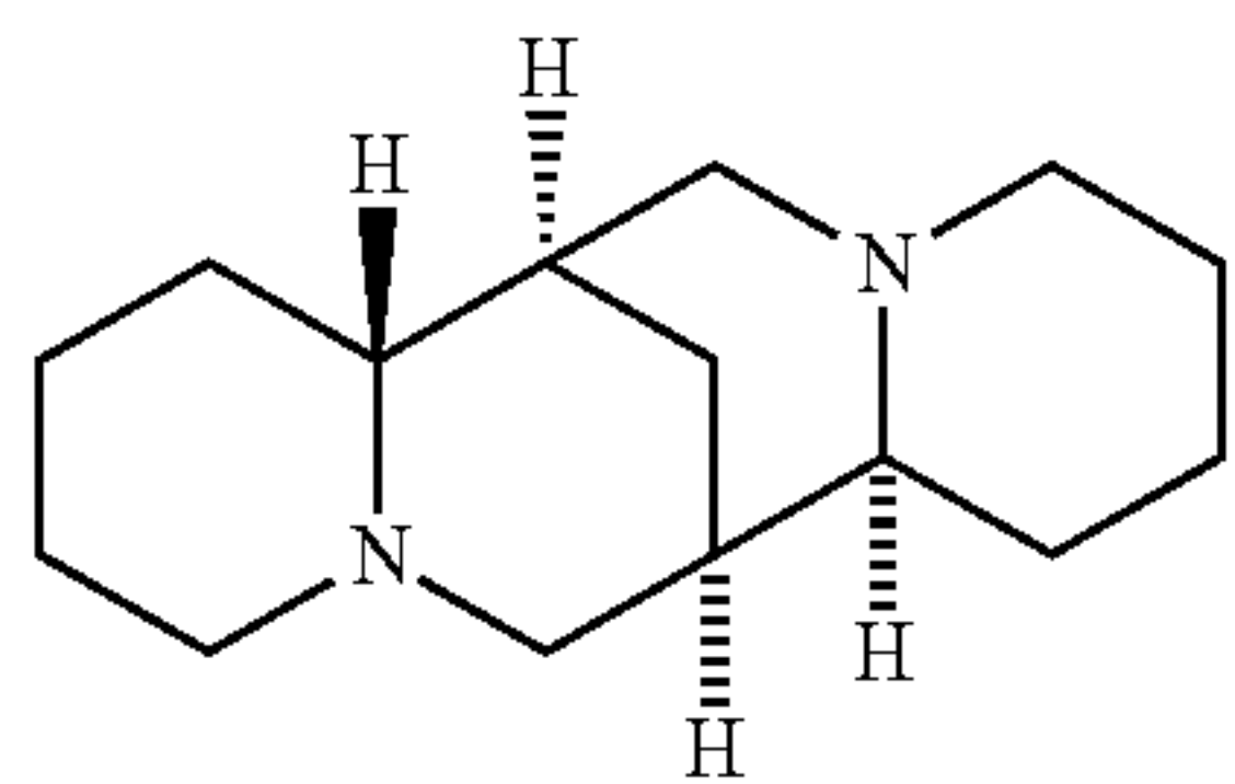
(-)-Sparteine (Sp)
