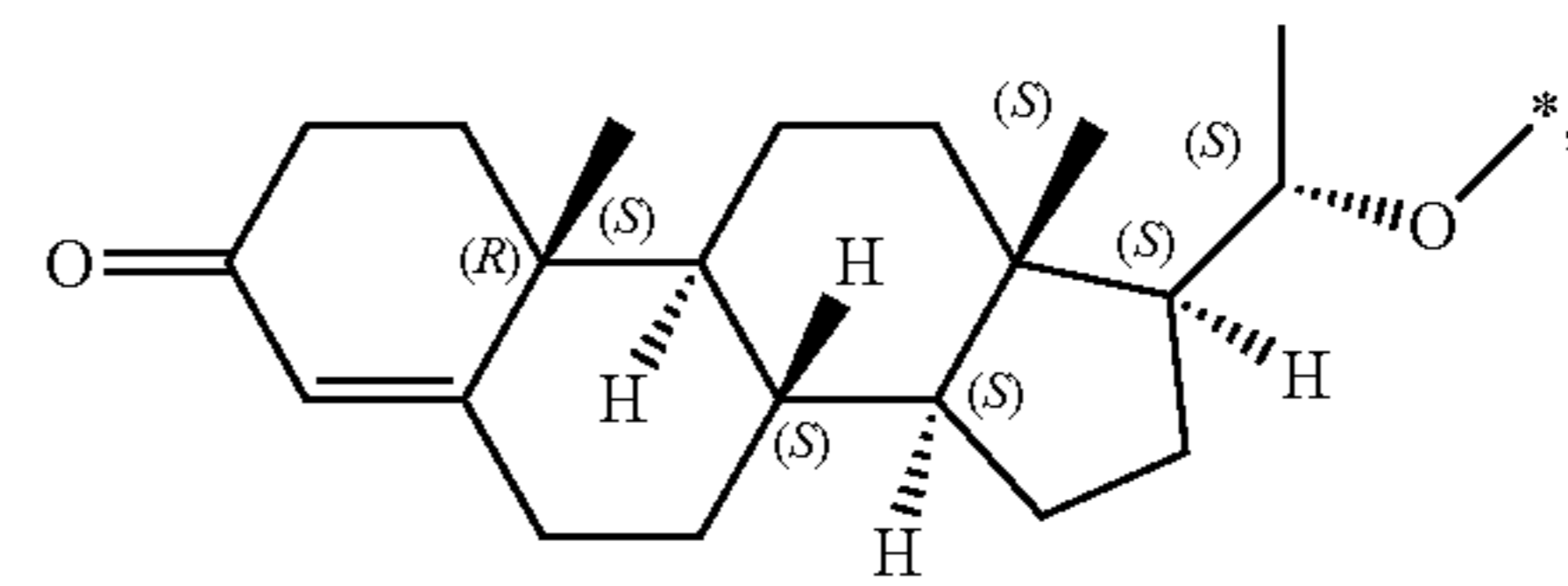
from dihydroprogesterone
