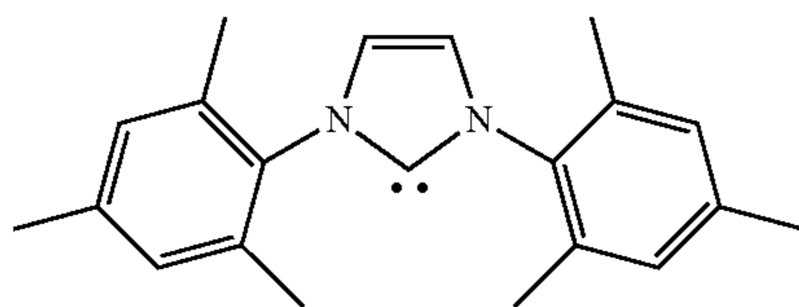
1,3-Bis(2,4,6-trimethylphenyl)imidazol-2-ylidene (Im-2)
