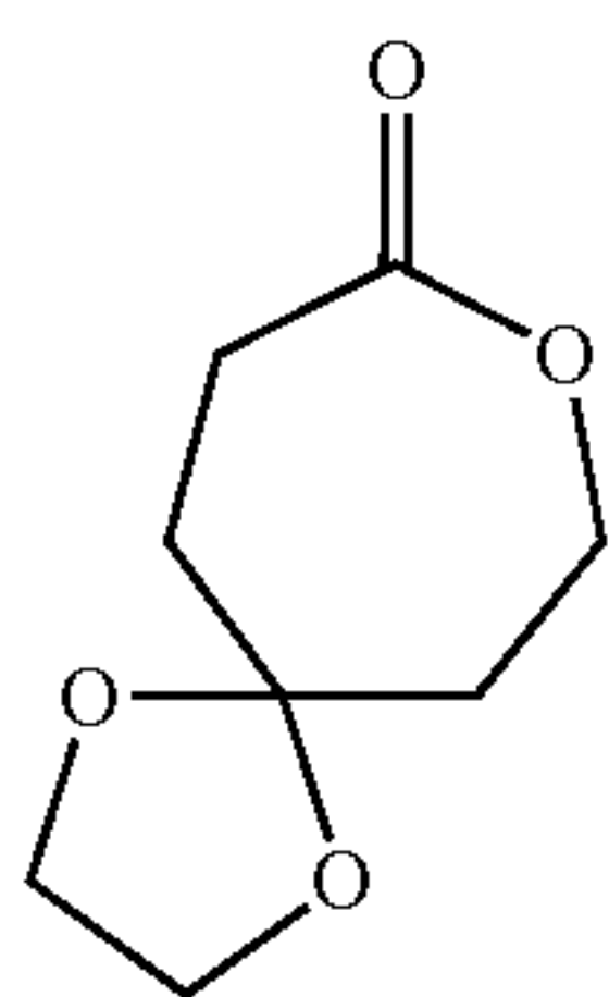
1,4,8-Trioxa(4,6)spiro-9-undecane (TOSUO)
