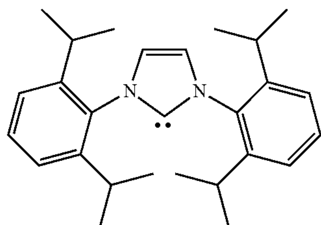
1,3-Bis(2,6-di-i-propylphenyl)imidazol-2-ylidene (Im-3)
