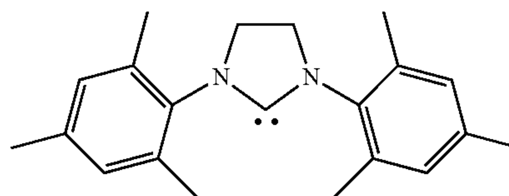
1,3-Bis(2,4,6-trimethylphenyl)-4,5- dihydroimidazol-2-ylidene (Im-7)
