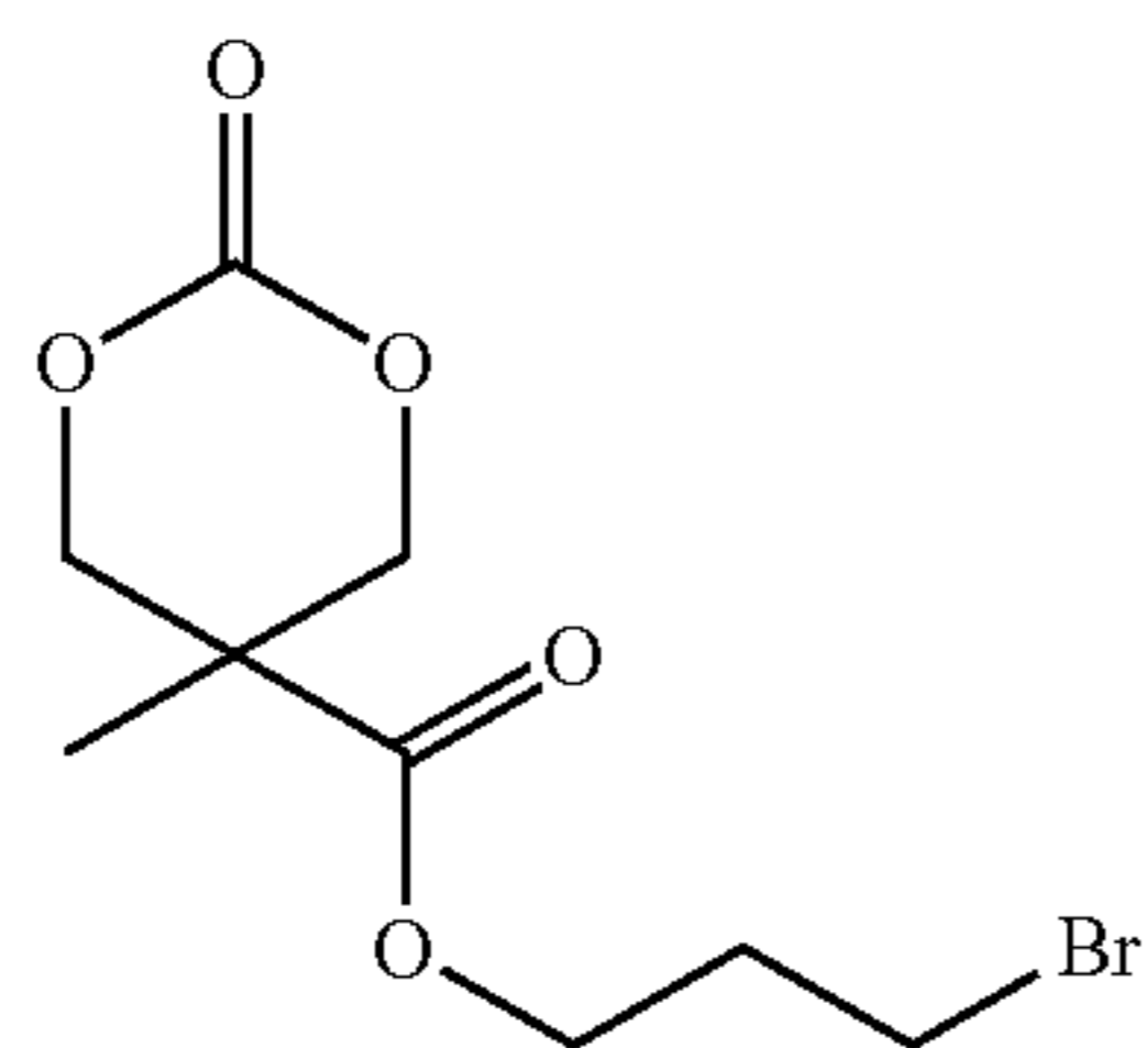
(MTC-PrBr)
