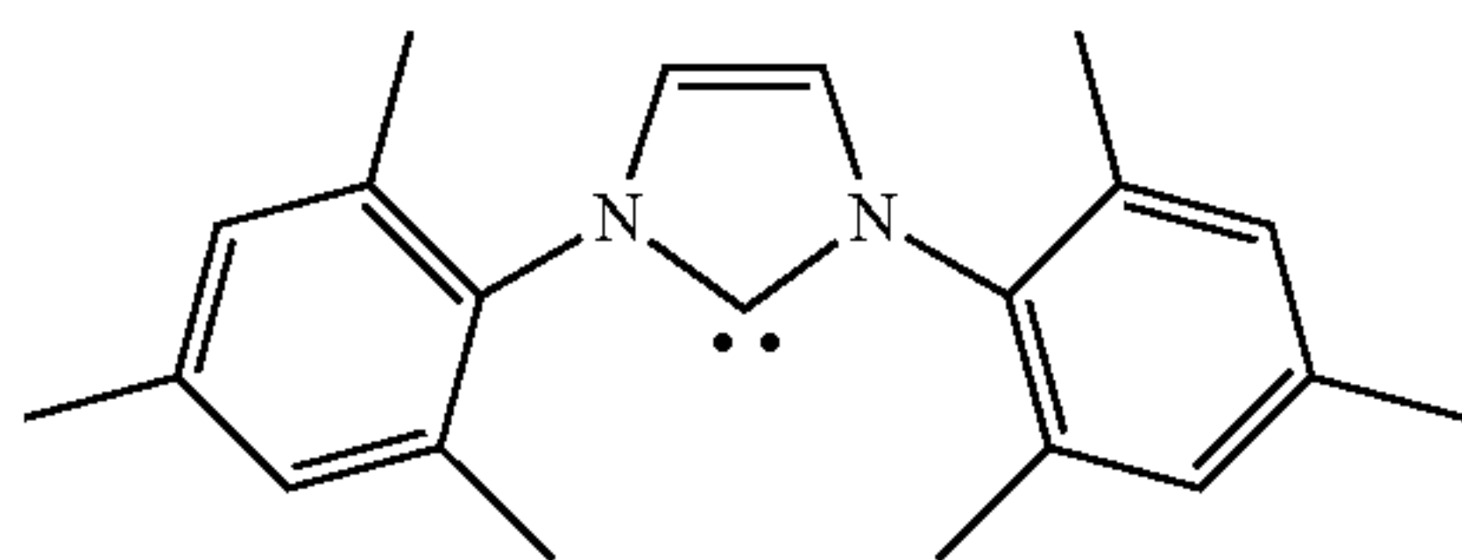
1,3-Bis(2,4,6-trimethylphenyl)imidazol-2-ylidene (Im-2)
