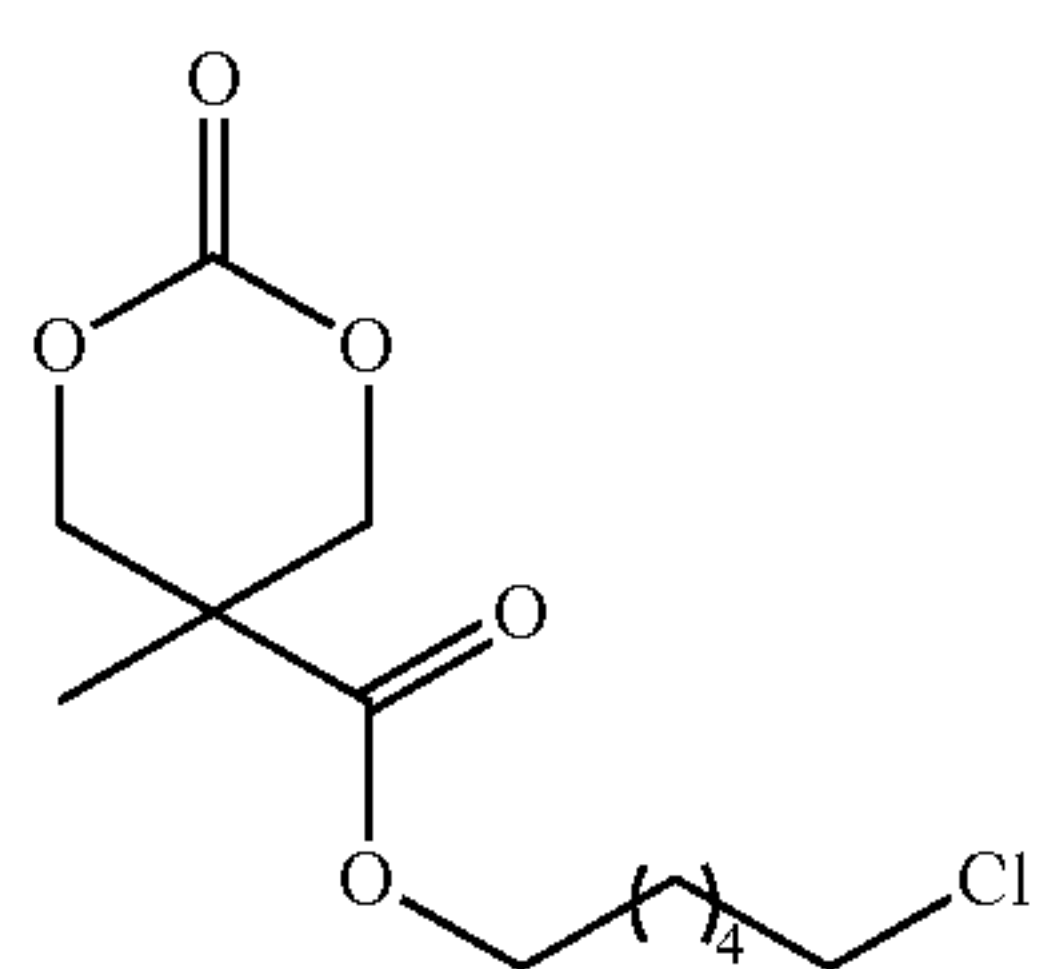
(MTC-C6Cl)
