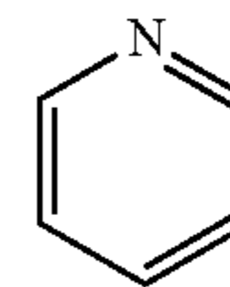
Pyridine (Py)
