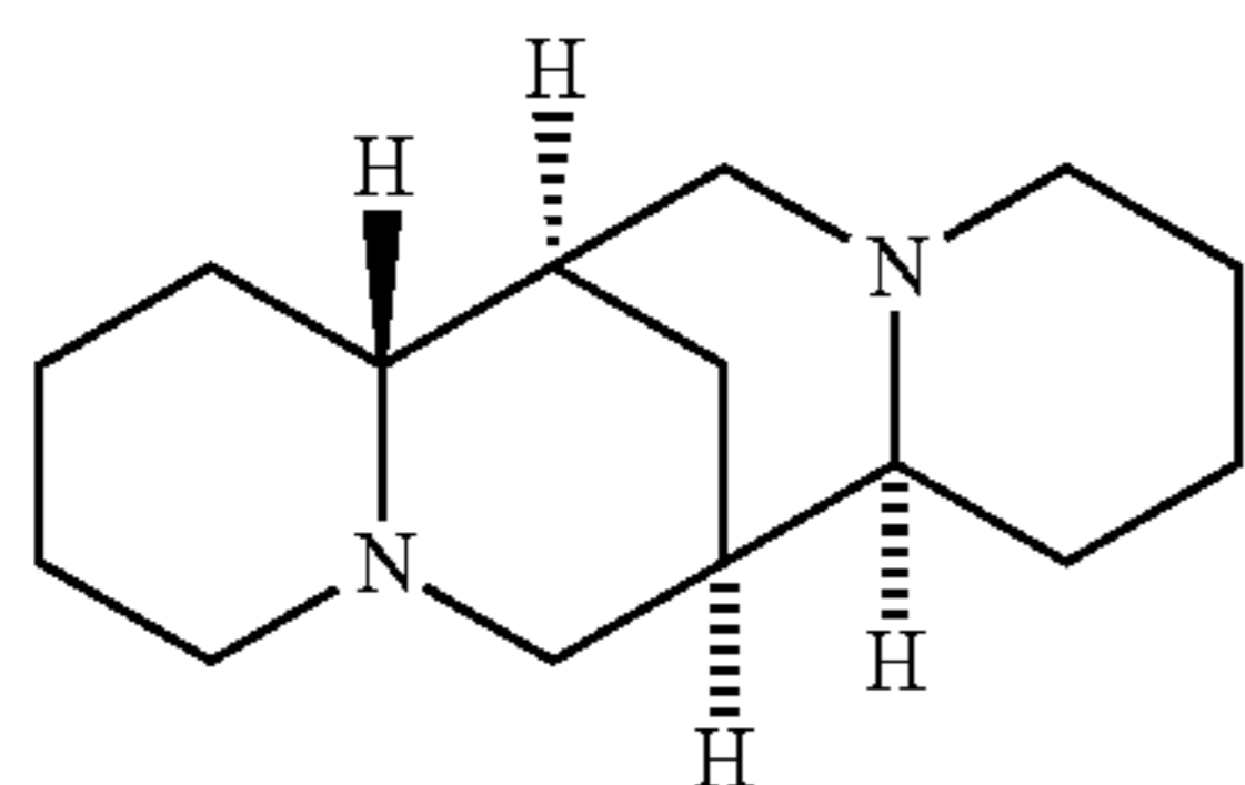
(-)-Sparteine (Sp)
