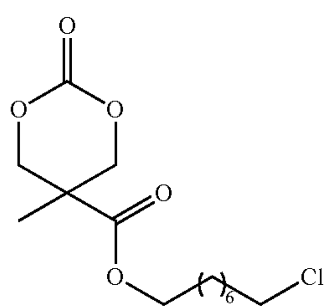
(MTC-C8Cl)
