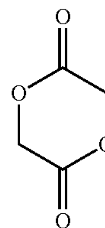
Glycolide (GLY)
