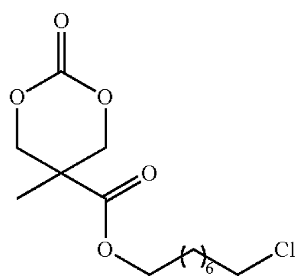
(MTC-C8Cl)
