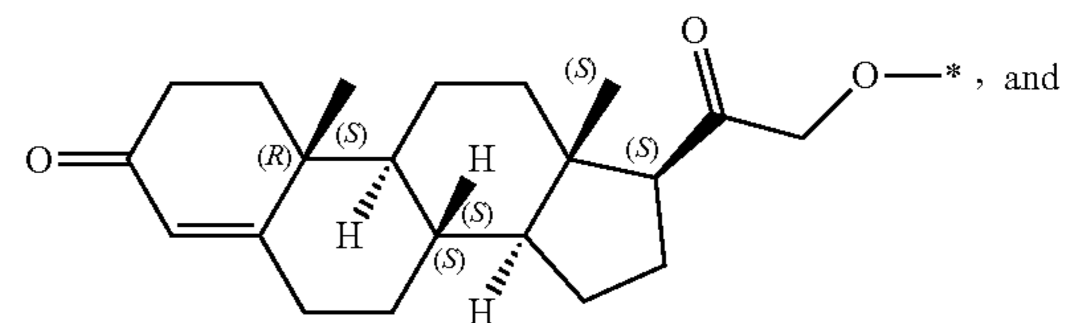
from deoxycorticosterone
