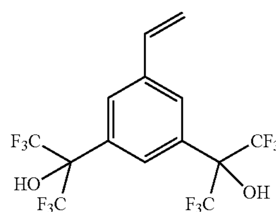
3,5-HFA-St
