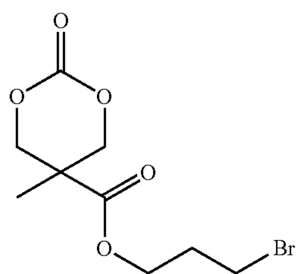
(MTC-PrBr)
