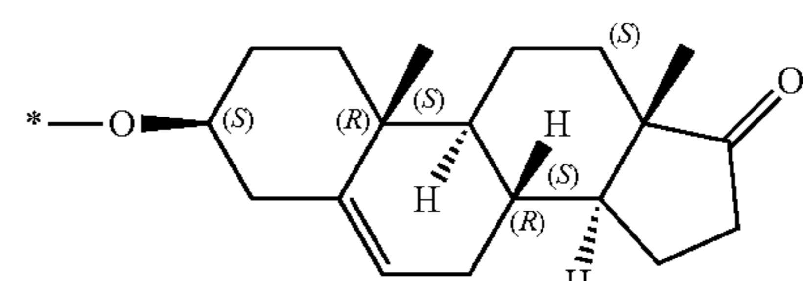
from dehydroepiandrosterone
