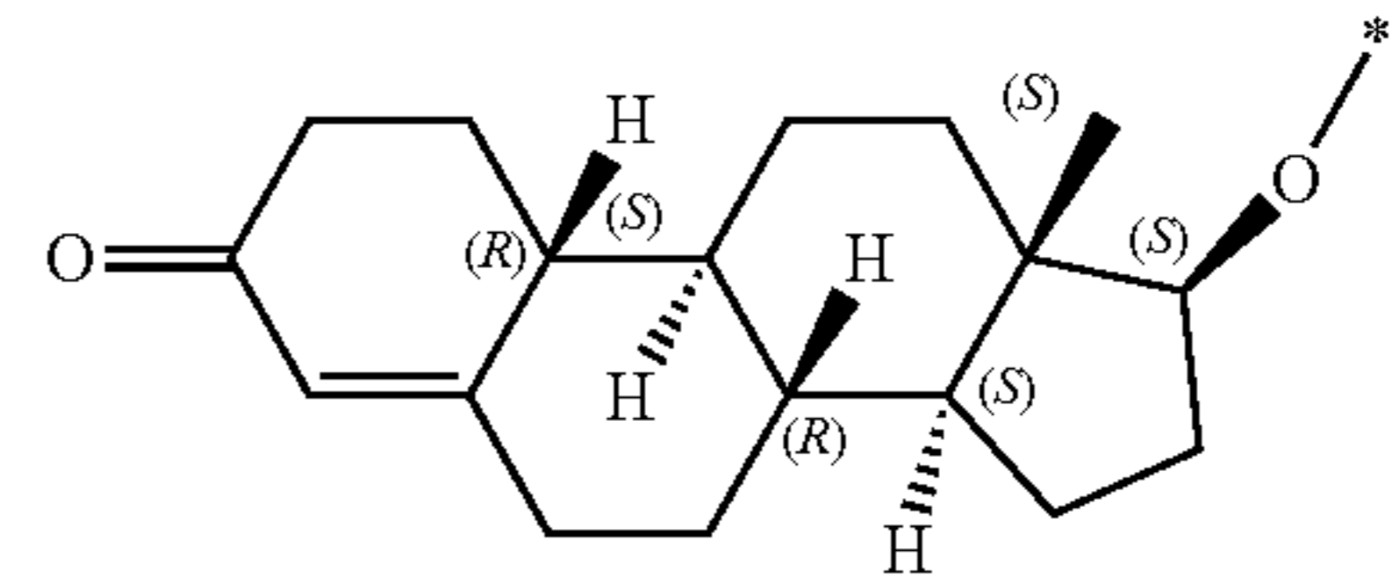
from nandrolone
