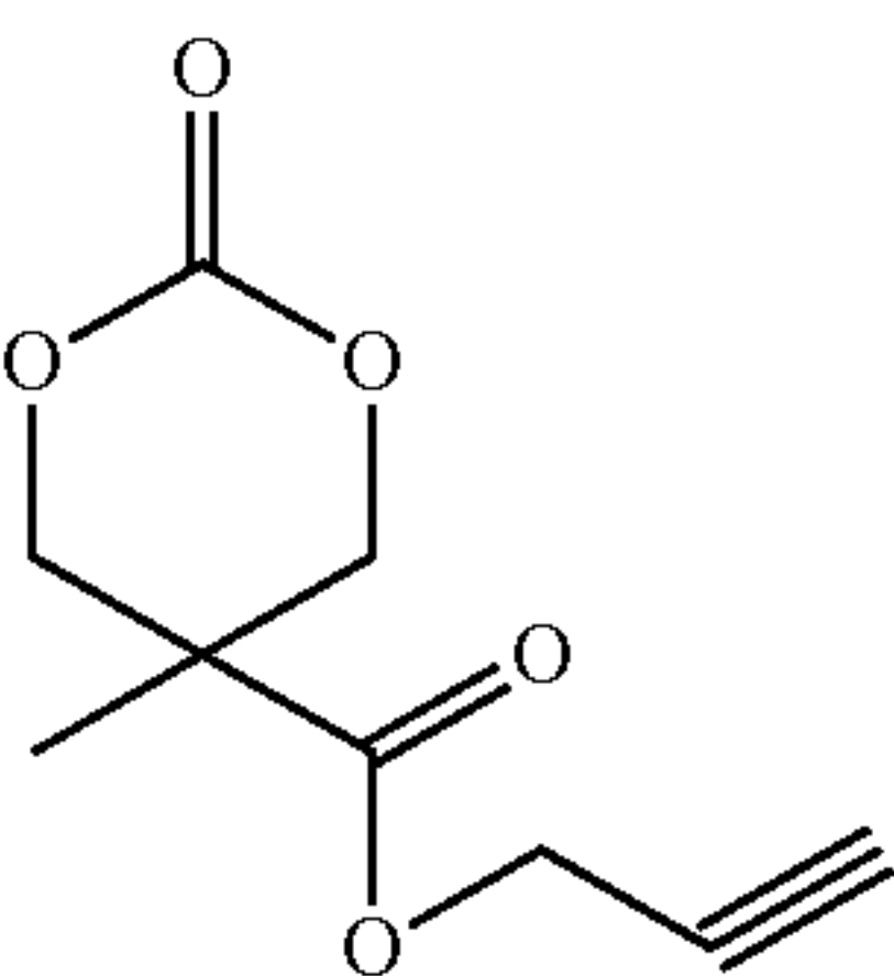
(MTCTFE)
