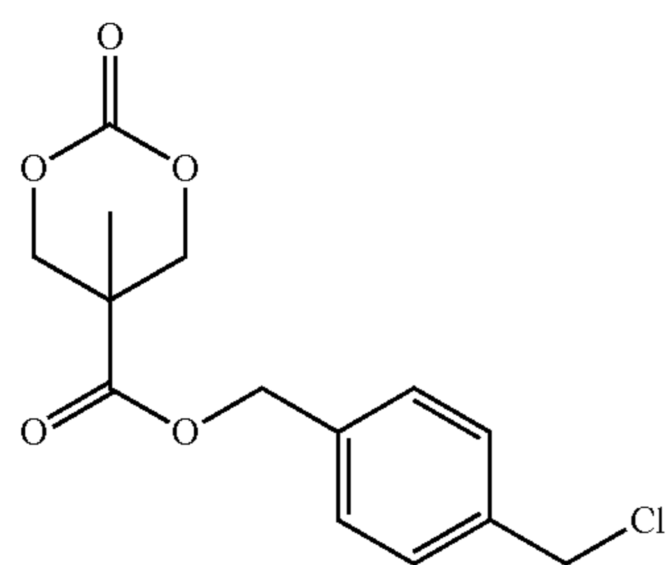
(MTC-BnCl)
