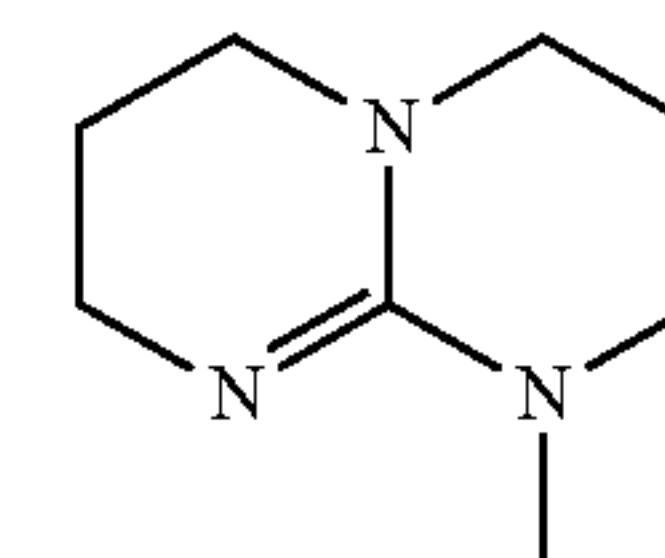
7-Methyl-1,5,7-triazabicyclo[4.4.0]dec-5-ene (MTBD)
