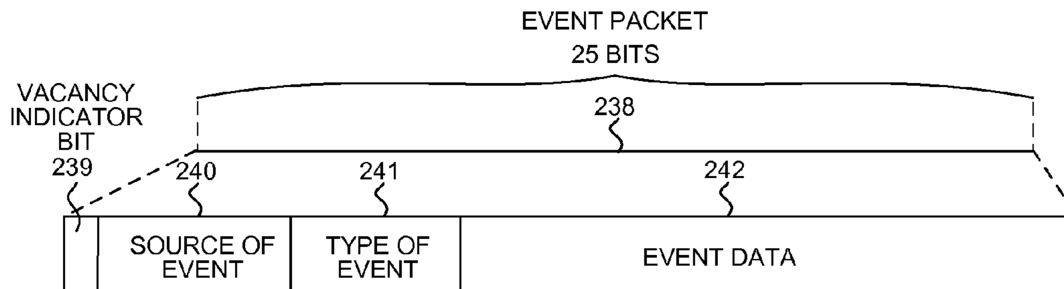
EVENT PACKET BIT SEQUENCE FIG. 38A
