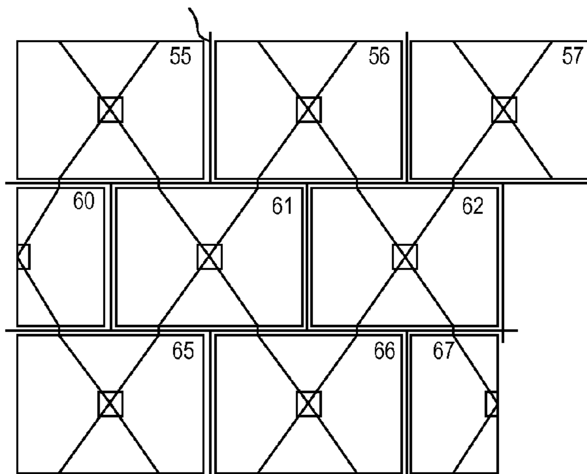
CONFIGURABLE MESH CONTROL BUS FIG. 27
