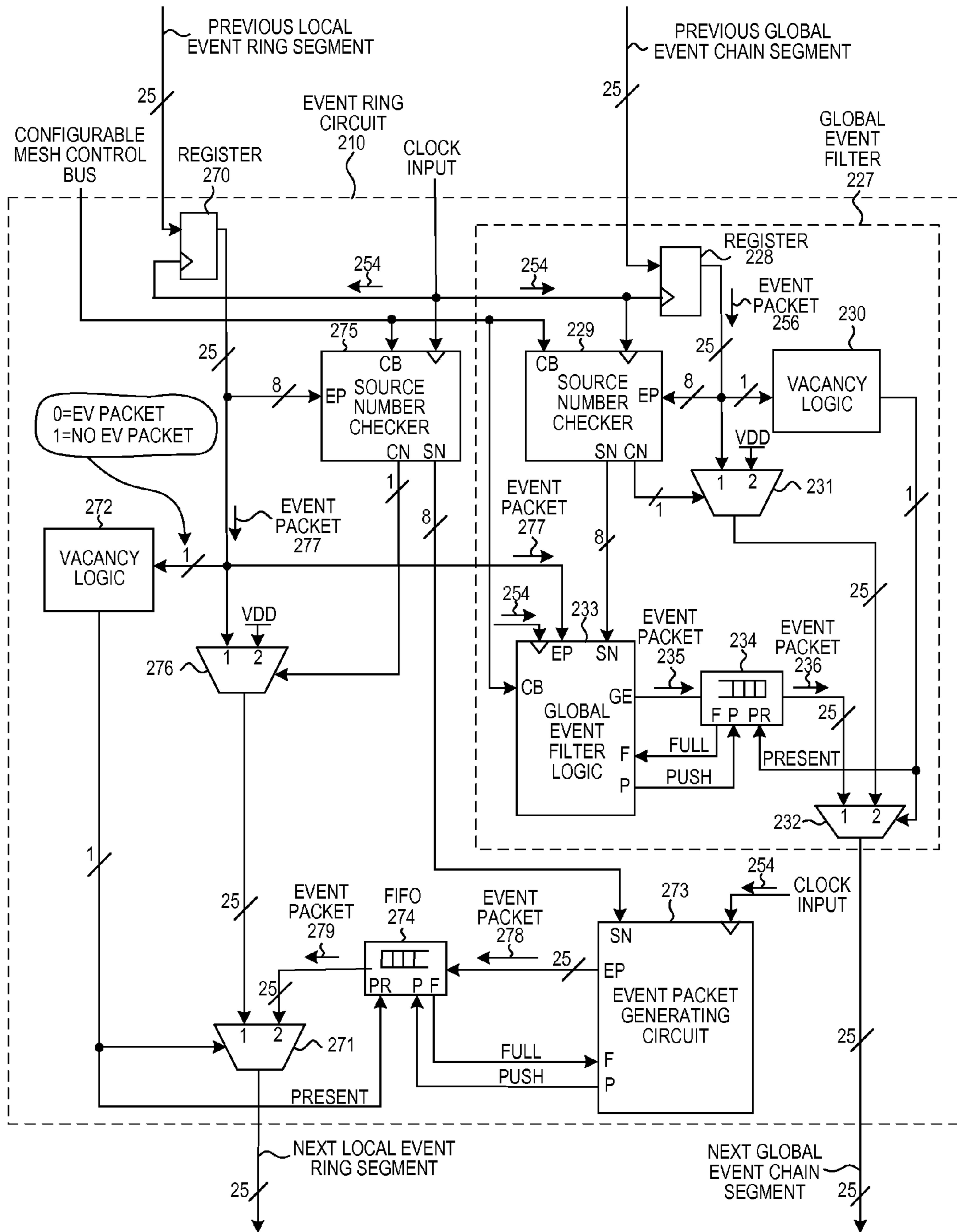
EVENT RING CIRCUIT WITH GLOBAL EVENT FILTER
