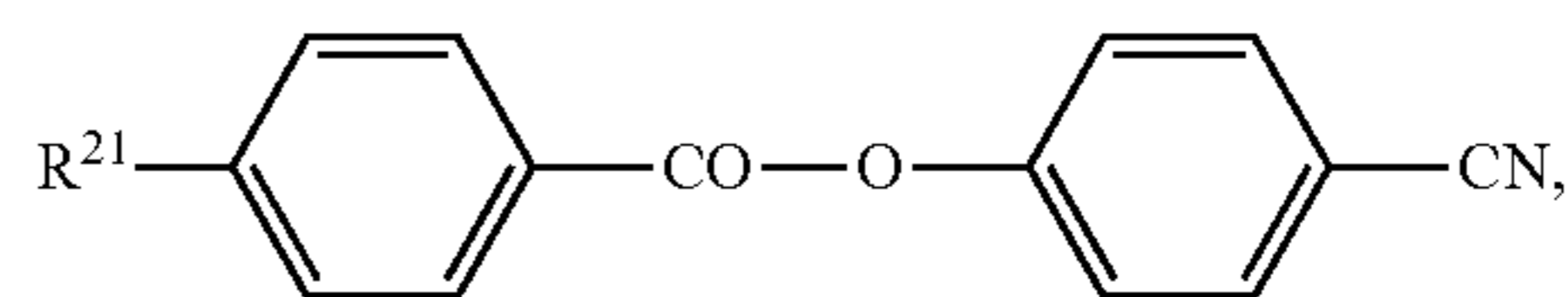
formula (II-4a-4)
