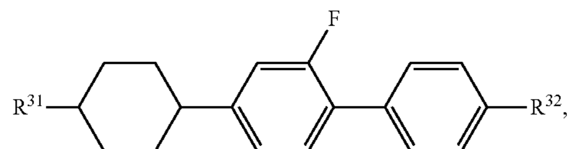
formula (III-1b-5)
