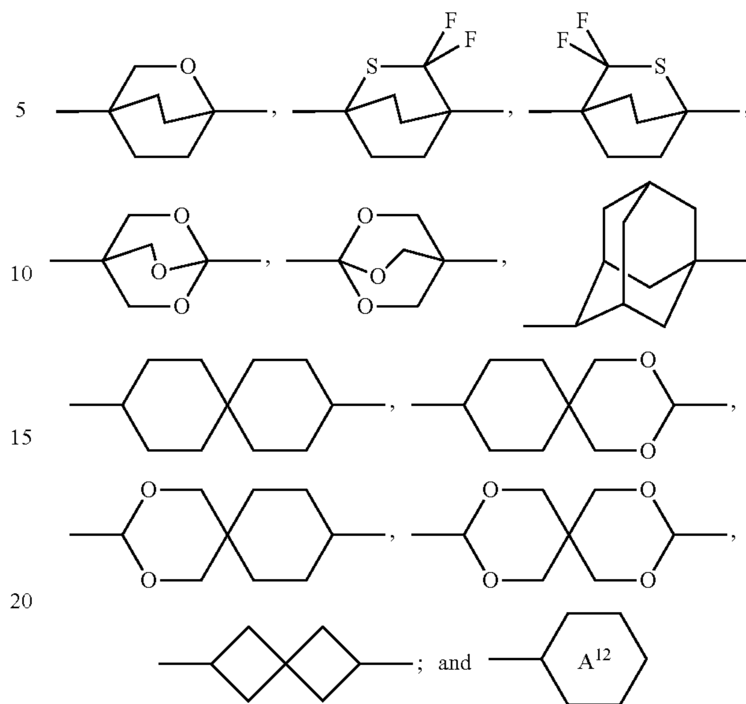
formula (I)
