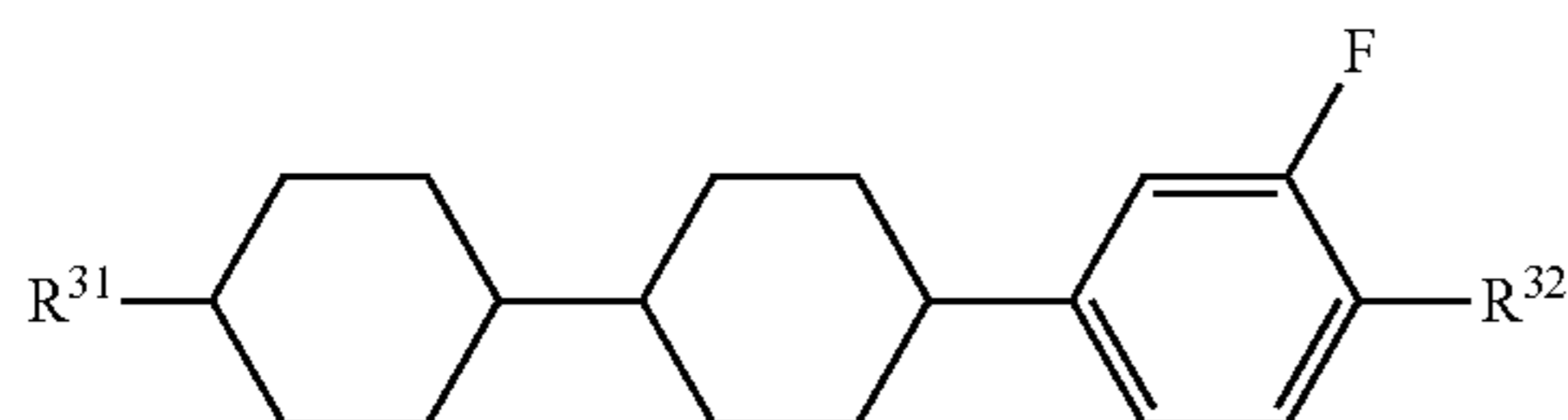
formula (III-1a-3)
