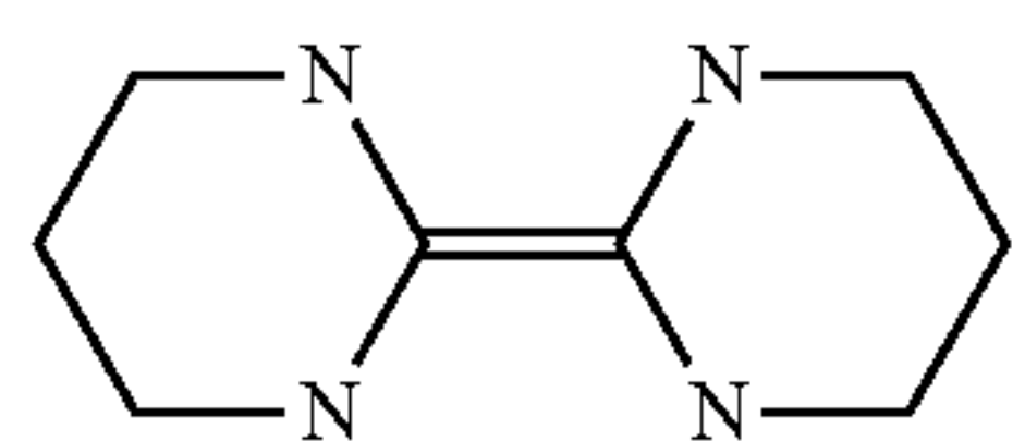
2-hexahydropyrimidin-2-ylidenehexahydropyrimidine
