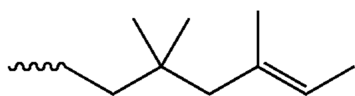
1,2,2 trisubstituted cis isomer beta
