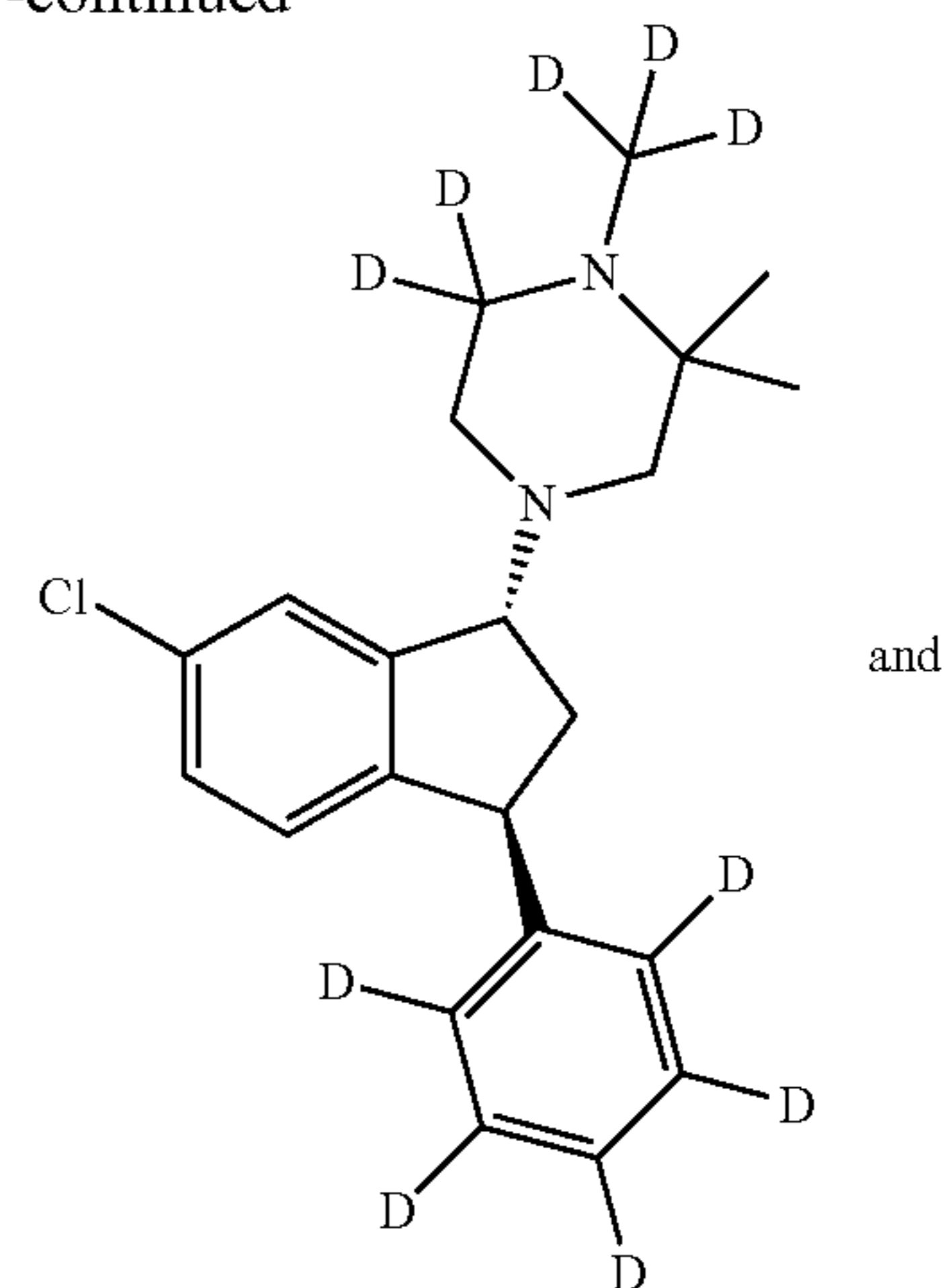
Compound (VI)
