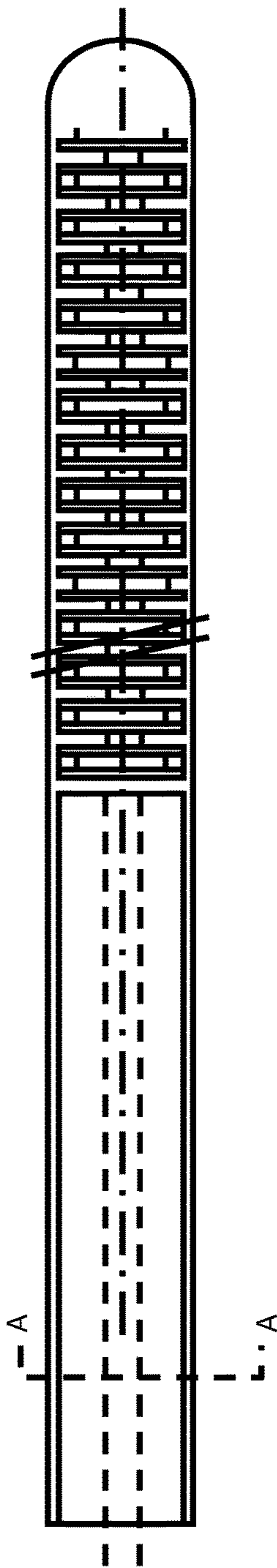
HOLLOW TUBE GUIDEWIRE WITH CORE WIRE AND INTERSPERSED ELASTOMER FILLING AND HYPOTUBE PROXIMAL.
