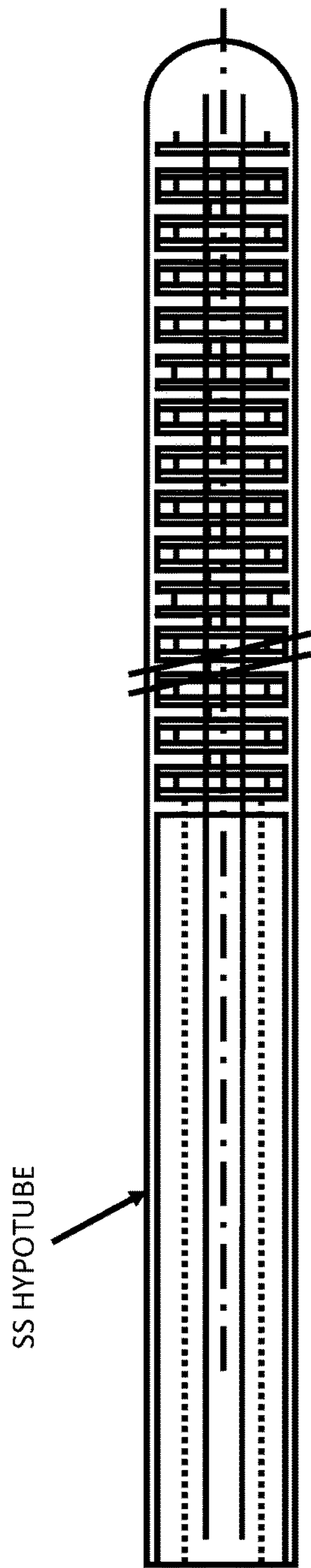
HOLLOW TUBE GUIDEWIRE WITH CORE WIRE AND INTERSPERSED ELASTOMER FILLING AND HYPOTUBE PROXIMAL.
