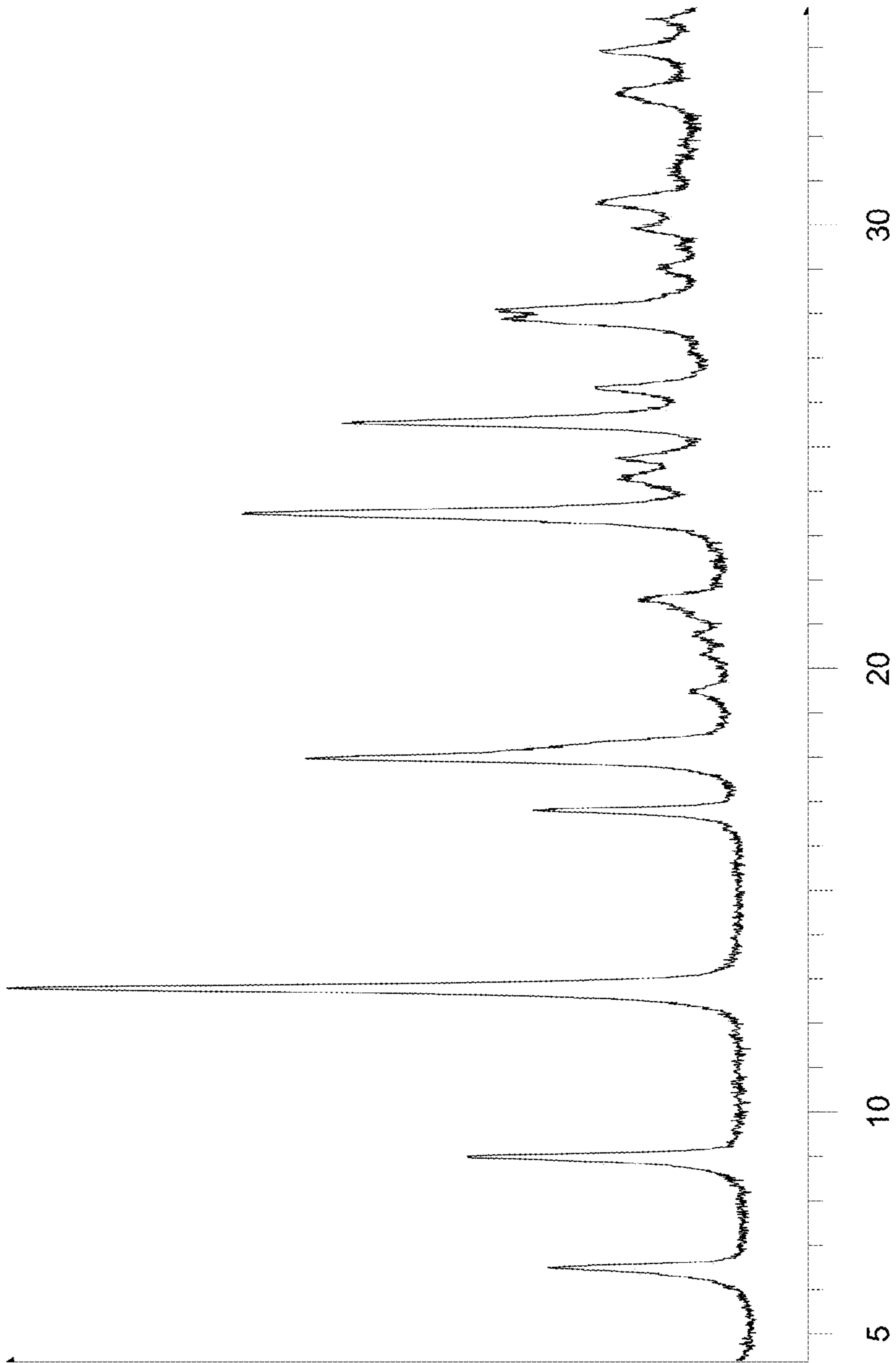
2-Theta - Scale
