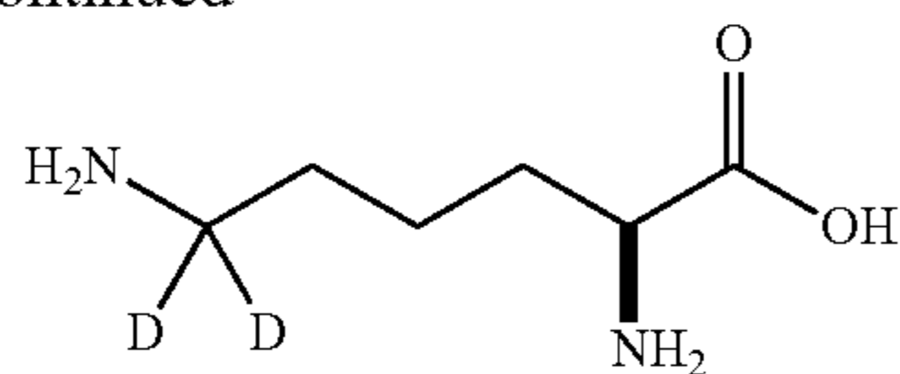
(S)-2,6-diaminohexanoic acid-6,6-D 2
