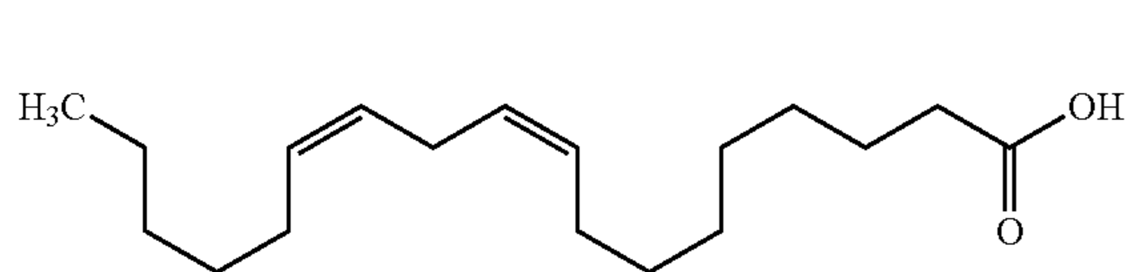
Linoleic Acid (18:2)
