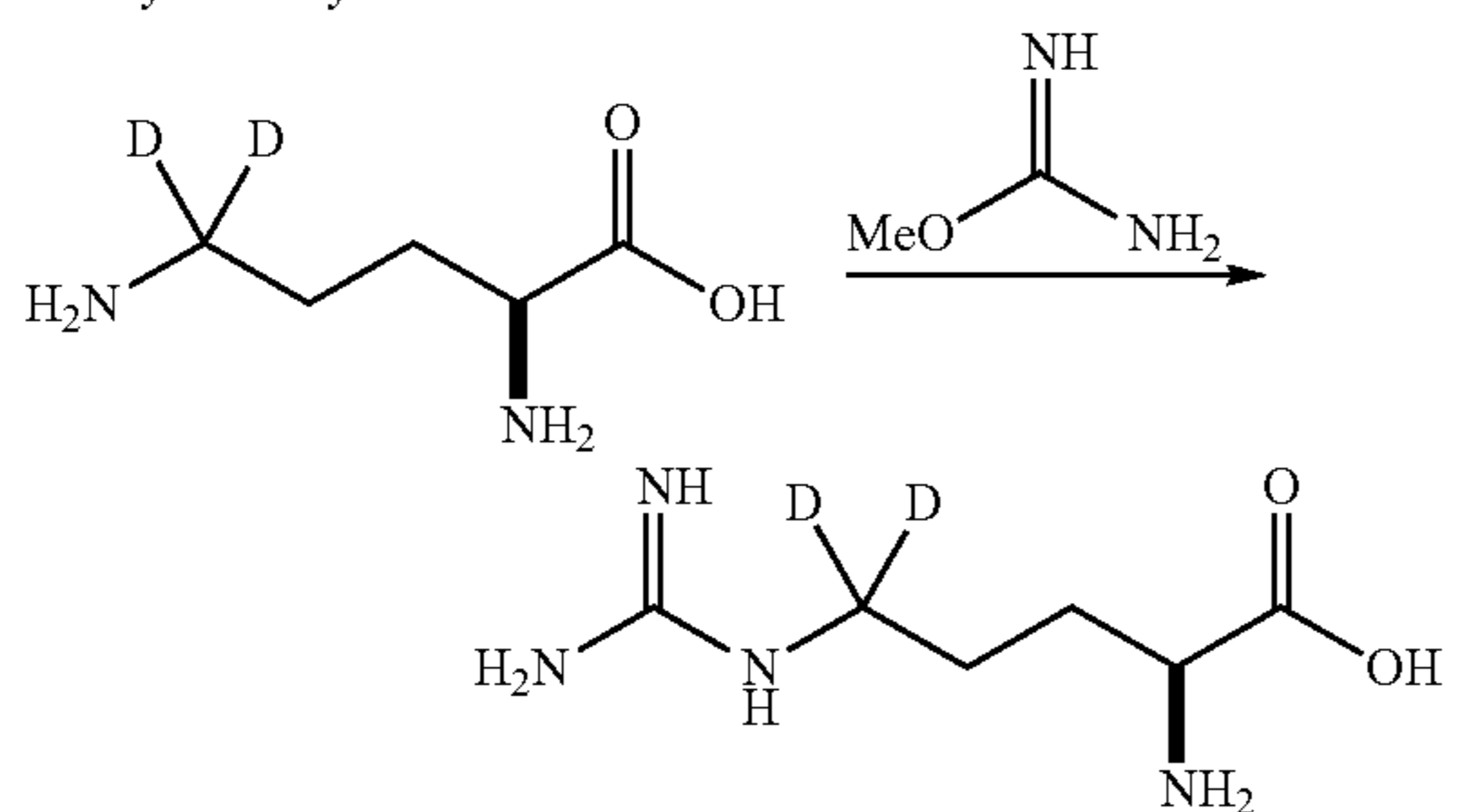
(S)-2-amino-5-guanidinopentanoic acid-5,5-D 2
