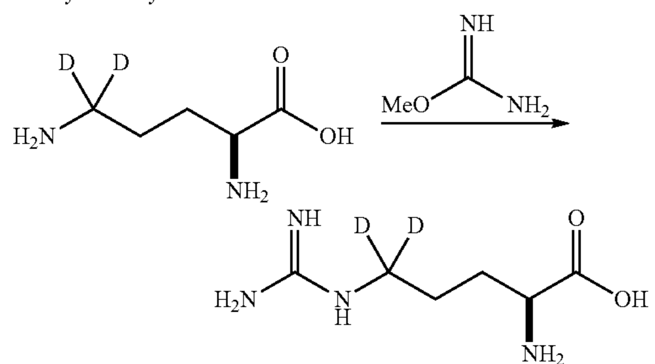
(S)-2-amino-5-guanidinopentanoic acid-5,5-D 2
