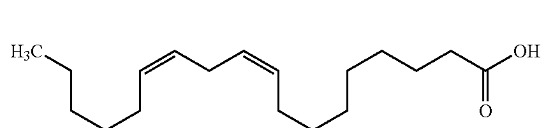
Linoleic Acid (18:2)
