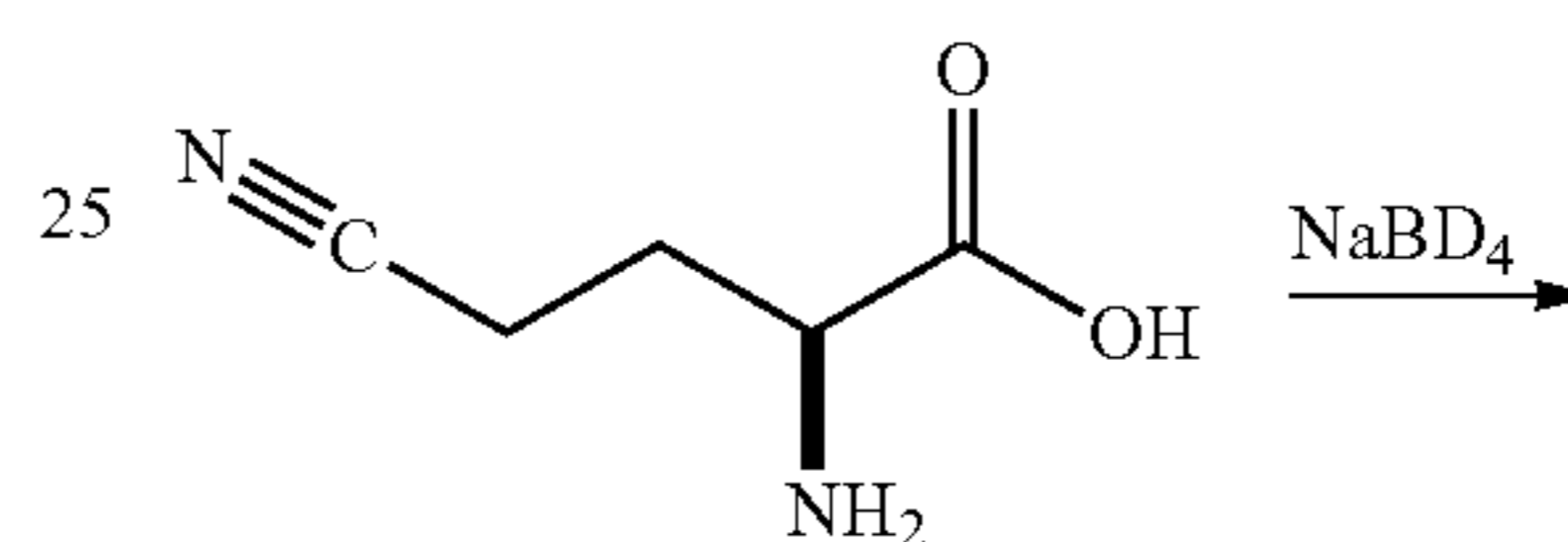
(S)-2-Amino-4-cyano-butyrac acid
