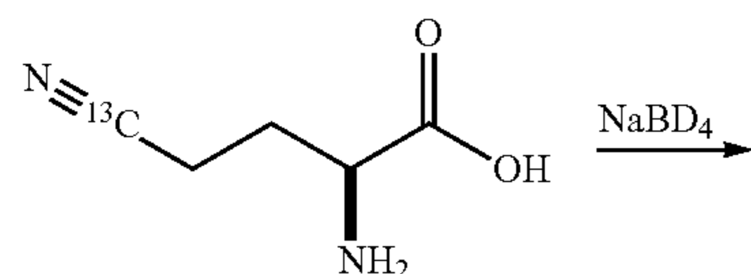
(S)-2-Amino-4-cyano( 13 C)-butyric acid
