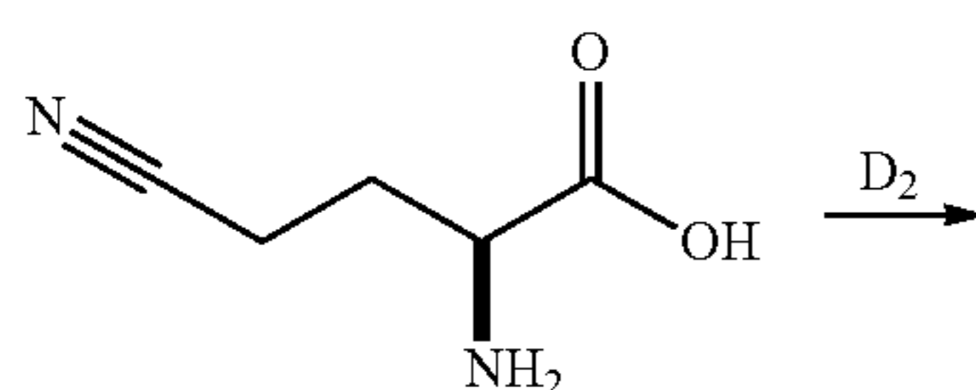
2-Amino-4-cyano-butanoic acid
