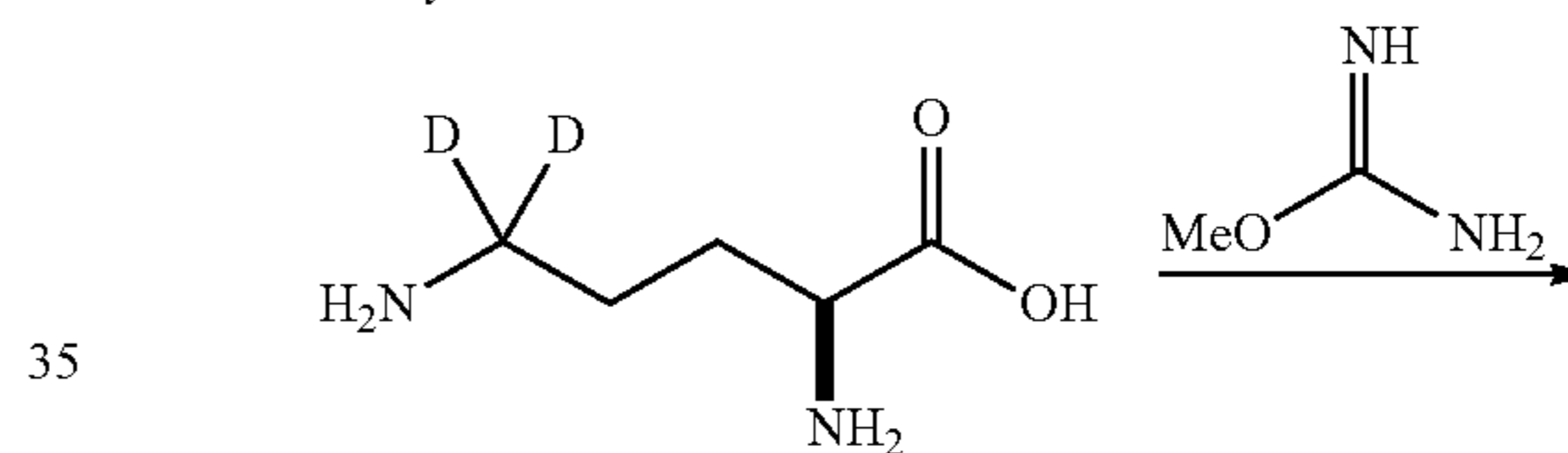
(S)-2-Amino-4-cyano-butyrinic acid
