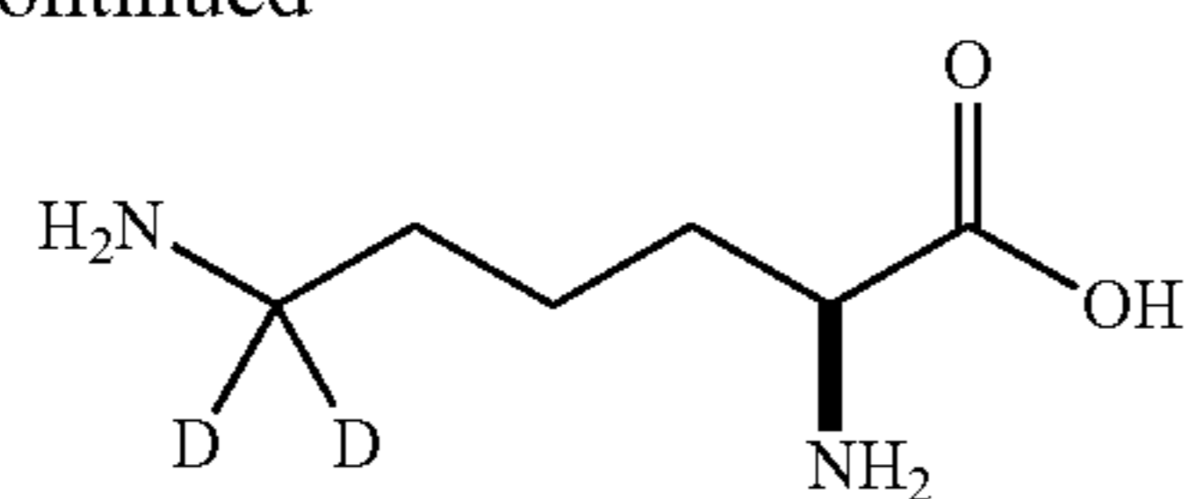
(S)-2,6-diaminohexanoic acid-6,6-D 2
