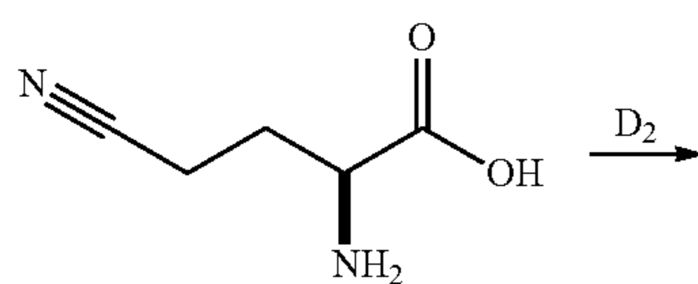
2-Amino-4-cyano-butanoic acid
