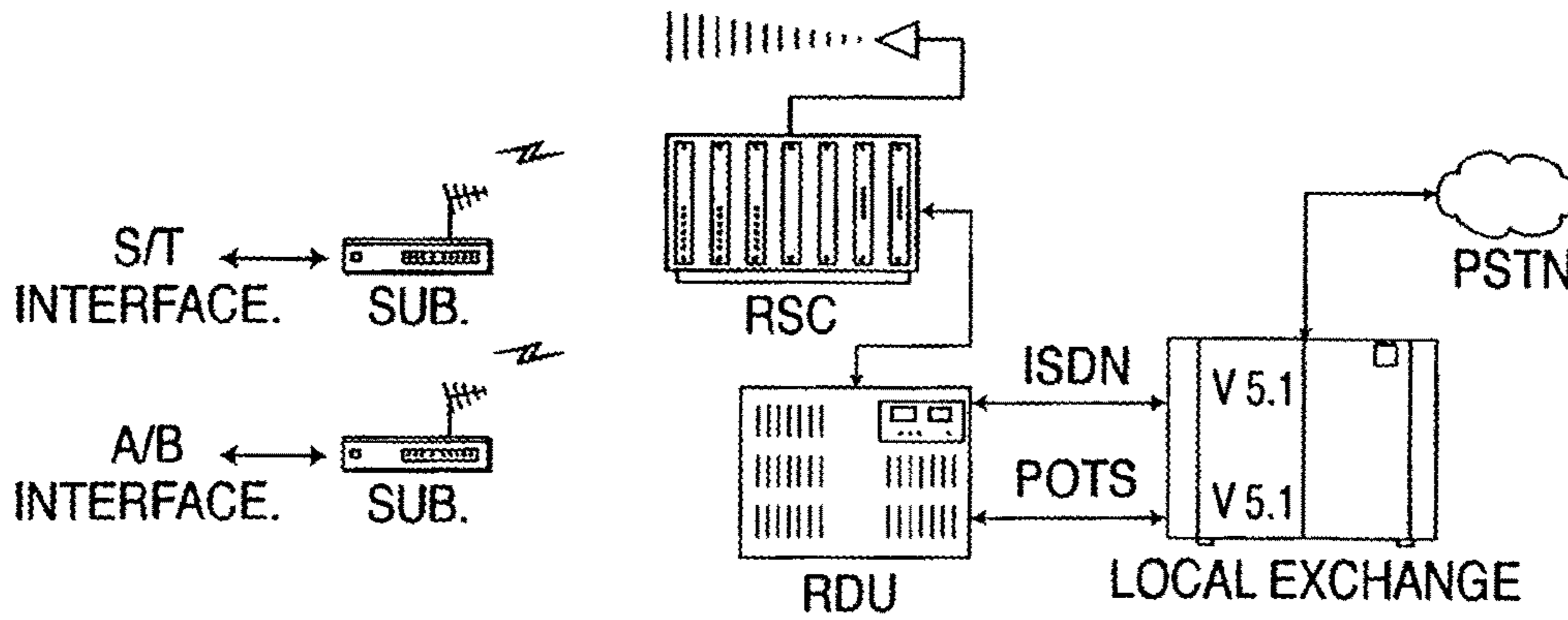
ISDN AND POTS NETWORK INTERFACE FIG. 2F
