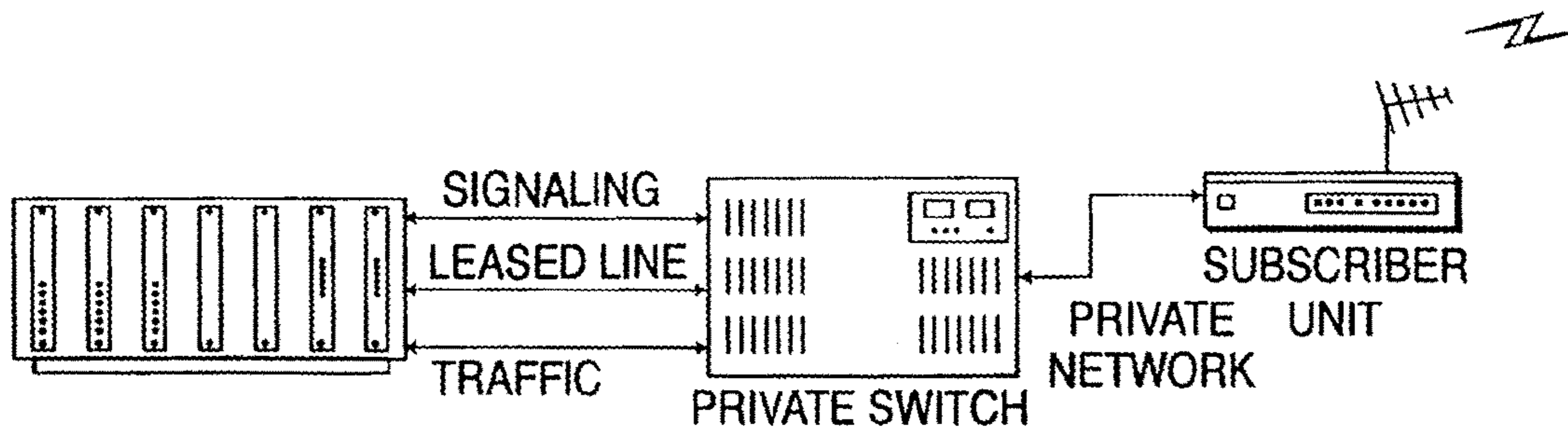
WIDEBAND AND PACKET NETWORK INTERFACE FIG. 2G
