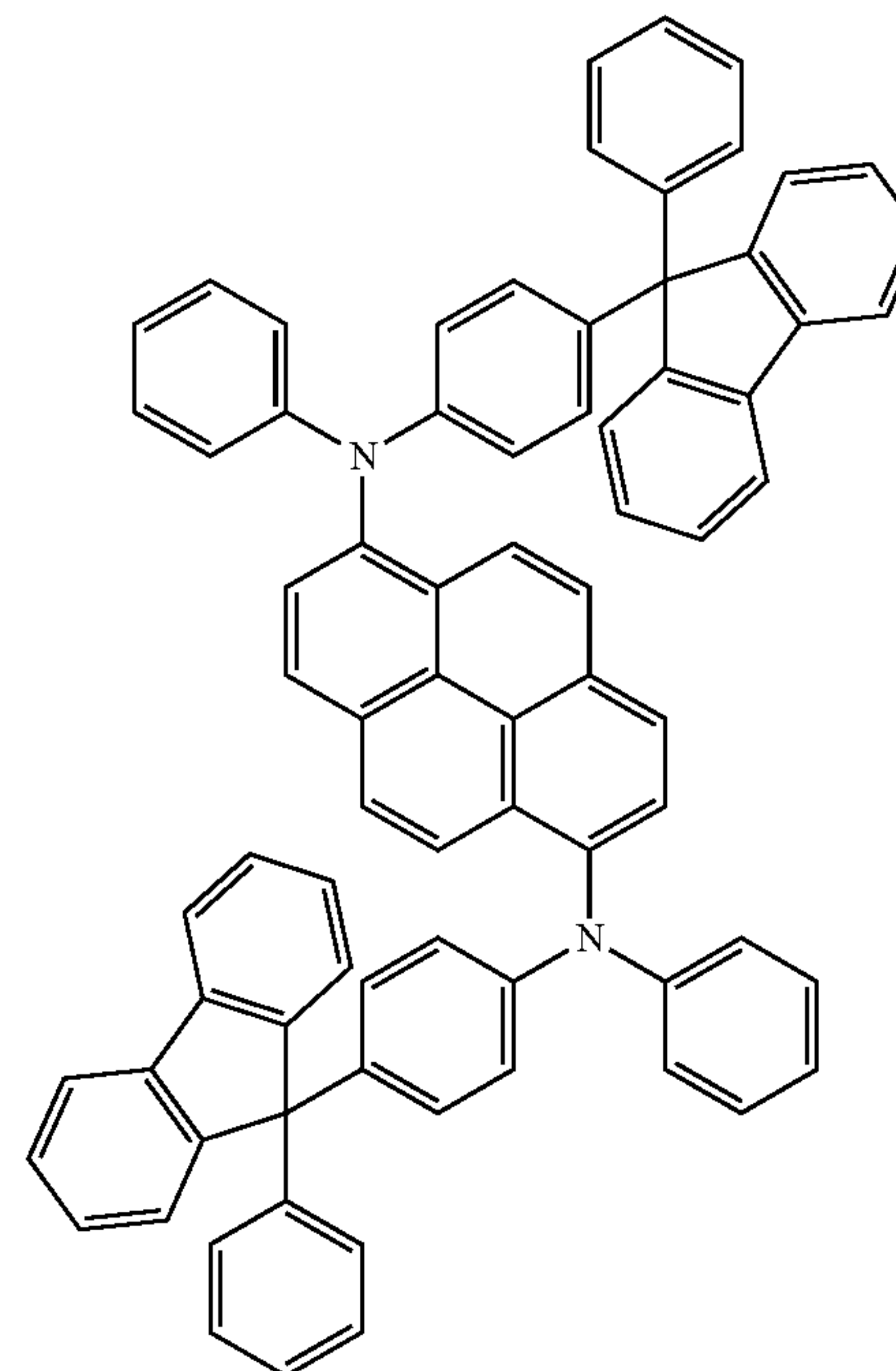
1,6FLPAPm
