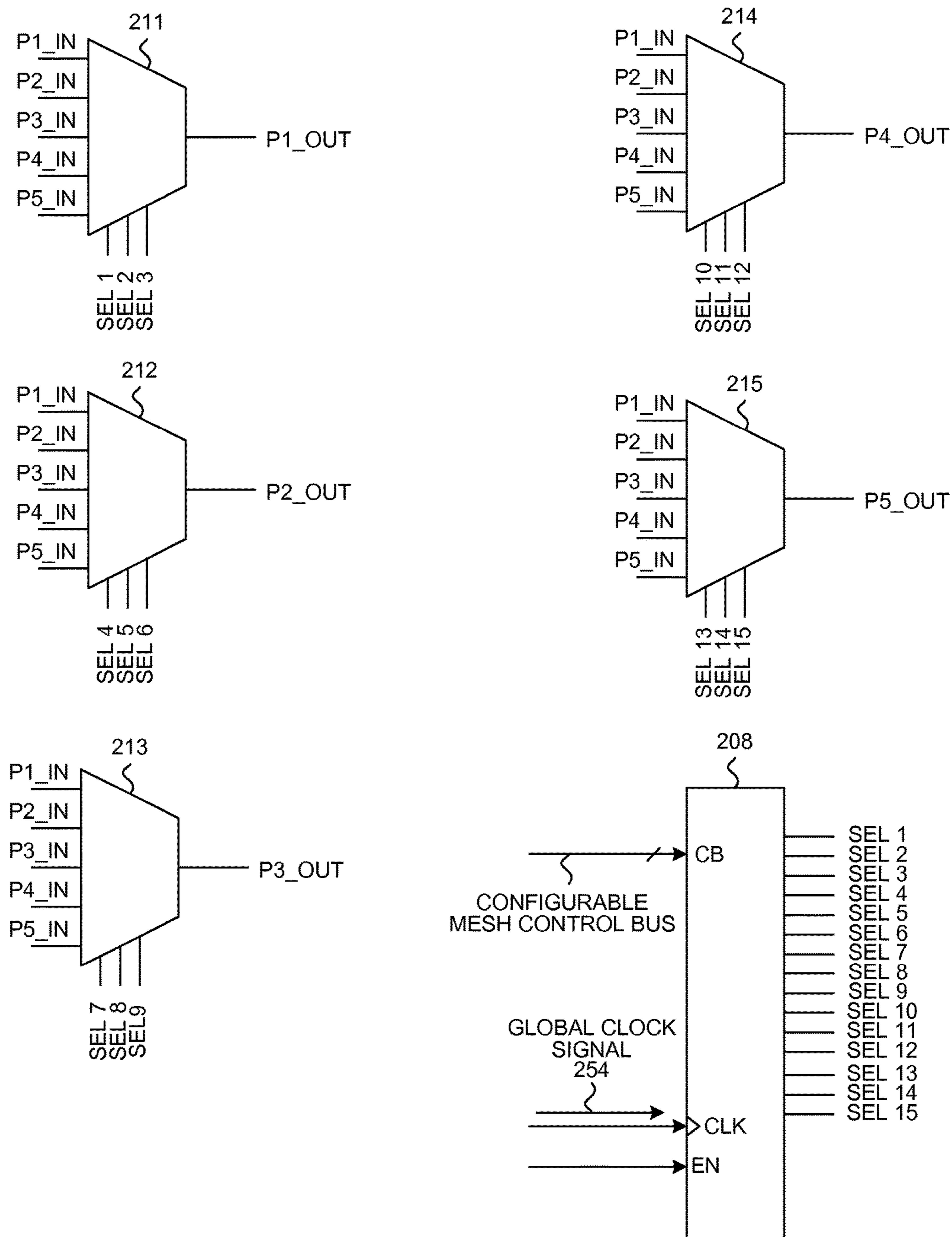
RUN TIME CONFIGURABLE SWITCH CIRCUIT
