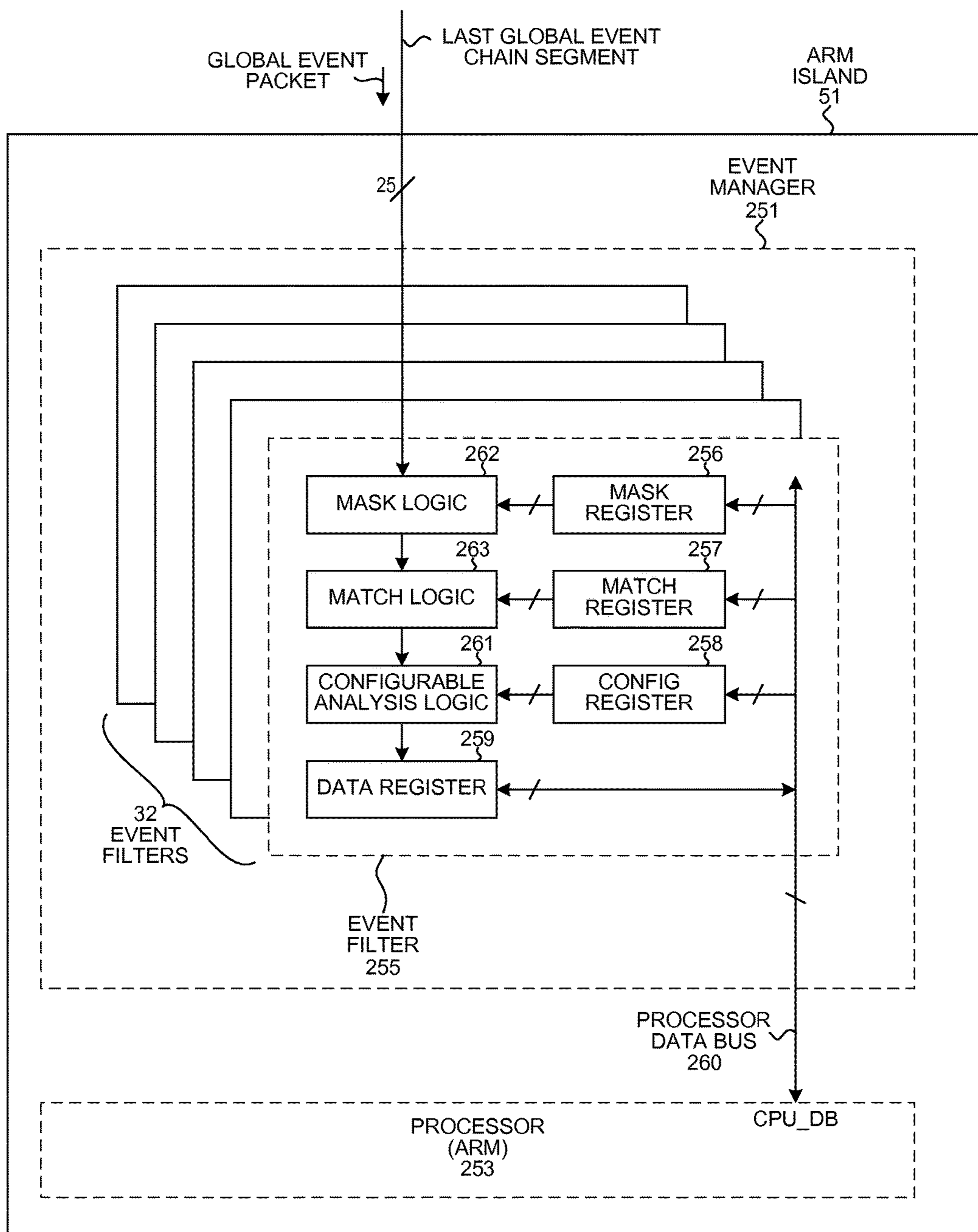
EVENT MANAGER
