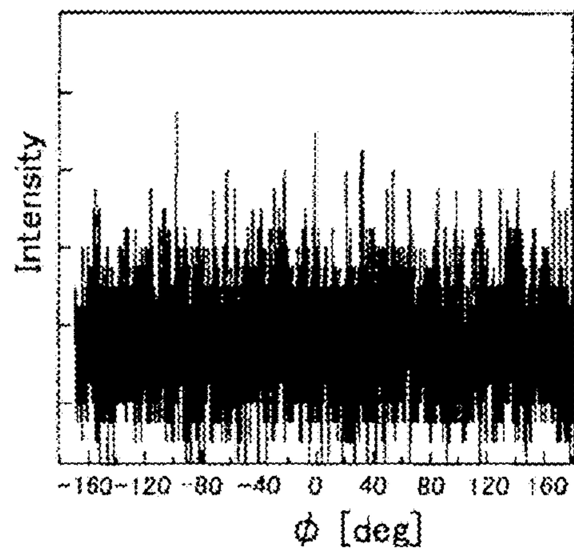
FIG. 28B in-plane method \phi scan CAAC-OS
