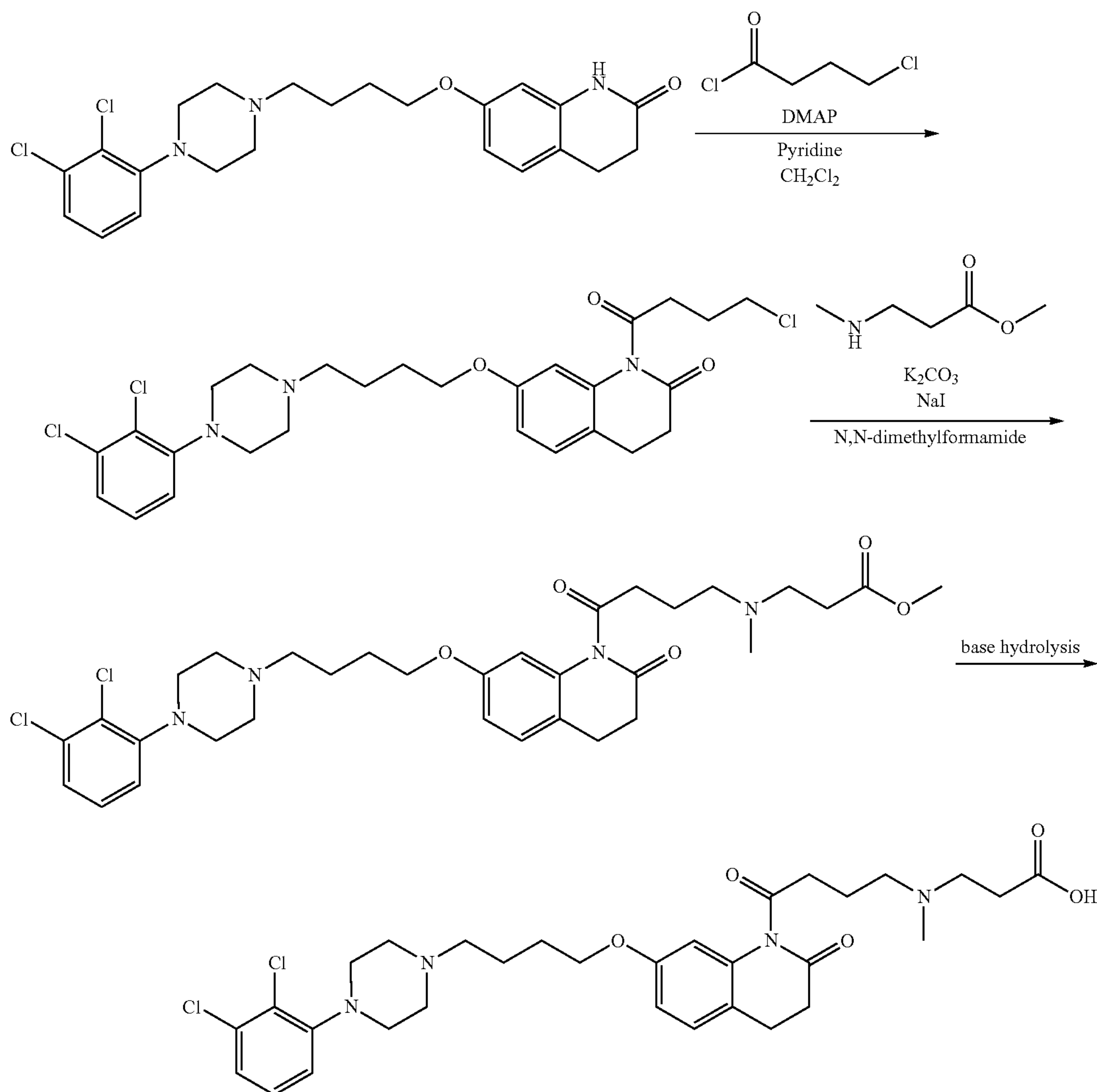
Scheme 6:
