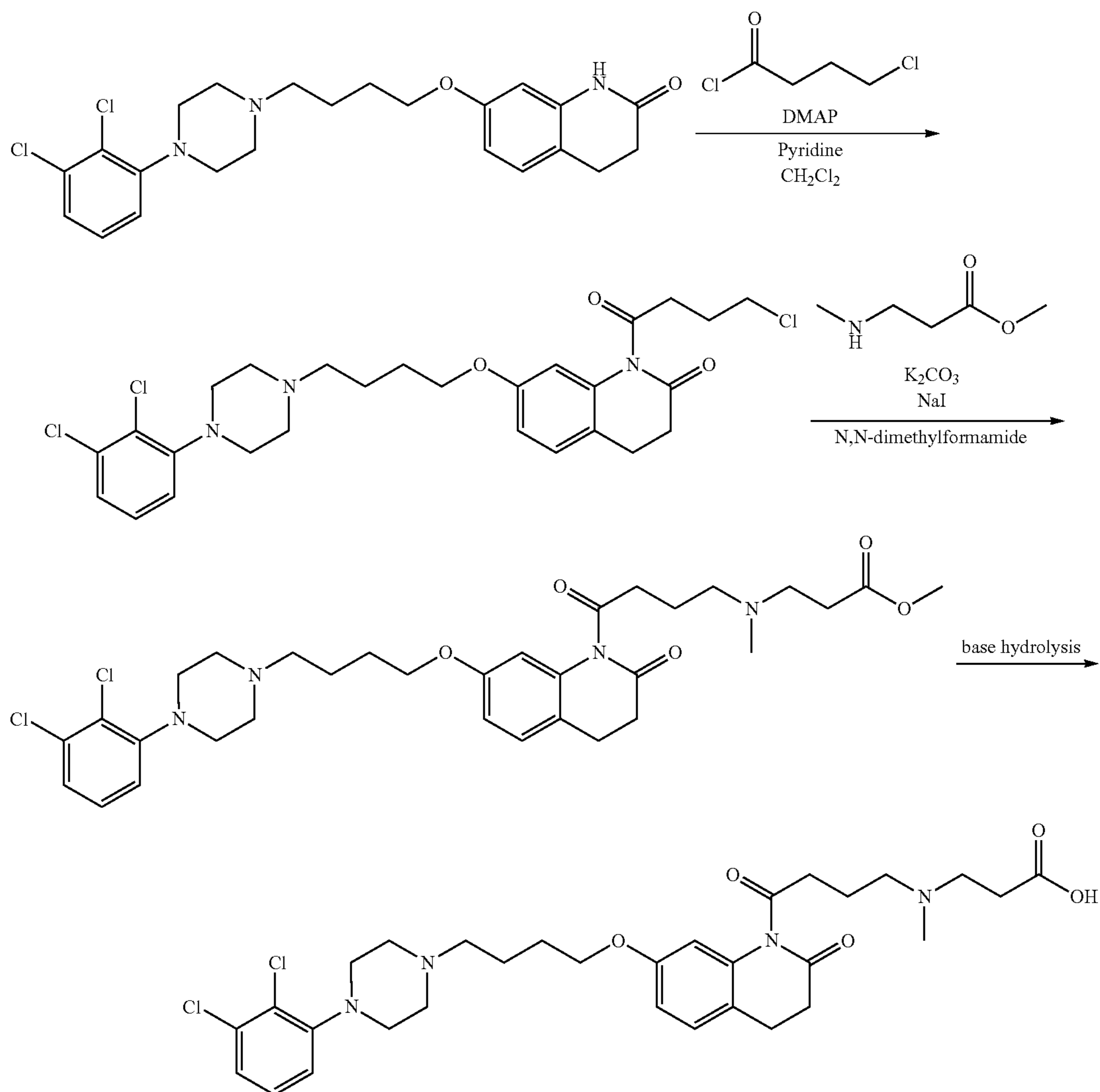
Scheme 6:
