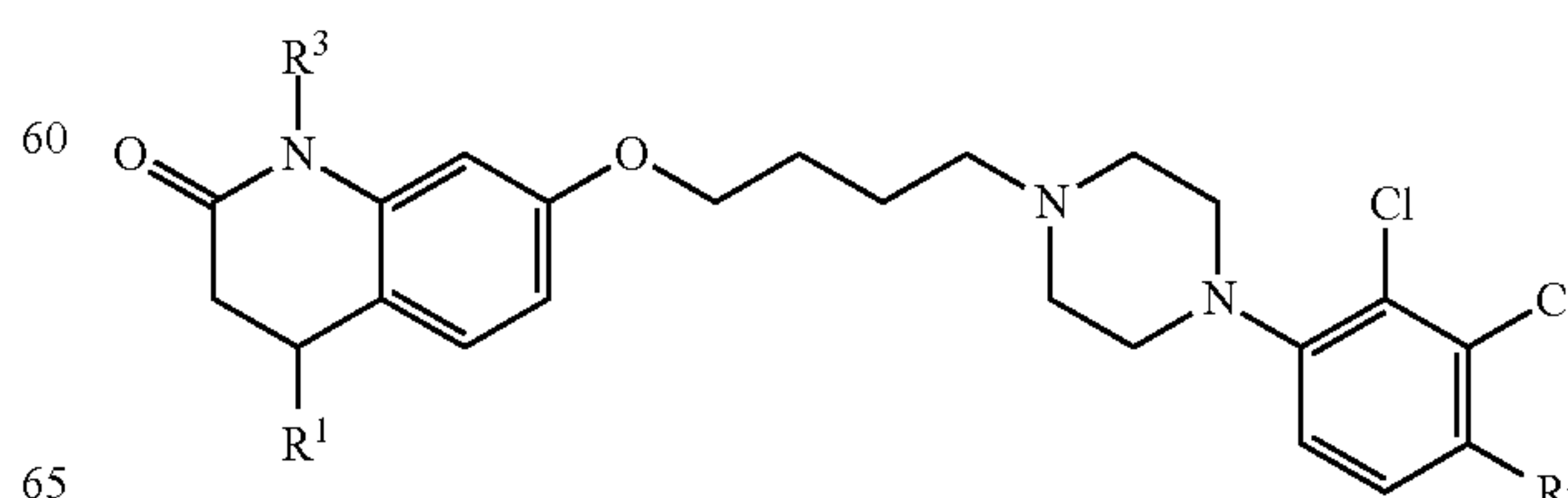
Formula I
