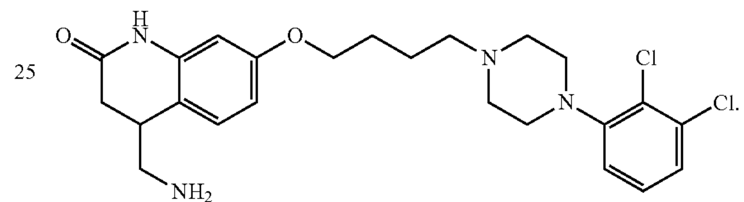
Formula III
