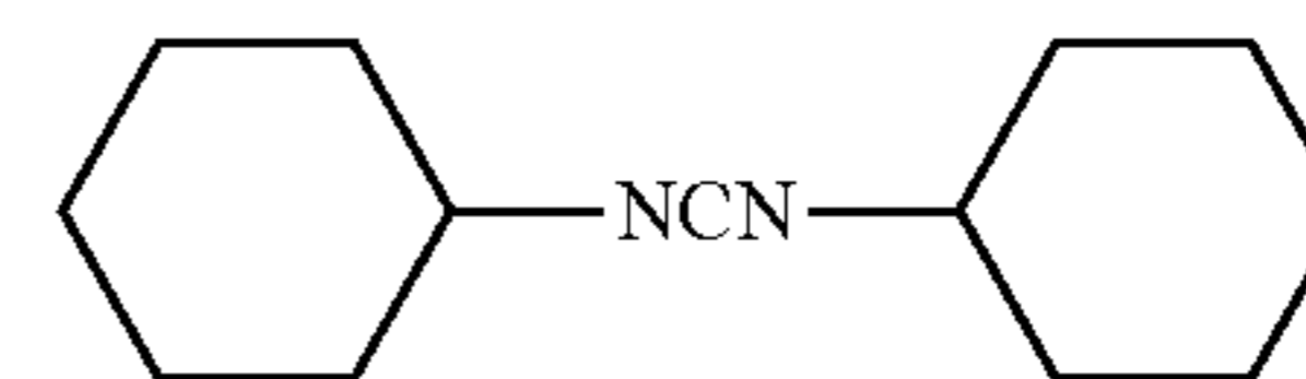
Dicyclohexylcarbodiimide (DCC)
