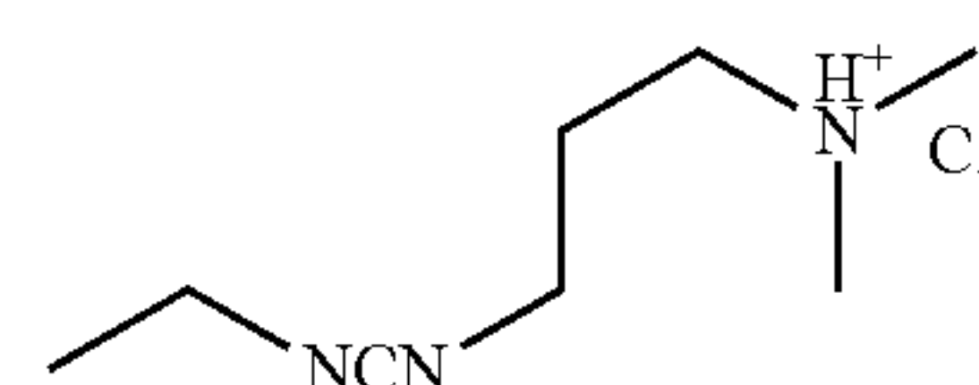
dimethylaminopropylcarbodiimide•HCl (EDC)
