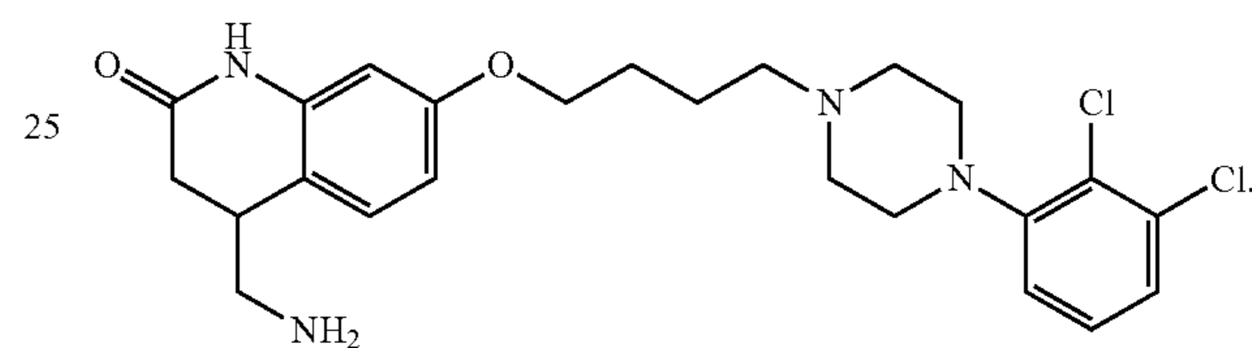
Formula III
