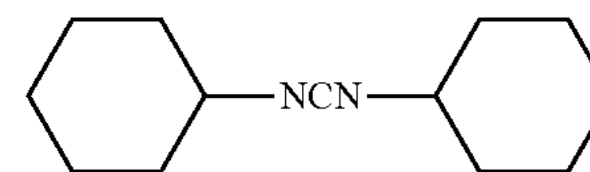
Dicyclohexylcarbodiimide (DCC)
