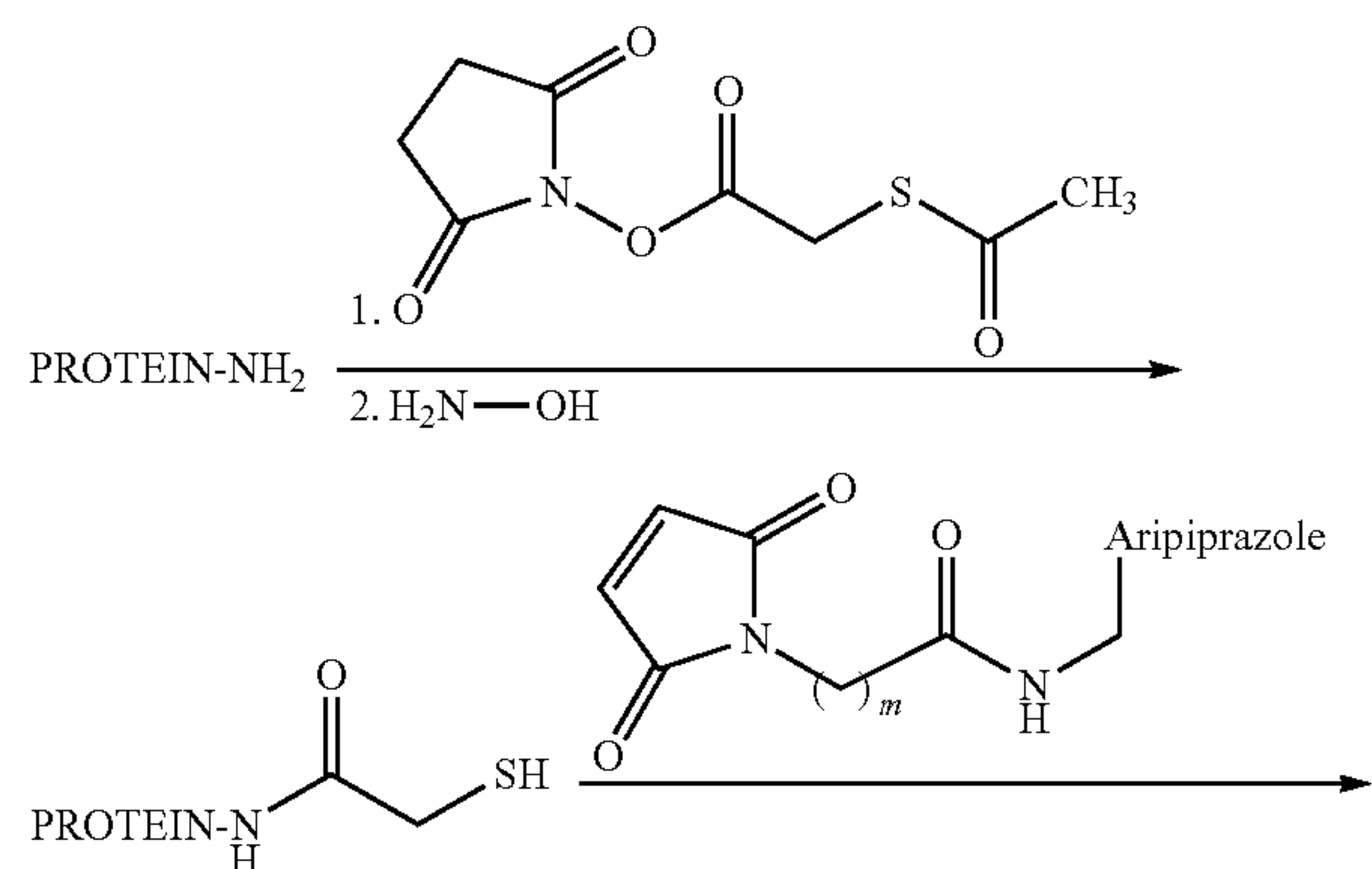
Scheme 8
