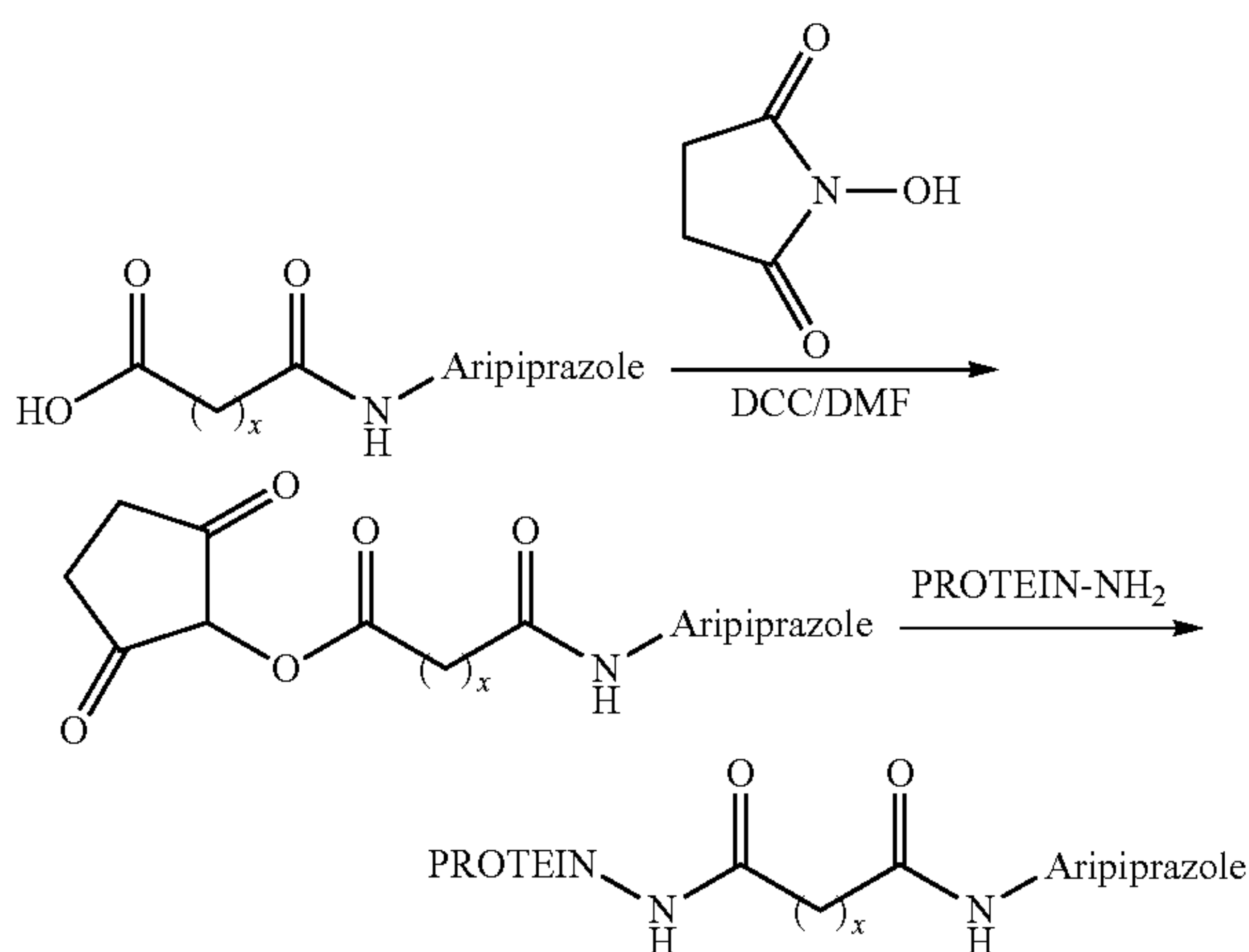
Scheme 9:
