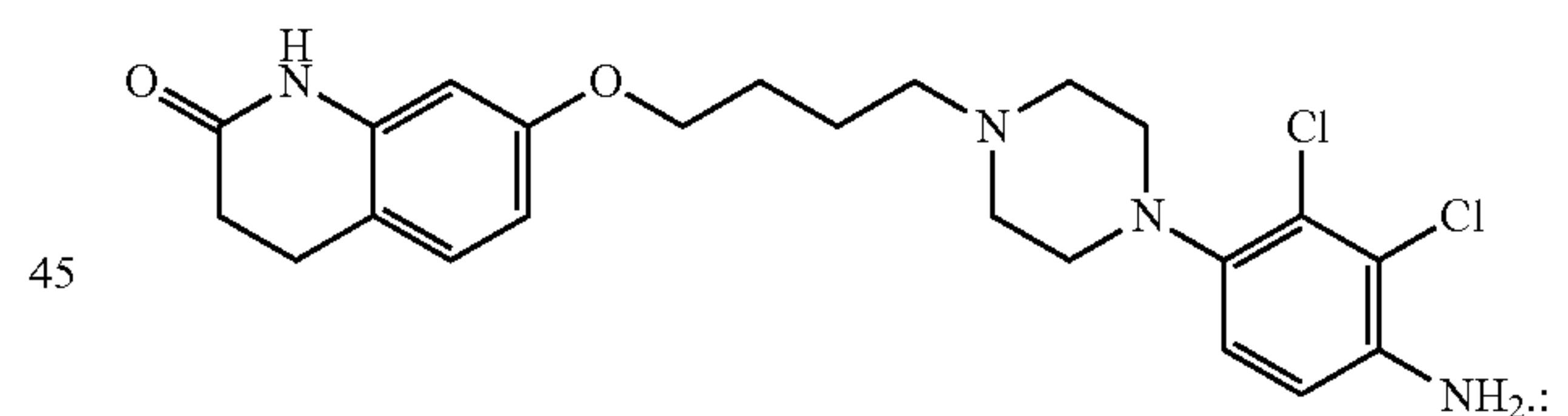
Formula IV
