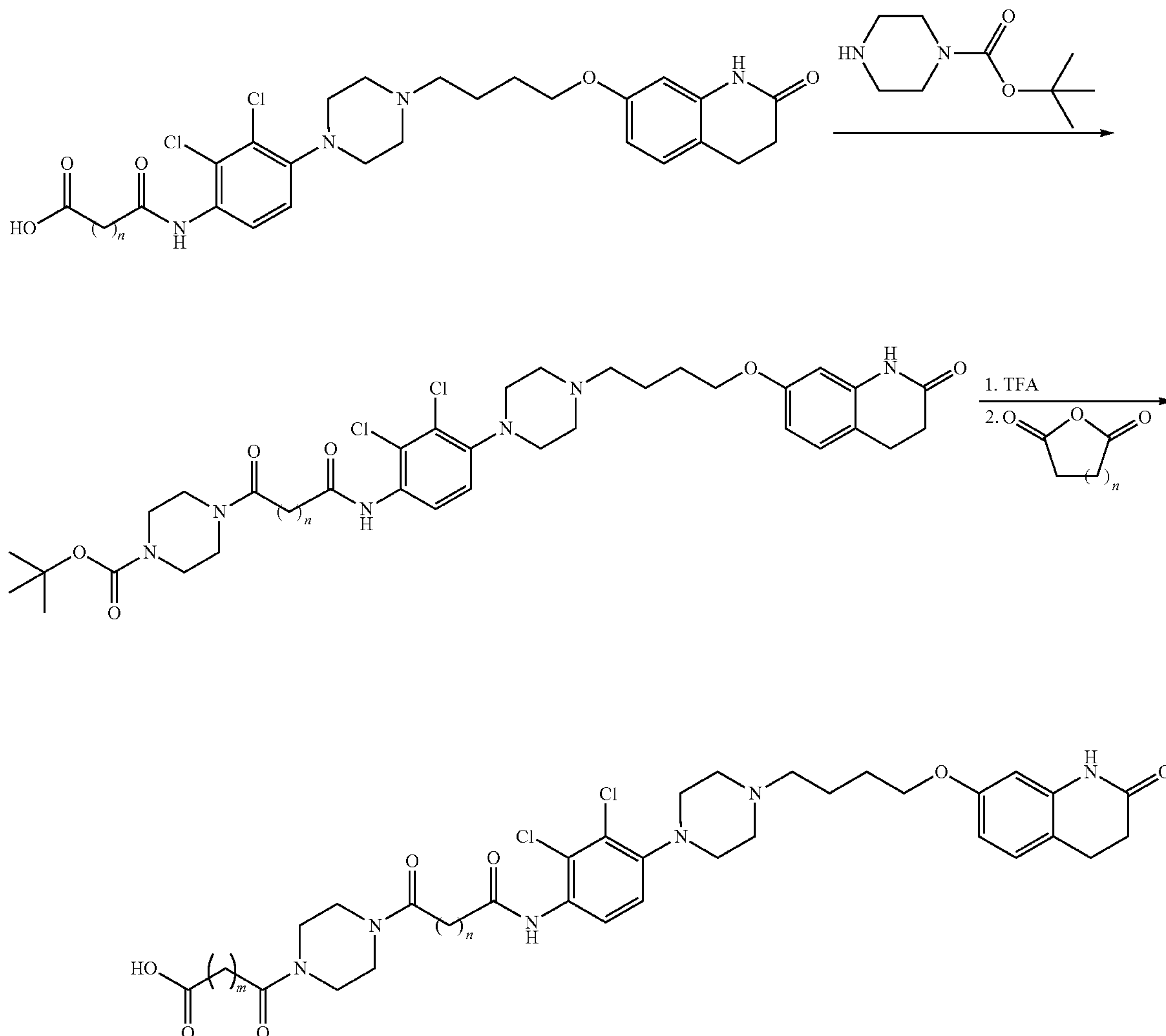
Scheme 5
