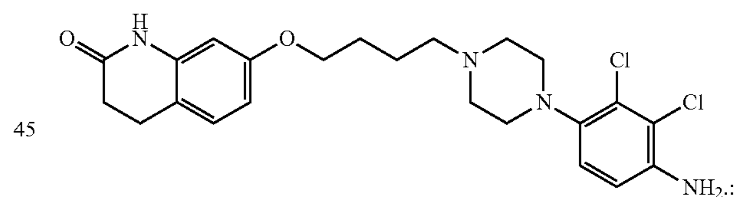
Formula IV
