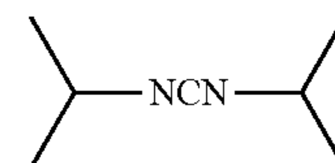
diisopropylcarbodiimide (DIC)
