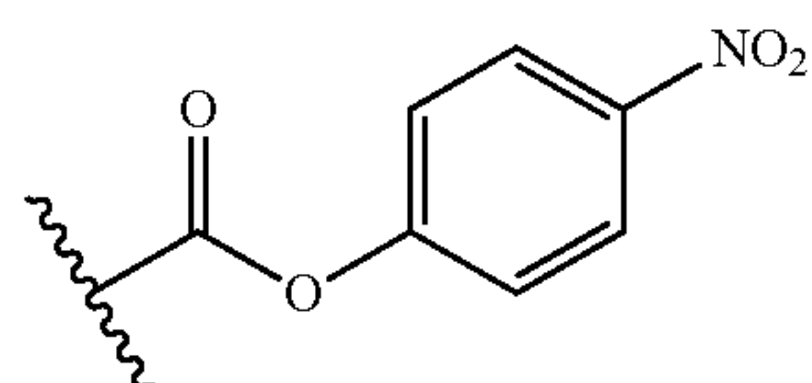
PNP
