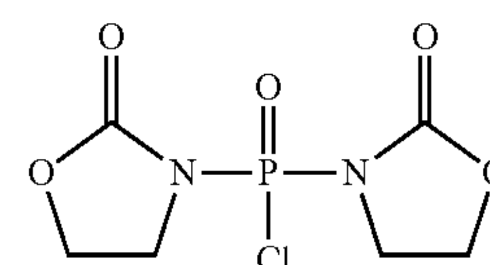
BOP-Cl
