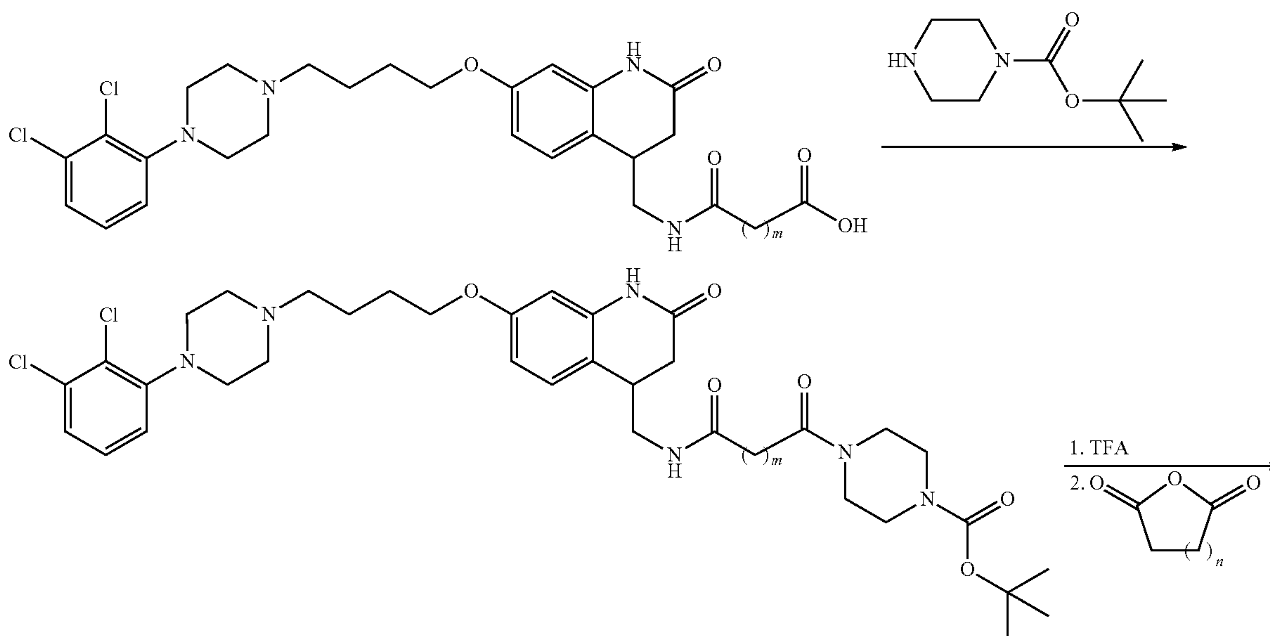
Scheme 4
