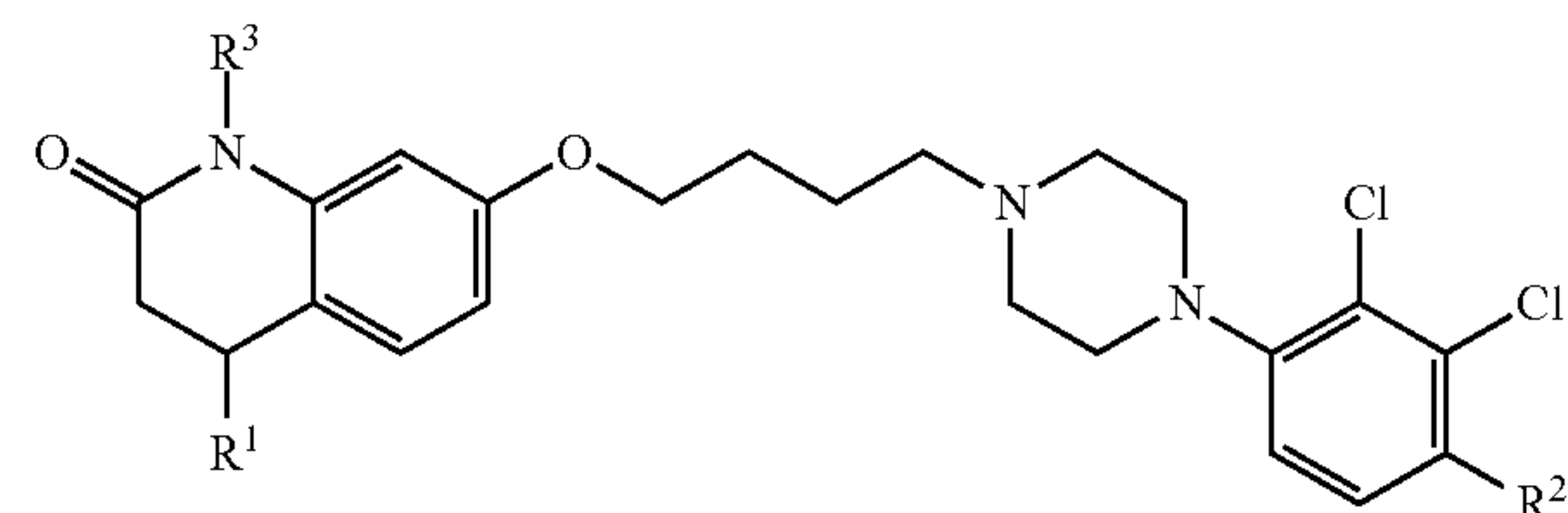
Formula I
