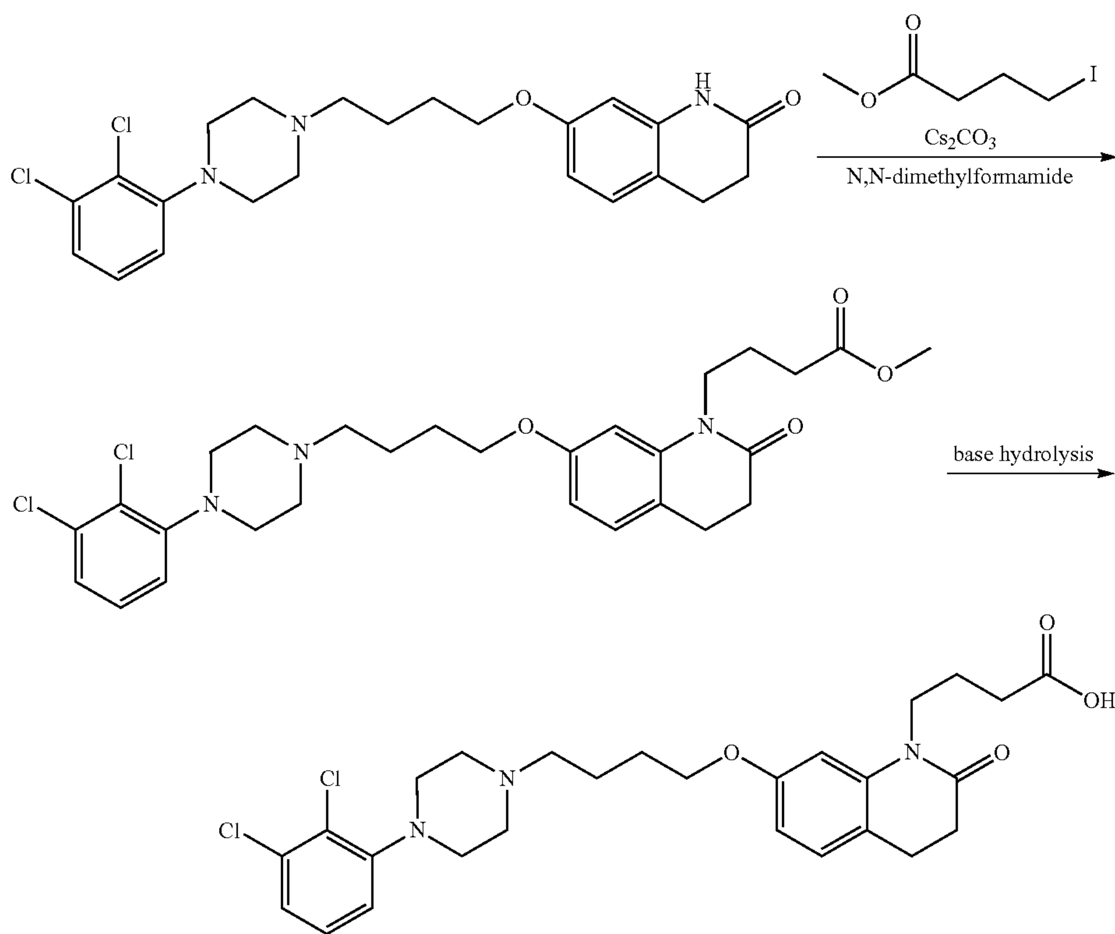
Scheme 7
