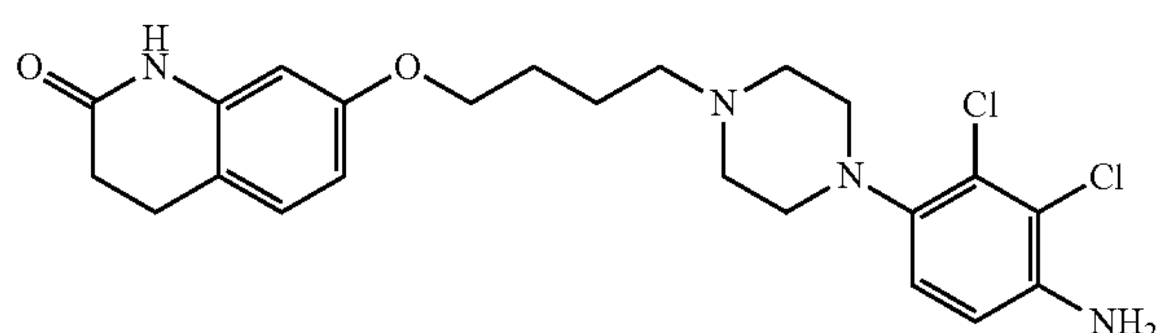
7-(4-(4-(4-amino-2,3-dichlorophenyl)piperazin-1-yl)butoxy)-3,4-dihydroquinolin-2(1H)-one
