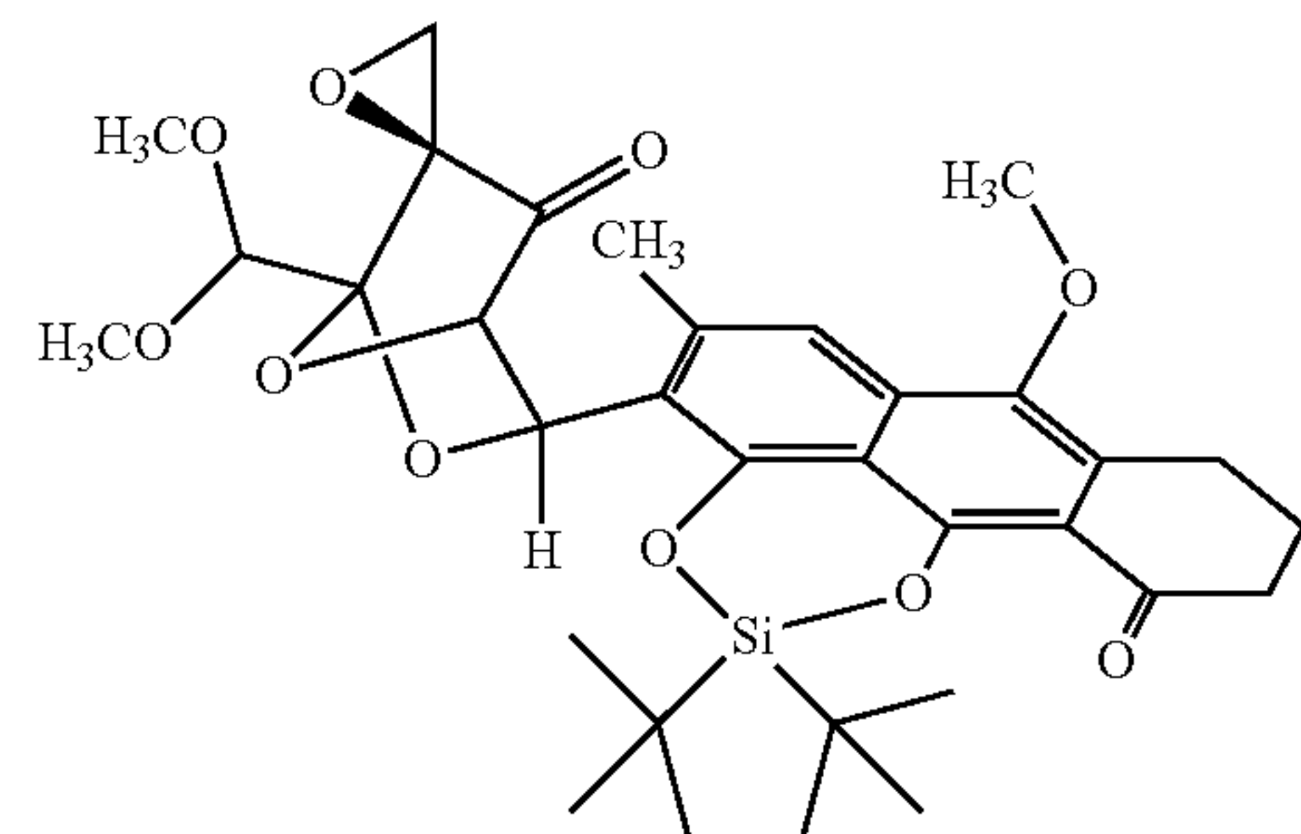
Dideoxy Endo cycloadduct 2
