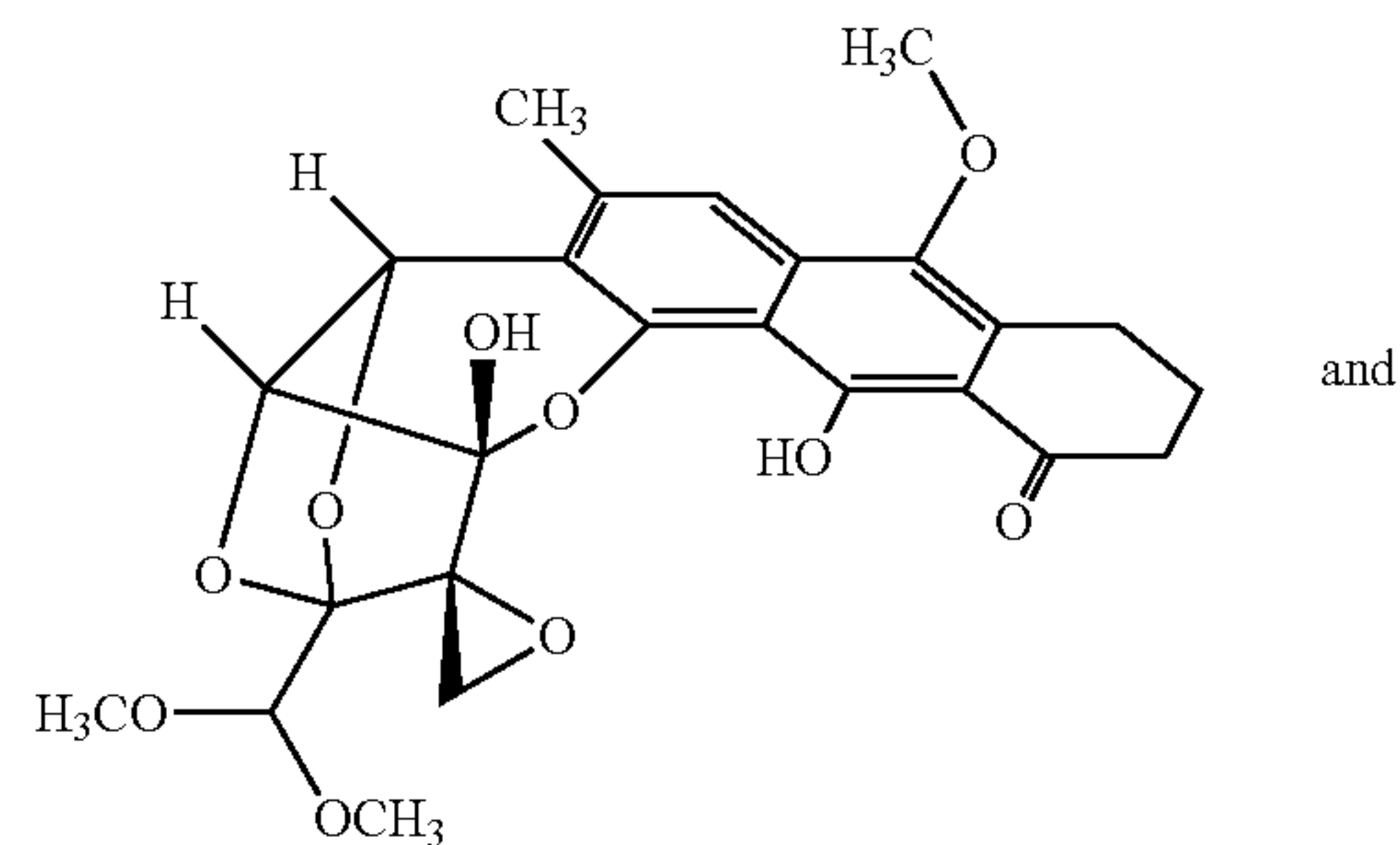
Dideoxy Endo 1 hemiketal "Iso-Dideoxy-DC-45-A2"
