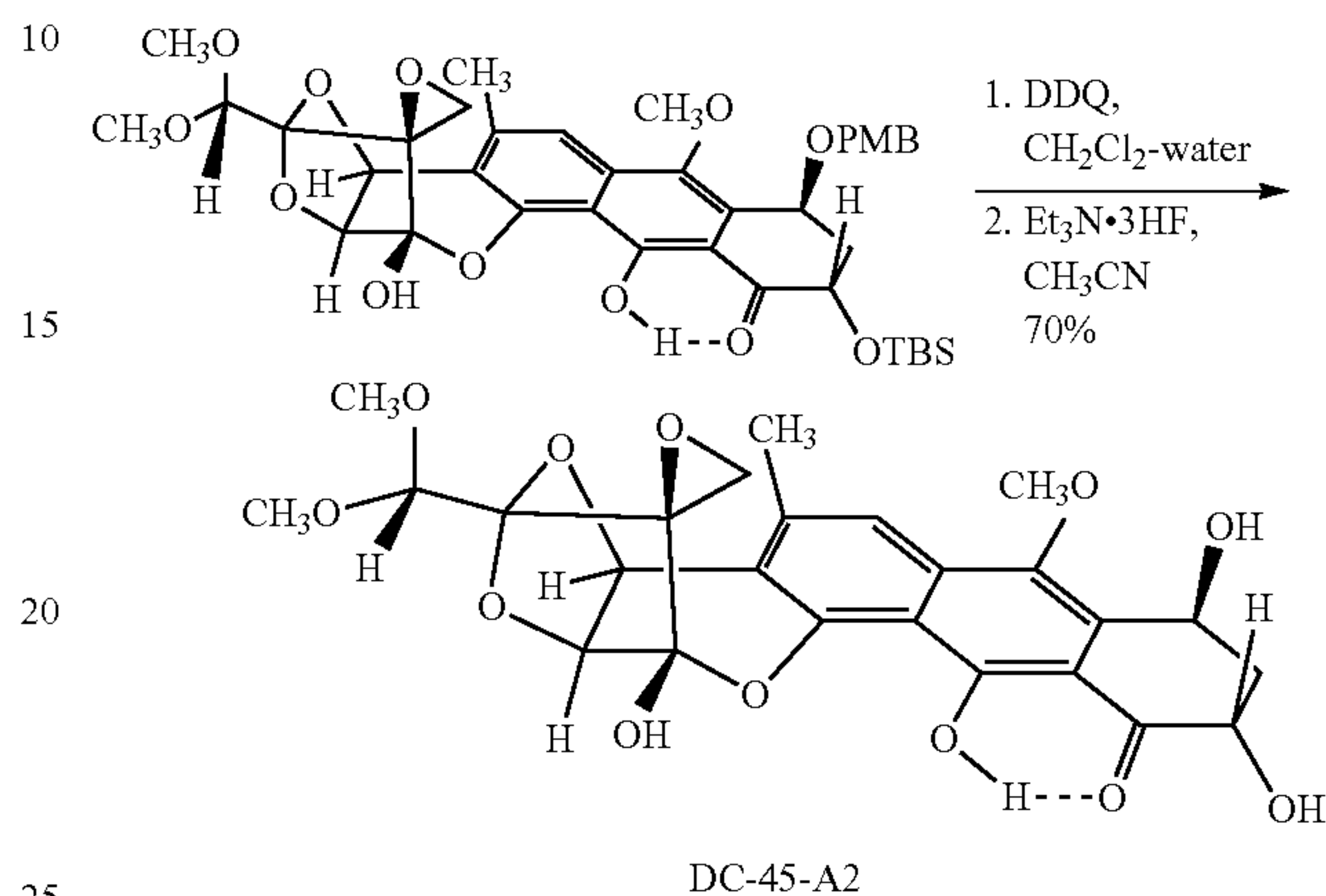
11,12,13,15-tetraepi-DC-45-A2 and chlorohydrin
