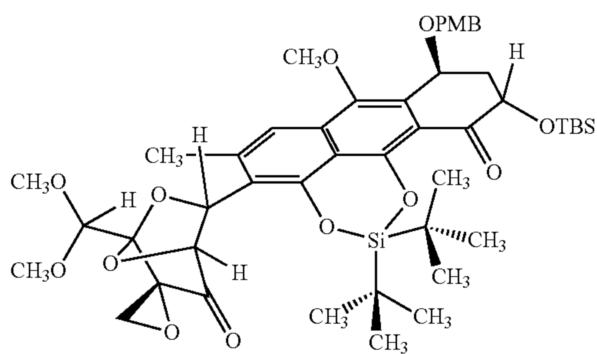
Endo Cycloadduct 1
