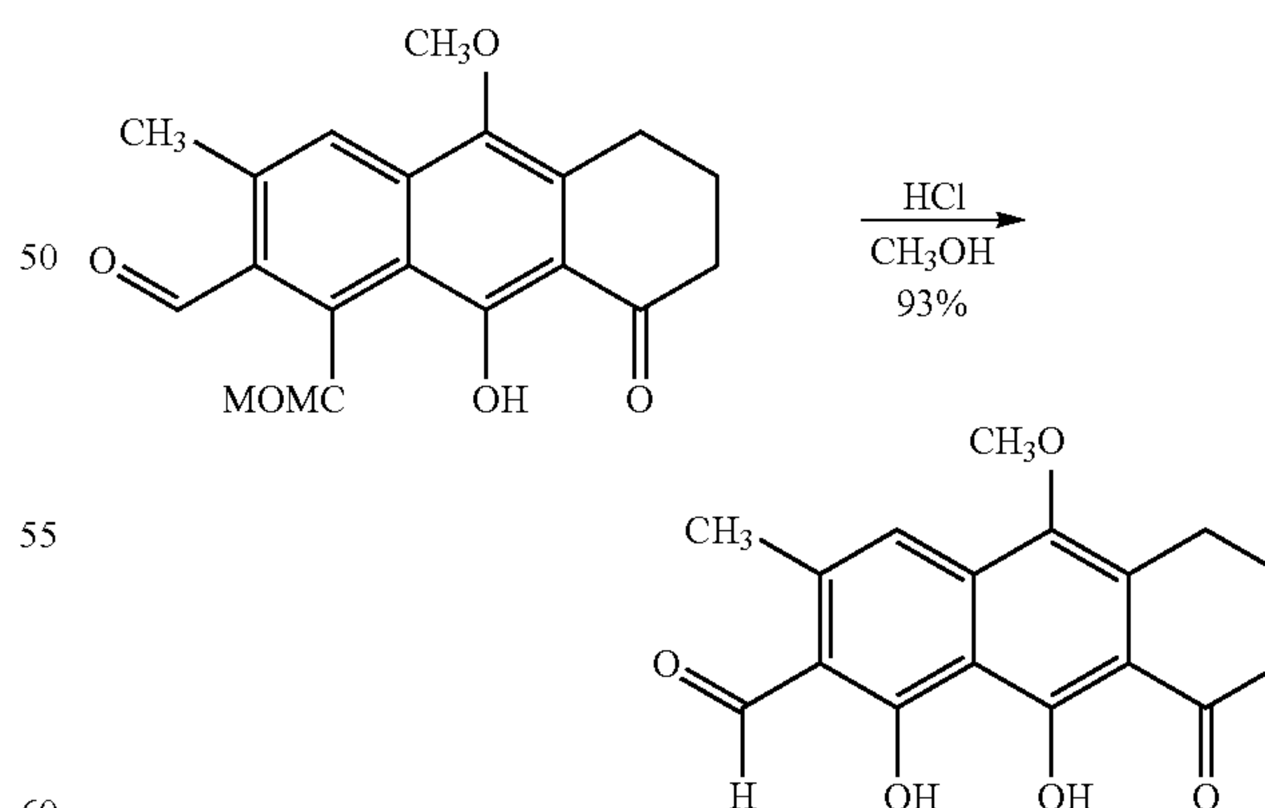
1,9-Dihydroxy-10-methoxy-3-methyl-8-oxo-5,6,7,8-tetrahydroanthracene-2-carbaldehyde
