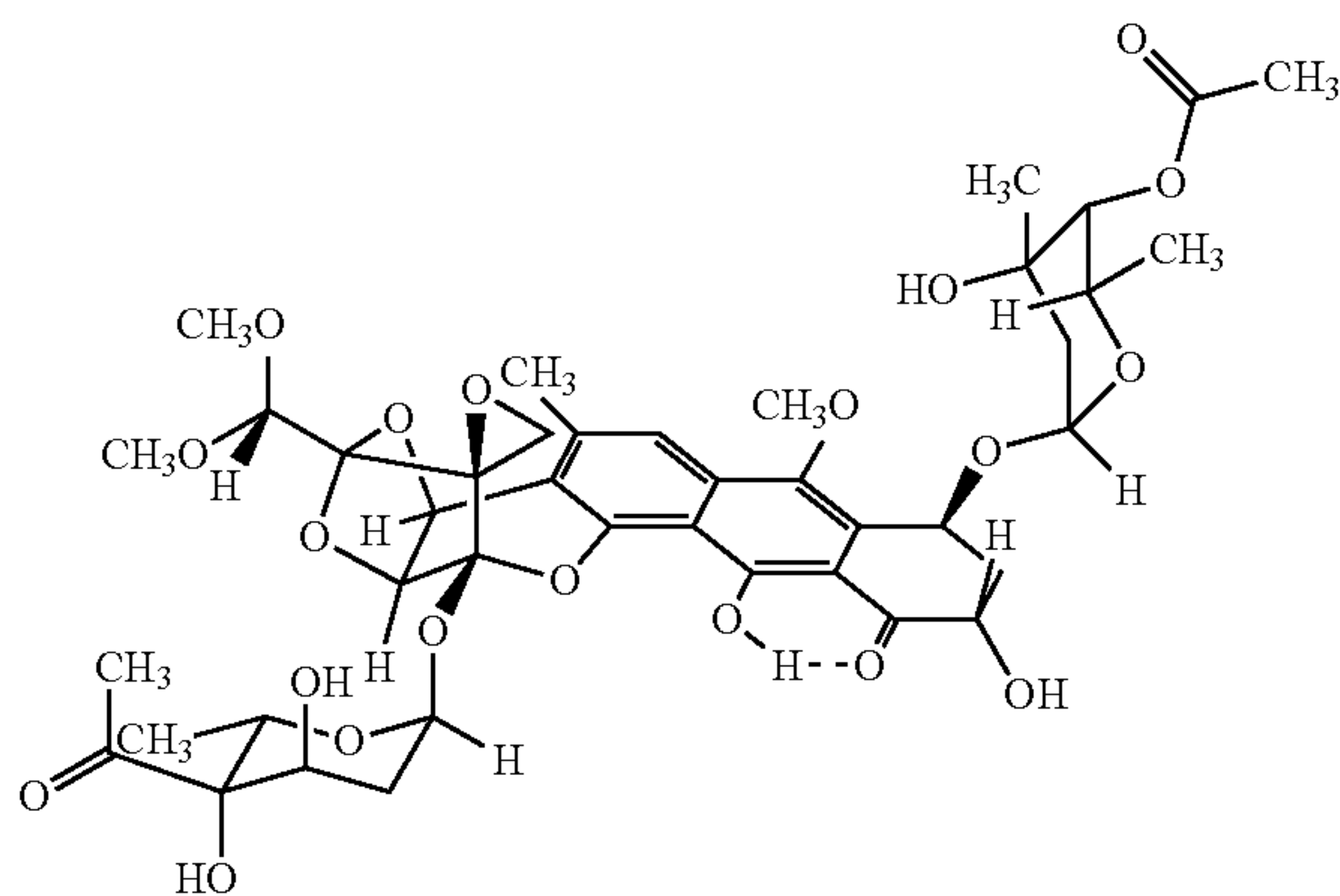
trioxacarcin A
