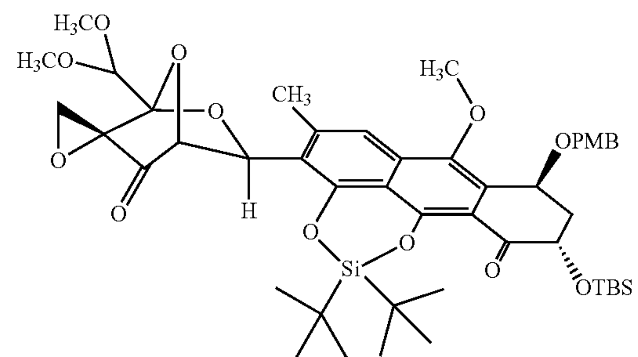
Exo cycloadduct 2
