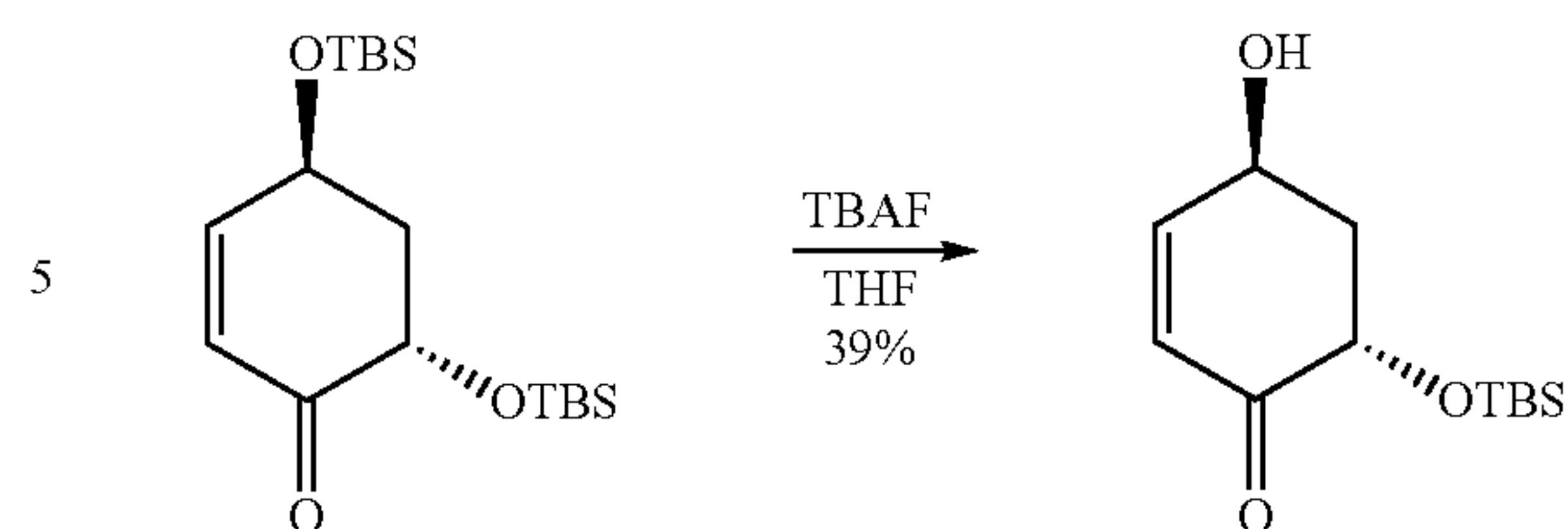
(4S,6S)-6-(tert-Butyldimethylsilyloxy)-4-hydroxycyclohex-2-enone
