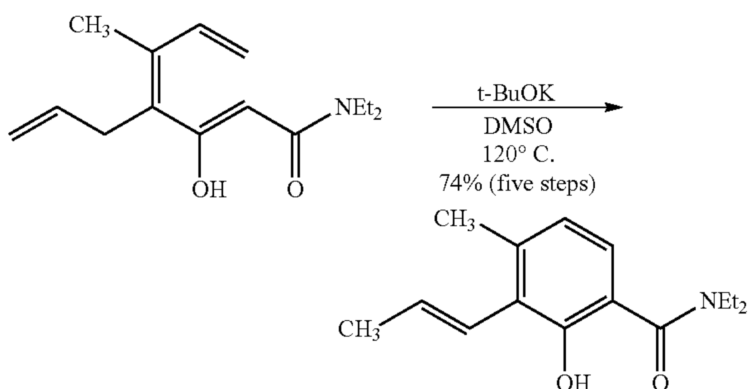
(E)-N,N-Diethyl-2-hydroxy-4-methyl-3-(prop-1-enyl)benzamide
