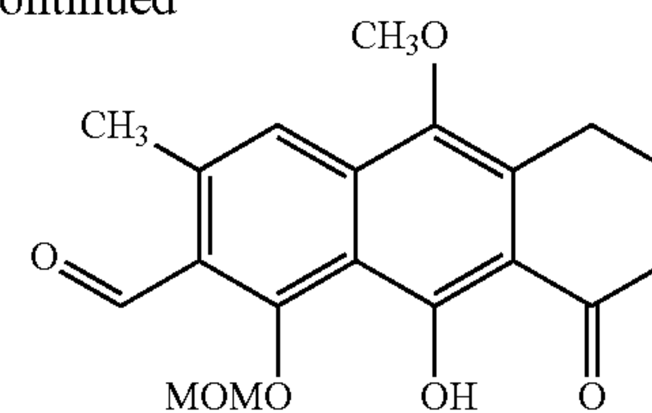
9-Hydroxy-10-methoxy-1-(methoxymethoxy)-3-methyl-8-oxo-5,6,7,8-tetrahydroanthracene-2-carbaldehyde
