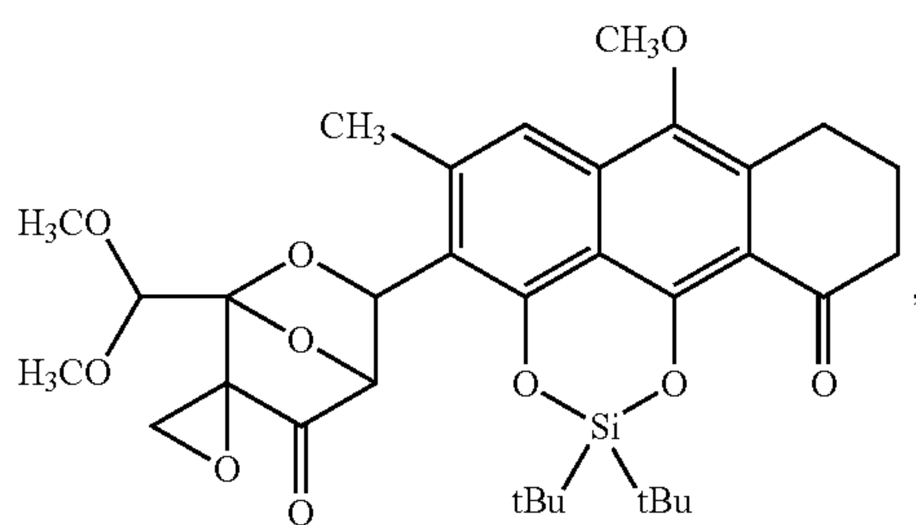
Dideoxy Cycloadduct
