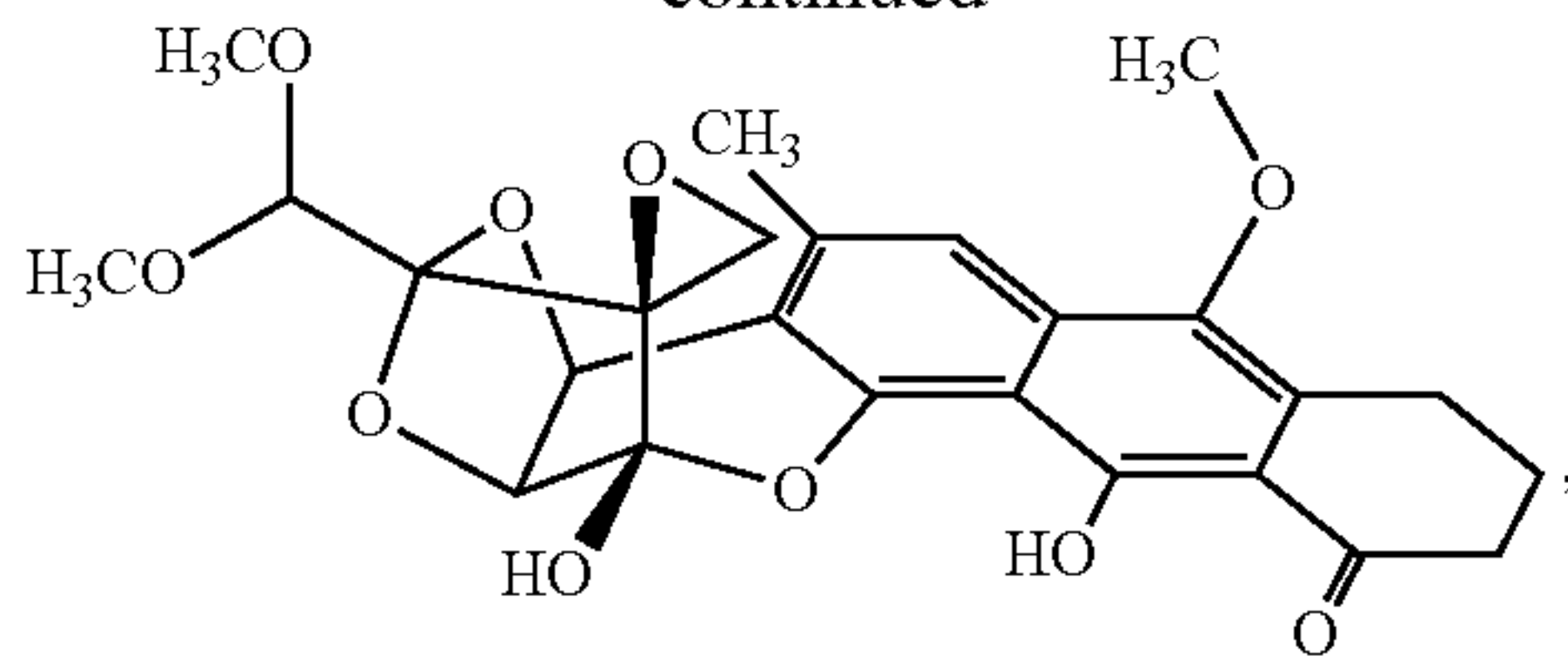
Dideoxy Endo 2 hemiketal "Dideoxy-DC-45-A2"
