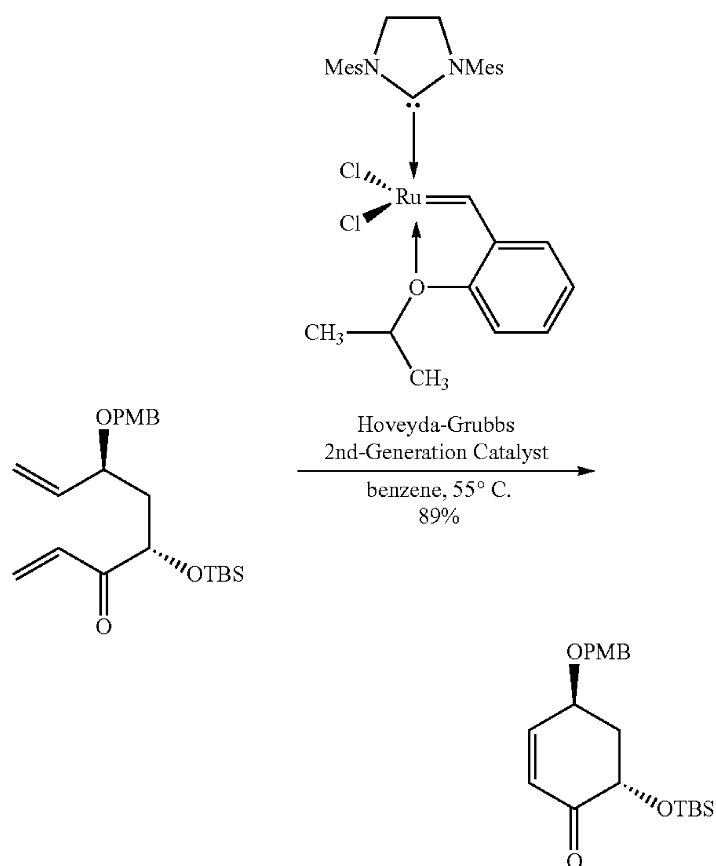
(4S,6S)-6-(tert-Butyldimethylsilyloxy)-4-(4-methoxybenzyloxy)cyclohex-2-enone ("Enone building block")
