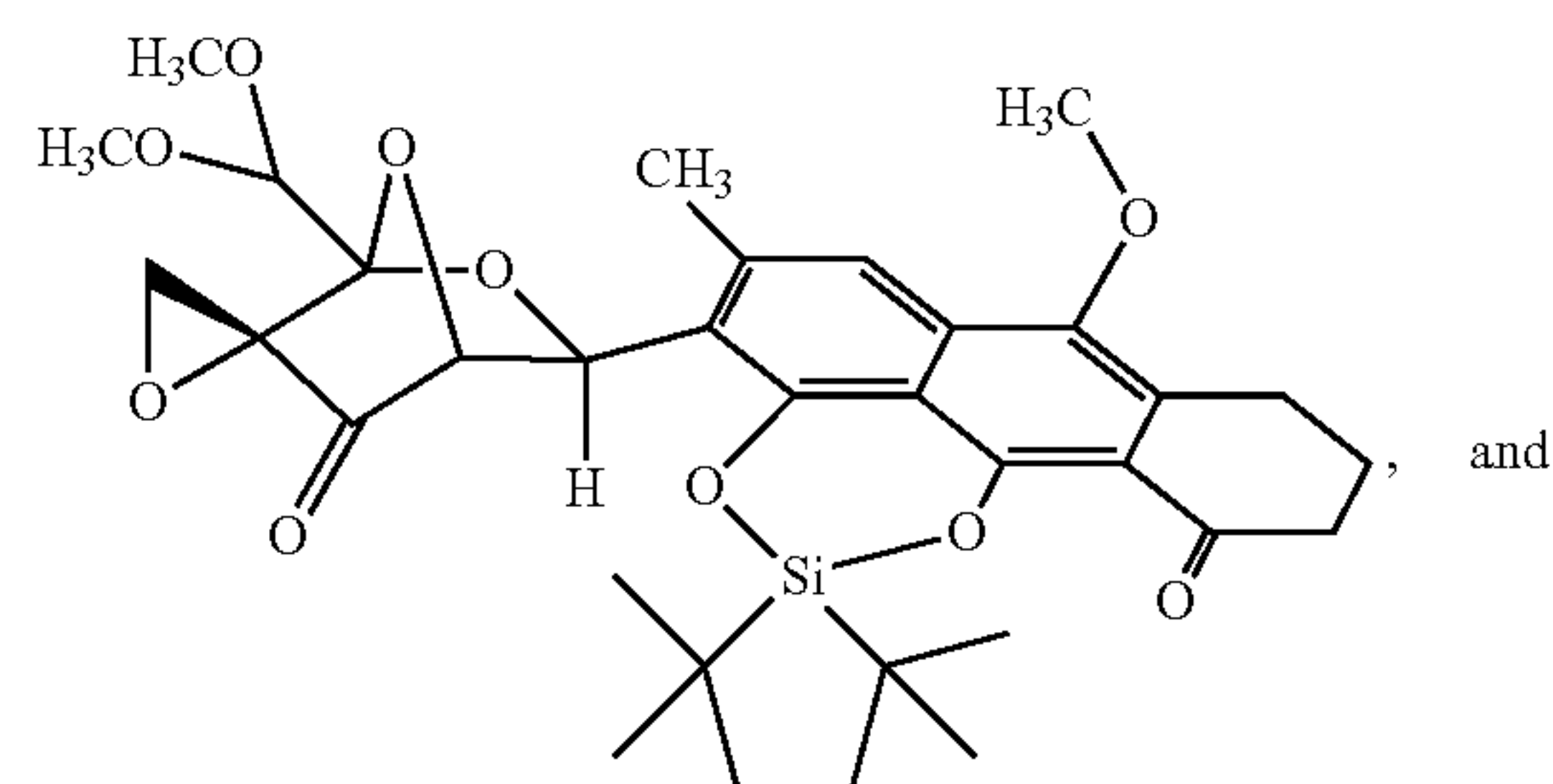
Dideoxy Exo cycloadduct 2
