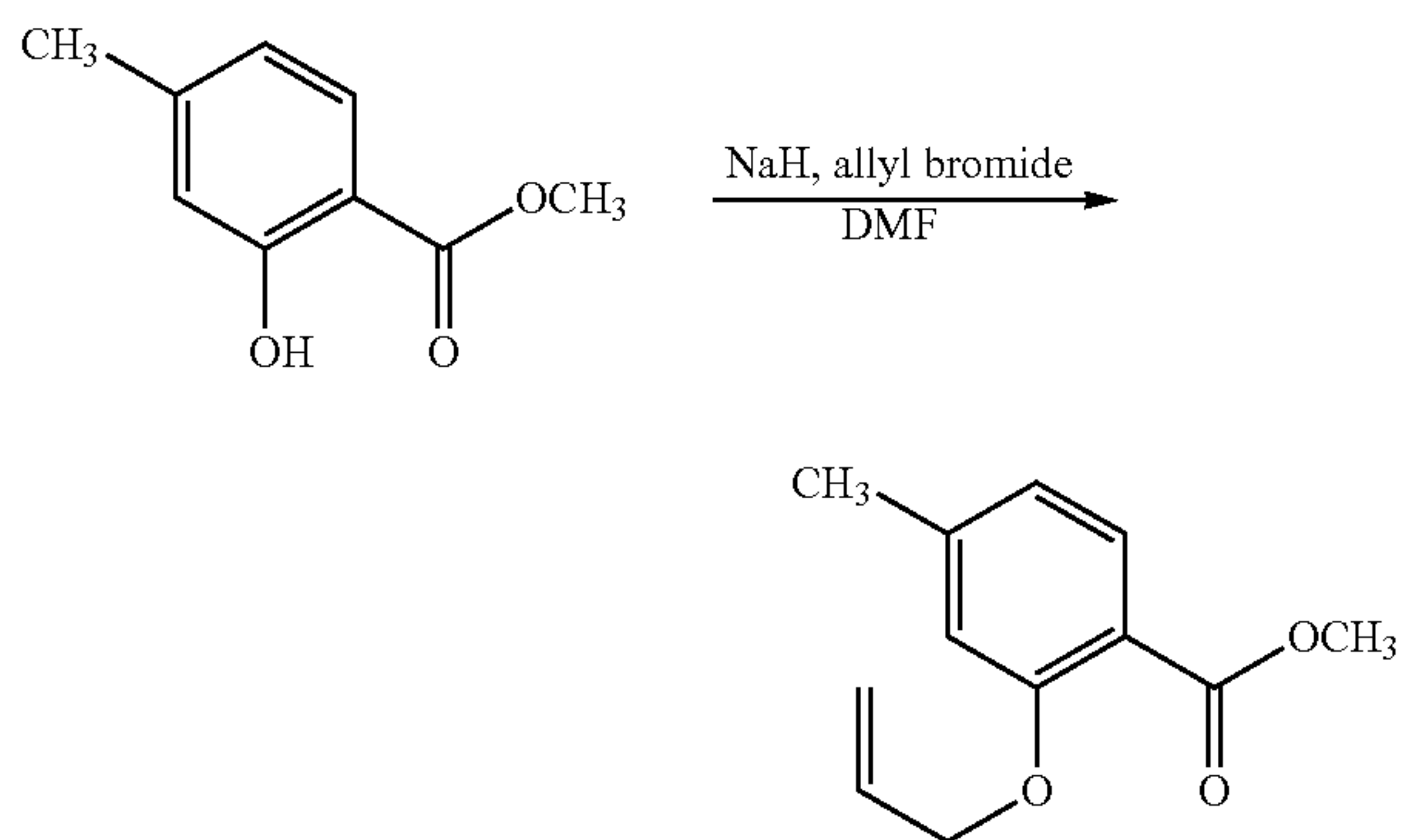
Methyl 2-(allyloxy)-4-methylbenzoate
