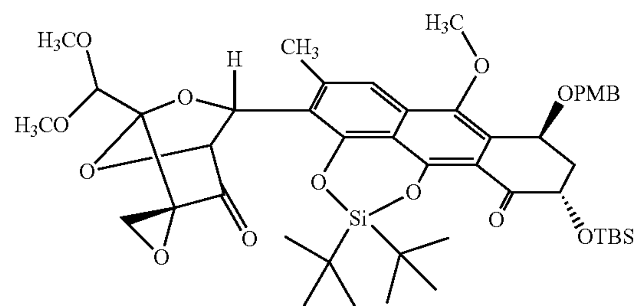
Endo cycloadduct 1
