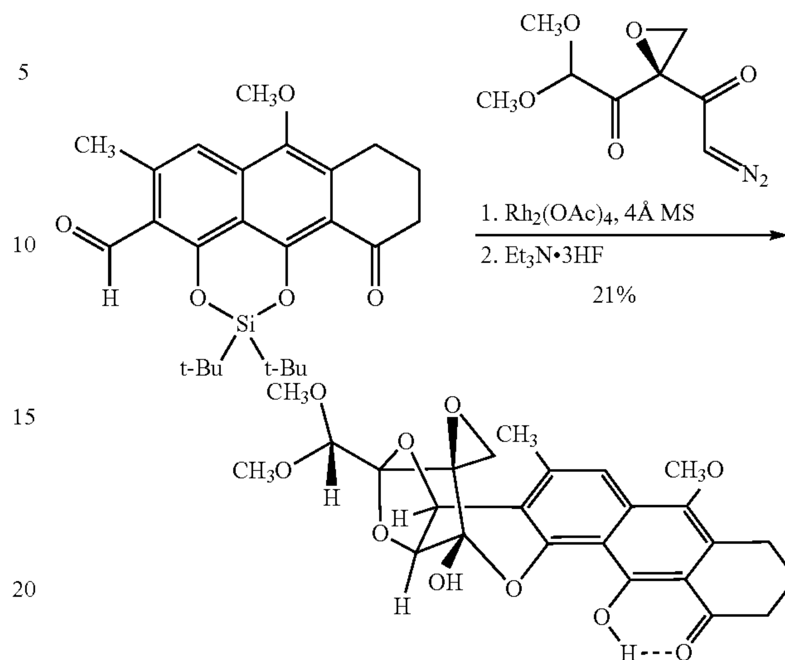
Dideoxy-DC-45-A2
