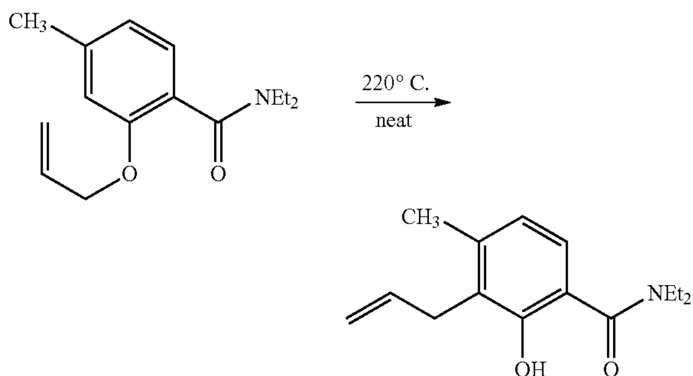
3-Allyl-N,N-diethyl-2-hydroxy-4-methylbenzamide
