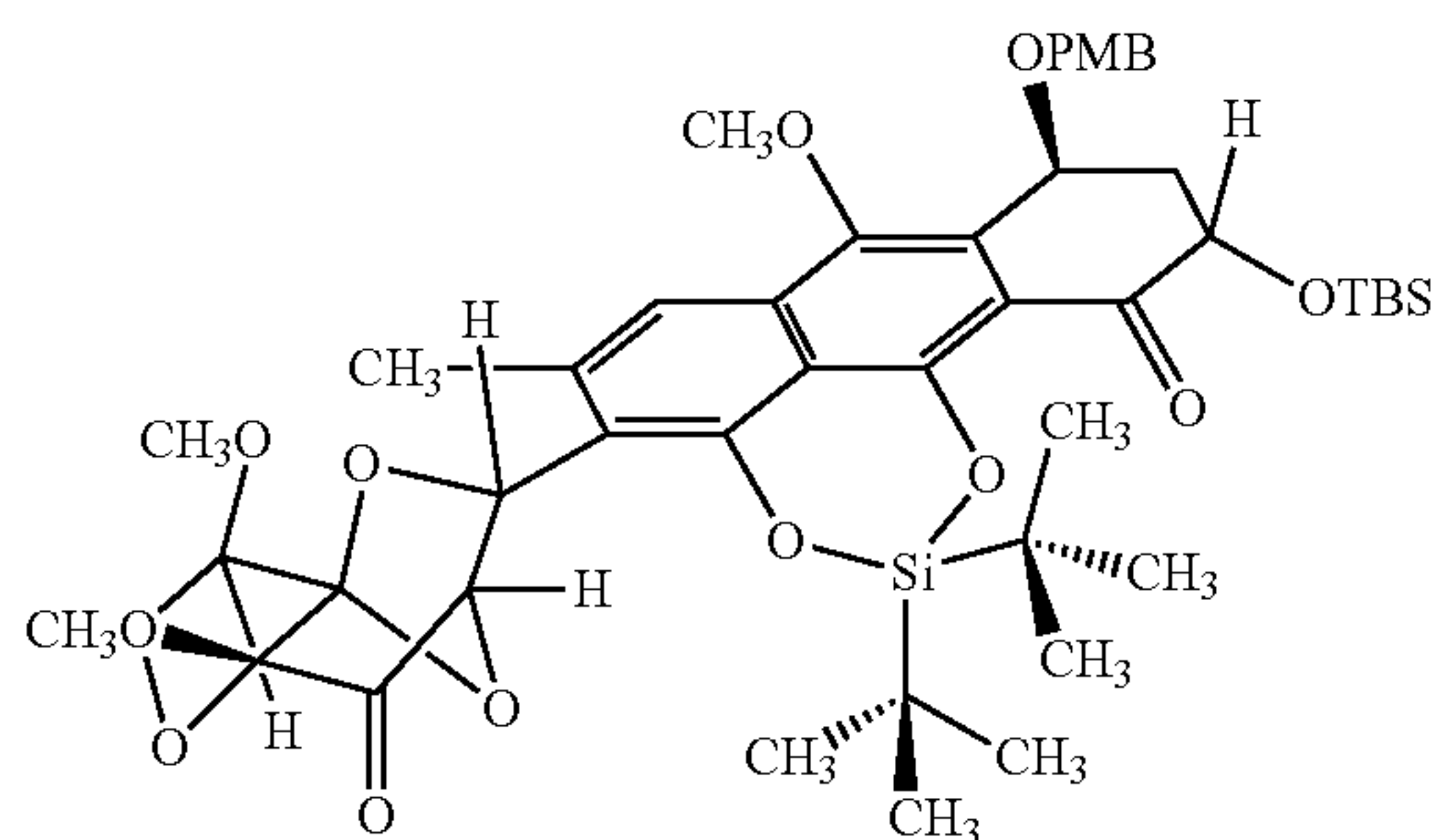
Exo Cycloadduct 1
