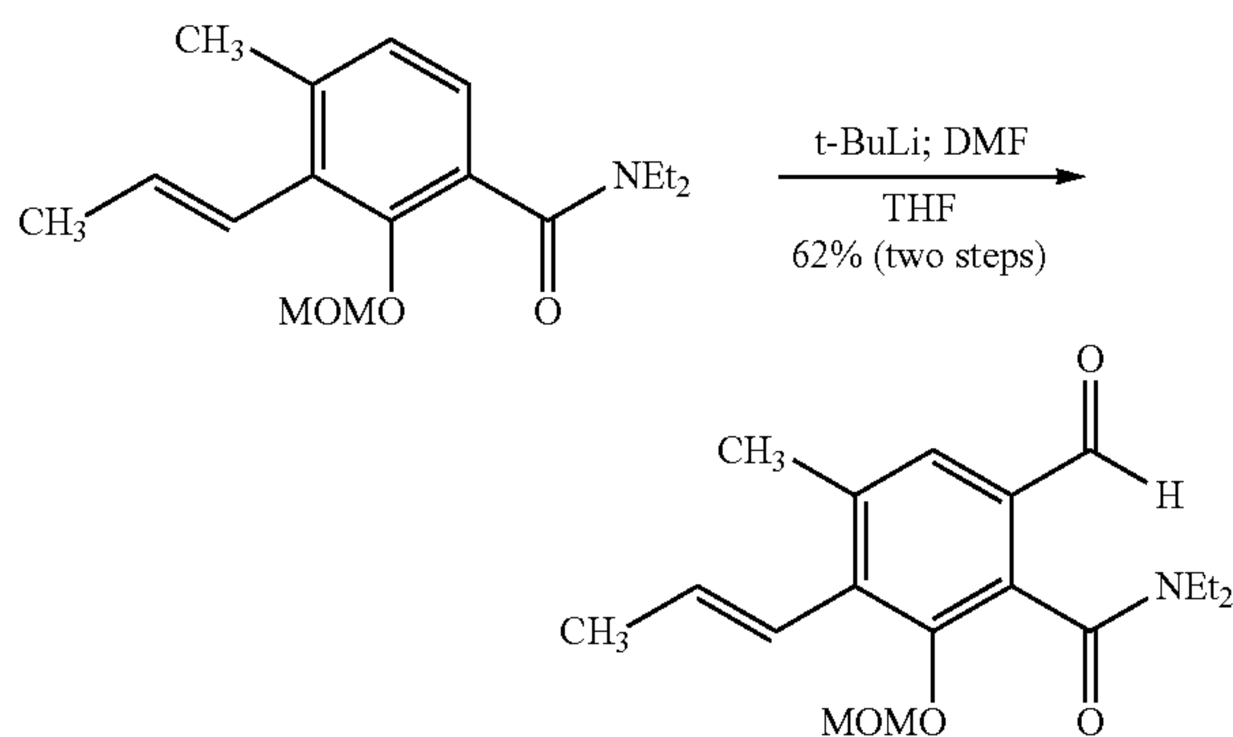
(E)-N,N-Diethyl-6-formyl-2-(methoxymethoxy)-4-methyl-3-(prop-1-enyl)benzamide
