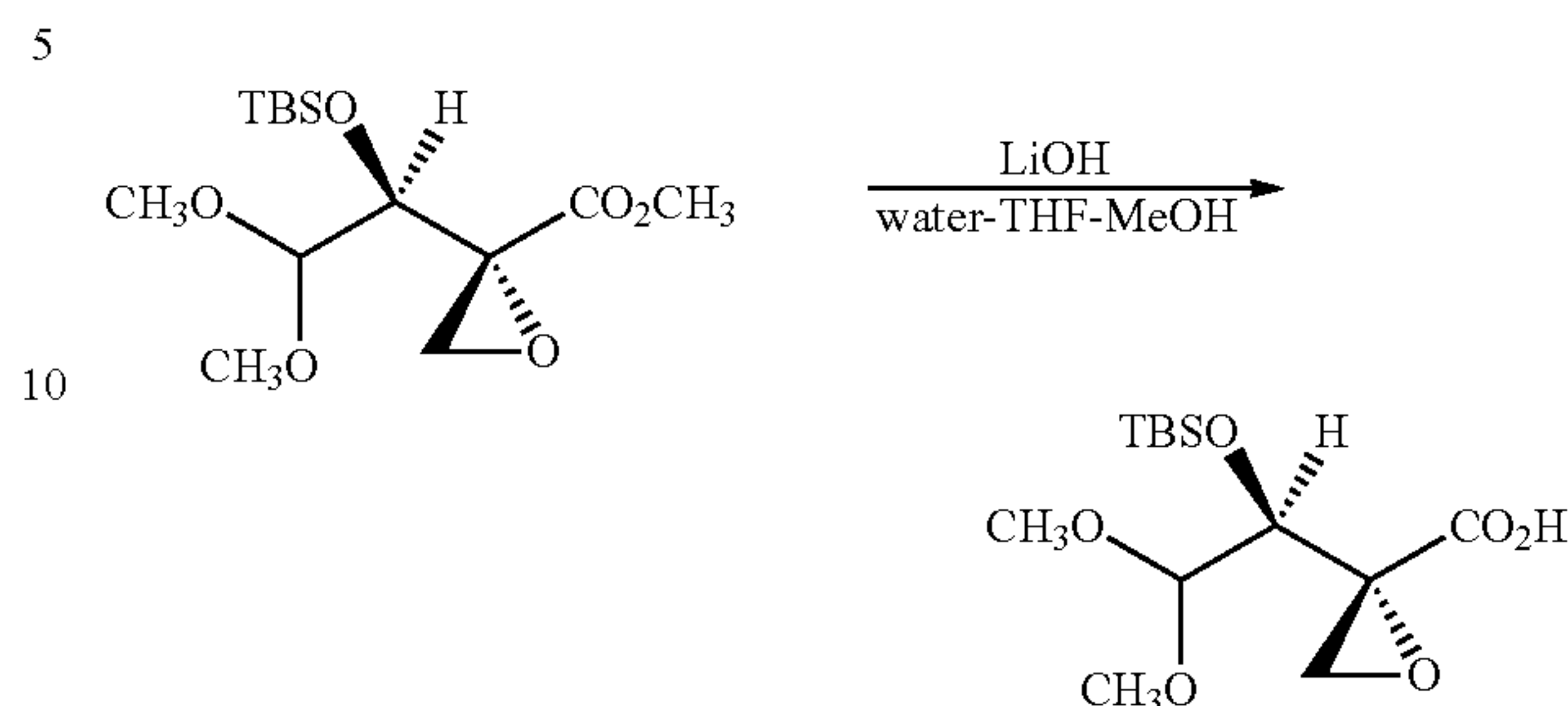
(2R,3S)-3-tert-Butyl dimethylsilyloxy-2-epoxy-4,4-dimethoxybutanoic acid
