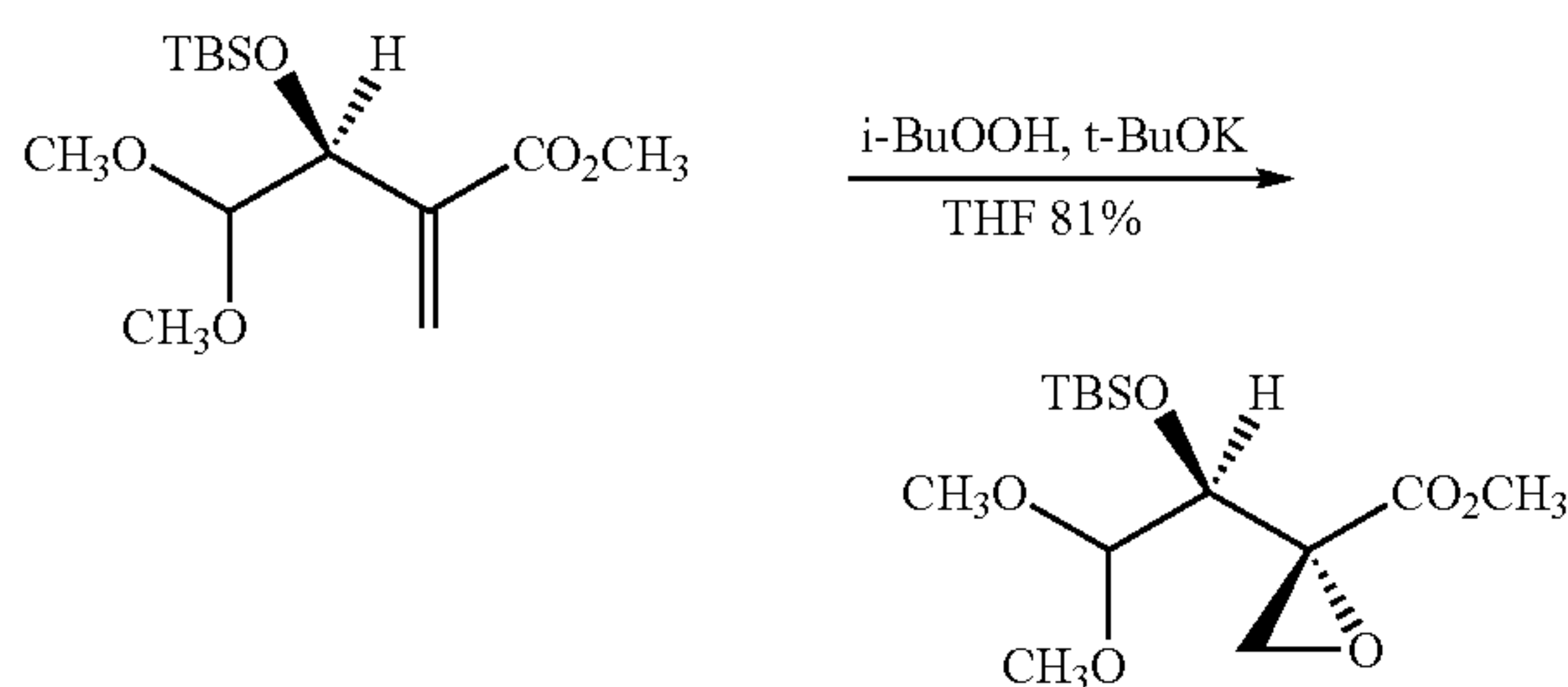
(2R,3S)-Methyl 3-tert-butyl dimethylsilyloxy-2-epoxy-4,4-dimethoxybutanoate
