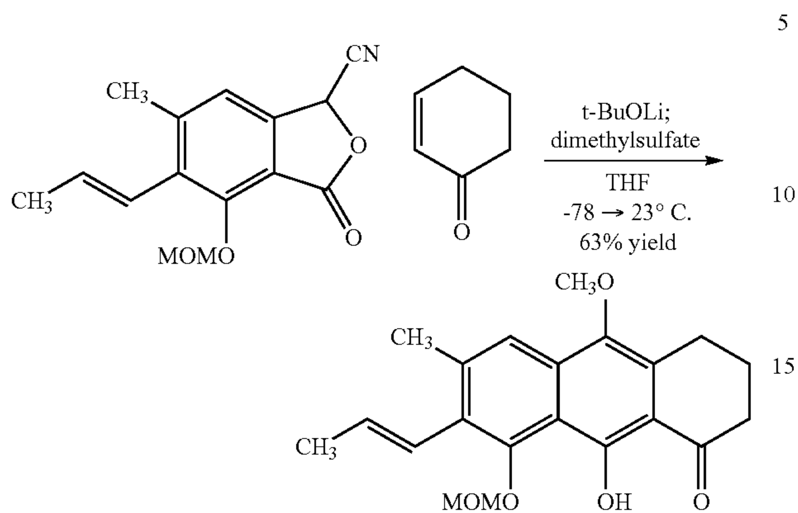
(E)-9-Hydroxy-10-methoxy-8-(methoxymethoxy)-6-methyl-7-(prop-1-enyl)-3,4-dihydroanthracen-1-one
