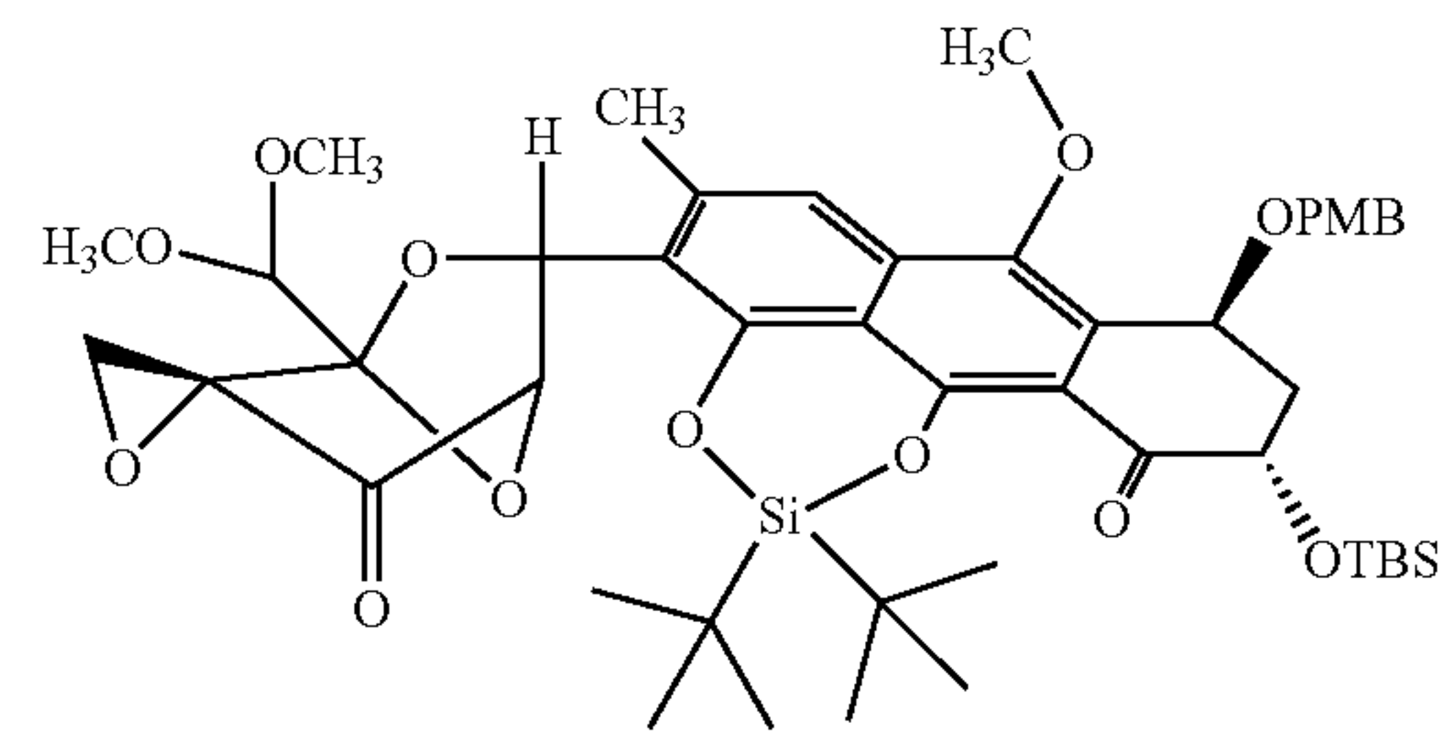
Exo cycloadduct 1
