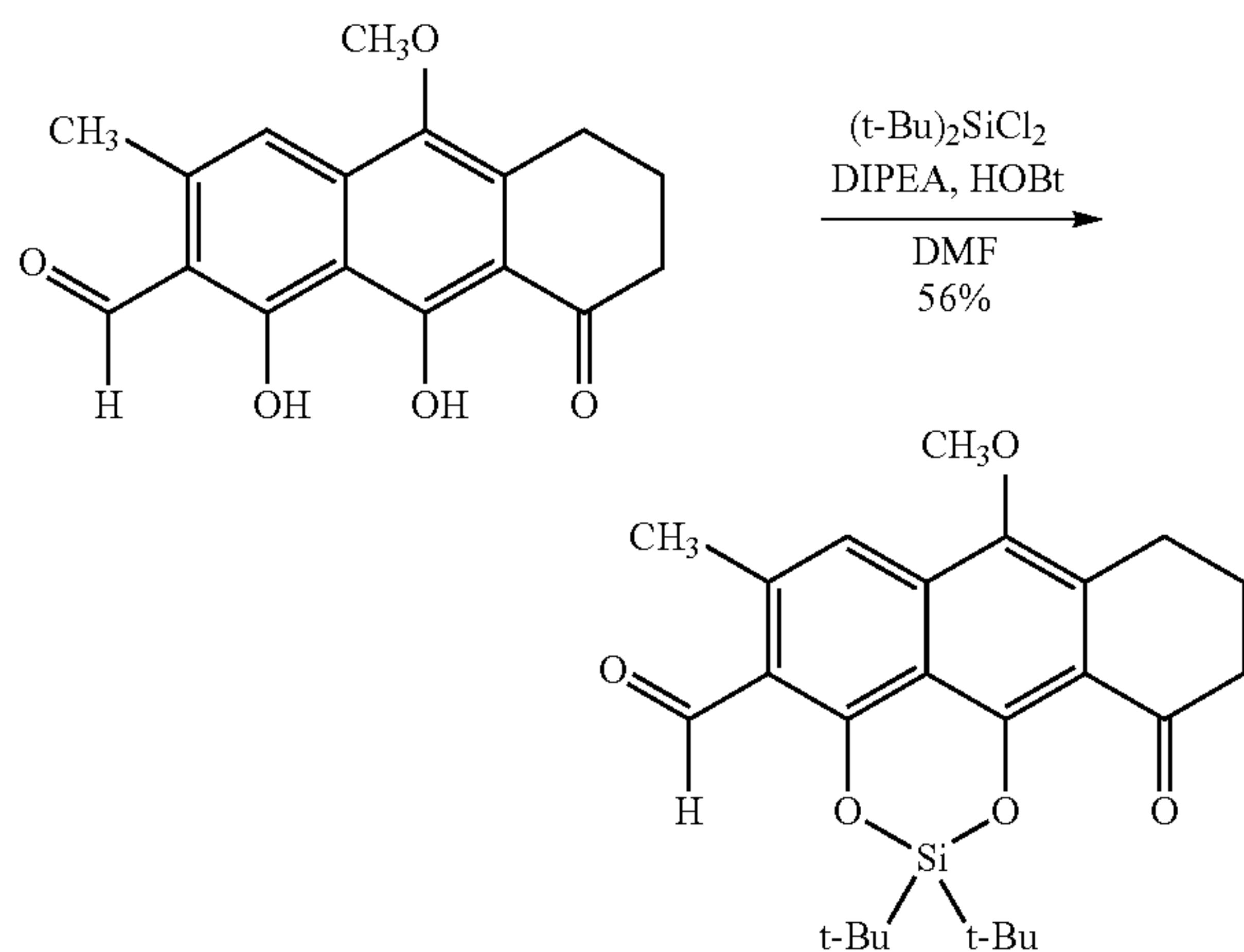
2,2-Di-tert-butyl-7-methoxy-5-methyl-11-oxo-8,9,10,11-tetrahydroanthra[9,1-de][1,3,2]dioxasiline-4-carbaldehyde
