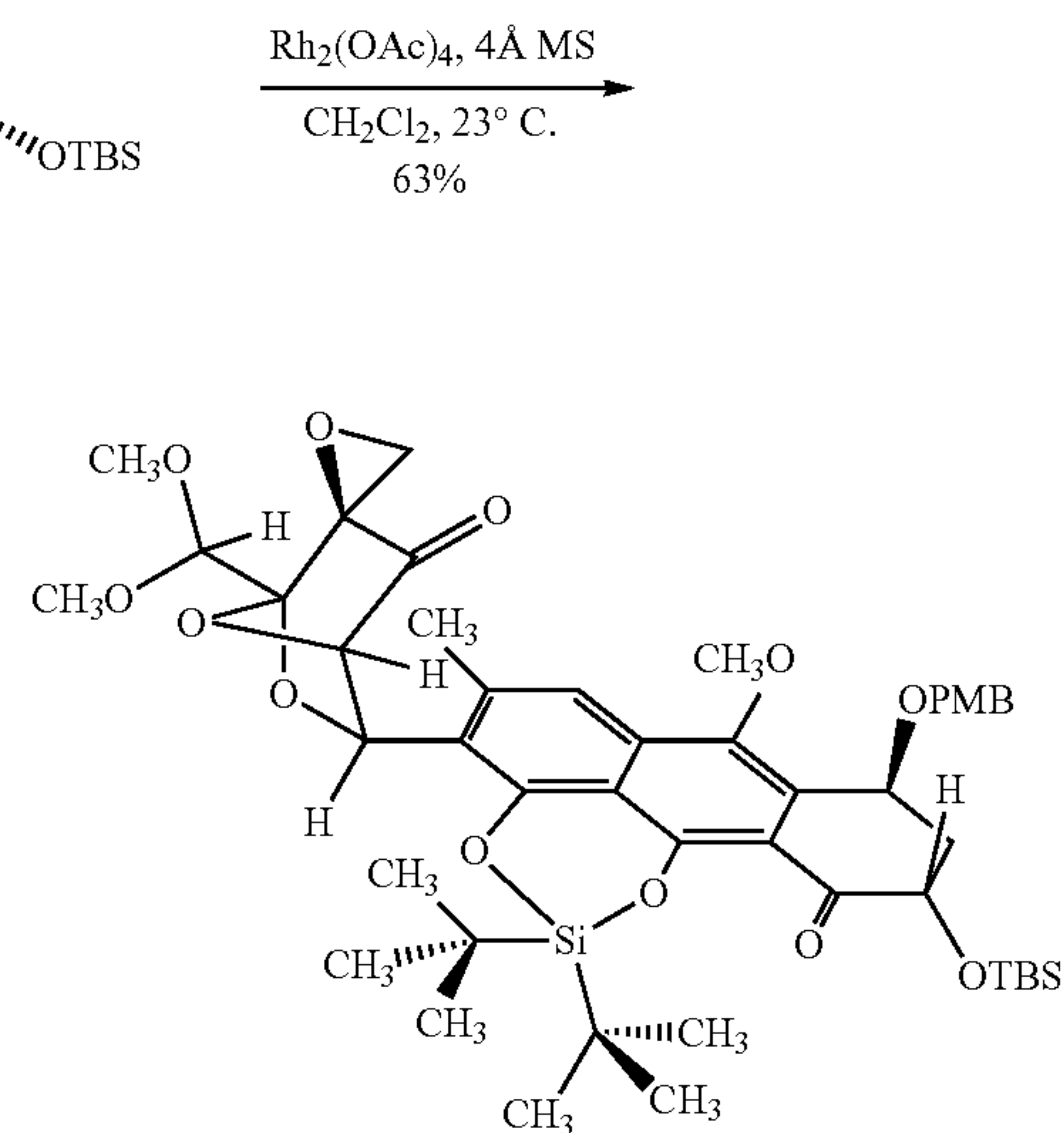
Endo Cycloadduct 2
