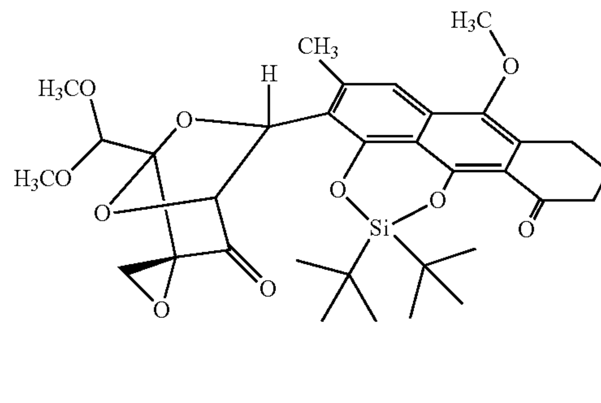
Dideoxy Endo cycloadduct 1
