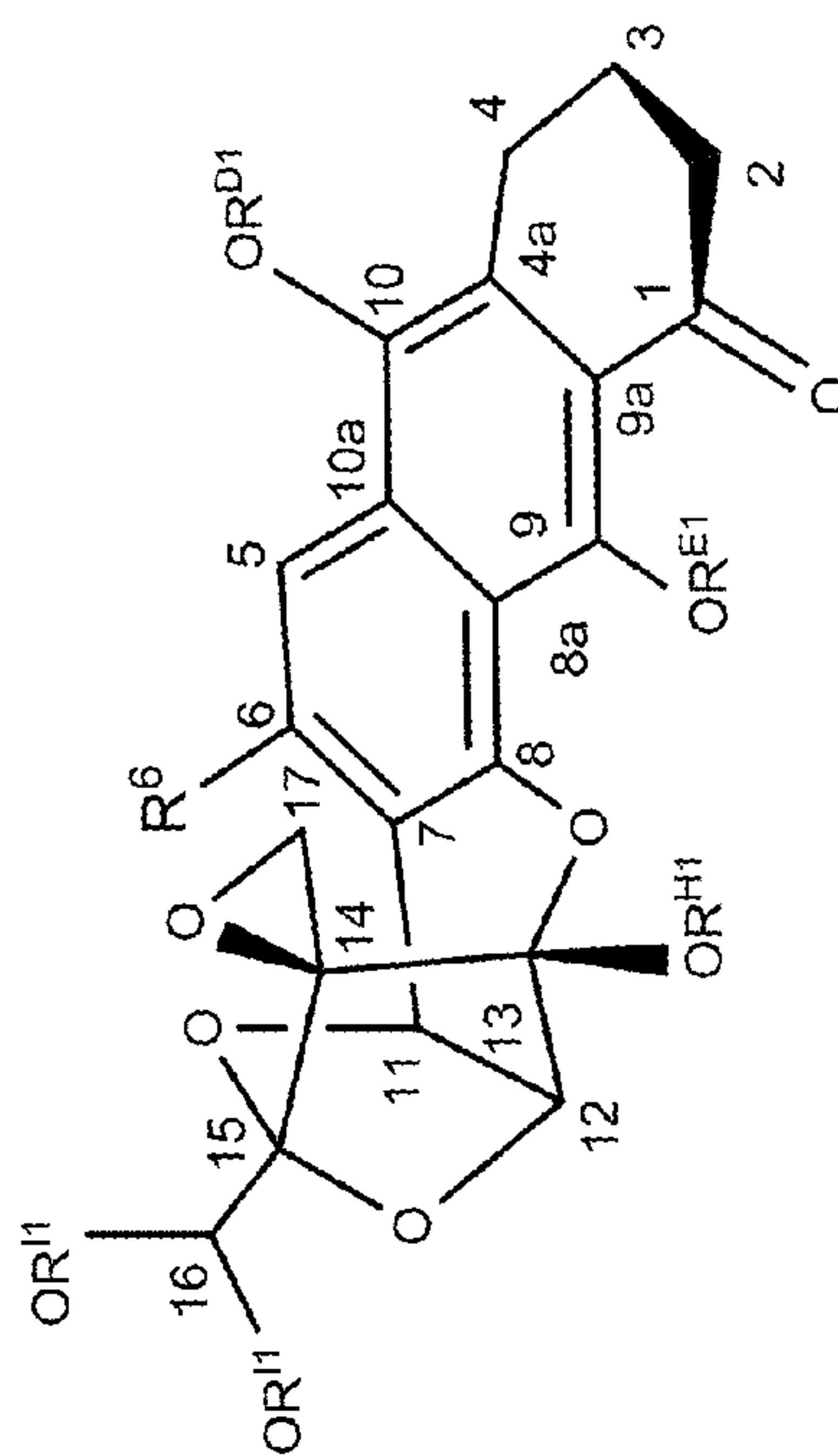
Trioxacarcin scaffold
