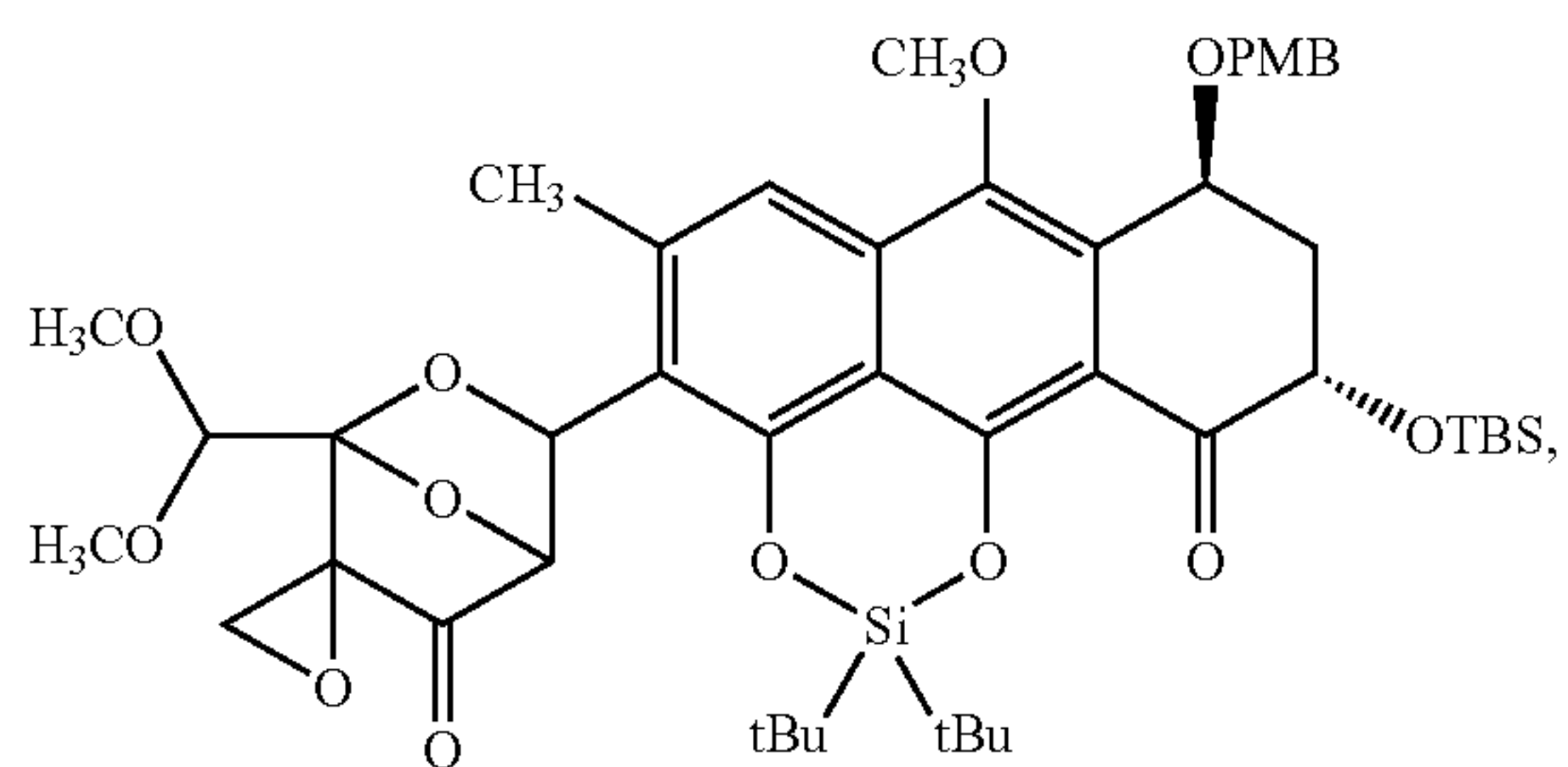
Cycloadduct
