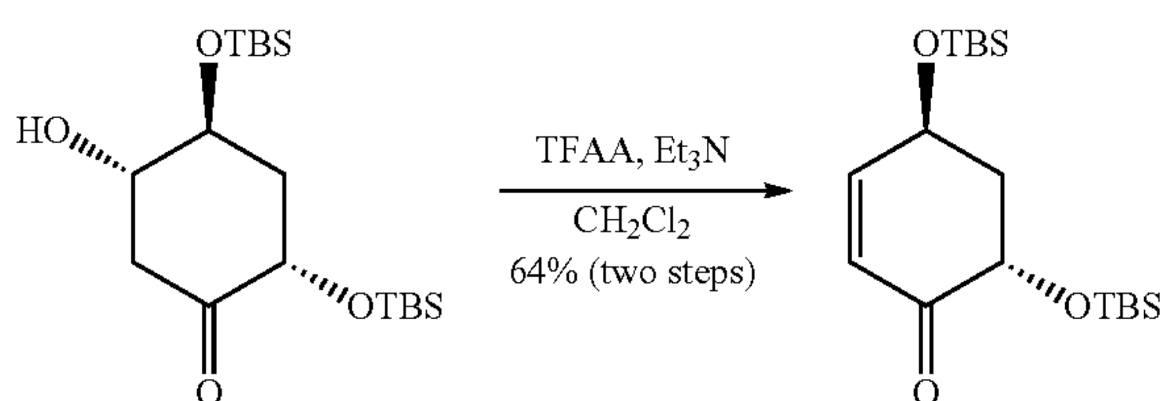
(4S,6S)-4,6-Bis(tert-butyldimethylsilyloxy)cyclohex-2-enone
