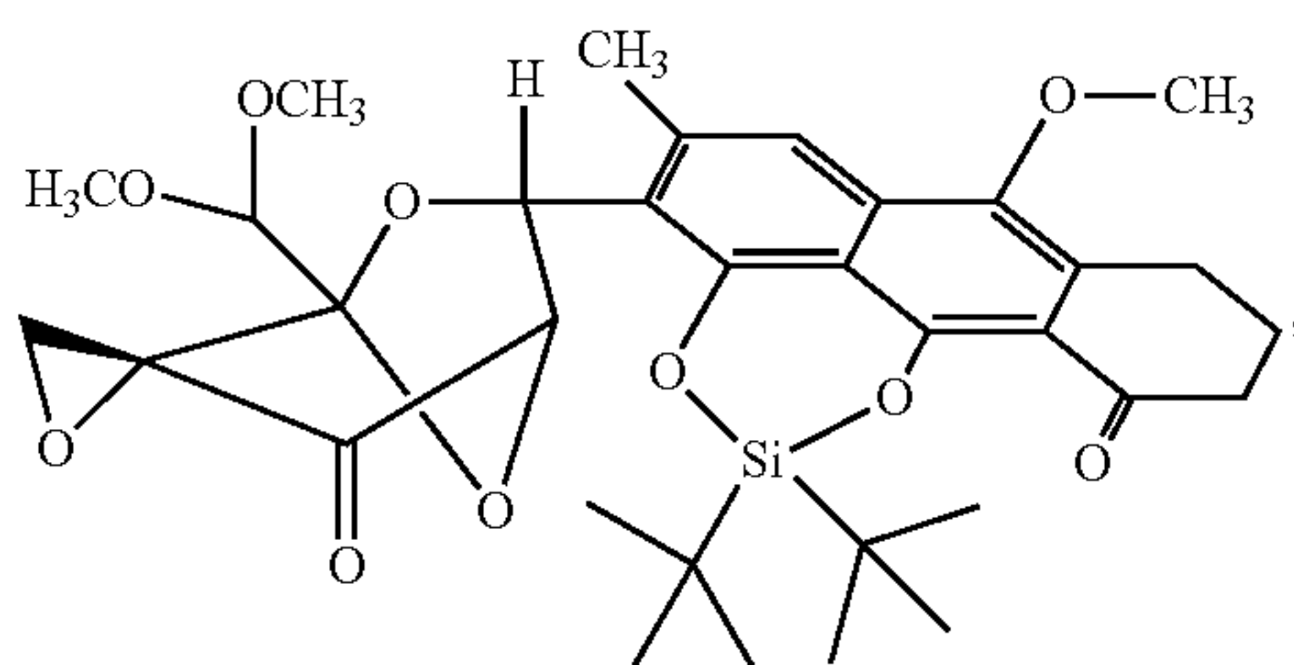
Dideoxy Exo cycloadduct 1
