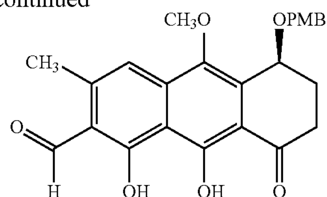
(S)-1,9-Dihydroxy-10-methoxy-5-(4-methoxybenzyloxy)-3-methyl-8-oxo-5,6,7,8-tetrahydroanthracene-2-carbaldehyde
