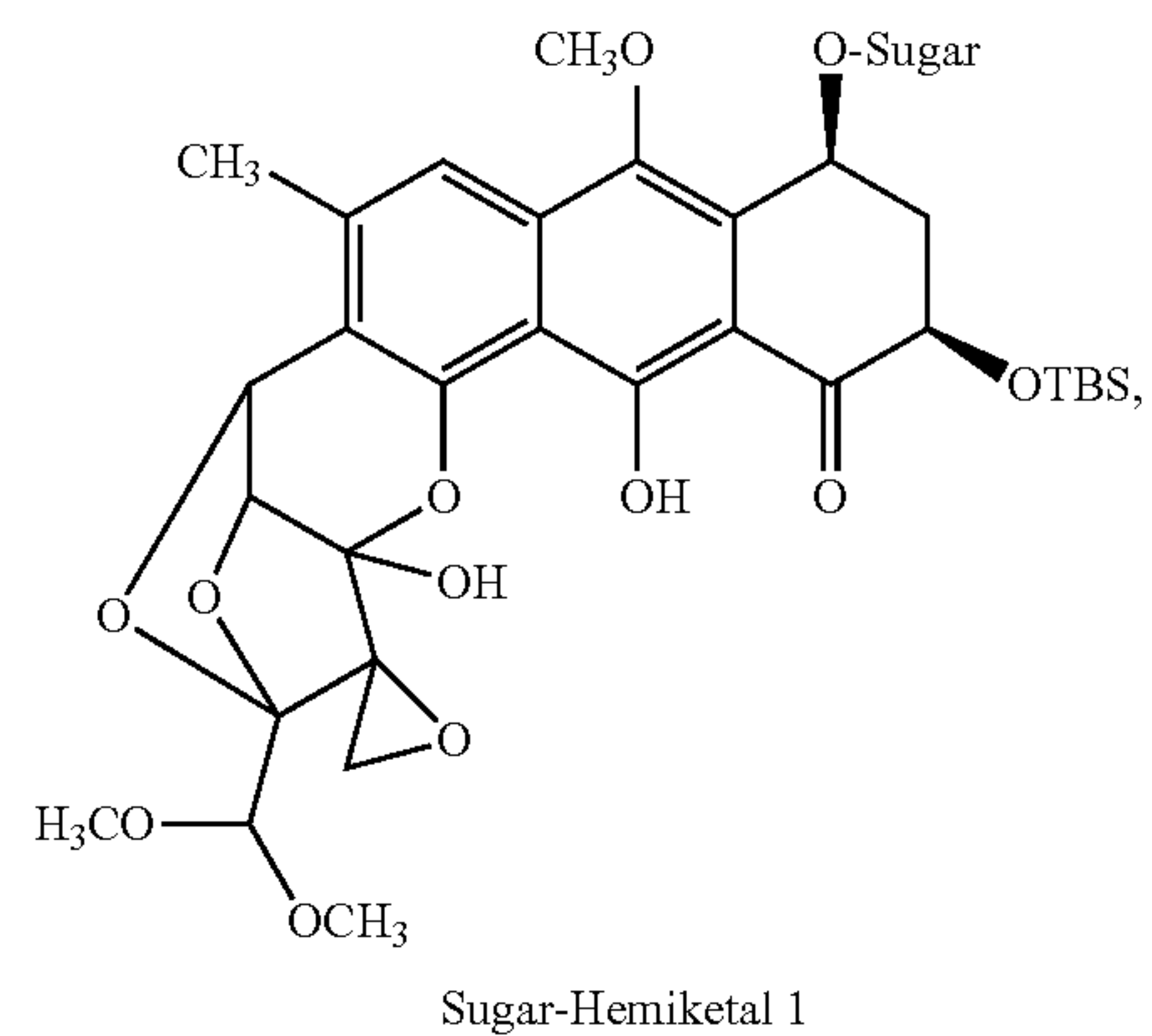
Dideoxy hemiketal
