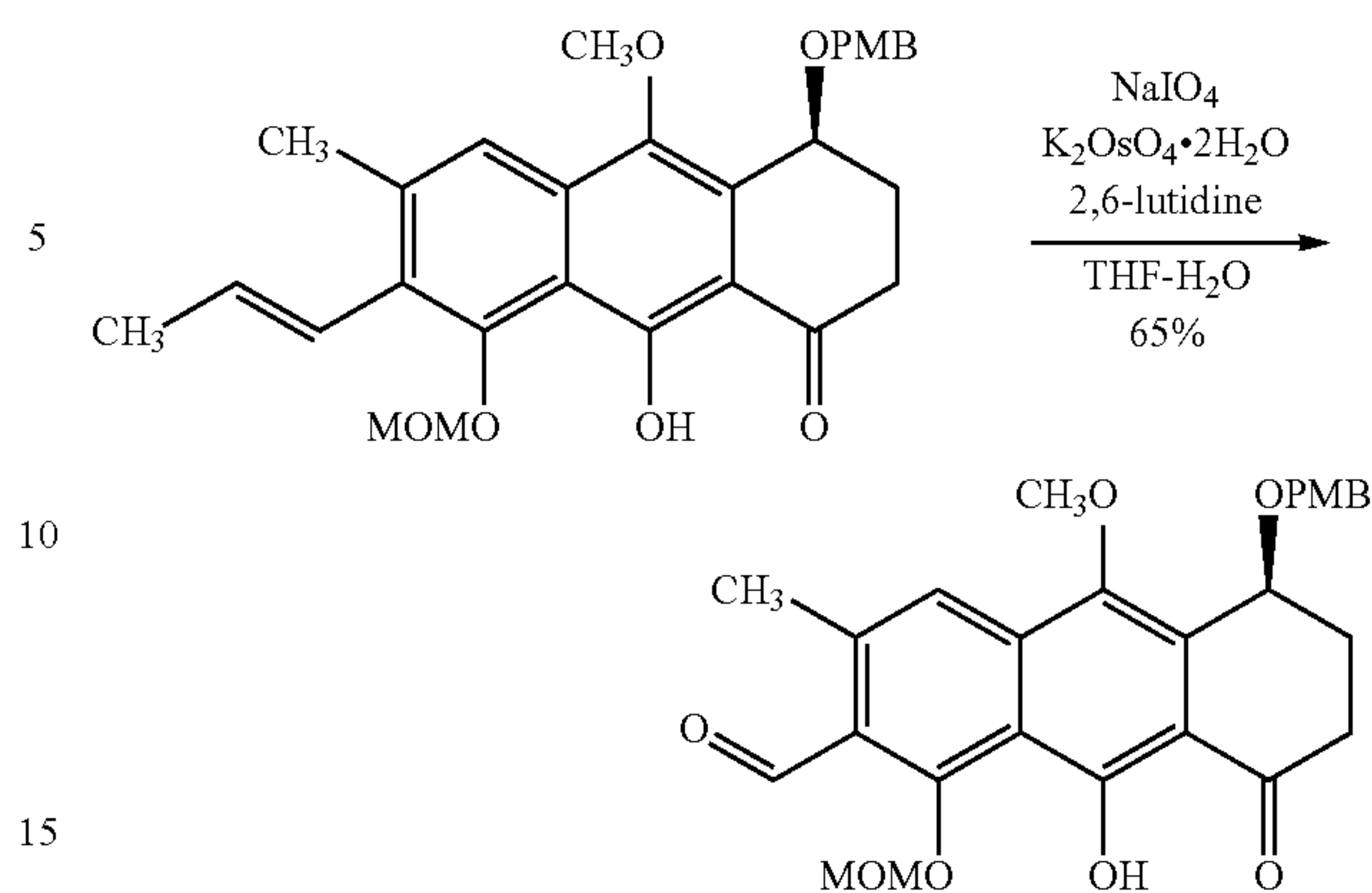
(S)-9-Hydroxy-10-methoxy-5-(4-methoxybenzyloxy)-1-(methoxymethoxy)-3-methyl-8-oxo-5,6,7,8-tetrahydroanthracene-2-carbaldehyde
