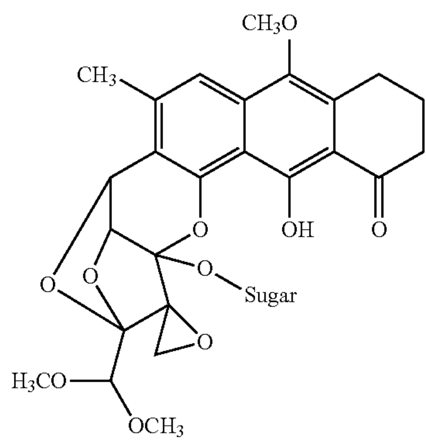
Dideoxy-Sugar-Hemiketal
