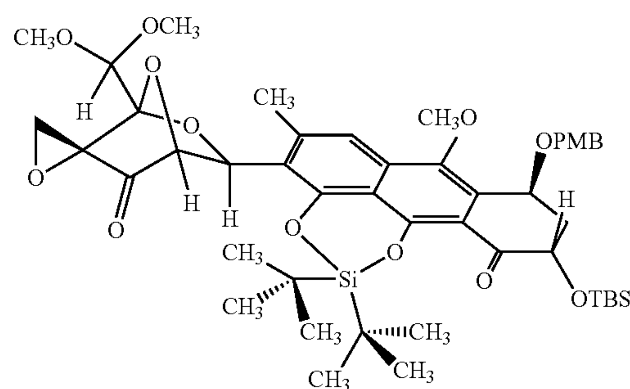
Exo Cycloadduct 2
