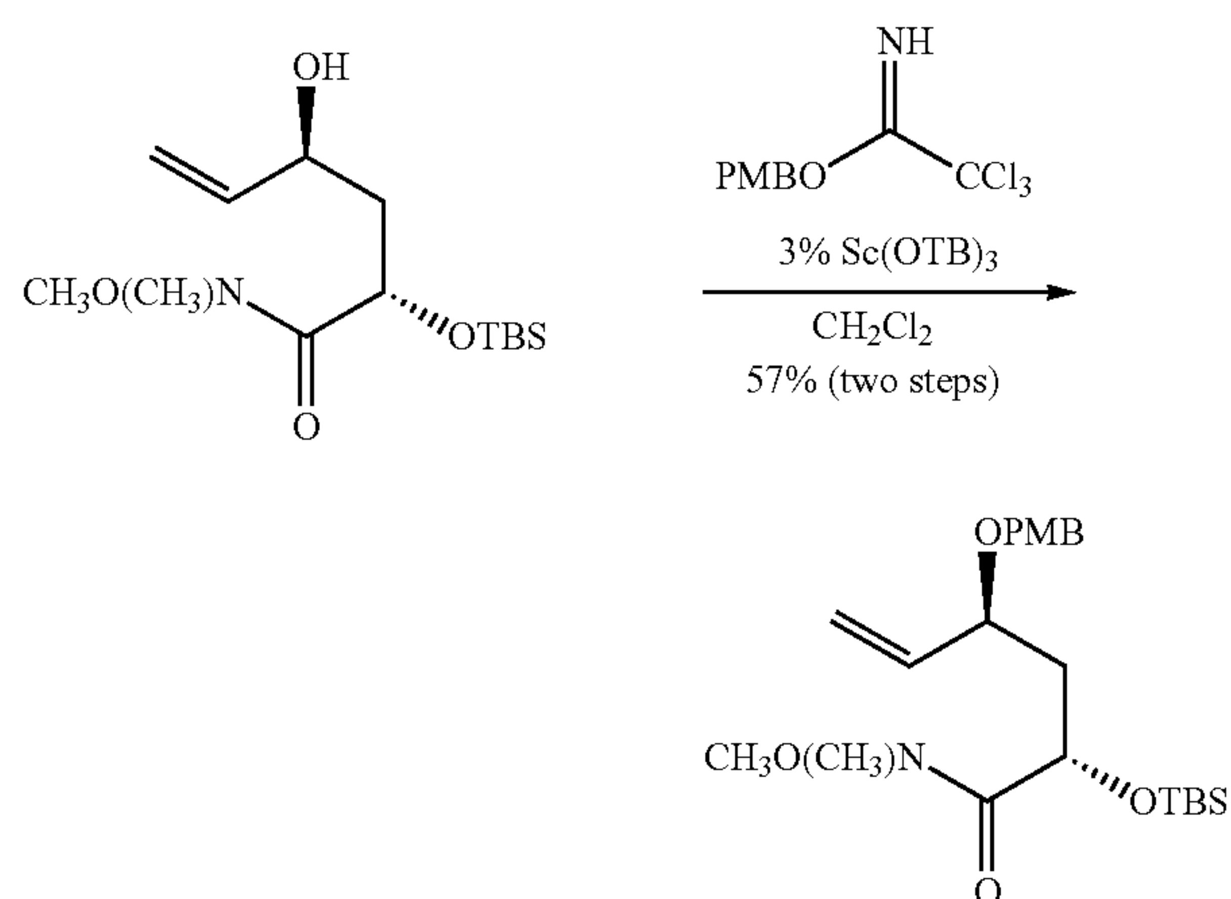
(2S,4S)-2-(tert-Butyldimethylsilyloxy)-N-methoxy-4-[(4-methoxybenzyl)oxy]-N-methylhex-5-enamide
