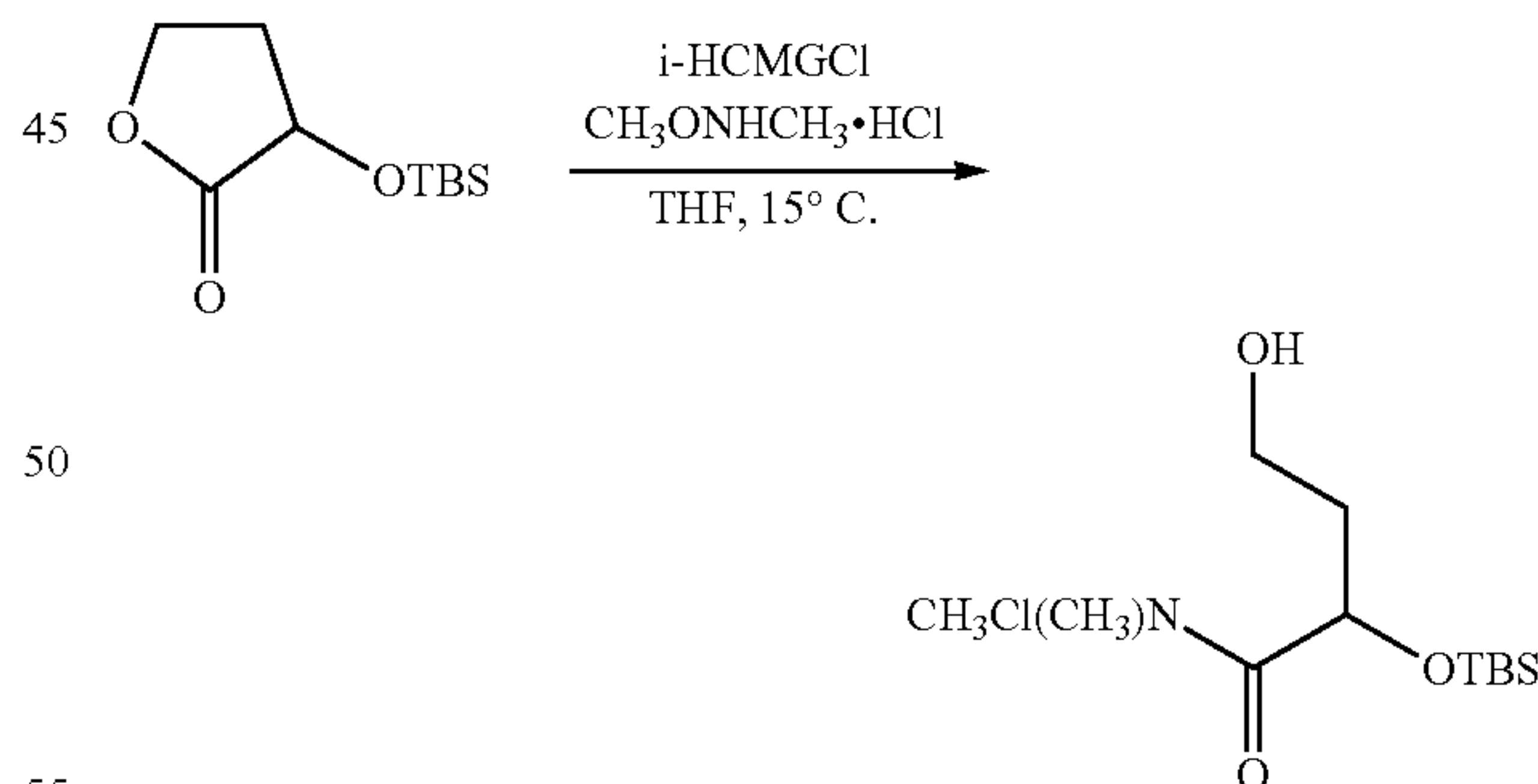
(2S)-2-(tert-Butyldimethylsilyloxy)-4-hydroxy-N-methoxy-N-methylbutanamide
