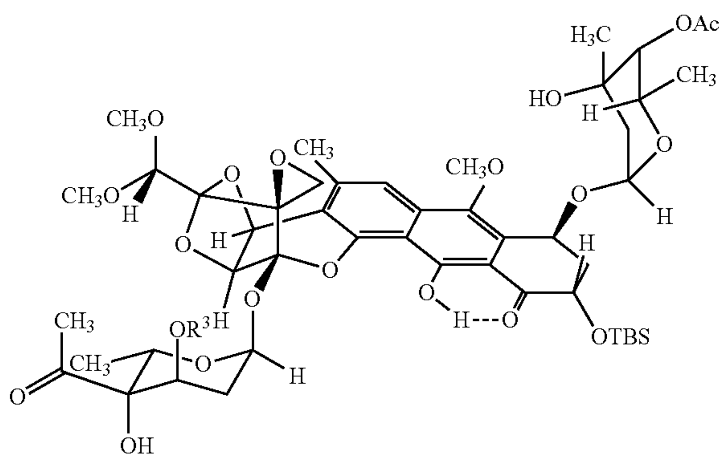
R^3 = \text{CO}(\text{CH}_2)_2\text{N}_3
