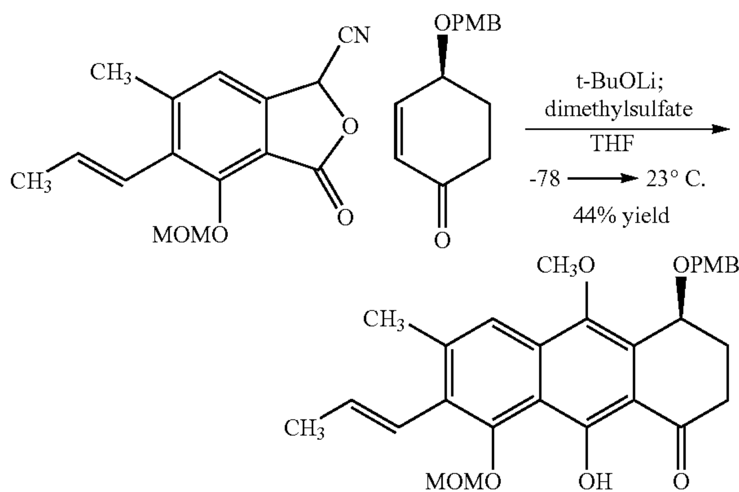
(S,E)-9-Hydroxy-10-methoxy-4-(4-methoxybenzyloxy)-8-(methoxymethoxy)-6-methyl-7-(prop-1-enyl)-3,4-dihydroanthracen-1-one
