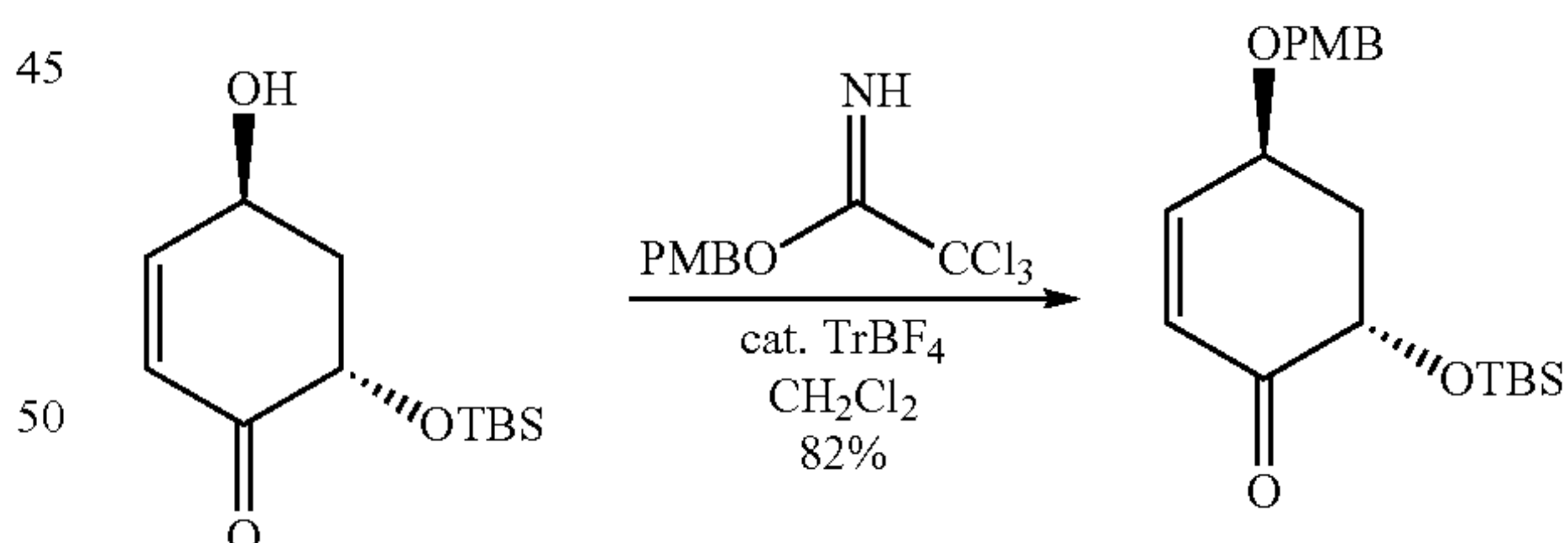
(4S,6S)-6-(tert-Butyldimethylsilyloxy)-4-(4-methoxybenzyloxy)cyclohex-2-enone
