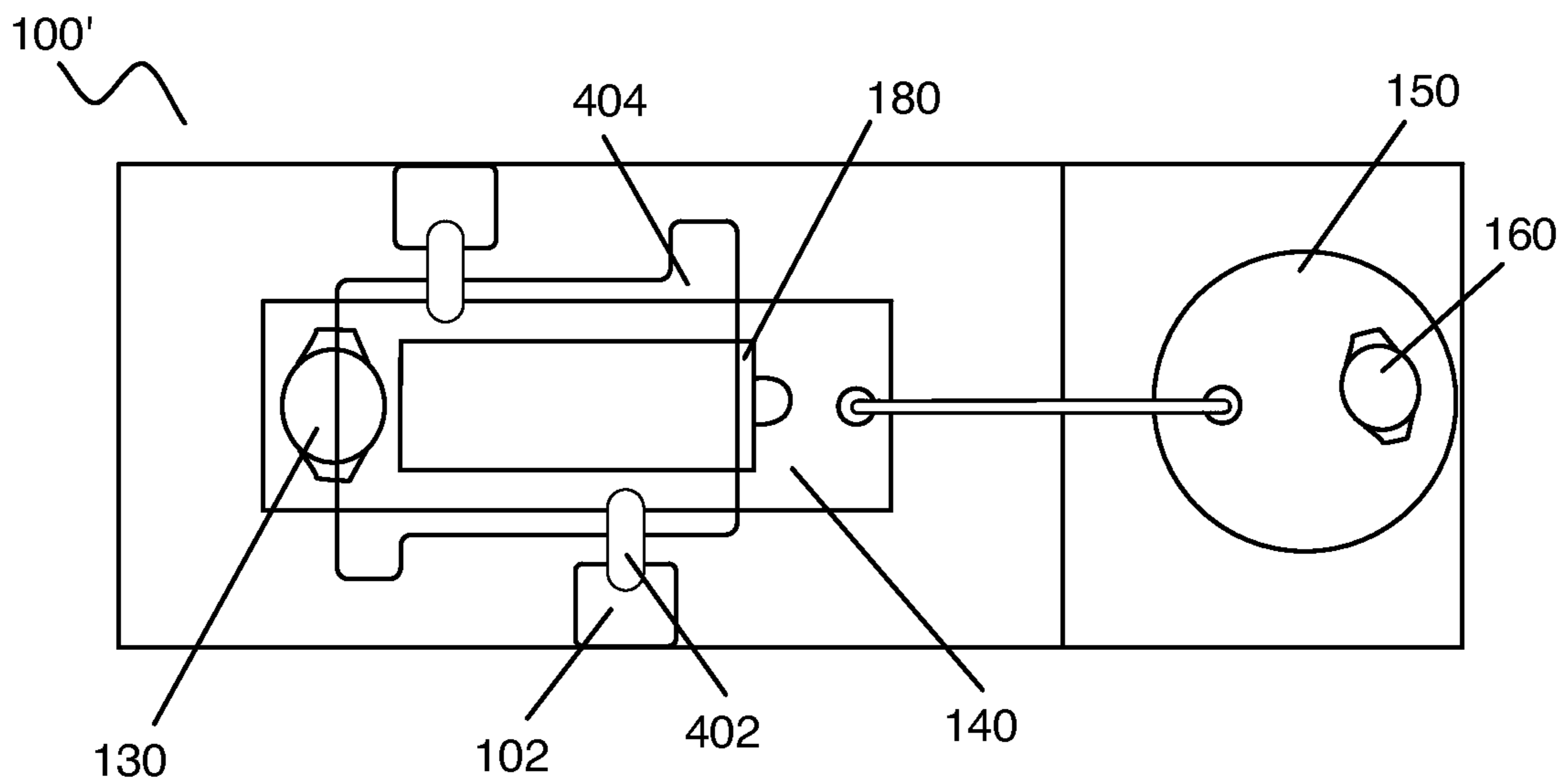
Top View
