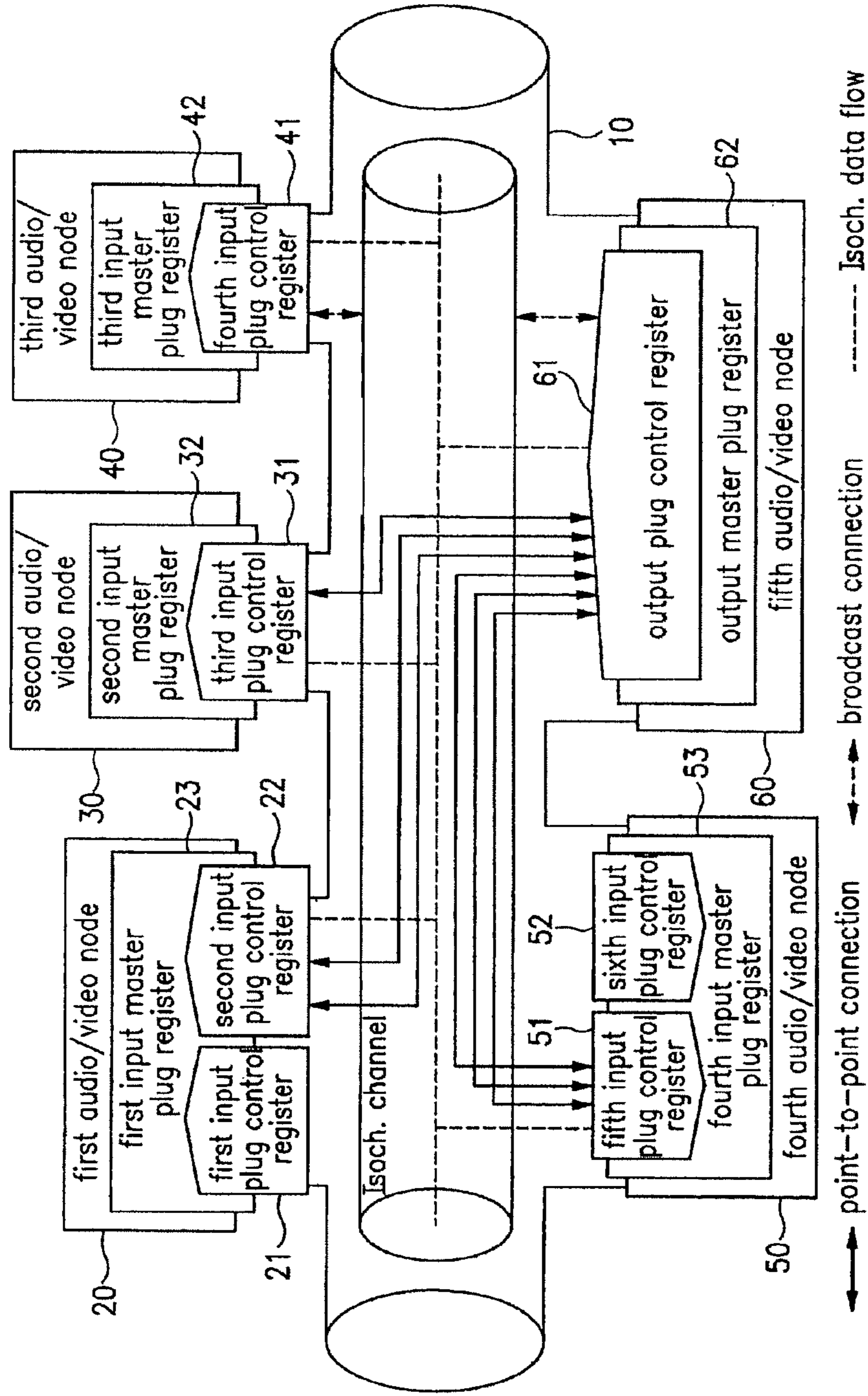
FIG. 1 Related Art
