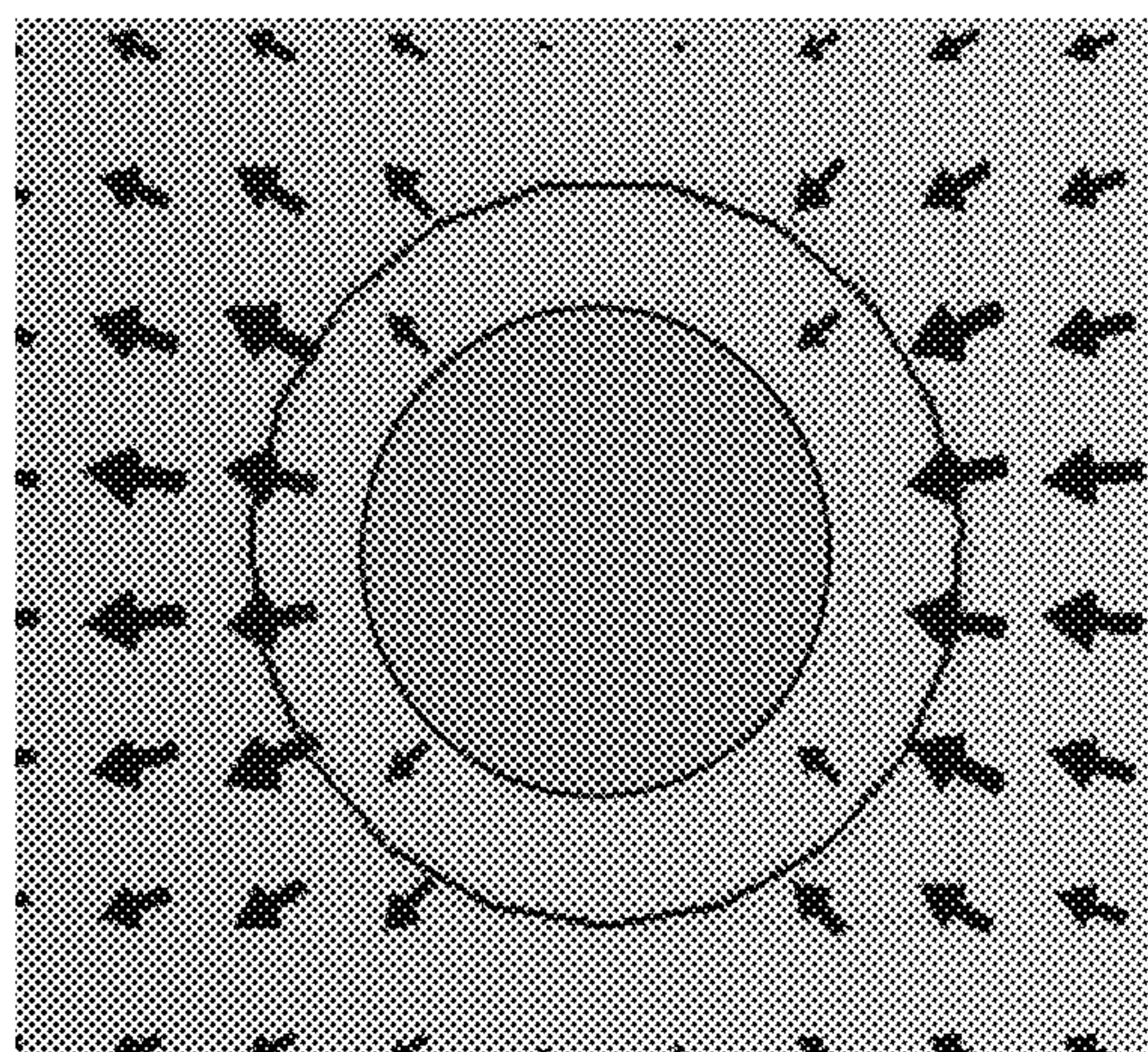
Conductor mode (HE11) 2057
