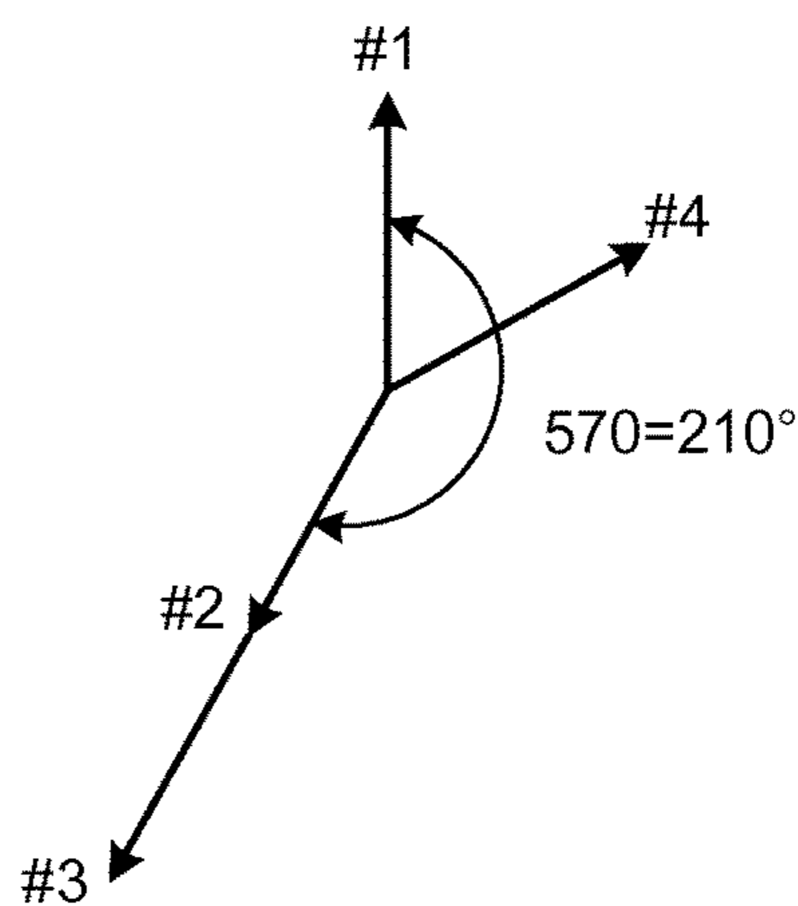
(f) NINETEENTH ORDER COMPONENT
