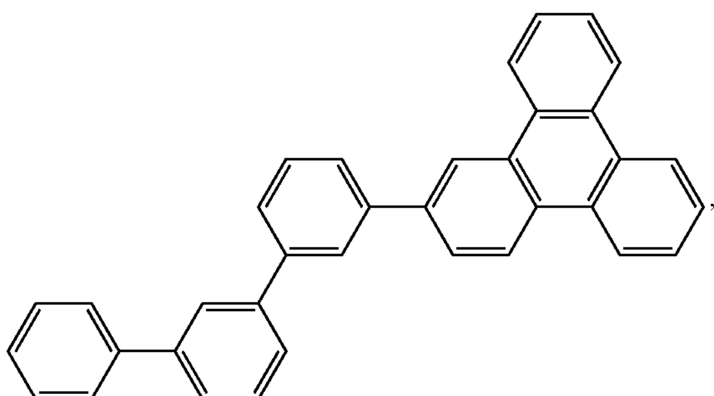
Compound 2
