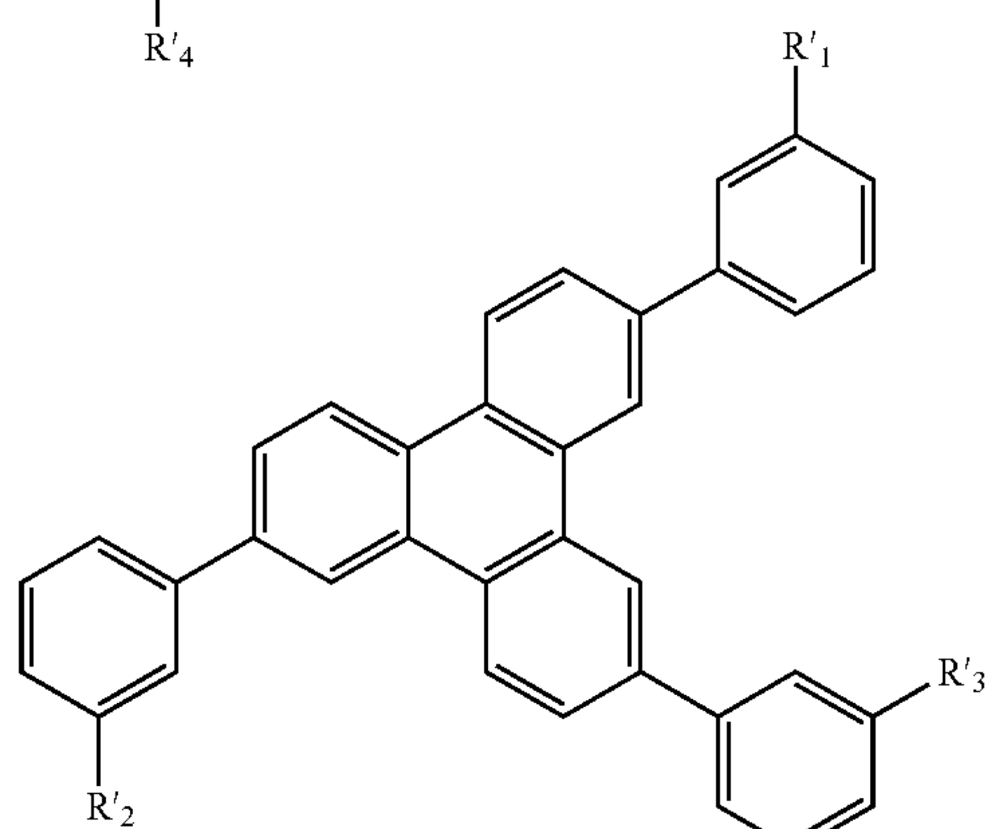
Substructure M
