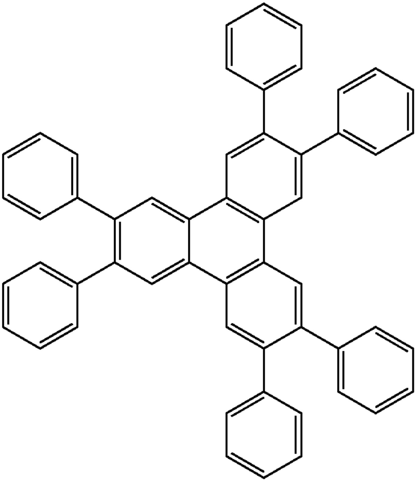
HPT
