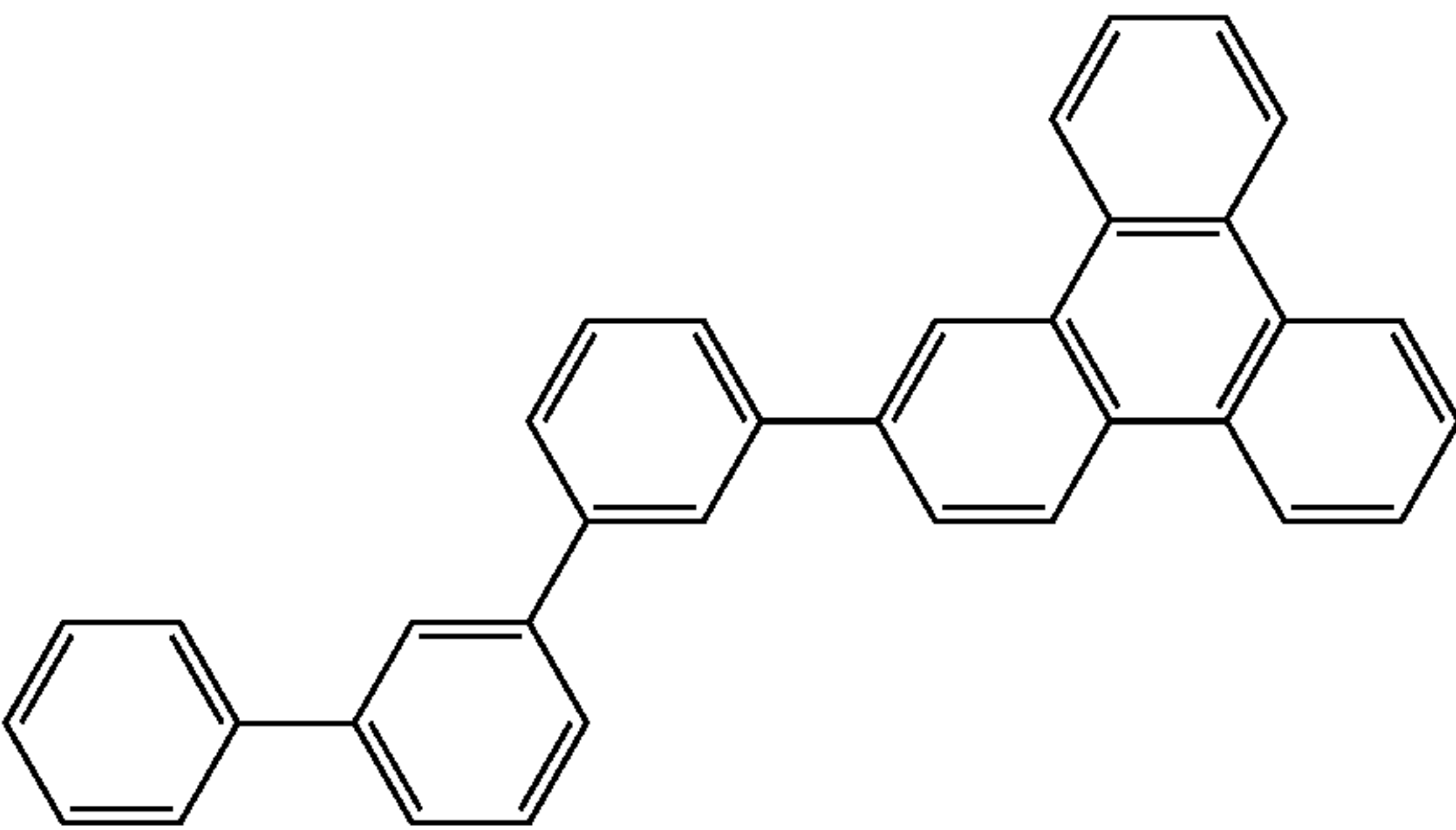
Compound 2
