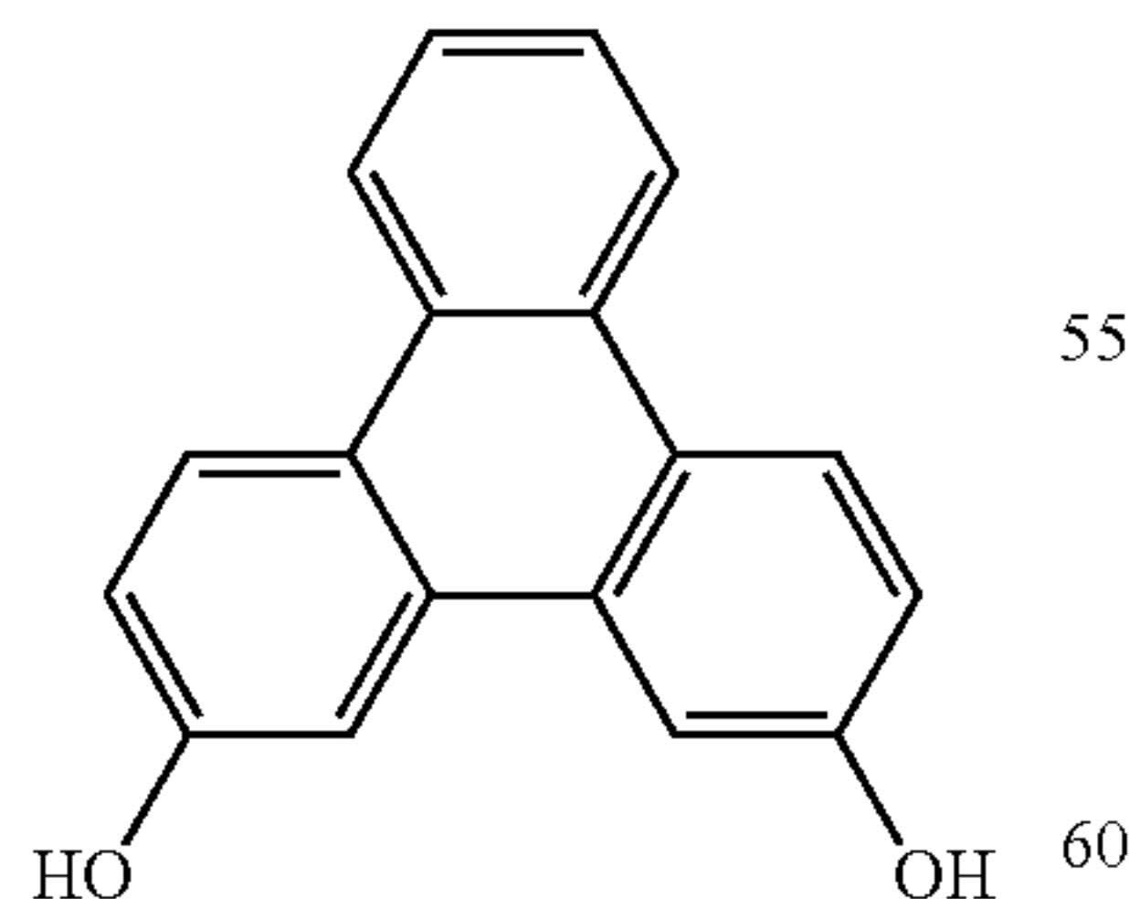
Triphenylene-2,11-diol
