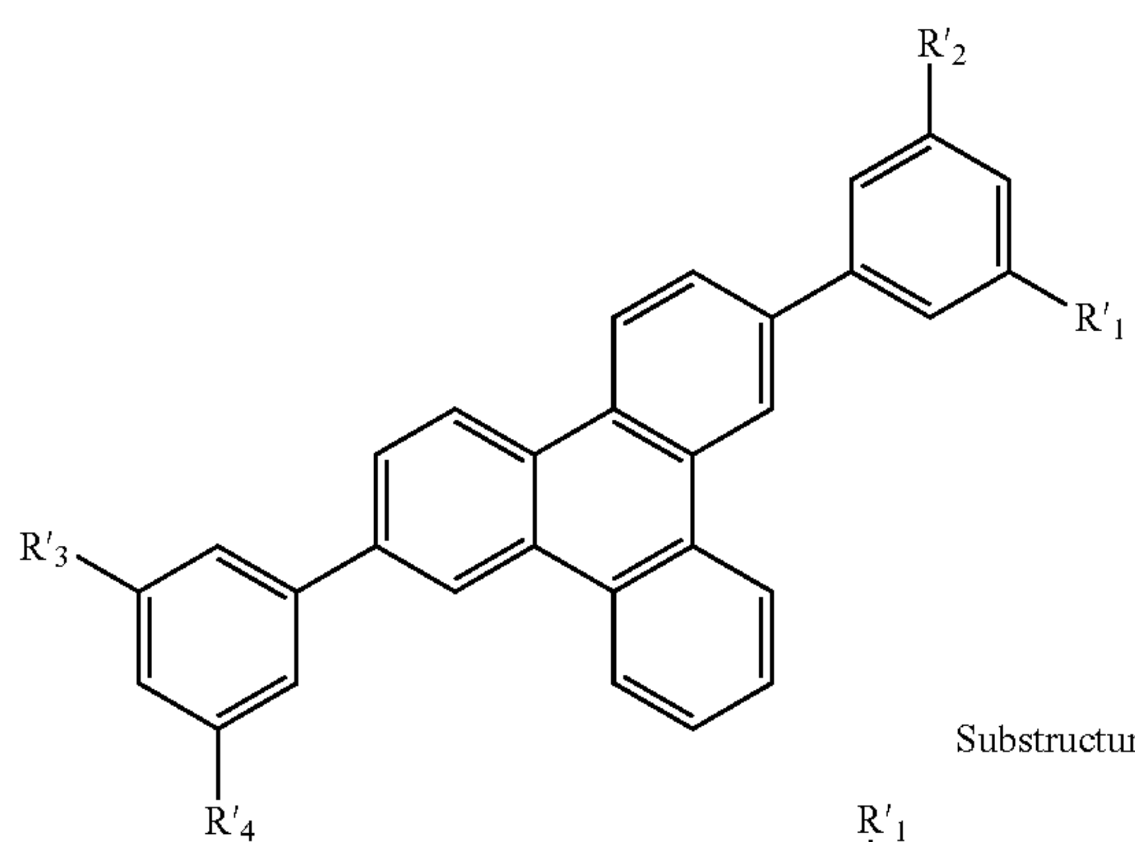
Substructure K
