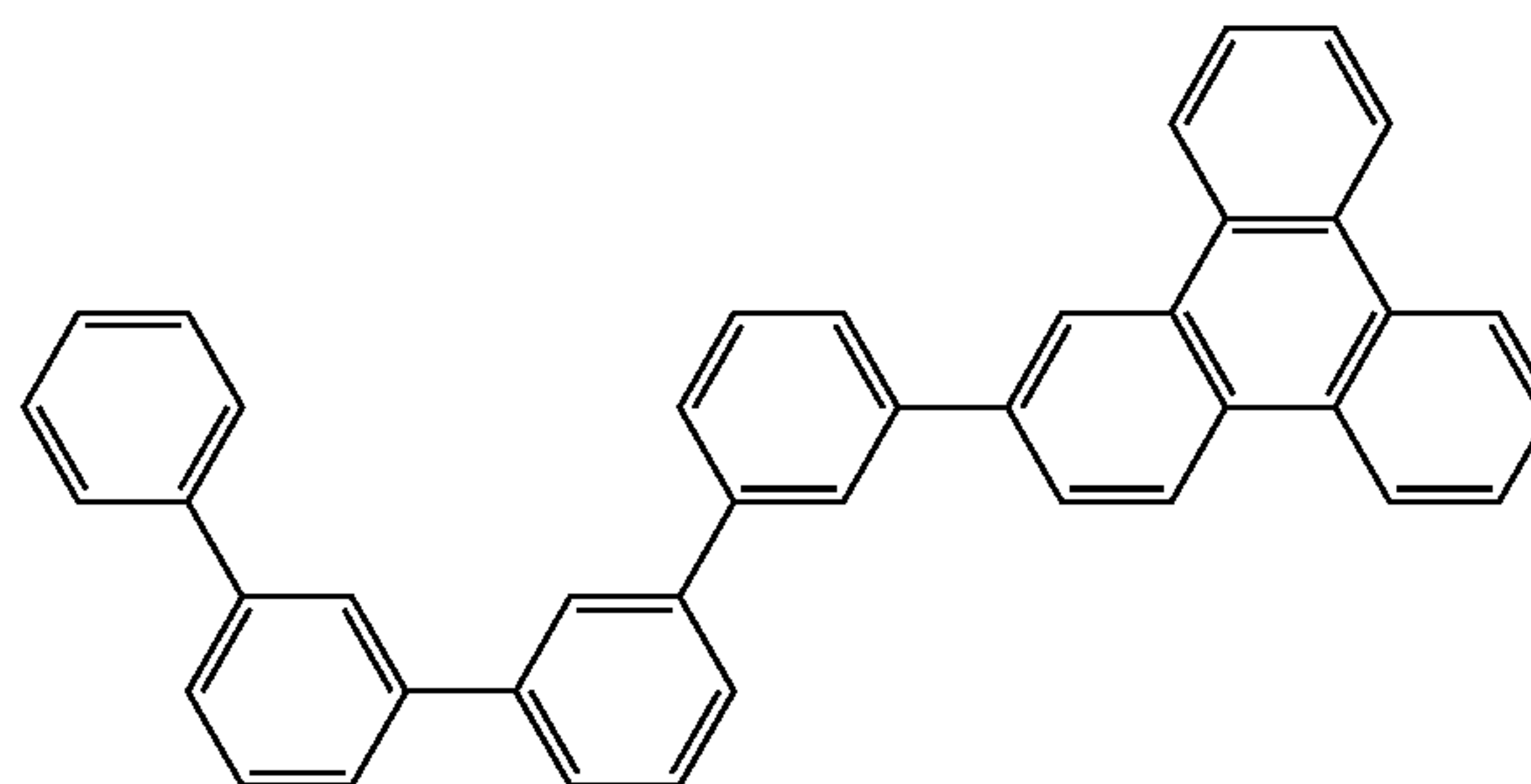
Compound 3
