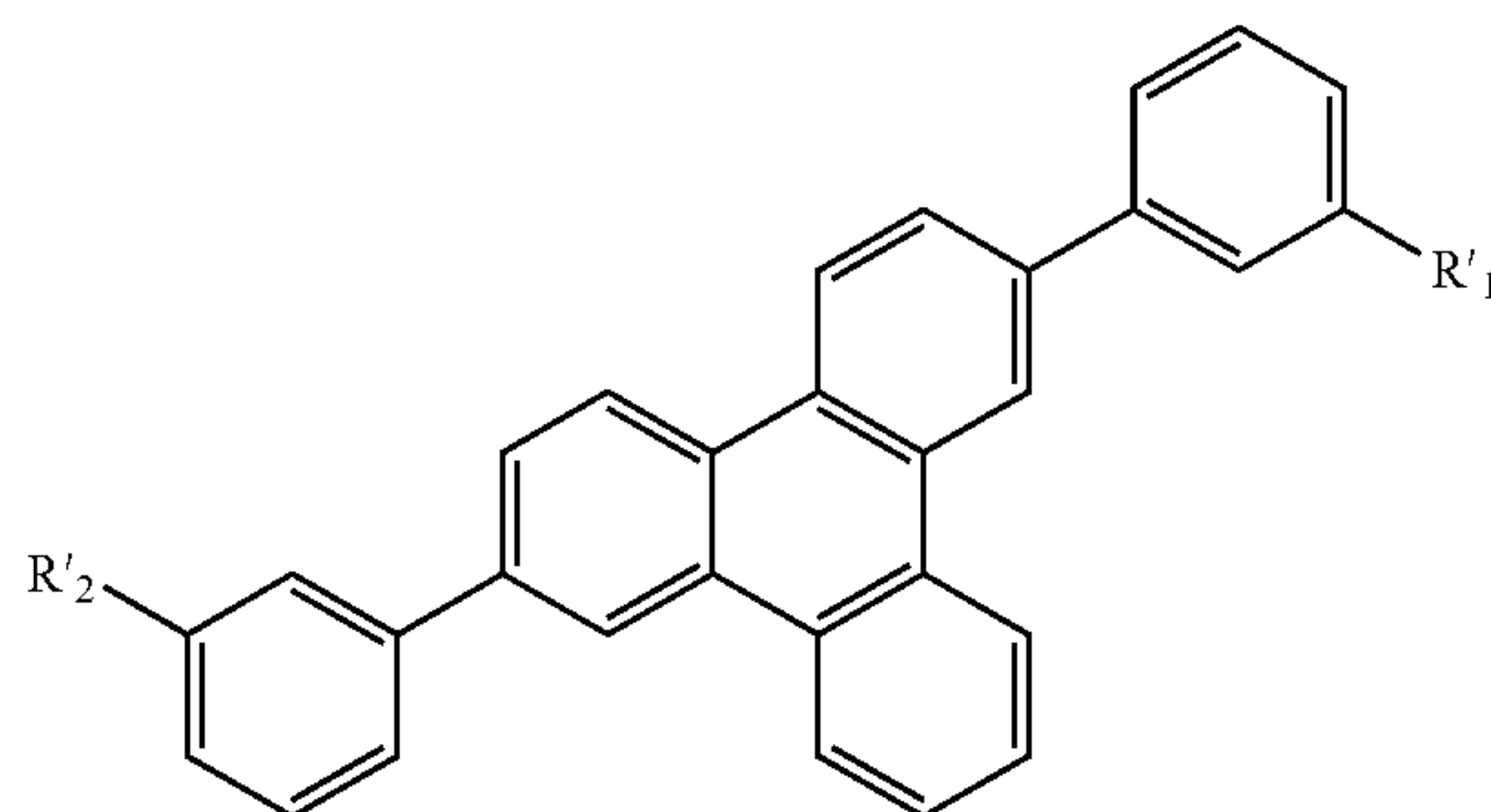
Substructure J
