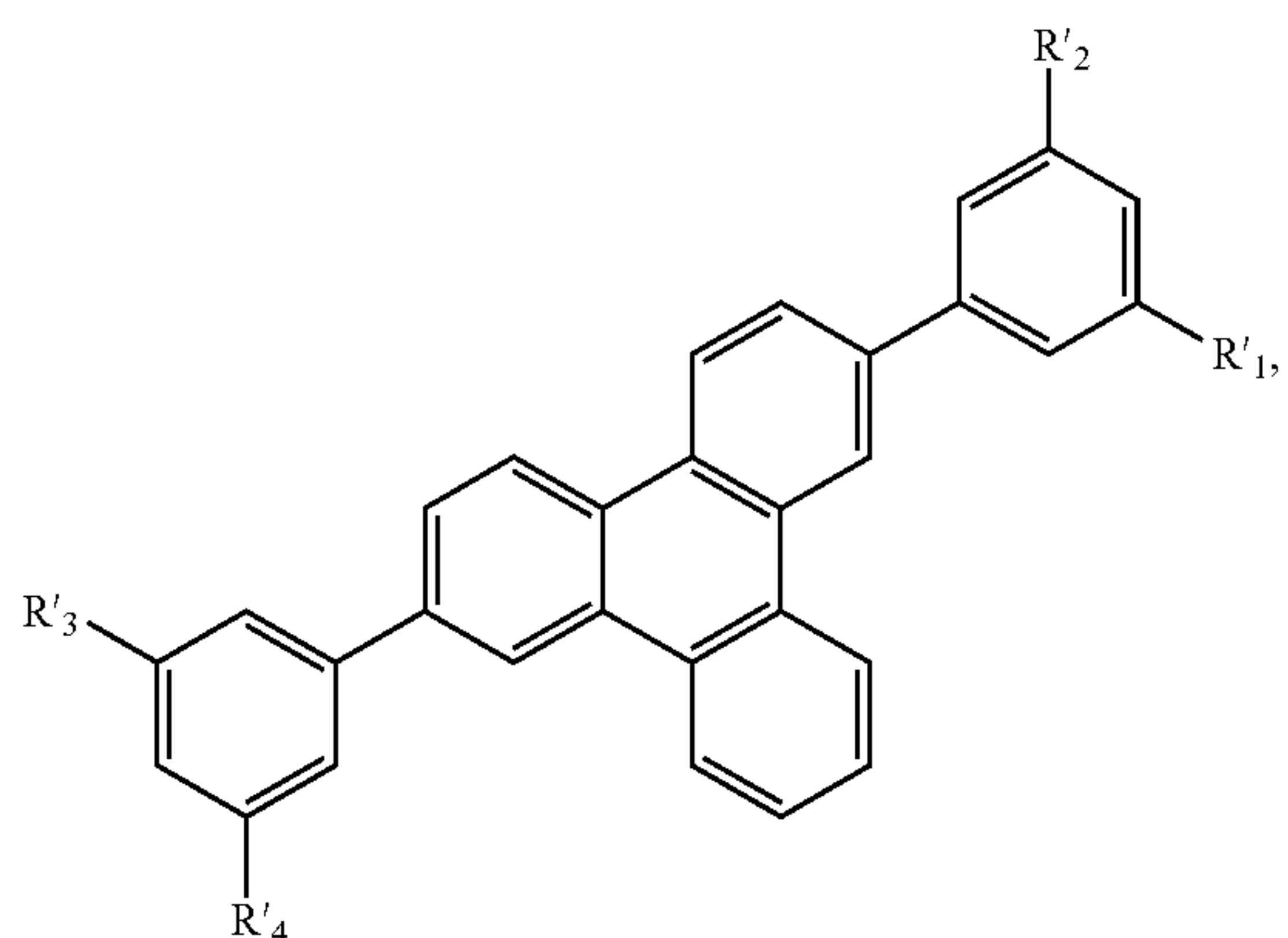
Substructure L
