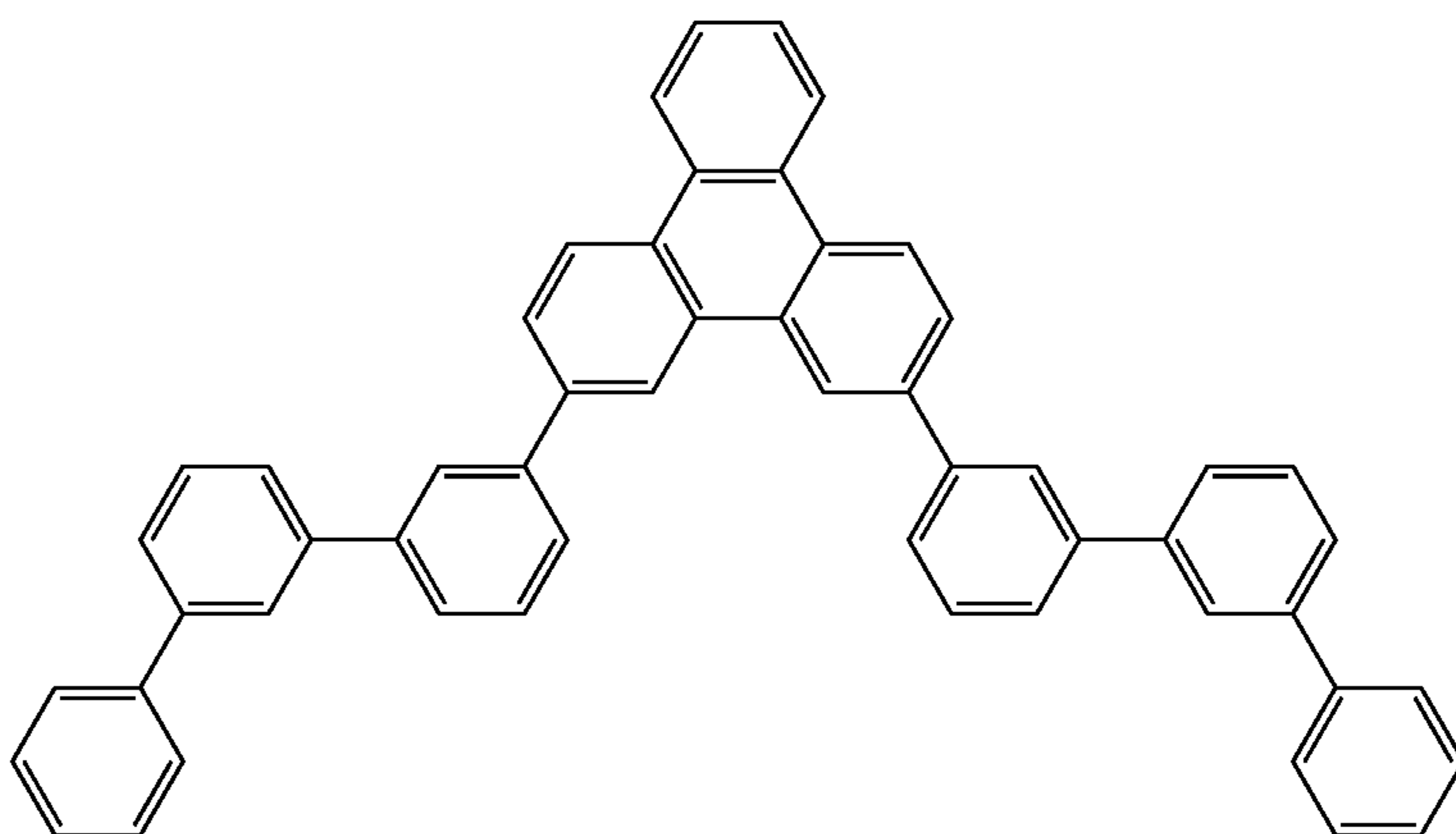
Compound 9
