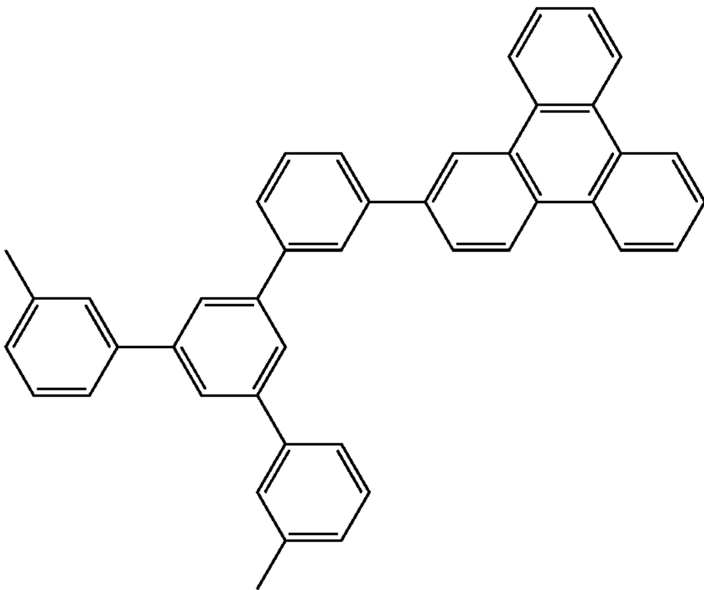
Compound 10
