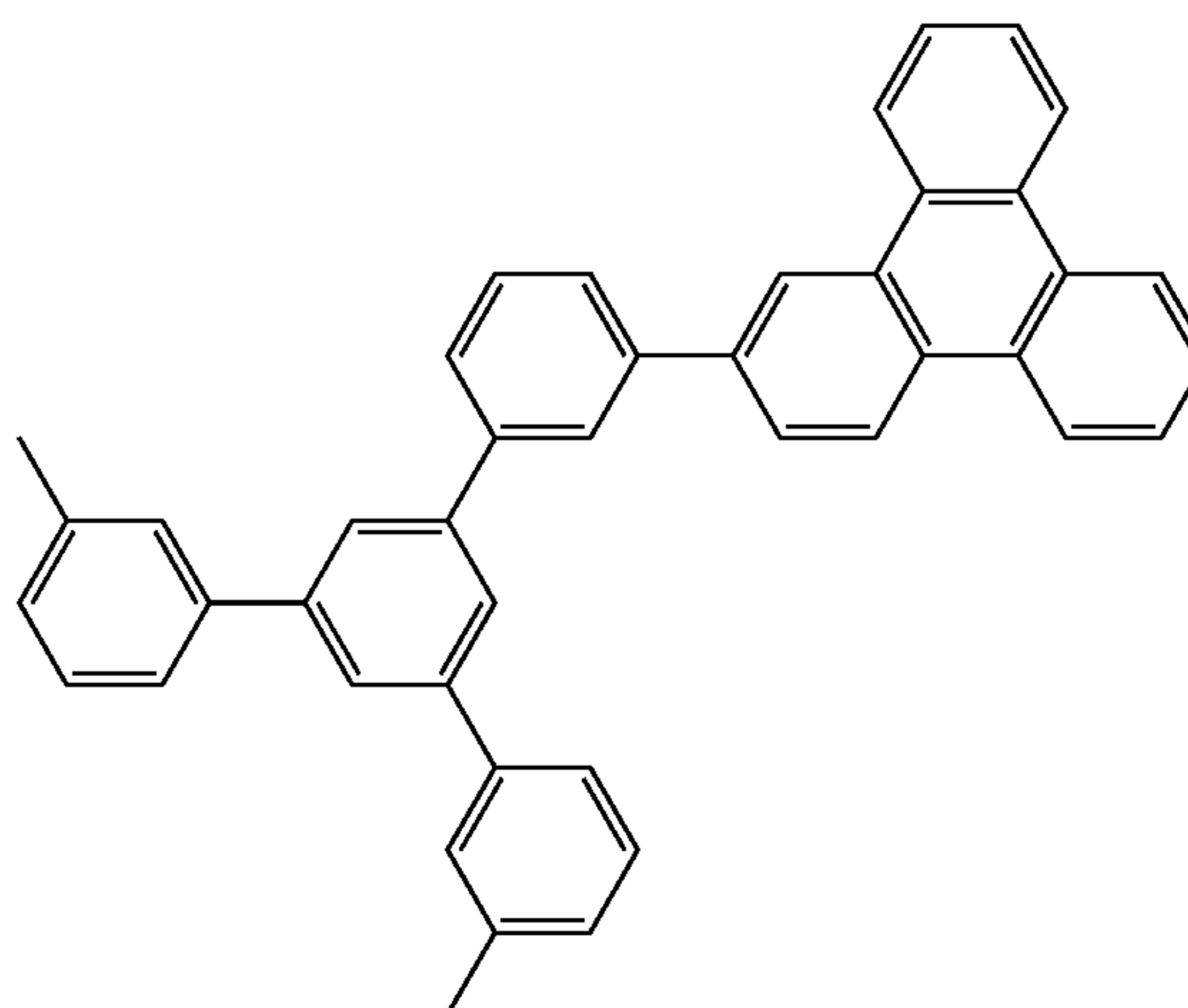
Compound 10
