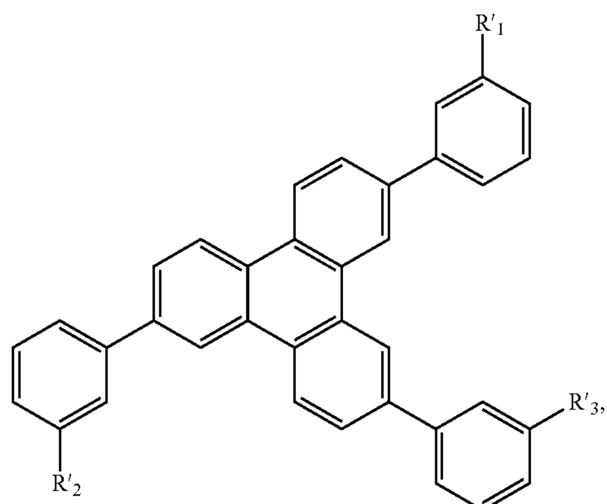
Substructure M
