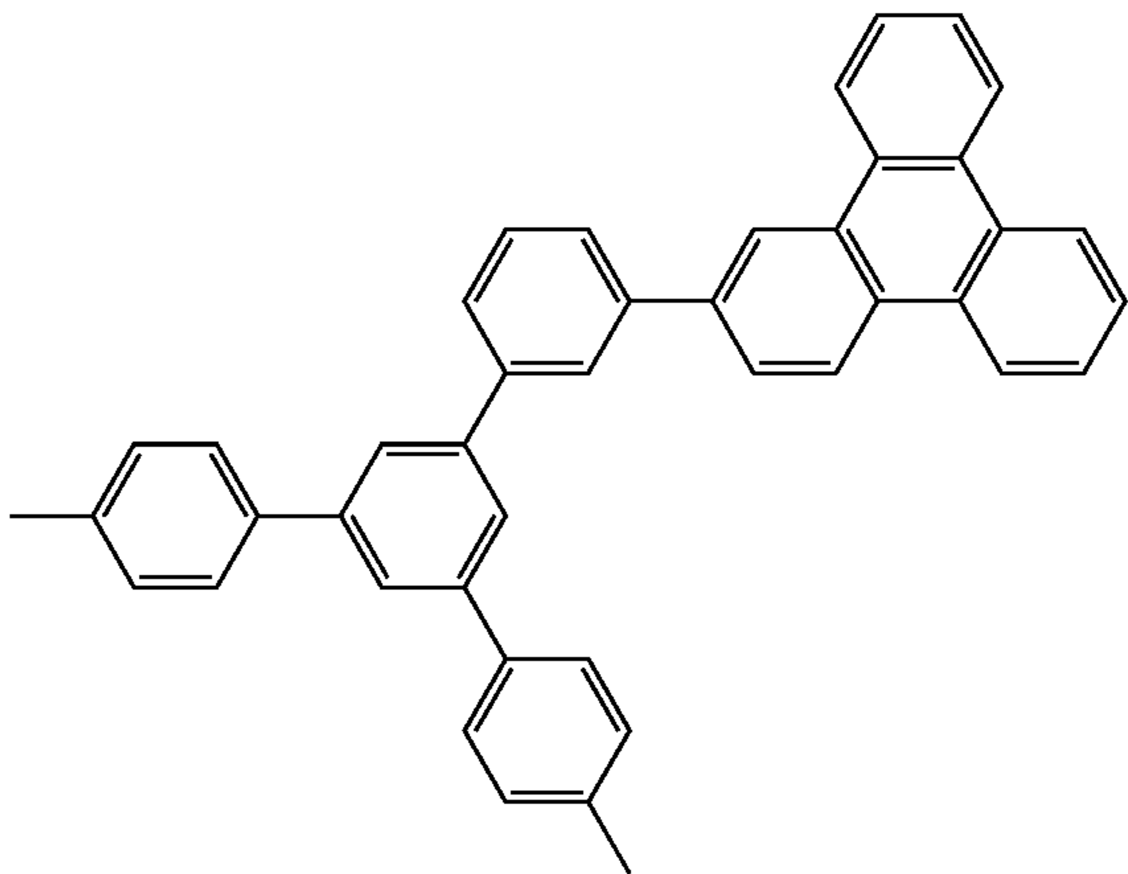
Compound 9
