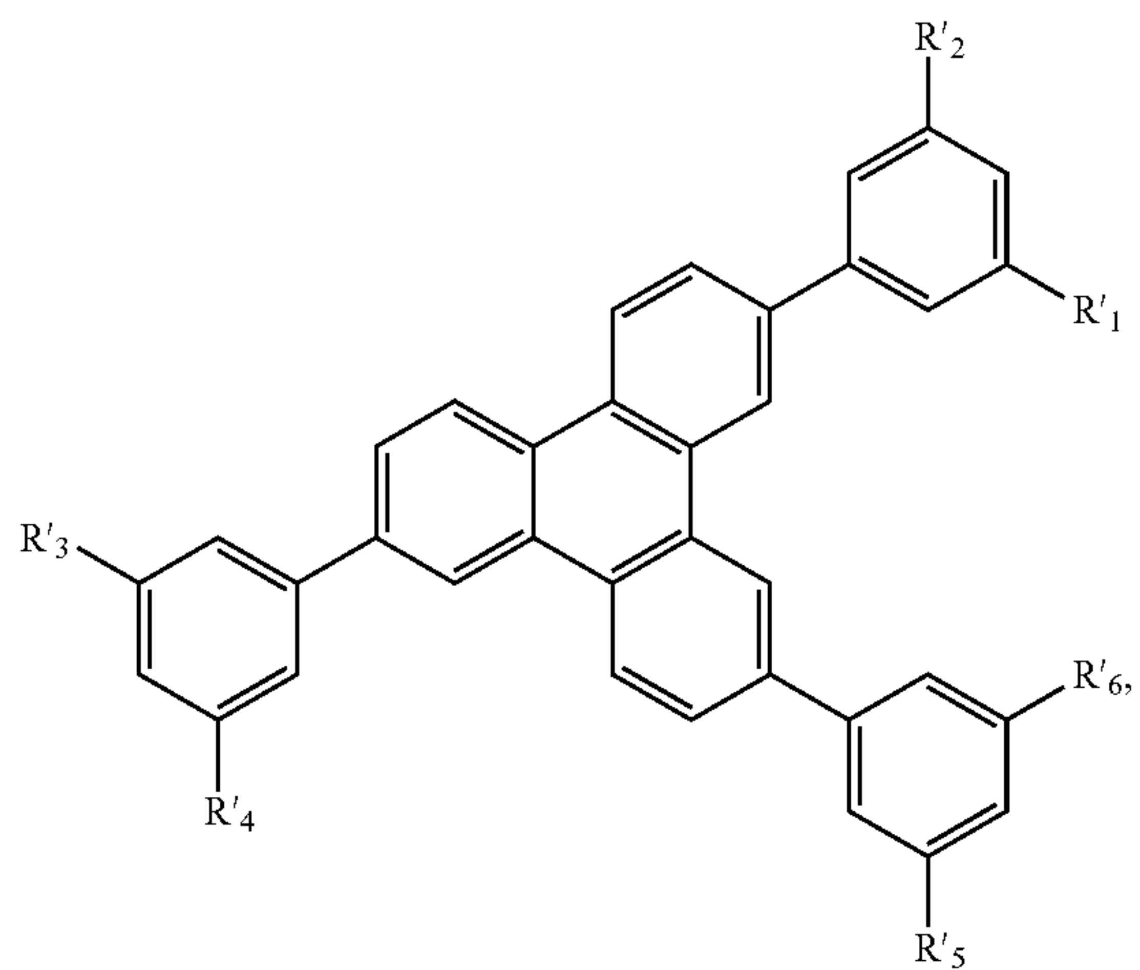
Substructure M
