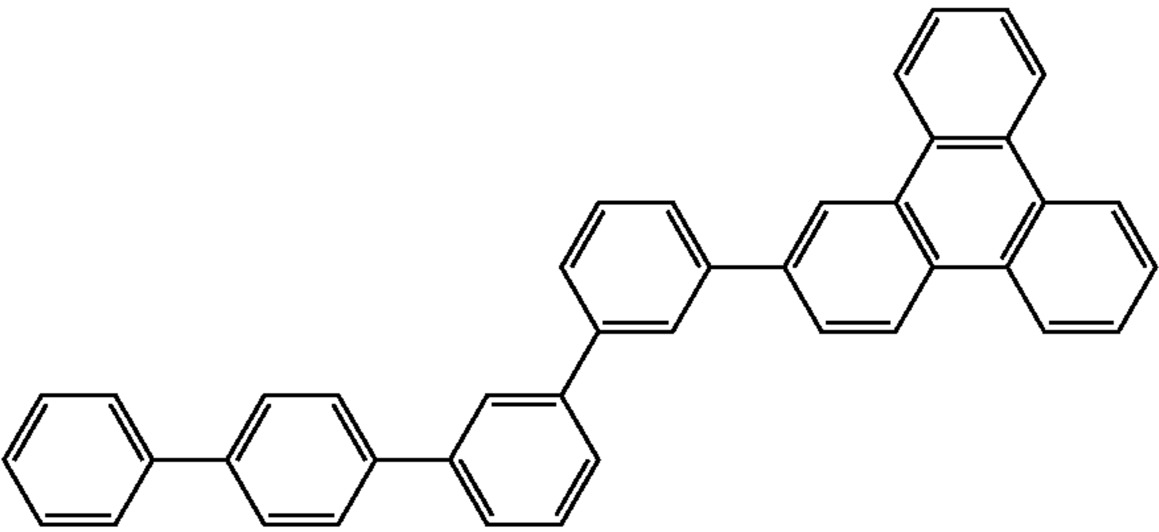
Compound 11
