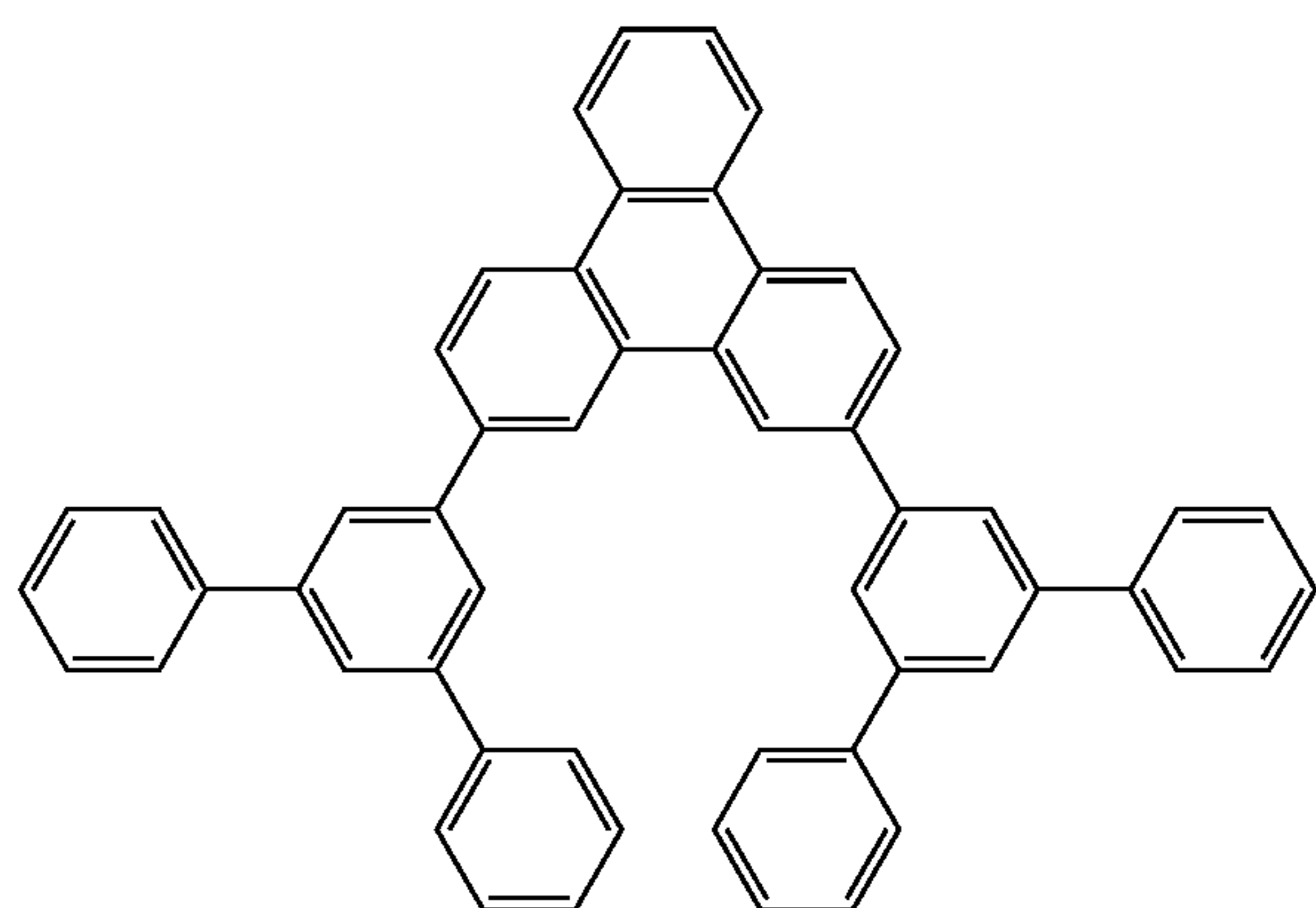
Compound 7
