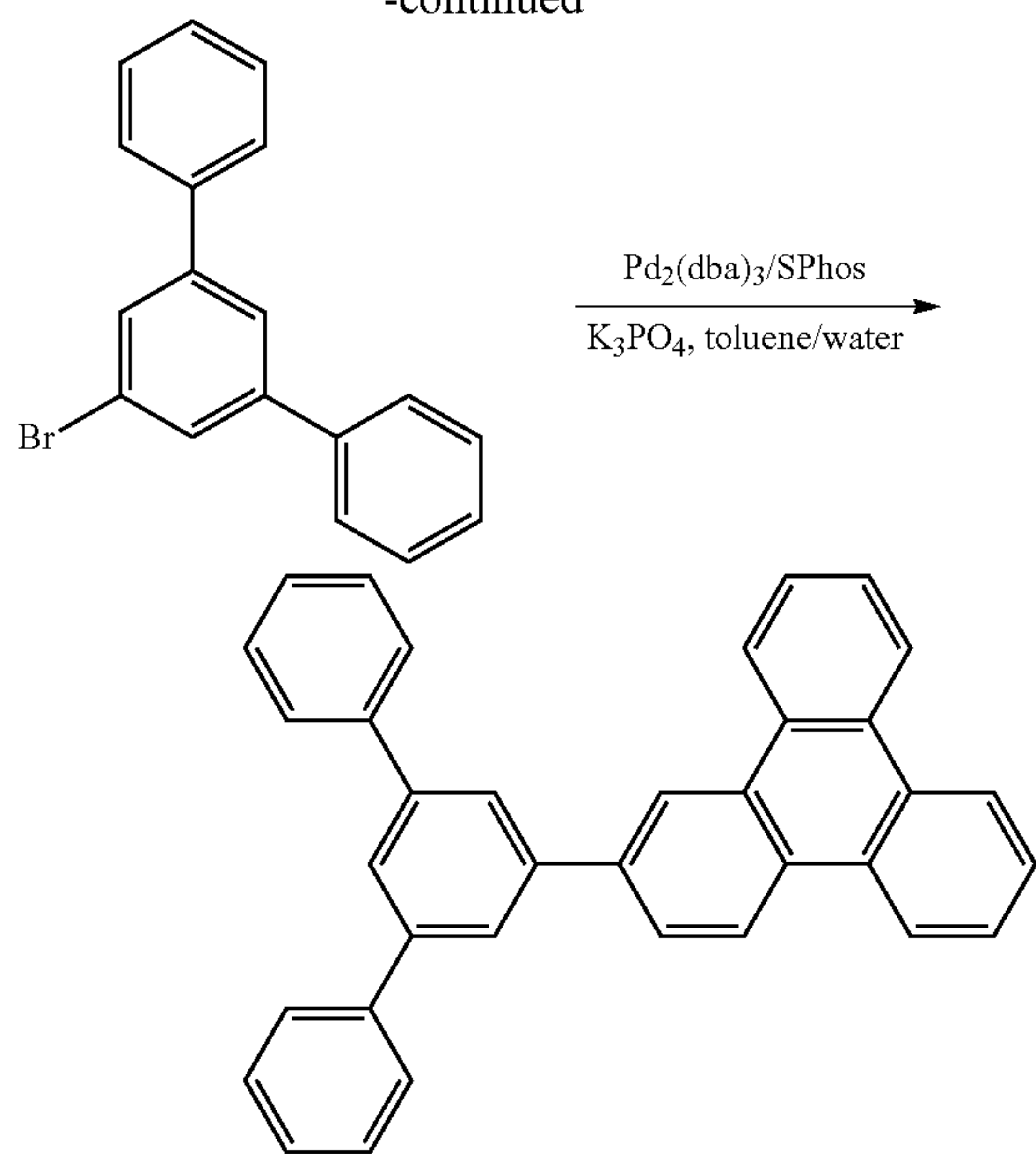
Compound 1
