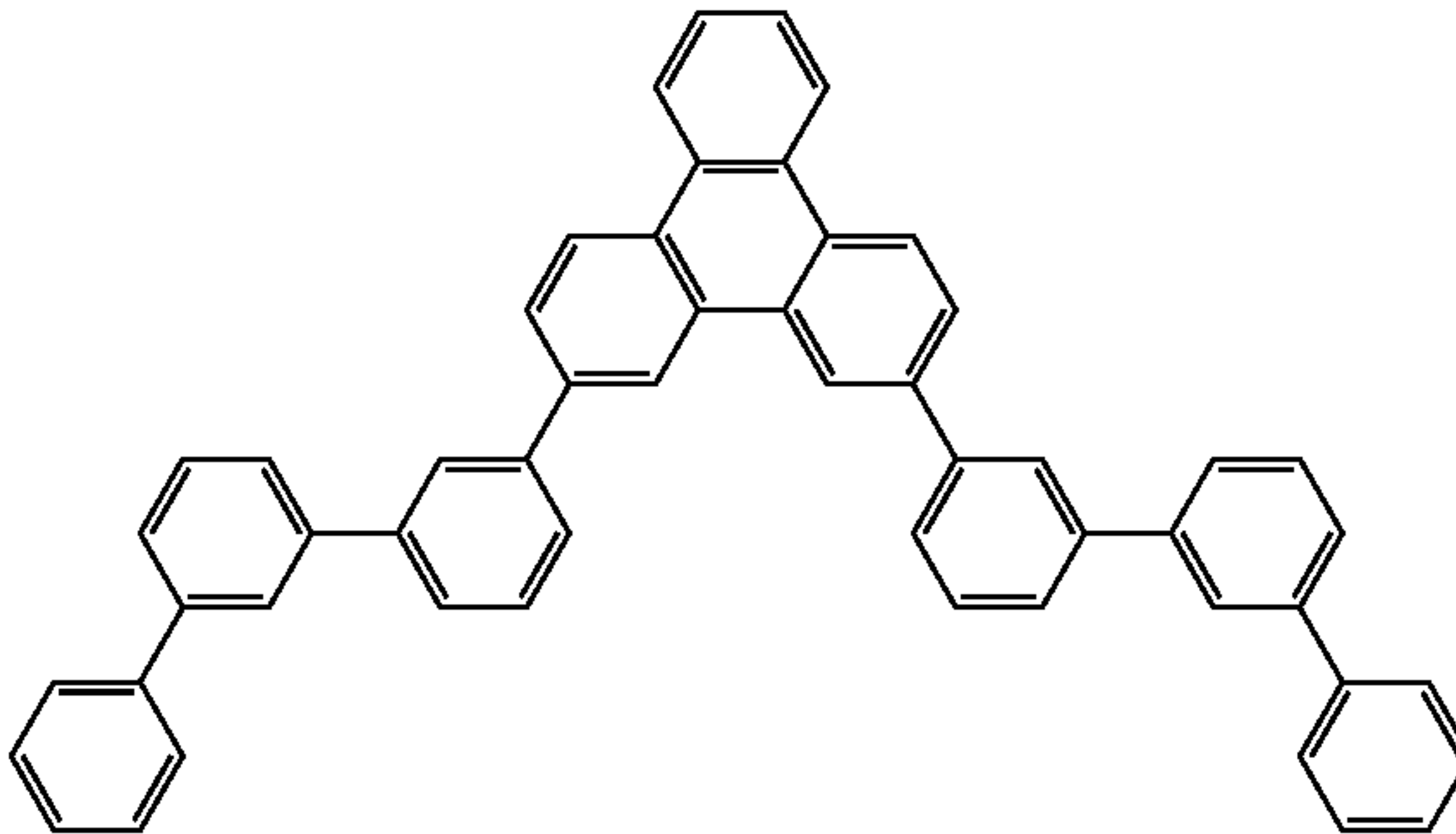
Compound 8
