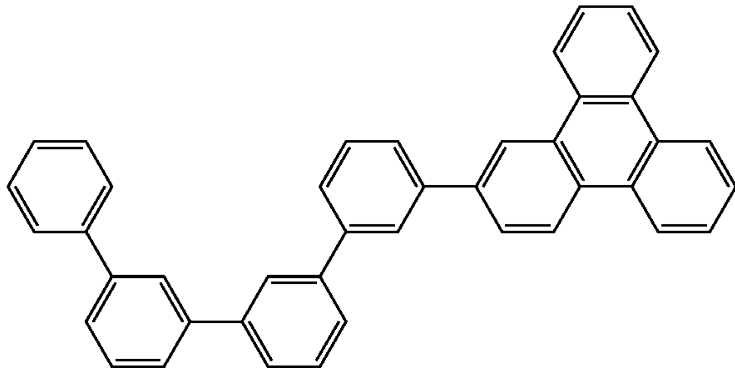
Compound 3
