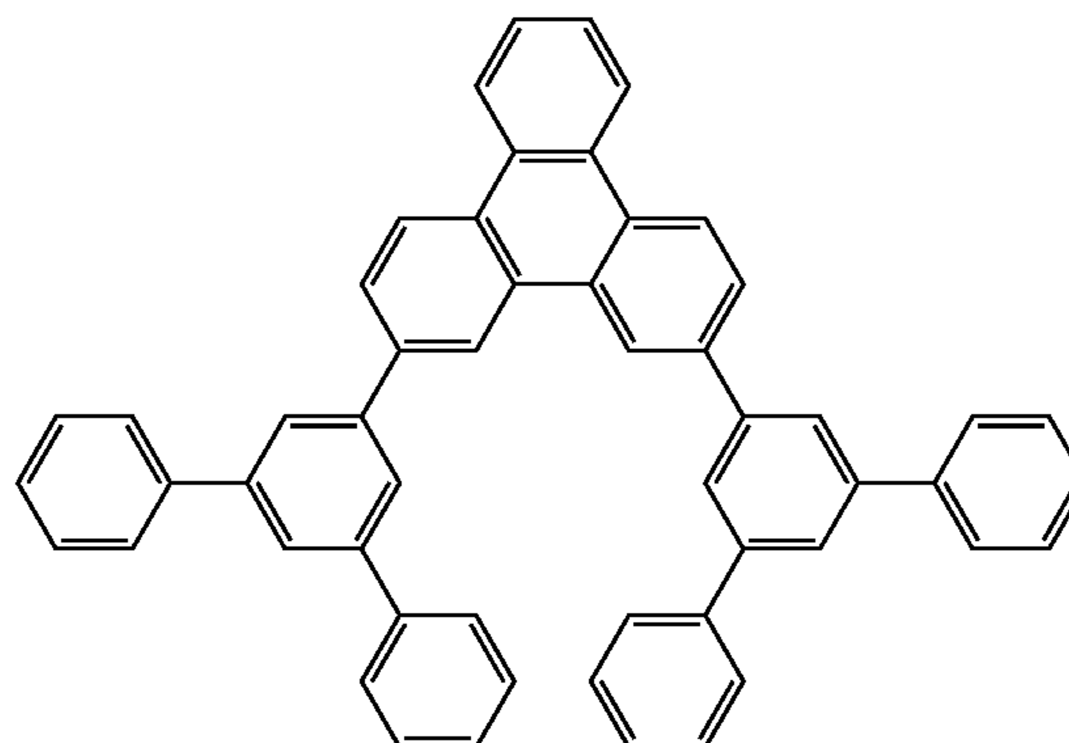
Compound 7
