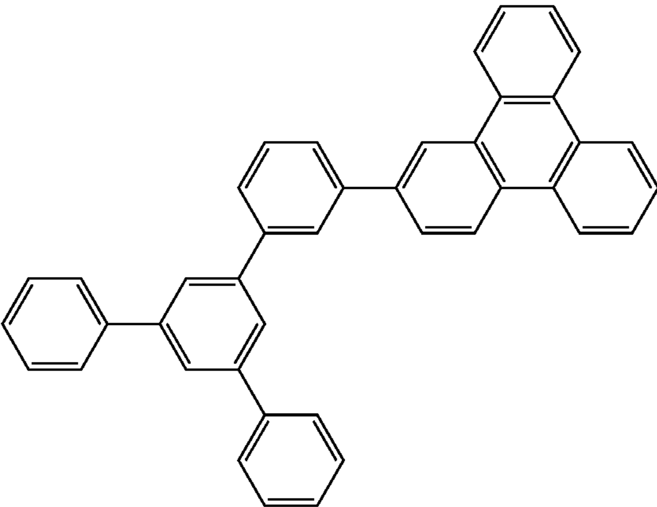
Compound 4
