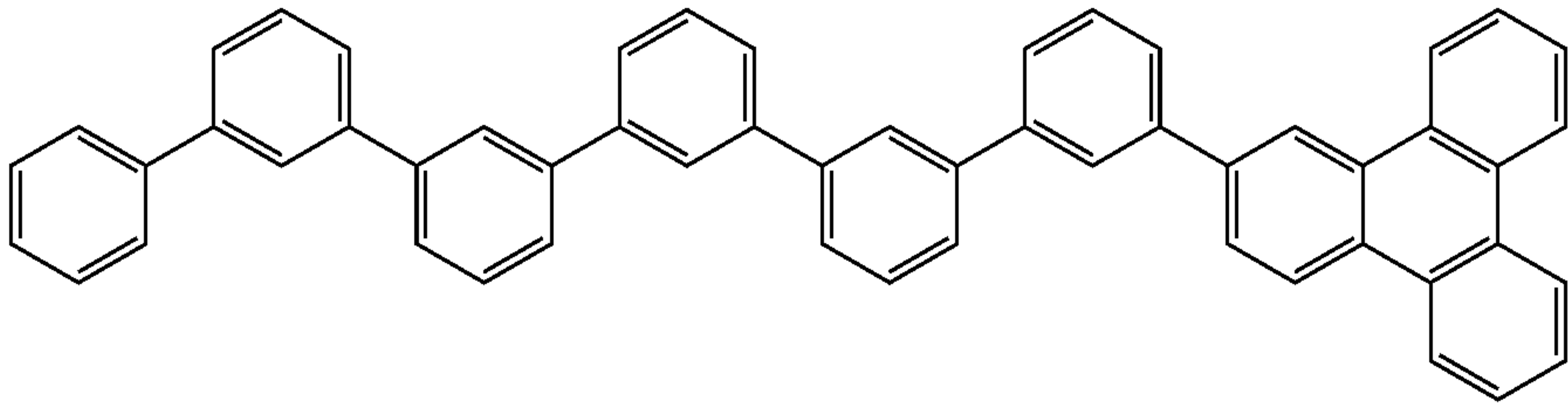
Compound 6
