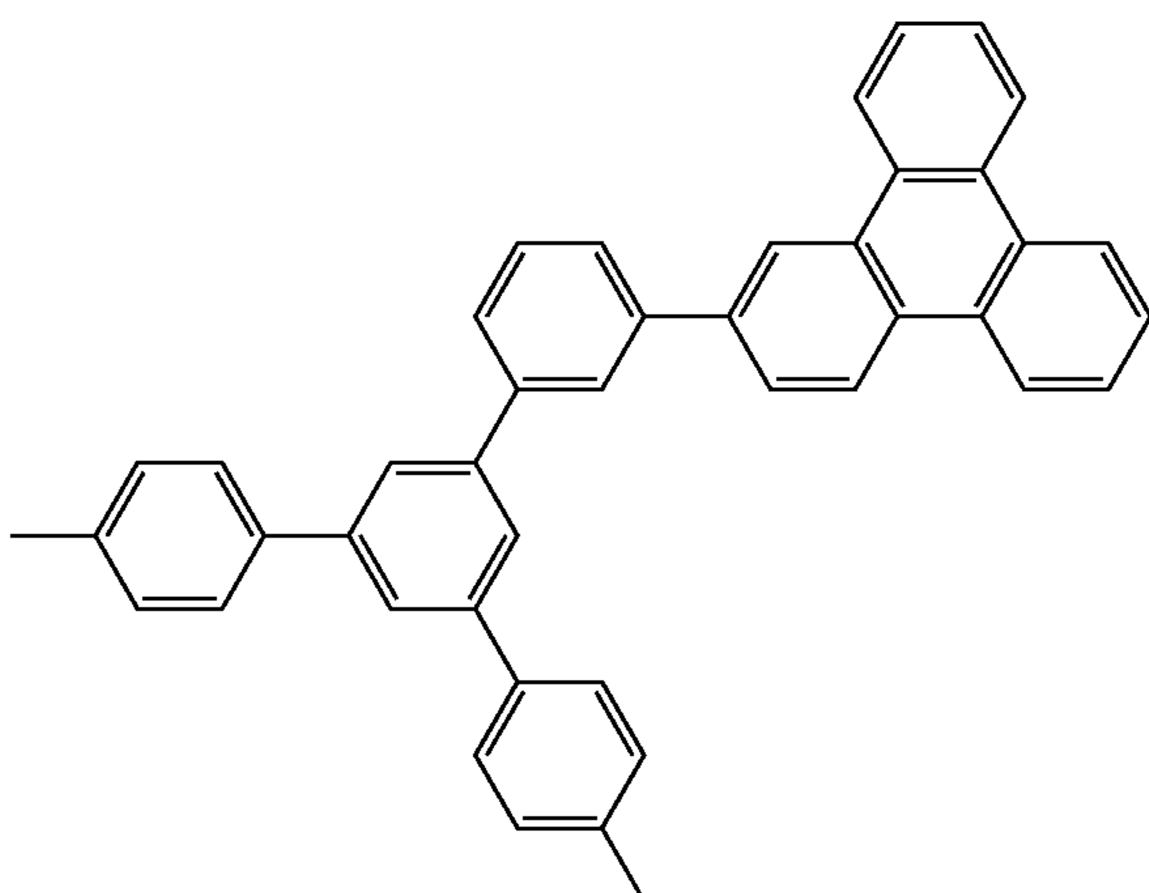
Compound 9
