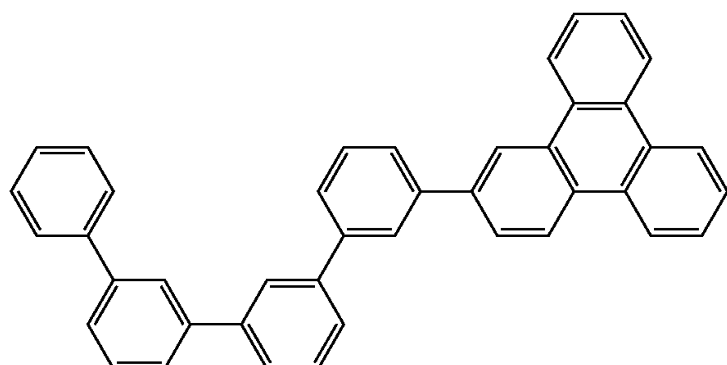
Compound 3
