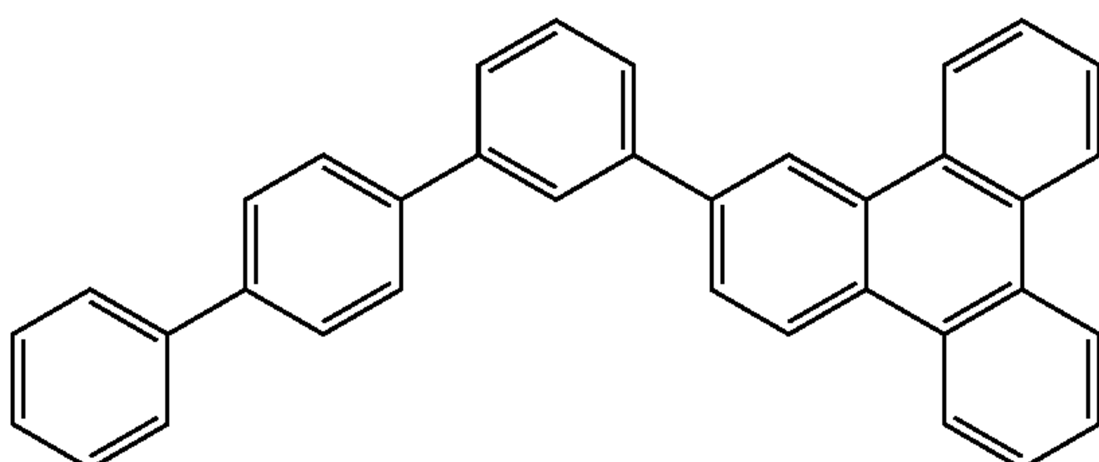
Compound 6
