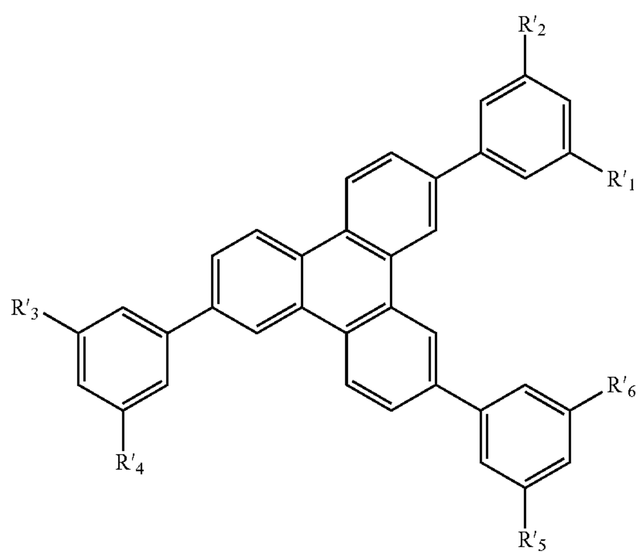
Substructure N
