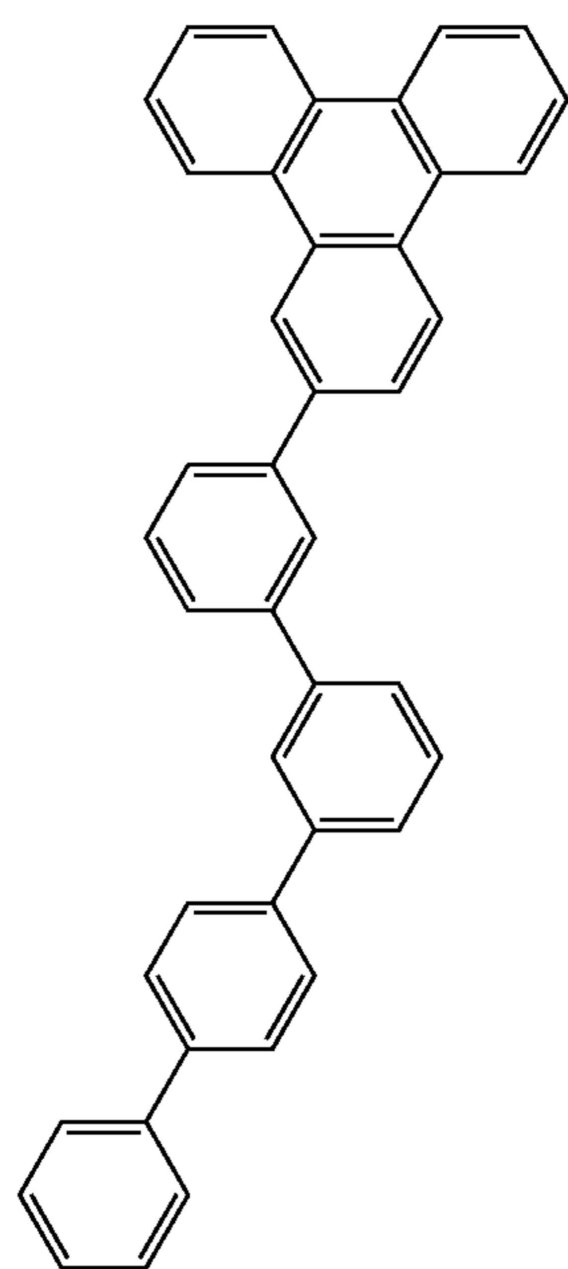
Compound 11
