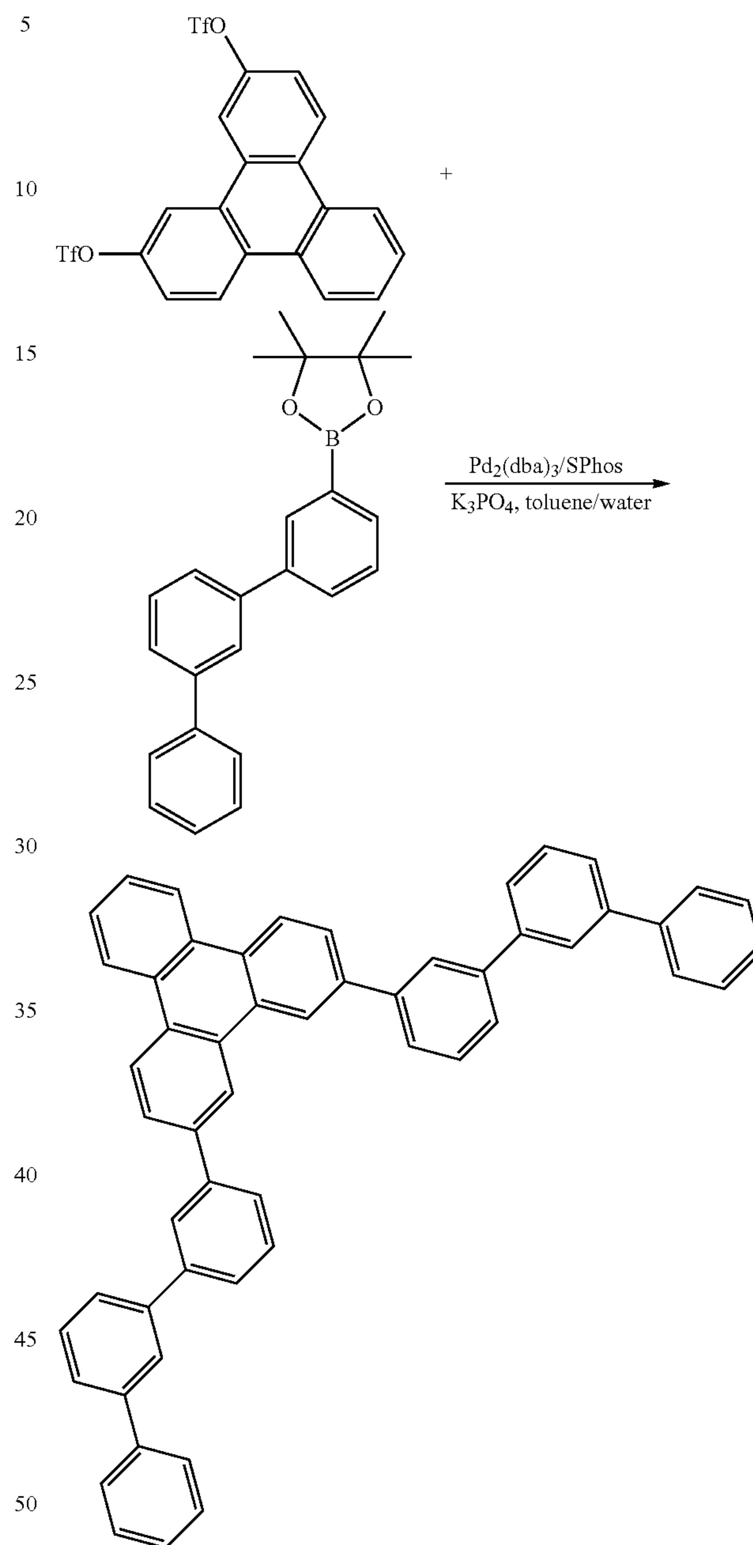
Compound 8
