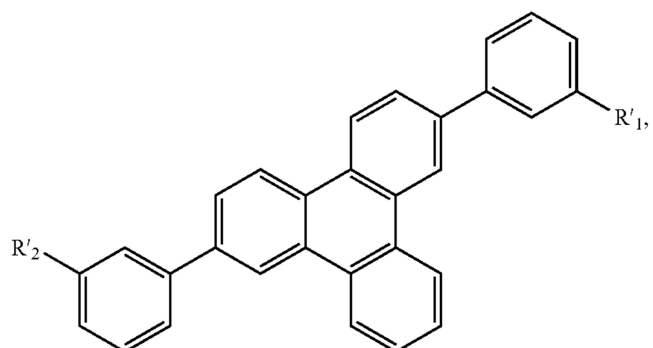
Substructure K
