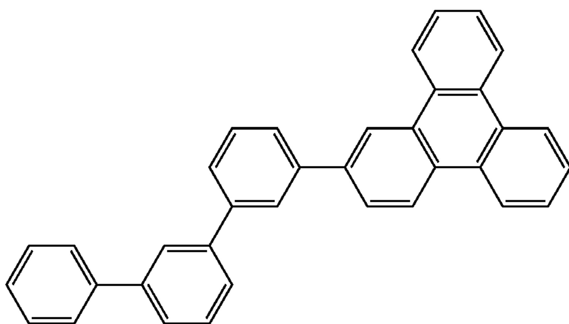
Compound 2
