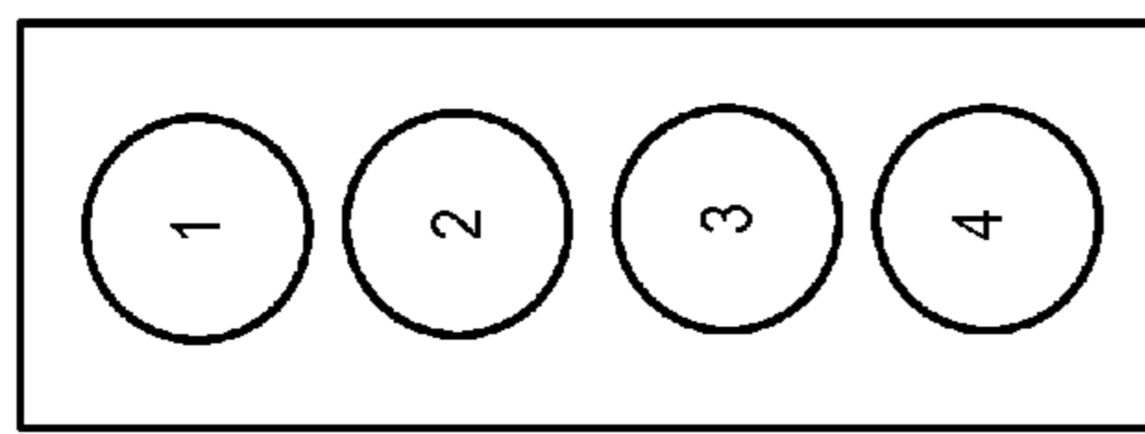
Firing Sequence: 1-3-4-2
