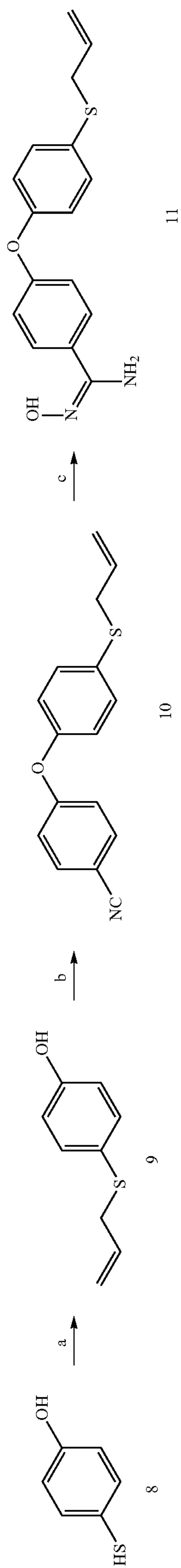
Scheme 1. Syntheses of the inhibitors 4, 5, 6 and 7 a .
