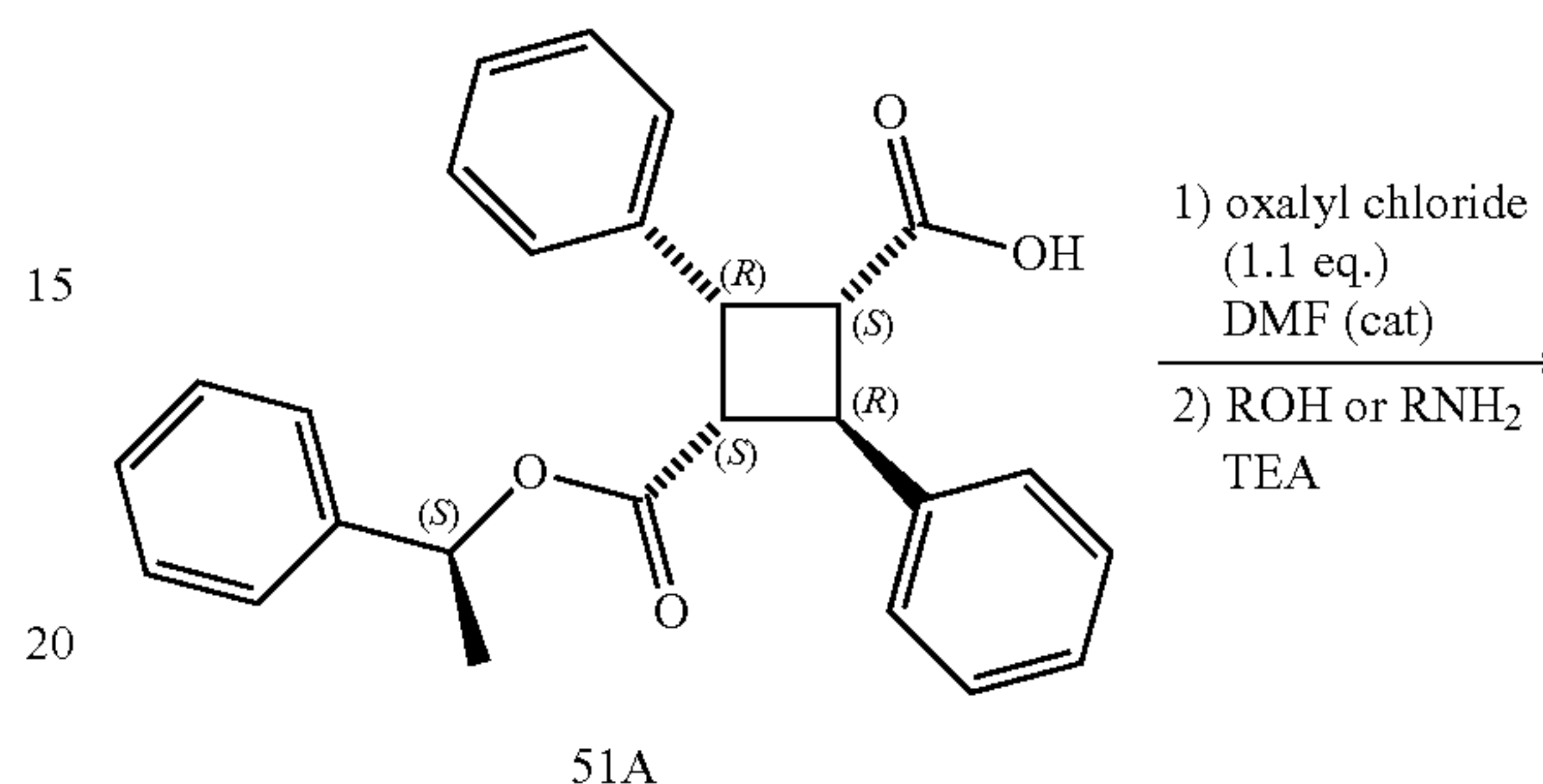
Scheme 7.
