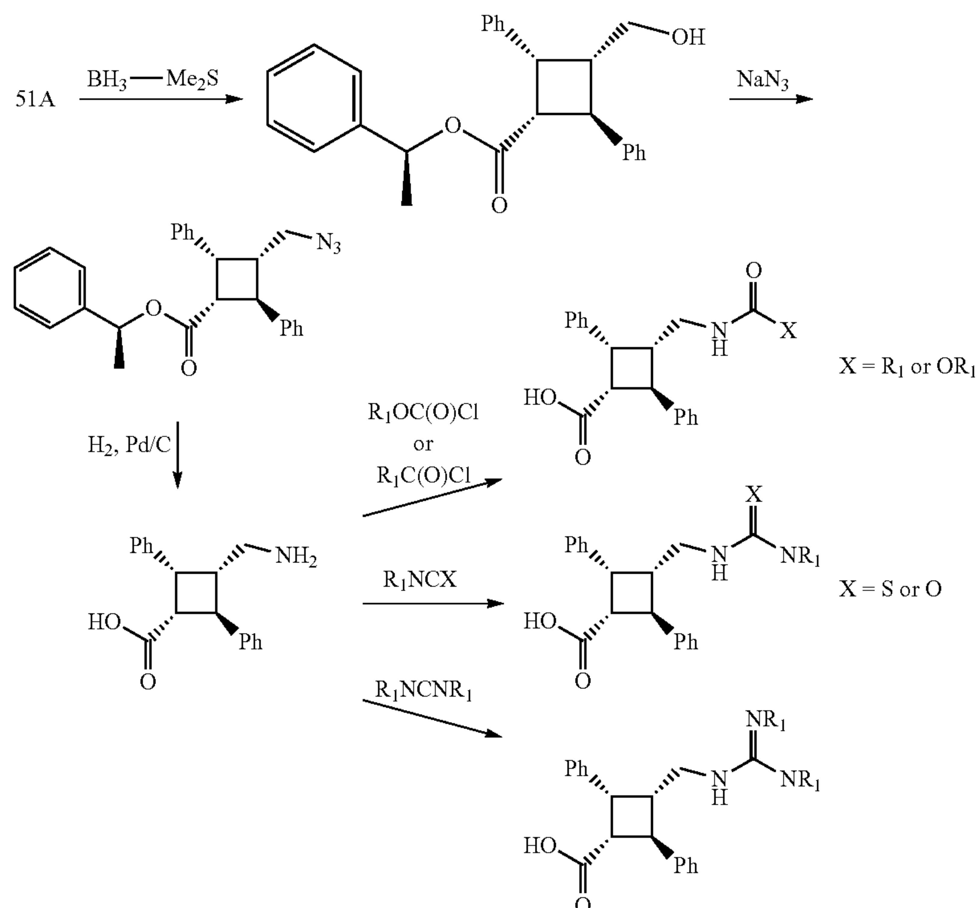
Scheme 10.
