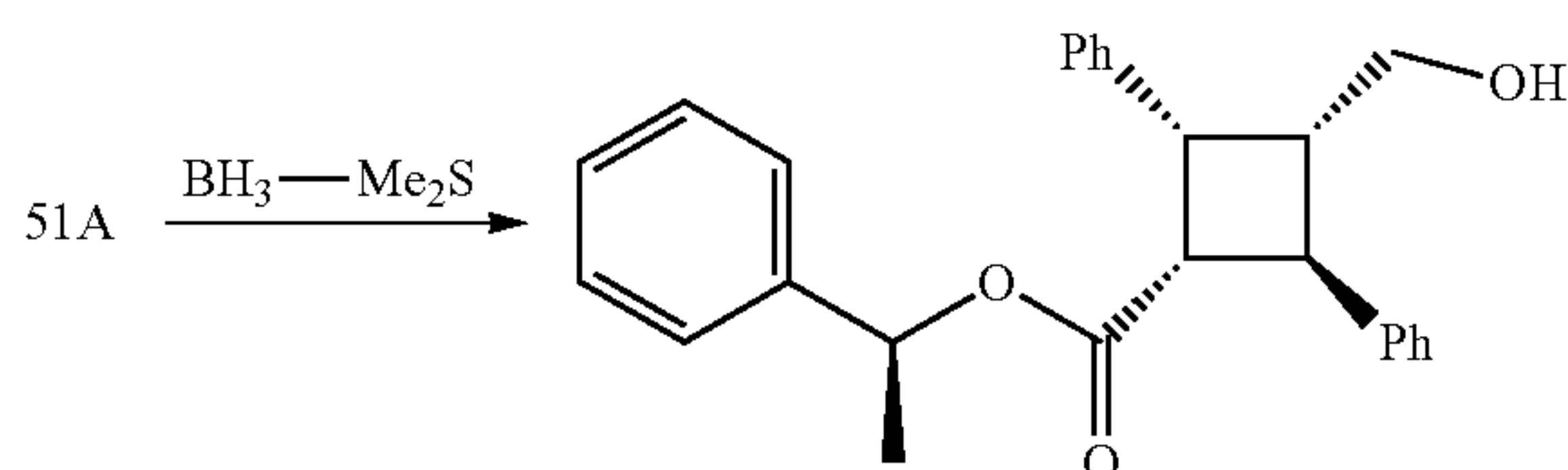
Scheme 8.
