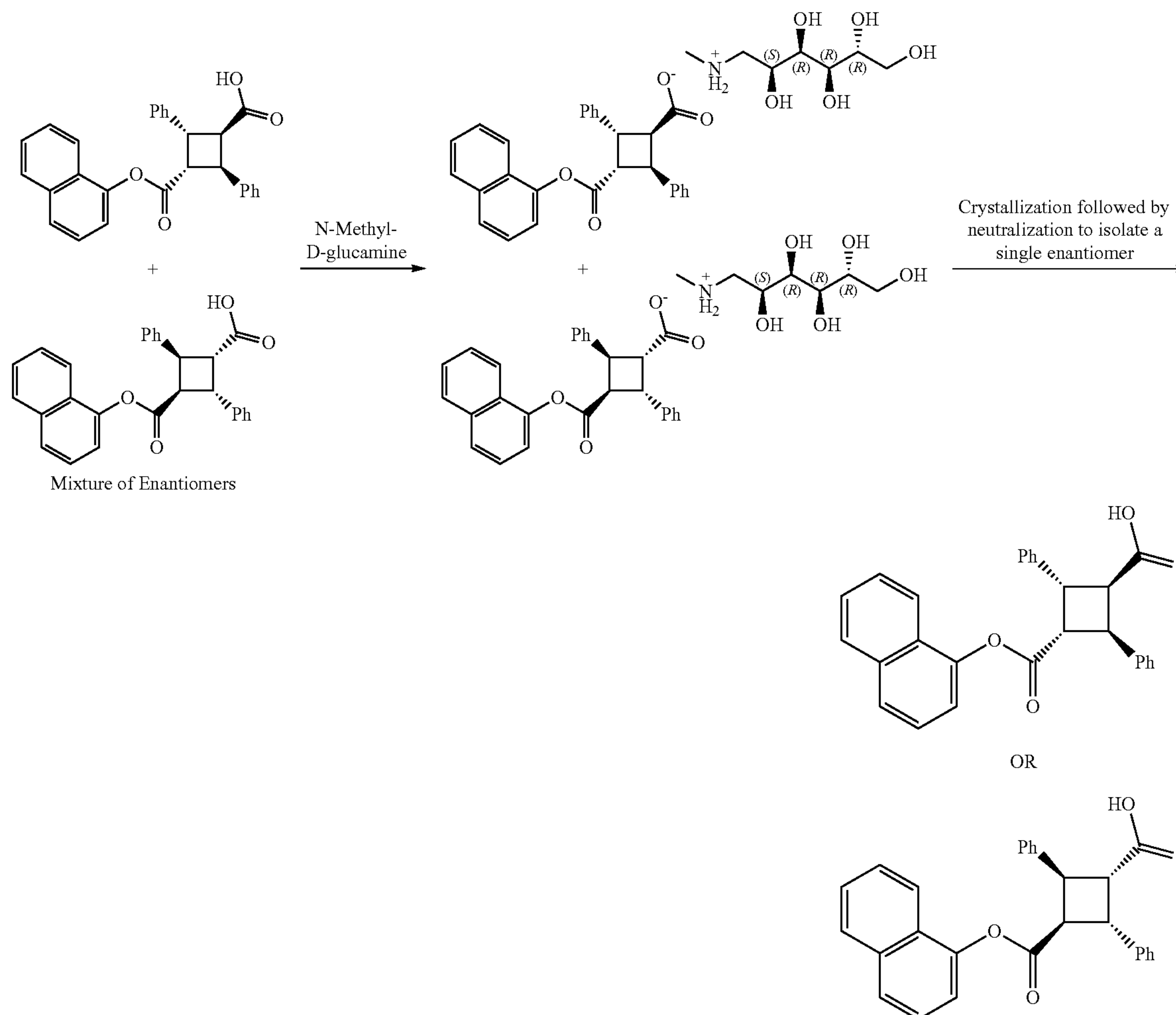
Scheme 12.
