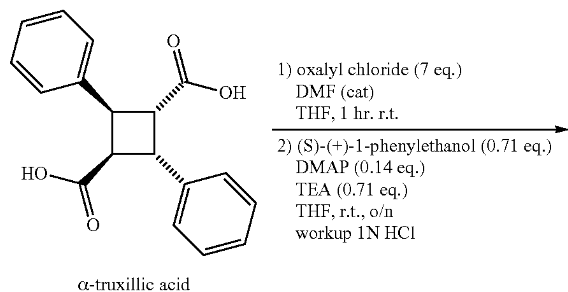
Scheme 6.
