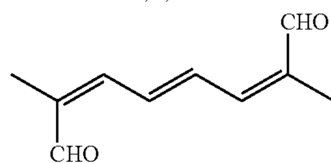
Z,E,Z-Isomer
