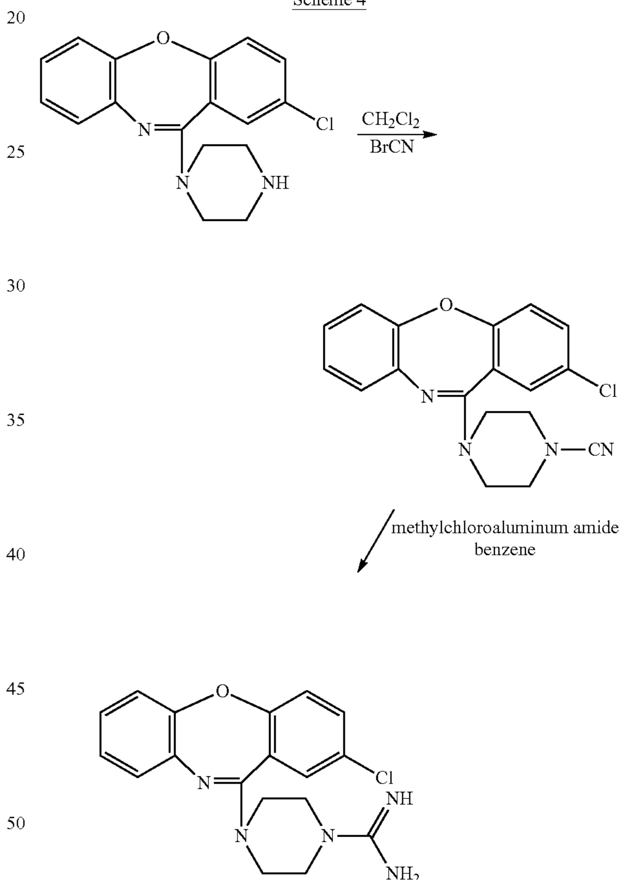
Scheme 4
