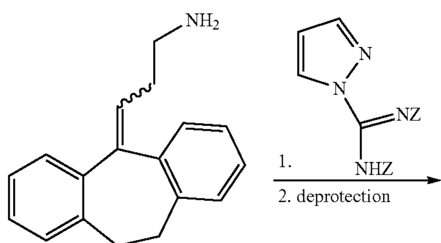
Scheme 3
