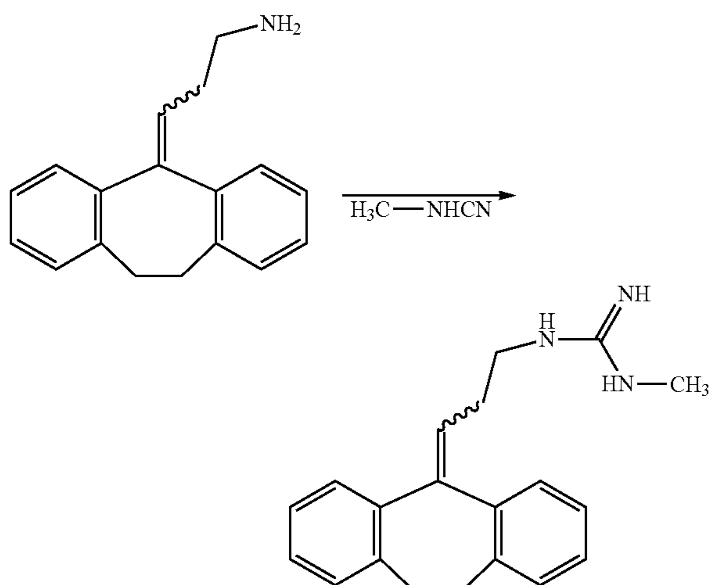
Scheme 2
