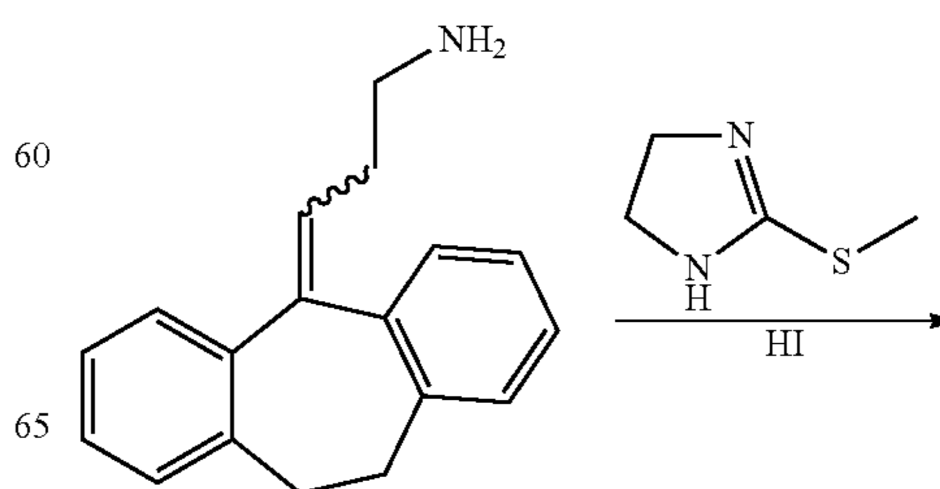
Scheme 5
