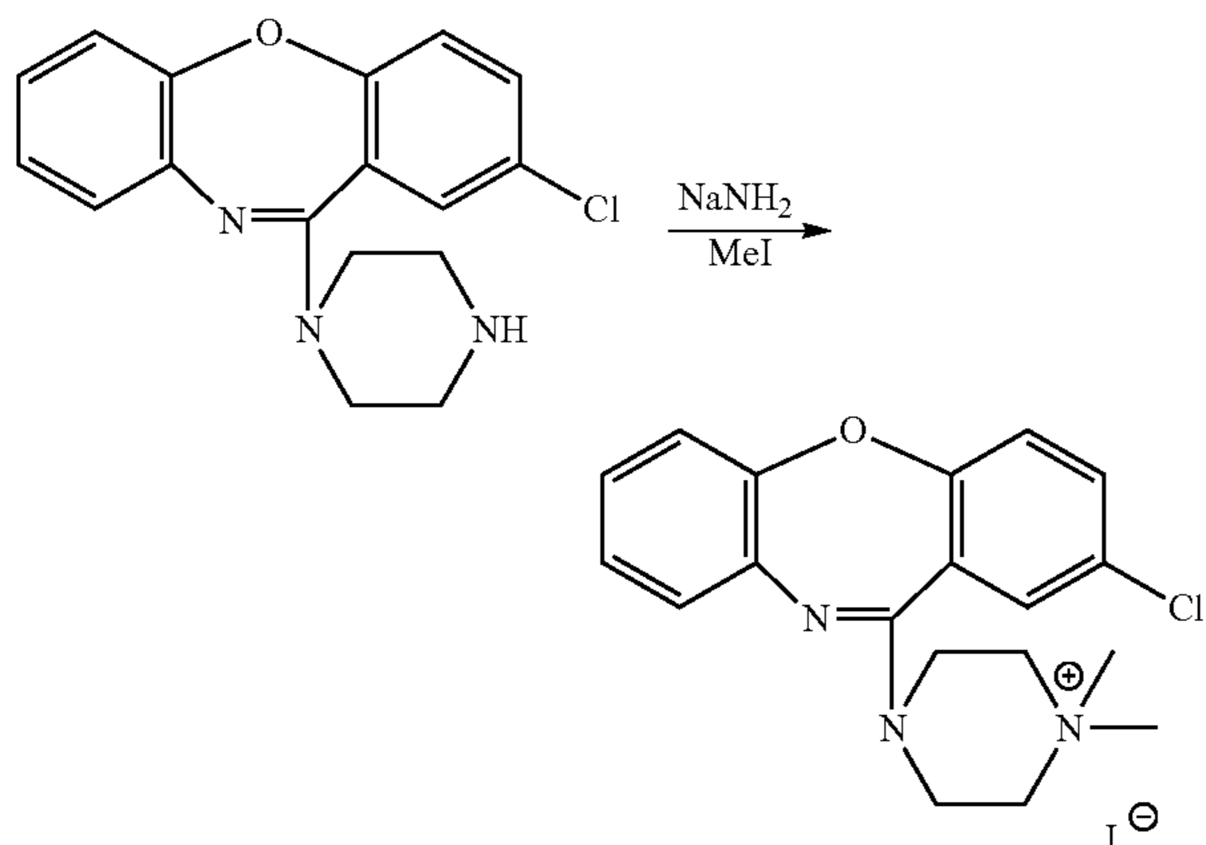
Scheme 1
