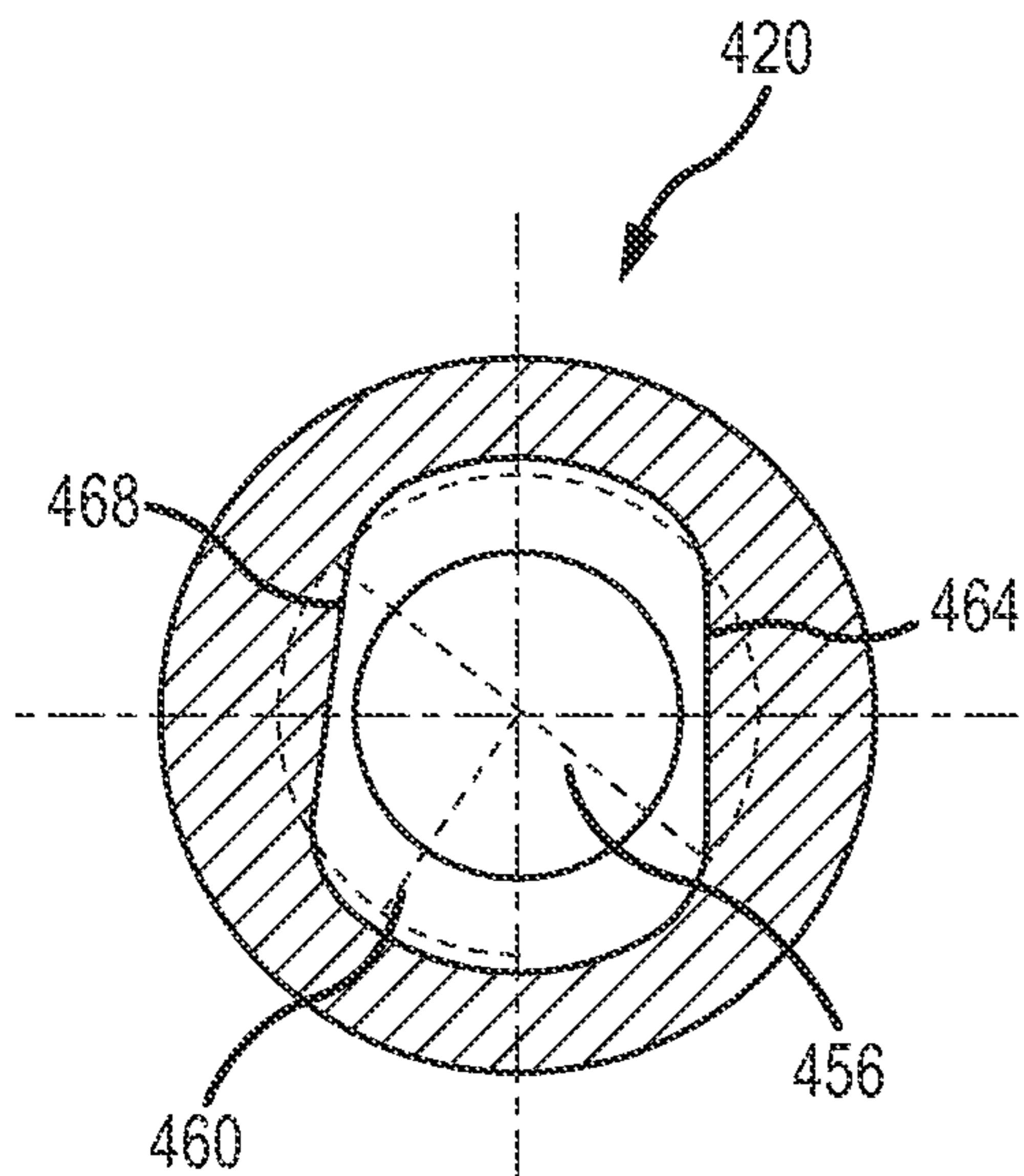
SECTION E-E
